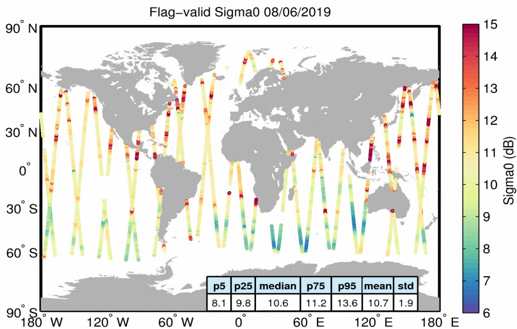
Figure 23. Geographical distribution of flag-valid sigma0 data over oceans and lakes for 08/06/2019. The statistical values shown in the table refer to the sigma0 in dB and are calculated over all measurements shown in the figure.
