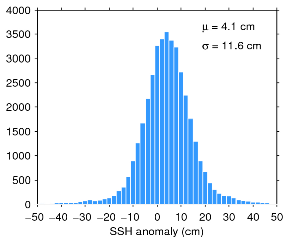
Figure 11. Histogram of science-valid SSH anomaly over oceans and lakes for 08/06/2019. The mean ( \mu ) and standard deviation ( \sigma ) are also shown. Note that values outside [-50 50] cm are excluded from the histogram for the sake of readability but not from the computation of \mu and \sigma .
