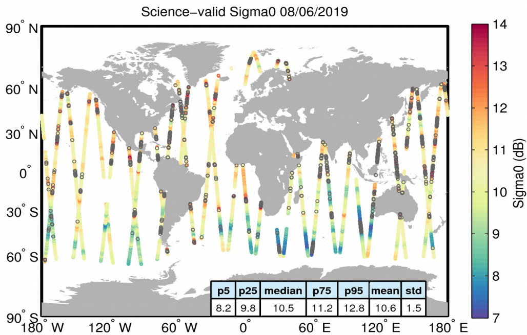
Figure 27. Geographical distribution of science-valid sigma0 data over oceans and lakes for 08/06/2019. The statistical values shown in the table refer to the sigma0 in dB and are calculated over all measurements shown in the figure. Gray circles denote records that have been rejected based on the editing criteria described in Table 4.
