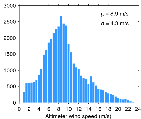
Figure 35. Histogram of science-valid wind over oceans and lakes for 08/06/2019. The mean ( \mu ) and standard deviation ( \sigma ) are also shown. Note that values larger than 24 m/s are excluded from the histogram for the sake of readability but not from the computation of \mu and \sigma .
