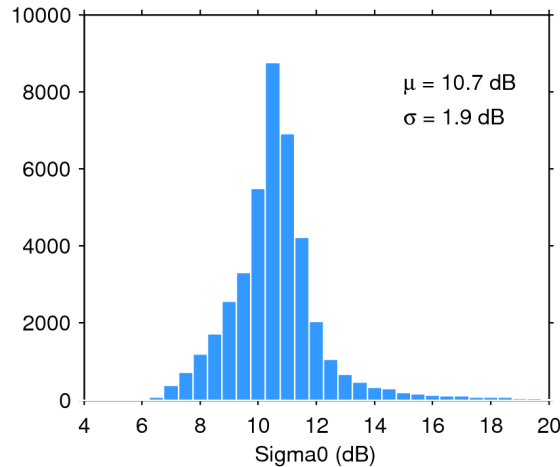
Figure 25. Histogram of flag-valid sigma0 over oceans and lakes for 08/06/2019. The mean ( \mu ) and standard deviation ( \sigma ) are also shown. Note that values outside [4 20] dB are excluded from the histogram for the sake of readability but not from the computation of \mu and \sigma .
