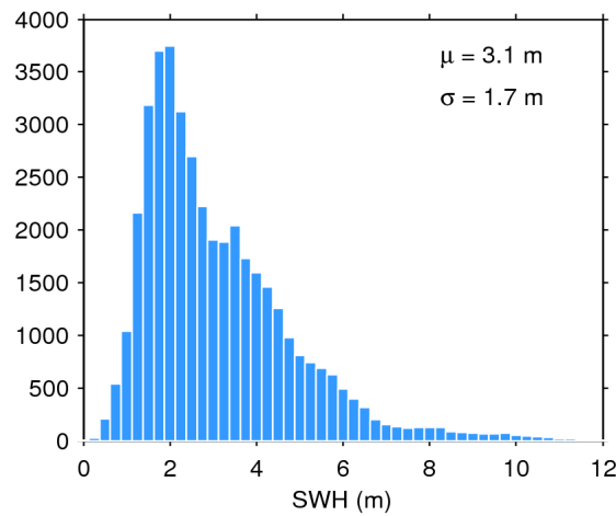
Figure 17. Histogram of flag-valid SWH over oceans and lakes for 08/06/2019. The mean ( \mu ) and standard deviation ( \sigma ) are also shown. Note that values larger than 12 m are excluded from the histogram for the sake of readability but not from the computation of \mu and \sigma .
