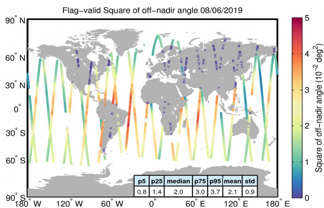
Figure 37. Geographical distribution of flag-valid mispointing data over oceans and lakes for 08/06/2019. The statistical values shown in the table refer to the mispointing in 10^{-2} \text{ deg}^2 and are calculated over all measurements shown in the figure.
