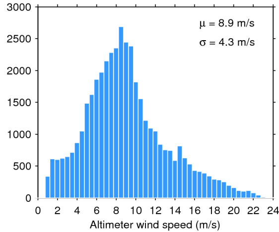
Figure 33. Histogram of flag-valid wind over oceans and lakes for 08/06/2019. The mean ( \mu ) and standard deviation ( \sigma ) are also shown. Note that values larger than 24 m/s are excluded from the histogram for the sake of readability but not from the computation of \mu and \sigma .
