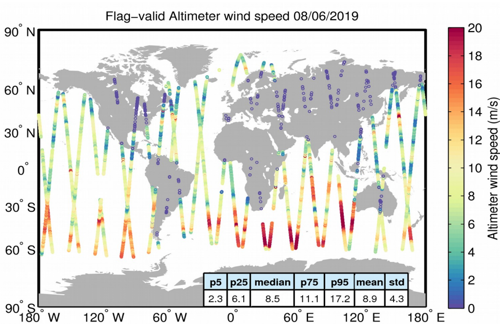
Figure 31. Geographical distribution of flag-valid wind data over oceans and lakes for 08/06/2019. The statistical values shown in the table refer to the wind in m/s and are calculated over all measurements shown in the figure.
