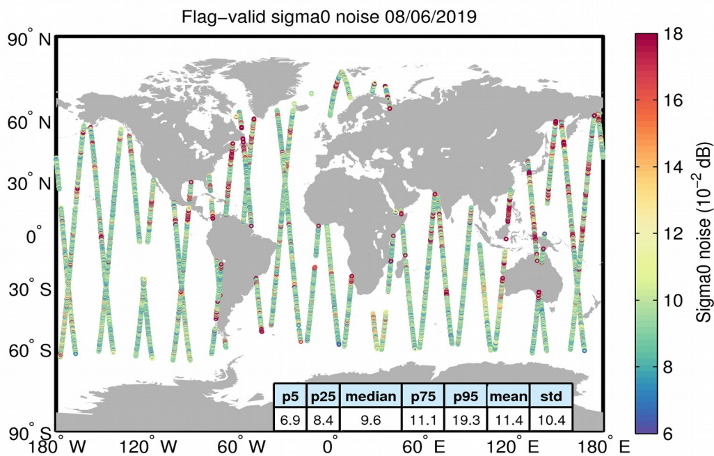
Figure 26. Geographical distribution of flag-valid 20-Hz sigma0 measurement noise over oceans and lakes for 08/06/2019. The statistical values shown in the table refer to the sigma0 noise and are calculated over all measurements shown in the figure.
