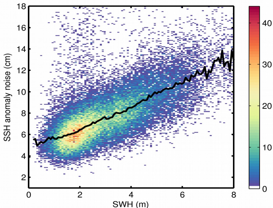
Figure 9. 2D histogram showing flag-valid SSH anomaly noise as a function of SWH for 08/06/2019. The black line denotes the median SSH anomaly noise as a function of SWH.
