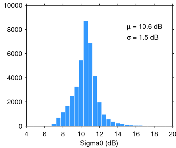
Figure 28. Histogram of science-valid sigma0 over oceans and lakes for 08/06/2019. The mean ( \mu ) and standard deviation ( \sigma ) are also shown. Note that values outside [4 20] dB are excluded from the histogram for the sake of readability but not from the computation of \mu and \sigma .
