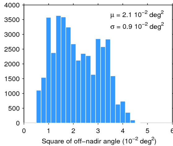
Figure 39. Histogram of flag-valid mispointing over oceans and lakes for 08/06/2019. The mean ( \mu ) and standard deviation ( \sigma ) are also shown. Note that values larger than 6 \cdot 10^{-2} \text{ deg}^2 are excluded from the histogram for the sake of readability but not from the computation of \mu and \sigma .
