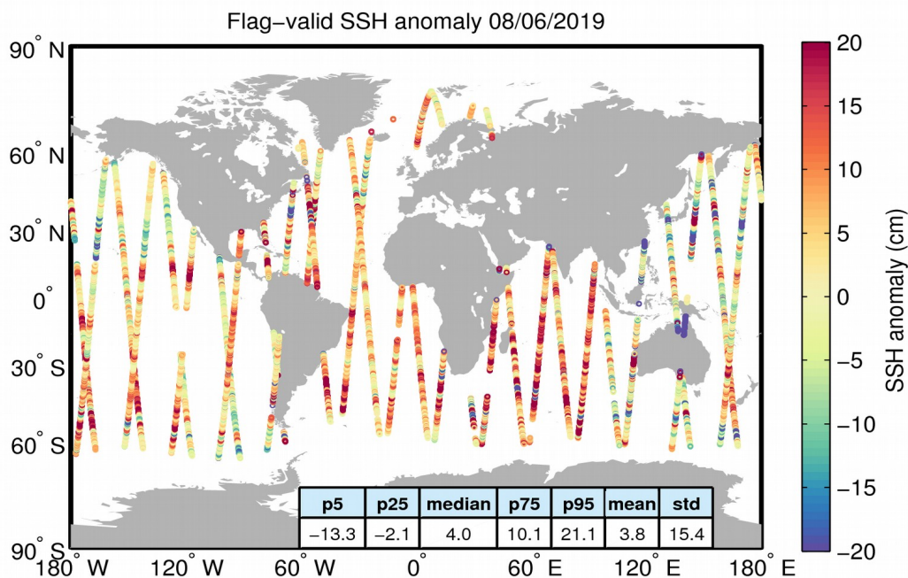
Figure 5. Geographical distribution of flag-valid 1-Hz SSH anomaly data over oceans and lakes for 08/06/2019. The statistical values shown in the table refer to the SSH anomaly in cm and are calculated over all measurements shown in the figure.
