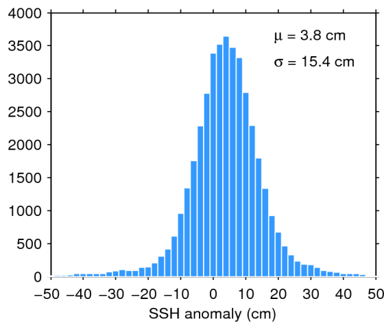
Figure 7. Histogram of flag-valid SSH anomaly over oceans and lakes for 08/06/2019. The mean ( \mu ) and standard deviation ( \sigma ) are also shown. Note that values outside [-50\ 50] cm are excluded from the histogram for the sake of readability but not from the computation of \mu and \sigma .
