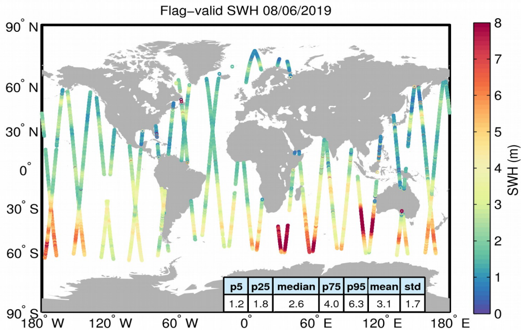
Figure 15. Geographical distribution of flag-valid SWH data over oceans and lakes for 08/06/2019. The statistical values shown in the table refer to the SWH in m and are calculated over all measurements shown in the figure.
