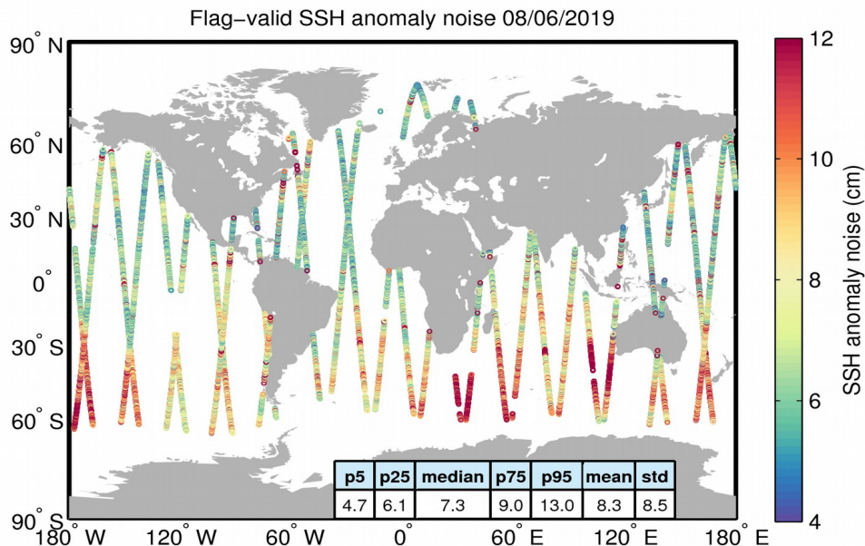
Figure 8. Geographical distribution of flag-valid 20-Hz SSH anomaly measurement noise over oceans and lakes for 08/06/2019. The statistical values shown in the table refer to the SSH anomaly noise and are calculated over all measurements shown in the figure.
