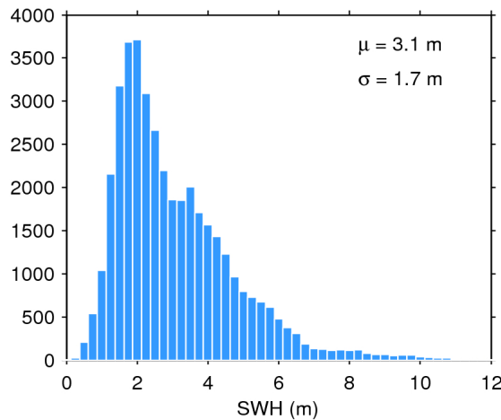
Figure 20. Histogram of science-valid SWH over oceans and lakes for 08/06/2019. The mean ( \mu ) and standard deviation ( \sigma ) are also shown. Note that values larger than 12 m are excluded from the histogram for the sake of readability but not from the computation of \mu and \sigma .
