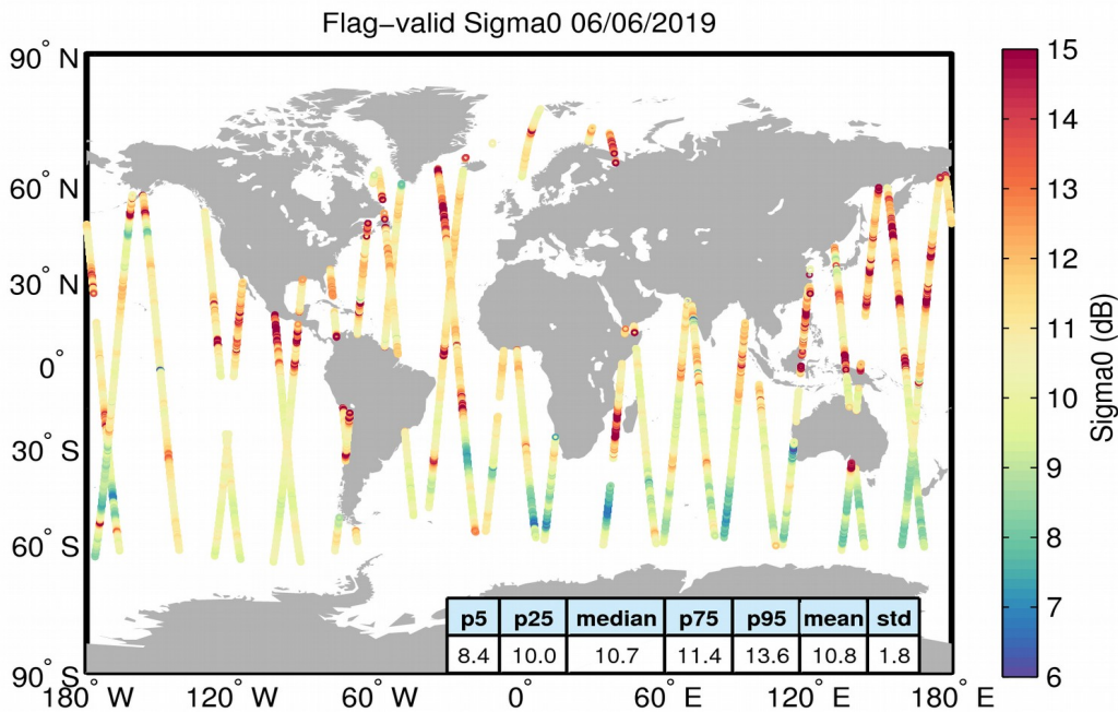
Figure 23. Geographical distribution of flag-valid sigma0 data over oceans and lakes for 06/06/2019. The statistical values shown in the table refer to the sigma0 in dB and are calculated over all measurements shown in the figure.
