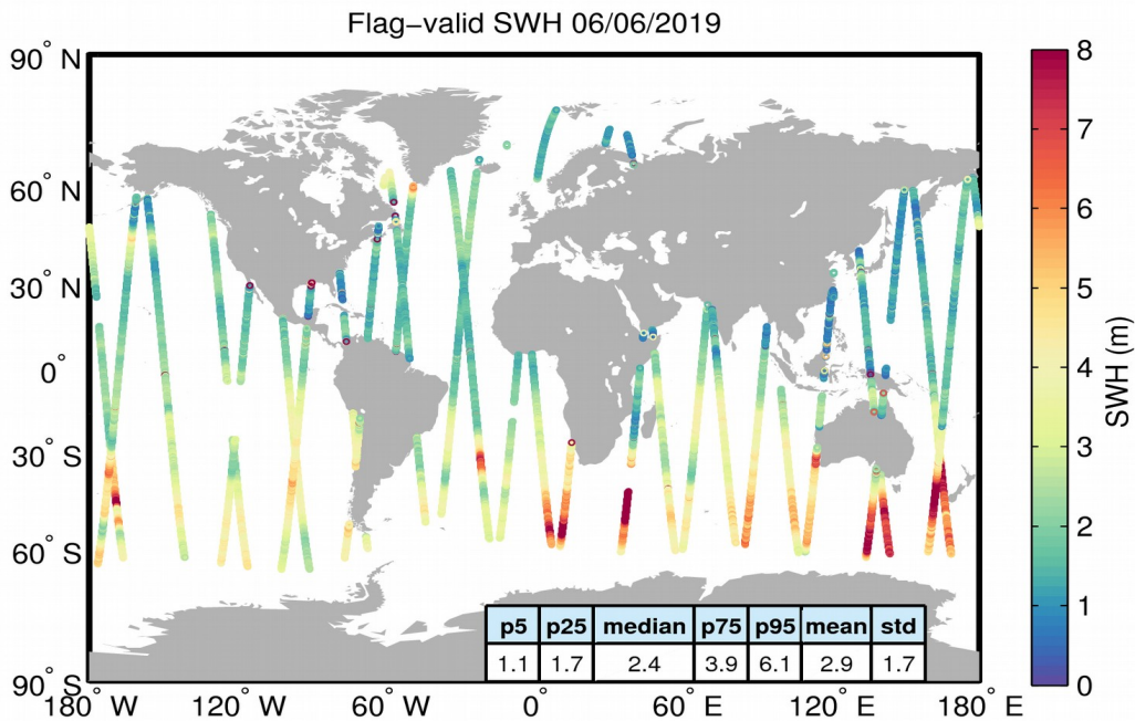
Figure 15. Geographical distribution of flag-valid SWH data over oceans and lakes for 06/06/2019. The statistical values shown in the table refer to the SWH in m and are calculated over all measurements shown in the figure.
