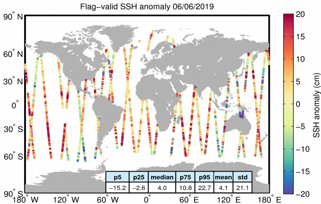
Figure 5. Geographical distribution of flag-valid 1-Hz SSH anomaly data over oceans and lakes for 06/06/2019. The statistical values shown in the table refer to the SSH anomaly in cm and are calculated over all measurements shown in the figure.
