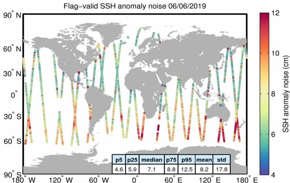
Figure 8. Geographical distribution of flag-valid 20-Hz SSH anomaly measurement noise over oceans and lakes for 06/06/2019. The statistical values shown in the table refer to the SSH anomaly noise and are calculated over all measurements shown in the figure.
