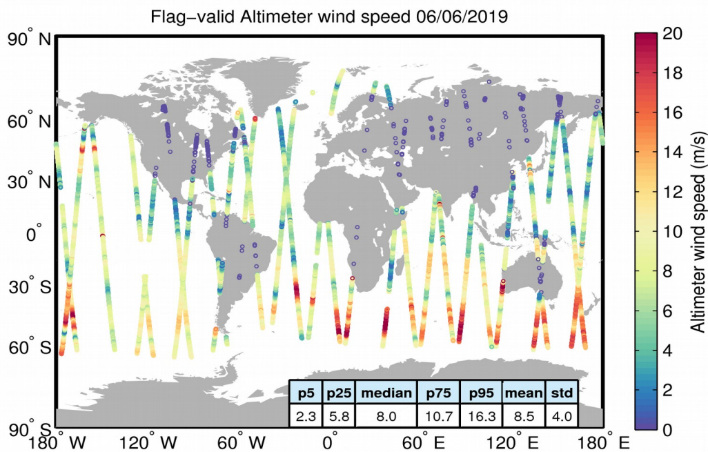
Figure 31. Geographical distribution of flag-valid wind data over oceans and lakes for 06/06/2019. The statistical values shown in the table refer to the wind in m/s and are calculated over all measurements shown in the figure.
