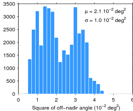
Figure 39. Histogram of flag-valid mispointing over oceans and lakes for 06/06/2019. The mean ( \mu ) and standard deviation ( \sigma ) are also shown. Note that values larger than 6 \cdot 10^{-2} \text{ deg}^2 are excluded from the histogram for the sake of readability but not from the computation of \mu and \sigma .
