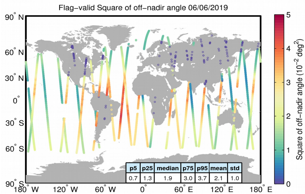
Figure 37. Geographical distribution of flag-valid mispointing data over oceans and lakes for 06/06/2019. The statistical values shown in the table refer to the mispointing in 10^{-2} deg 2 and are calculated over all measurements shown in the figure.
