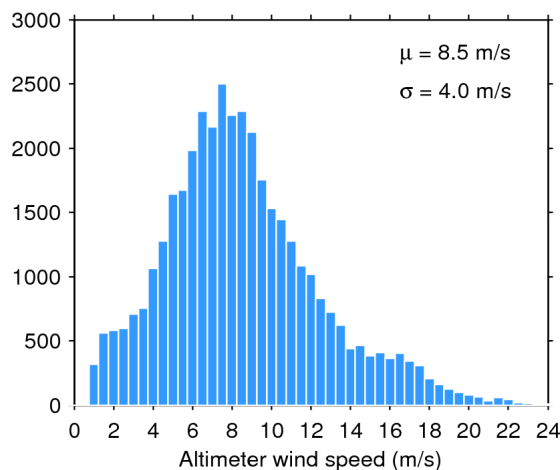
Figure 35. Histogram of science-valid wind over oceans and lakes for 06/06/2019. The mean ( \mu ) and standard deviation ( \sigma ) are also shown. Note that values larger than 24 m/s are excluded from the histogram for the sake of readability but not from the computation of \mu and \sigma .
