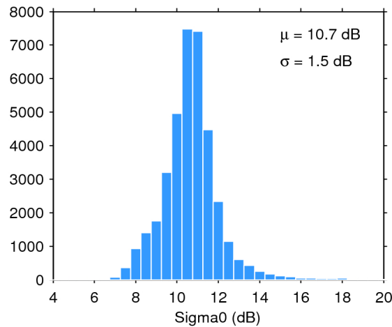
Figure 28. Histogram of science-valid sigma0 over oceans and lakes for 06/06/2019. The mean ( \mu ) and standard deviation ( \sigma ) are also shown. Note that values outside [4 20] dB are excluded from the histogram for the sake of readability but not from the computation of \mu and \sigma .
