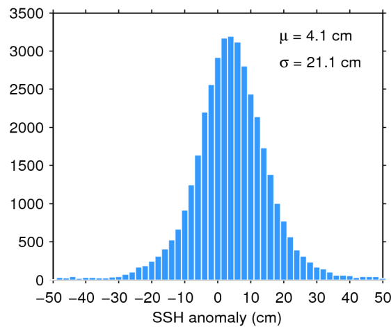
Figure 7. Histogram of flag-valid SSH anomaly over oceans and lakes for 06/06/2019. The mean ( \mu ) and standard deviation ( \sigma ) are also shown. Note that values outside [-50\ 50] cm are excluded from the histogram for the sake of readability but not from the computation of \mu and \sigma .
