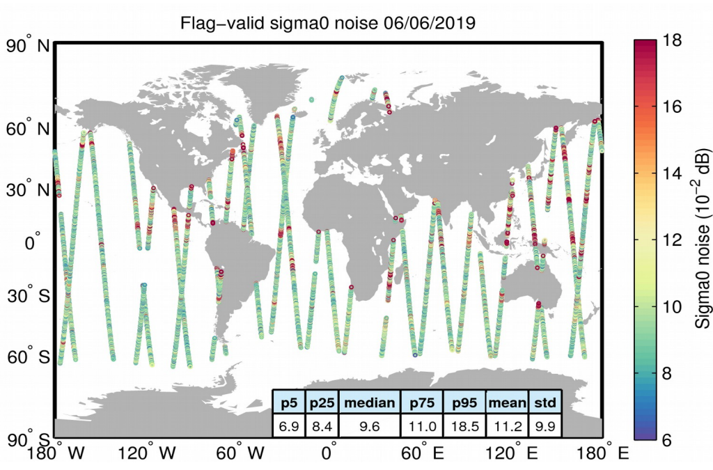
Figure 26. Geographical distribution of flag-valid 20-Hz sigma0 measurement noise over oceans and lakes for 06/06/2019. The statistical values shown in the table refer to the sigma0 noise and are calculated over all measurements shown in the figure.
