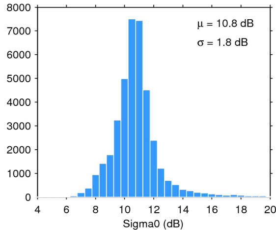
Figure 25. Histogram of flag-valid sigma0 over oceans and lakes for 06/06/2019. The mean ( \mu ) and standard deviation ( \sigma ) are also shown. Note that values outside [4 20] dB are excluded from the histogram for the sake of readability but not from the computation of \mu and \sigma .
