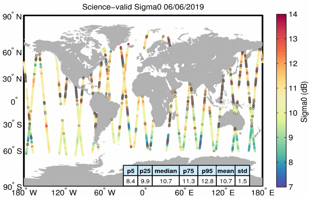
Figure 27. Geographical distribution of science-valid sigma0 data over oceans and lakes for 06/06/2019. The statistical values shown in the table refer to the sigma0 in dB and are calculated over all measurements shown in the figure. Gray circles denote records that have been rejected based on the editing criteria described in Table 4.
