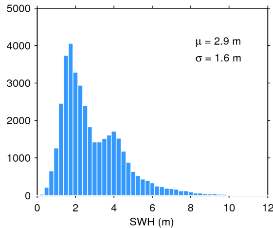
Figure 20. Histogram of science-valid SWH over oceans and lakes for 06/06/2019. The mean ( \mu ) and standard deviation ( \sigma ) are also shown. Note that values larger than 12 m are excluded from the histogram for the sake of readability but not from the computation of \mu and \sigma .
