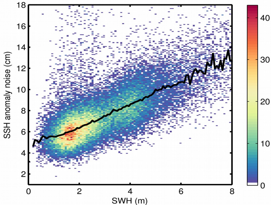
Figure 9. 2D histogram showing flag-valid SSH anomaly noise as a function of SWH for 06/06/2019. The black line denotes the median SSH anomaly noise as a function of SWH.
