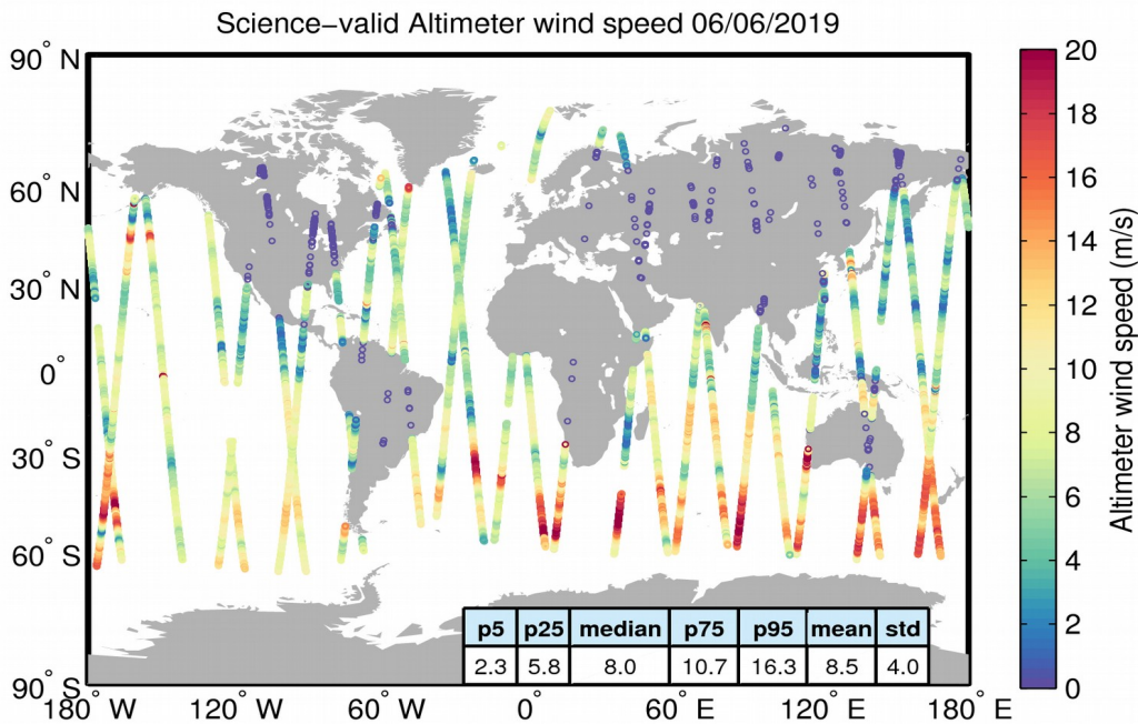
Figure 34. Geographical distribution of science-valid wind data over oceans and lakes for 06/06/2019. The statistical values shown in the table refer to the wind in m/s and are calculated over all measurements shown in the figure. Gray circles denote records that have been rejected based on the editing criteria described in Table 5.
