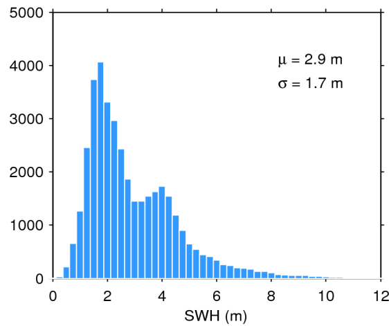
Figure 17. Histogram of flag-valid SWH over oceans and lakes for 06/06/2019. The mean ( \mu ) and standard deviation ( \sigma ) are also shown. Note that values larger than 12 m are excluded from the histogram for the sake of readability but not from the computation of \mu and \sigma .
