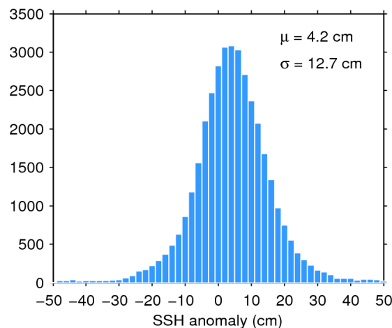
Figure 11. Histogram of science-valid SSH anomaly over oceans and lakes for 06/06/2019. The mean ( \mu ) and standard deviation ( \sigma ) are also shown. Note that values outside [-50 50] cm are excluded from the histogram for the sake of readability but not from the computation of \mu and \sigma .
