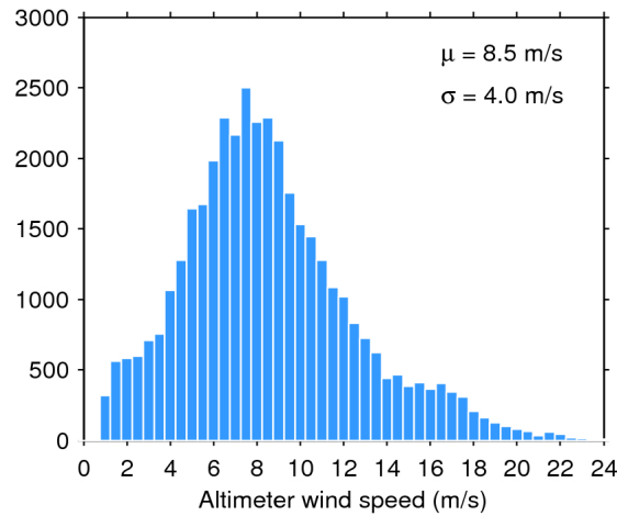
Figure 33. Histogram of flag-valid wind over oceans and lakes for 06/06/2019. The mean ( \mu ) and standard deviation ( \sigma ) are also shown. Note that values larger than 24 m/s are excluded from the histogram for the sake of readability but not from the computation of \mu and \sigma .
