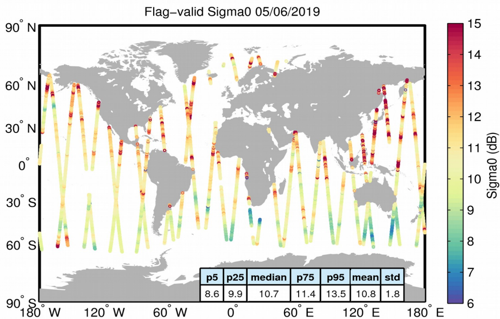
Figure 23. Geographical distribution of flag-valid sigma0 data over oceans and lakes for 05/06/2019. The statistical values shown in the table refer to the sigma0 in dB and are calculated over all measurements shown in the figure.
