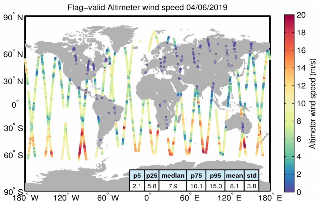
Figure 31. Geographical distribution of flag-valid wind data over oceans and lakes for 04/06/2019. The statistical values shown in the table refer to the wind in m/s and are calculated over all measurements shown in the figure.
