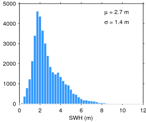
Figure 20. Histogram of science-valid SWH over oceans and lakes for 04/06/2019. The mean ( \mu ) and standard deviation ( \sigma ) are also shown. Note that values larger than 12 m are excluded from the histogram for the sake of readability but not from the computation of \mu and \sigma .
