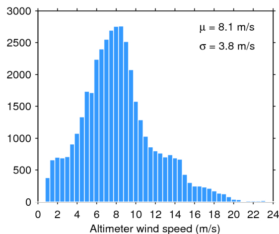
Figure 35. Histogram of science-valid wind over oceans and lakes for 04/06/2019. The mean ( \mu ) and standard deviation ( \sigma ) are also shown. Note that values larger than 24 m/s are excluded from the histogram for the sake of readability but not from the computation of \mu and \sigma .
