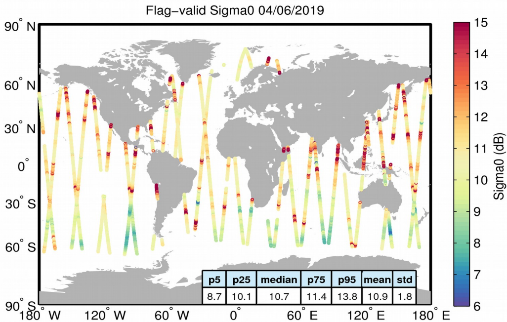
Figure 23. Geographical distribution of flag-valid sigma0 data over oceans and lakes for 04/06/2019. The statistical values shown in the table refer to the sigma0 in dB and are calculated over all measurements shown in the figure.
