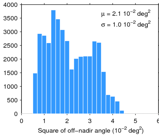
Figure 39. Histogram of flag-valid mispointing over oceans and lakes for 04/06/2019. The mean ( \mu ) and standard deviation ( \sigma ) are also shown. Note that values larger than 6 \cdot 10^{-2} \text{ deg}^2 are excluded from the histogram for the sake of readability but not from the computation of \mu and \sigma .
