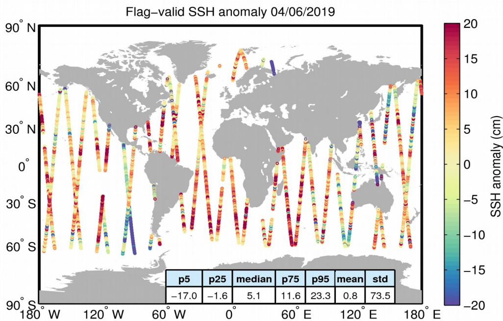
Figure 5. Geographical distribution of flag-valid 1-Hz SSH anomaly data over oceans and lakes for 04/06/2019. The statistical values shown in the table refer to the SSH anomaly in cm and are calculated over all measurements shown in the figure.
