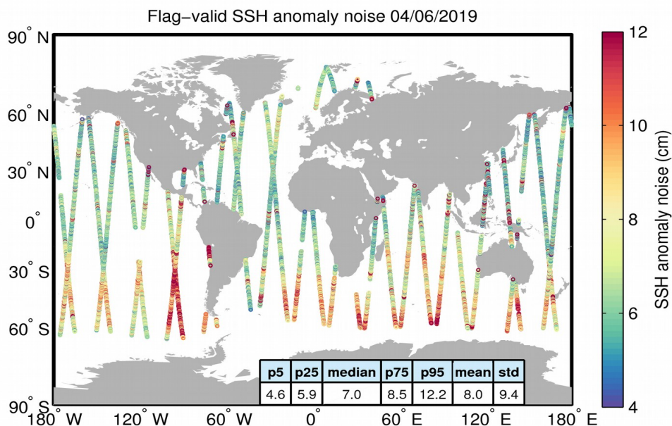
Figure 8. Geographical distribution of flag-valid 20-Hz SSH anomaly measurement noise over oceans and lakes for 04/06/2019. The statistical values shown in the table refer to the SSH anomaly noise and are calculated over all measurements shown in the figure.
