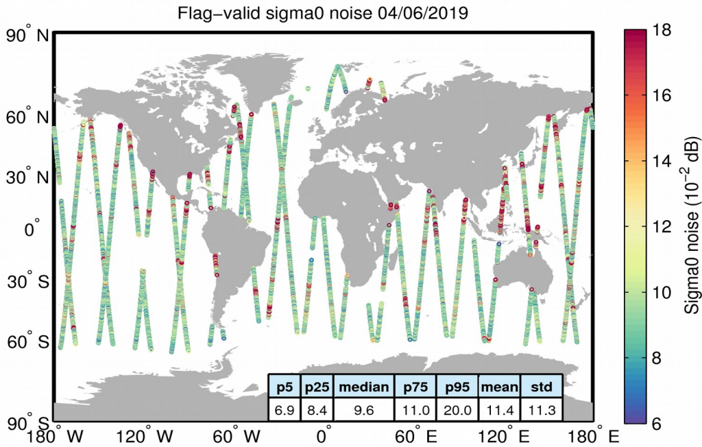
Figure 26. Geographical distribution of flag-valid 20-Hz sigma0 measurement noise over oceans and lakes for 04/06/2019. The statistical values shown in the table refer to the sigma0 noise and are calculated over all measurements shown in the figure.
