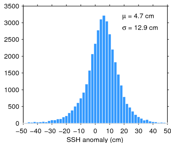
Figure 11. Histogram of science-valid SSH anomaly over oceans and lakes for 04/06/2019. The mean ( \mu ) and standard deviation ( \sigma ) are also shown. Note that values outside [-50 50] cm are excluded from the histogram for the sake of readability but not from the computation of \mu and \sigma .
