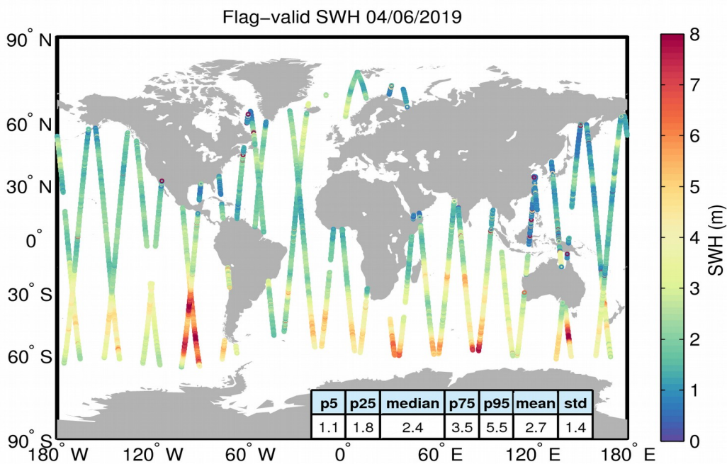
Figure 15. Geographical distribution of flag-valid SWH data over oceans and lakes for 04/06/2019. The statistical values shown in the table refer to the SWH in m and are calculated over all measurements shown in the figure.
