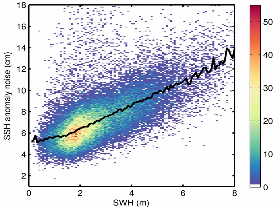
Figure 9. 2D histogram showing flag-valid SSH anomaly noise as a function of SWH for 04/06/2019. The black line denotes the median SSH anomaly noise as a function of SWH.
