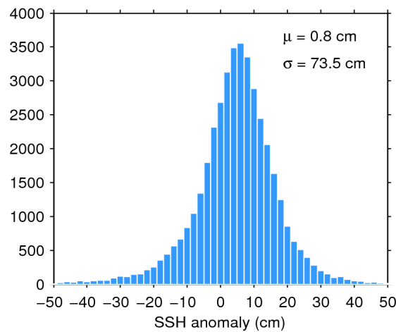
Figure 7. Histogram of flag-valid SSH anomaly over oceans and lakes for 04/06/2019. The mean ( \mu ) and standard deviation ( \sigma ) are also shown. Note that values outside [-50\ 50] cm are excluded from the histogram for the sake of readability but not from the computation of \mu and \sigma .
