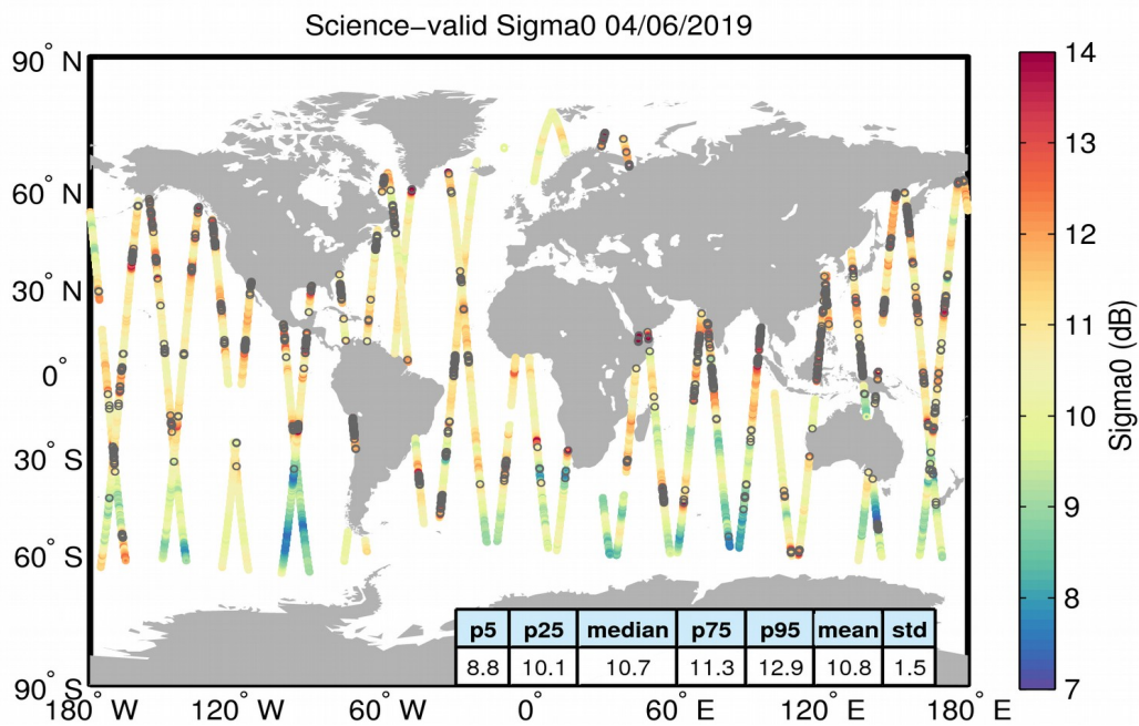
Figure 27. Geographical distribution of science-valid sigma0 data over oceans and lakes for 04/06/2019. The statistical values shown in the table refer to the sigma0 in dB and are calculated over all measurements shown in the figure. Gray circles denote records that have been rejected based on the editing criteria described in Table 4.
