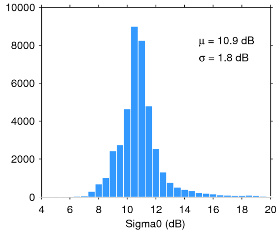
Figure 25. Histogram of flag-valid sigma0 over oceans and lakes for 04/06/2019. The mean ( \mu ) and standard deviation ( \sigma ) are also shown. Note that values outside [4 20] dB are excluded from the histogram for the sake of readability but not from the computation of \mu and \sigma .
