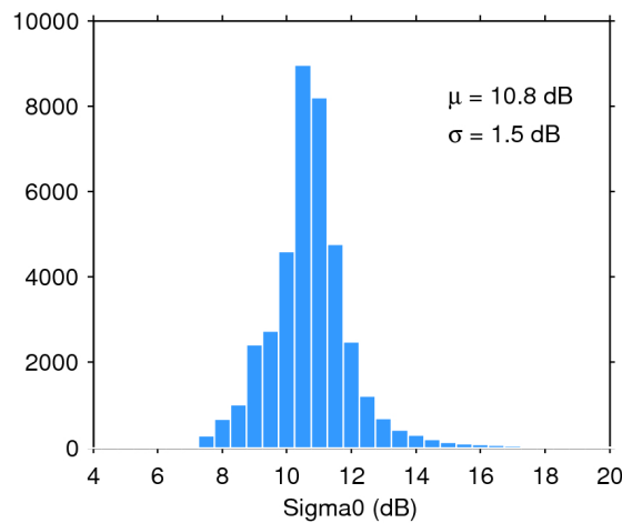
Figure 28. Histogram of science-valid sigma0 over oceans and lakes for 04/06/2019. The mean ( \mu ) and standard deviation ( \sigma ) are also shown. Note that values outside [4 20] dB are excluded from the histogram for the sake of readability but not from the computation of \mu and \sigma .
