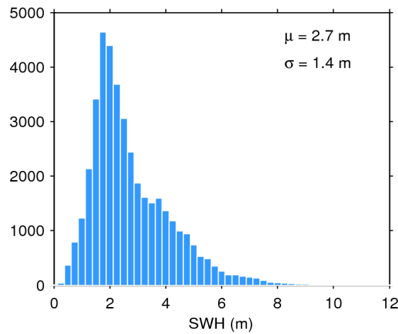
Figure 17. Histogram of flag-valid SWH over oceans and lakes for 04/06/2019. The mean ( \mu ) and standard deviation ( \sigma ) are also shown. Note that values larger than 12 m are excluded from the histogram for the sake of readability but not from the computation of \mu and \sigma .
