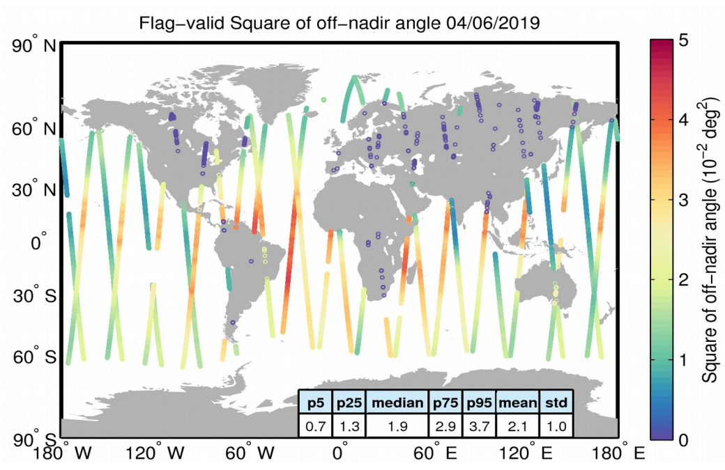
Figure 37. Geographical distribution of flag-valid mispointing data over oceans and lakes for 04/06/2019. The statistical values shown in the table refer to the mispointing in 10^{-2} \text{ deg}^2 and are calculated over all measurements shown in the figure.
