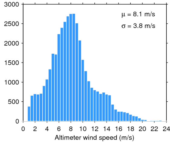
Figure 33. Histogram of flag-valid wind over oceans and lakes for 04/06/2019. The mean ( \mu ) and standard deviation ( \sigma ) are also shown. Note that values larger than 24 m/s are excluded from the histogram for the sake of readability but not from the computation of \mu and \sigma .
