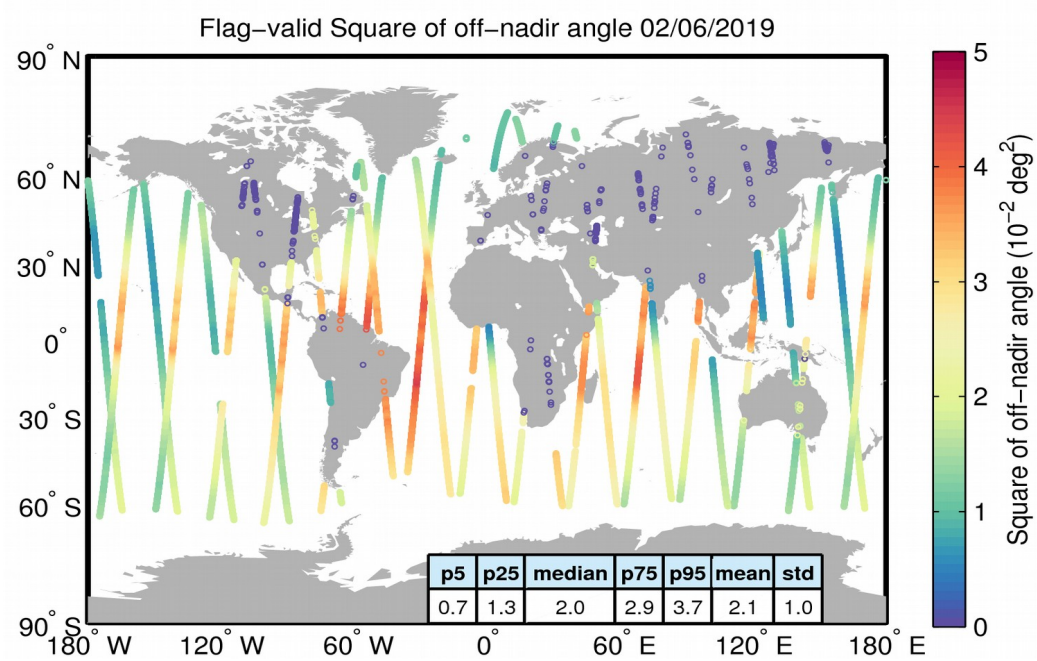
Figure 37. Geographical distribution of flag-valid mispointing data over oceans and lakes for 02/06/2019. The statistical values shown in the table refer to the mispointing in 10^{-2} \text{ deg}^2 and are calculated over all measurements shown in the figure.
