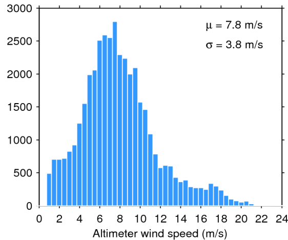
Figure 33. Histogram of flag-valid wind over oceans and lakes for 02/06/2019. The mean ( \mu ) and standard deviation ( \sigma ) are also shown. Note that values larger than 24 m/s are excluded from the histogram for the sake of readability but not from the computation of \mu and \sigma .
