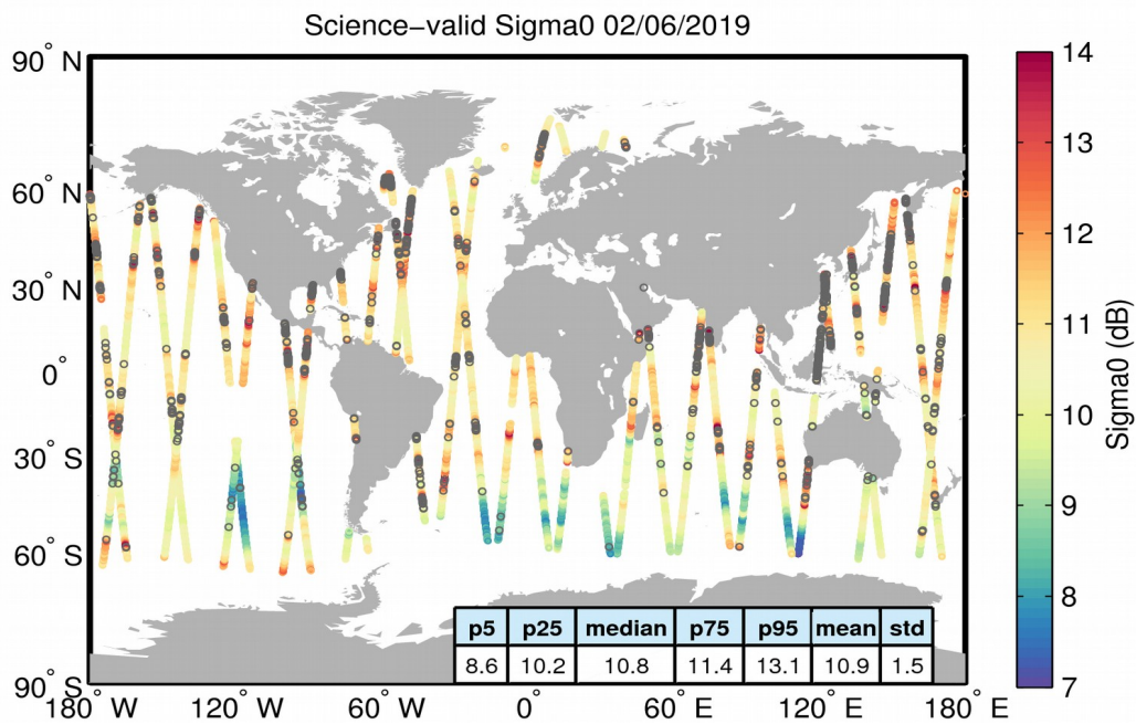
Figure 27. Geographical distribution of science-valid sigma0 data over oceans and lakes for 02/06/2019. The statistical values shown in the table refer to the sigma0 in dB and are calculated over all measurements shown in the figure. Gray circles denote records that have been rejected based on the editing criteria described in Table 4.
