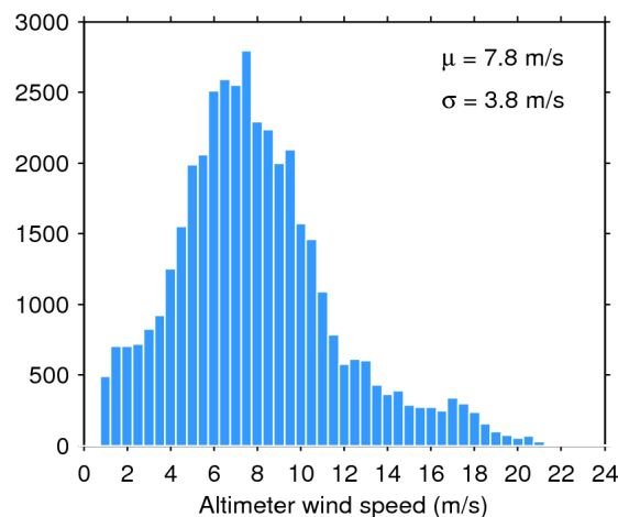
Figure 35. Histogram of science-valid wind over oceans and lakes for 02/06/2019. The mean ( \mu ) and standard deviation ( \sigma ) are also shown. Note that values larger than 24 m/s are excluded from the histogram for the sake of readability but not from the computation of \mu and \sigma .
