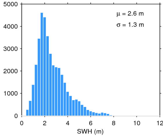
Figure 20. Histogram of science-valid SWH over oceans and lakes for 02/06/2019. The mean ( \mu ) and standard deviation ( \sigma ) are also shown. Note that values larger than 12 m are excluded from the histogram for the sake of readability but not from the computation of \mu and \sigma .
