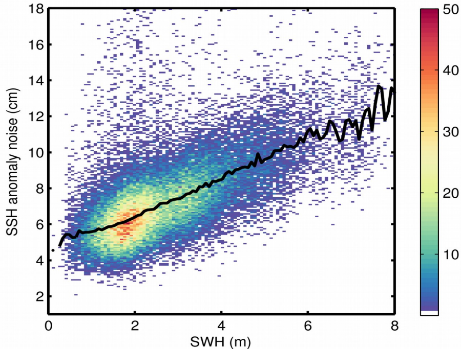
Figure 9. 2D histogram showing flag-valid SSH anomaly noise as a function of SWH for 02/06/2019. The black line denotes the median SSH anomaly noise as a function of SWH.
