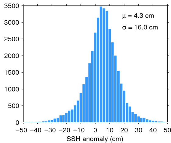
Figure 7. Histogram of flag-valid SSH anomaly over oceans and lakes for 02/06/2019. The mean ( \mu ) and standard deviation ( \sigma ) are also shown. Note that values outside [-50\ 50] cm are excluded from the histogram for the sake of readability but not from the computation of \mu and \sigma .
