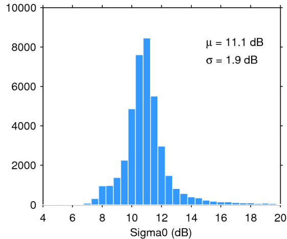
Figure 25. Histogram of flag-valid sigma0 over oceans and lakes for 02/06/2019. The mean ( \mu ) and standard deviation ( \sigma ) are also shown. Note that values outside [4 20] dB are excluded from the histogram for the sake of readability but not from the computation of \mu and \sigma .
