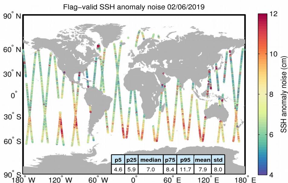
Figure 8. Geographical distribution of flag-valid 20-Hz SSH anomaly measurement noise over oceans and lakes for 02/06/2019. The statistical values shown in the table refer to the SSH anomaly noise and are calculated over all measurements shown in the figure.
