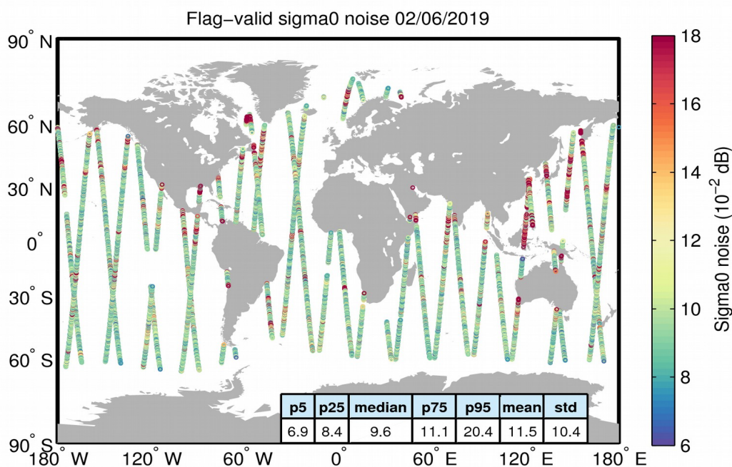
Figure 26. Geographical distribution of flag-valid 20-Hz sigma0 measurement noise over oceans and lakes for 02/06/2019. The statistical values shown in the table refer to the sigma0 noise and are calculated over all measurements shown in the figure.
