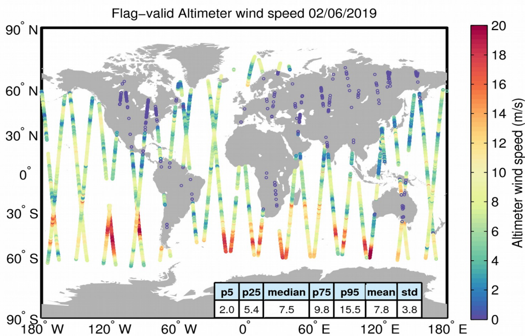
Figure 31. Geographical distribution of flag-valid wind data over oceans and lakes for 02/06/2019. The statistical values shown in the table refer to the wind in m/s and are calculated over all measurements shown in the figure.
