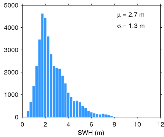
Figure 17. Histogram of flag-valid SWH over oceans and lakes for 02/06/2019. The mean ( \mu ) and standard deviation ( \sigma ) are also shown. Note that values larger than 12 m are excluded from the histogram for the sake of readability but not from the computation of \mu and \sigma .
