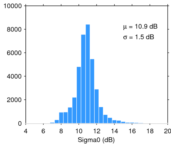
Figure 28. Histogram of science-valid sigma0 over oceans and lakes for 02/06/2019. The mean ( \mu ) and standard deviation ( \sigma ) are also shown. Note that values outside [4 20] dB are excluded from the histogram for the sake of readability but not from the computation of \mu and \sigma .
