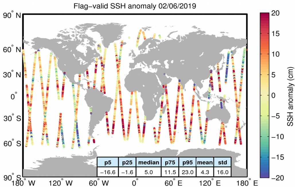
Figure 5. Geographical distribution of flag-valid 1-Hz SSH anomaly data over oceans and lakes for 02/06/2019. The statistical values shown in the table refer to the SSH anomaly in cm and are calculated over all measurements shown in the figure.
