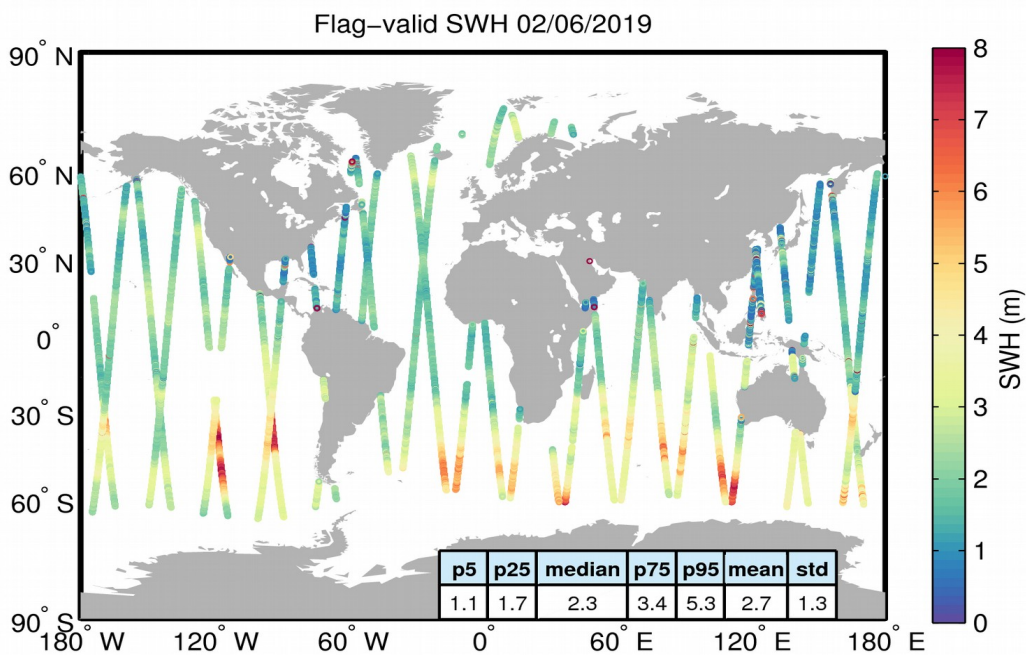
Figure 15. Geographical distribution of flag-valid SWH data over oceans and lakes for 02/06/2019. The statistical values shown in the table refer to the SWH in m and are calculated over all measurements shown in the figure.
