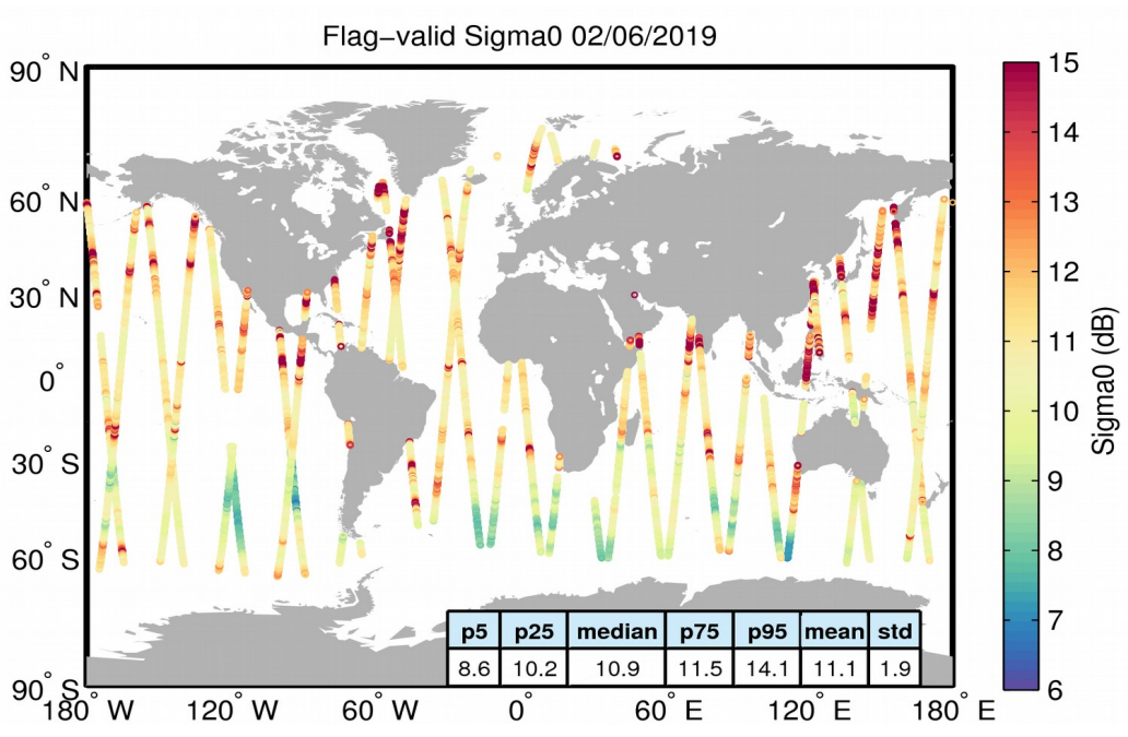
Figure 23. Geographical distribution of flag-valid sigma0 data over oceans and lakes for 02/06/2019. The statistical values shown in the table refer to the sigma0 in dB and are calculated over all measurements shown in the figure.
