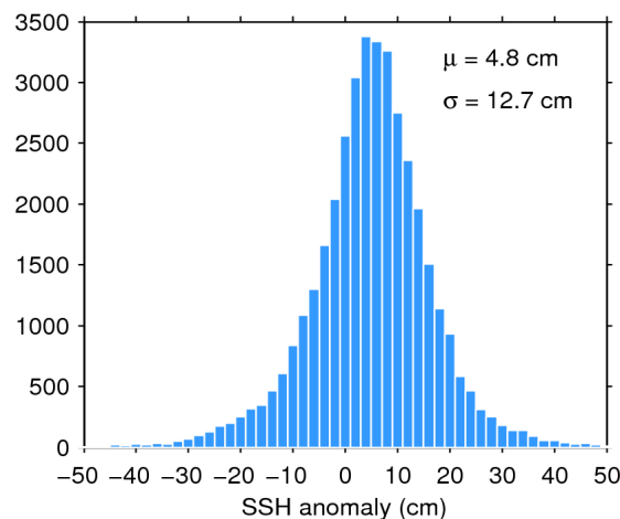
Figure 11. Histogram of science-valid SSH anomaly over oceans and lakes for 02/06/2019. The mean ( \mu ) and standard deviation ( \sigma ) are also shown. Note that values outside [-50 50] cm are excluded from the histogram for the sake of readability but not from the computation of \mu and \sigma .
