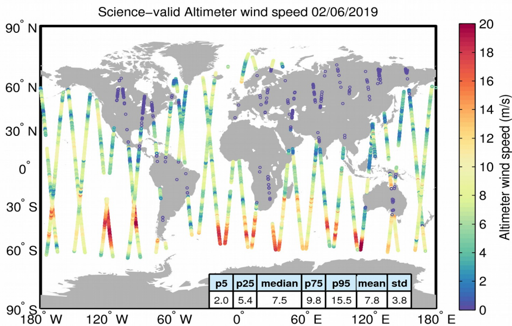
Figure 34. Geographical distribution of science-valid wind data over oceans and lakes for 02/06/2019. The statistical values shown in the table refer to the wind in m/s and are calculated over all measurements shown in the figure. Gray circles denote records that have been rejected based on the editing criteria described in Table 5.
