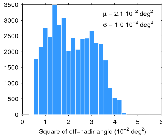
Figure 39. Histogram of flag-valid mispointing over oceans and lakes for 02/06/2019. The mean ( \mu ) and standard deviation ( \sigma ) are also shown. Note that values larger than 6 \cdot 10^{-2} \text{ deg}^2 are excluded from the histogram for the sake of readability but not from the computation of \mu and \sigma .
