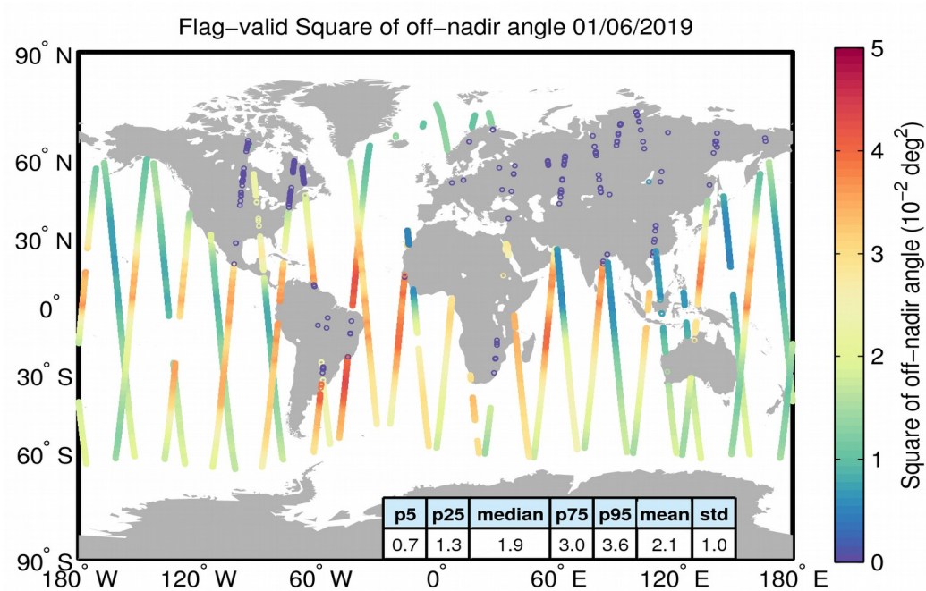
Figure 37. Geographical distribution of flag-valid mispointing data over oceans and lakes for 01/06/2019. The statistical values shown in the table refer to the mispointing in 10^{-2} deg 2 and are calculated over all measurements shown in the figure.
