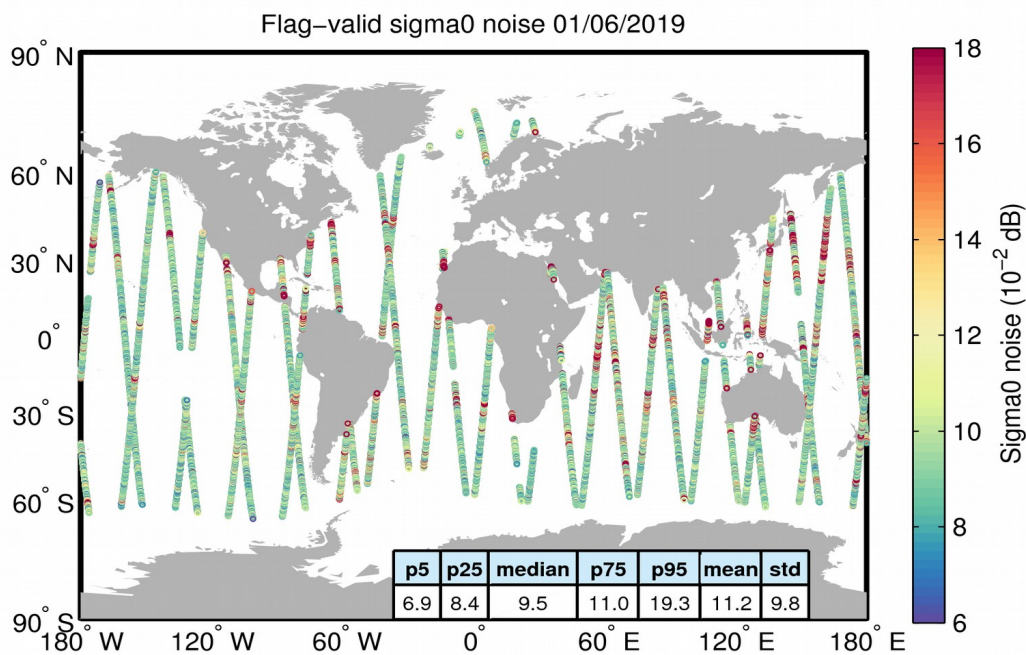
Figure 26. Geographical distribution of flag-valid 20-Hz sigma0 measurement noise over oceans and lakes for 01/06/2019. The statistical values shown in the table refer to the sigma0 noise and are calculated over all measurements shown in the figure.
