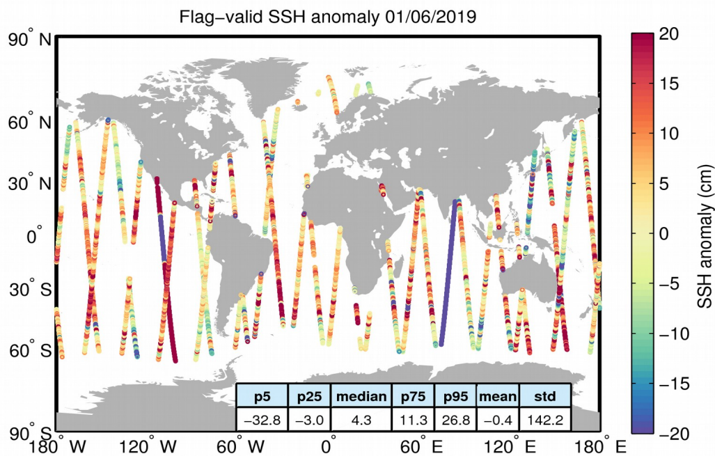
Figure 5. Geographical distribution of flag-valid 1-Hz SSH anomaly data over oceans and lakes for 01/06/2019. The statistical values shown in the table refer to the SSH anomaly in cm and are calculated over all measurements shown in the figure.
