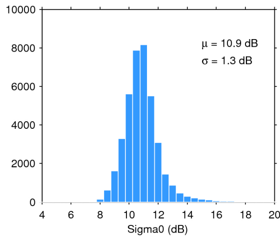
Figure 28. Histogram of science-valid sigma0 over oceans and lakes for 01/06/2019. The mean ( \mu ) and standard deviation ( \sigma ) are also shown. Note that values outside [4 20] dB are excluded from the histogram for the sake of readability but not from the computation of \mu and \sigma .
