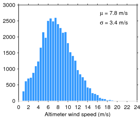
Figure 35. Histogram of science-valid wind over oceans and lakes for 01/06/2019. The mean ( \mu ) and standard deviation ( \sigma ) are also shown. Note that values larger than 24 m/s are excluded from the histogram for the sake of readability but not from the computation of \mu and \sigma .
