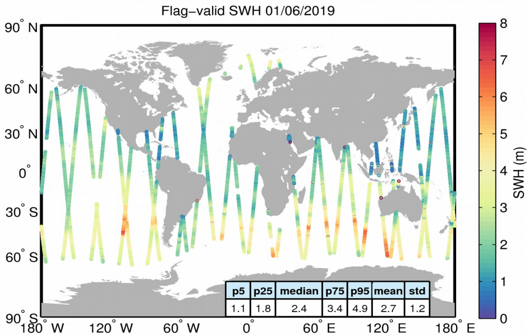
Figure 15. Geographical distribution of flag-valid SWH data over oceans and lakes for 01/06/2019. The statistical values shown in the table refer to the SWH in m and are calculated over all measurements shown in the figure.
