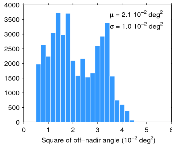
Figure 39. Histogram of flag-valid mispointing over oceans and lakes for 01/06/2019. The mean ( \mu ) and standard deviation ( \sigma ) are also shown. Note that values larger than 6 \cdot 10^{-2} \text{ deg}^2 are excluded from the histogram for the sake of readability but not from the computation of \mu and \sigma .
