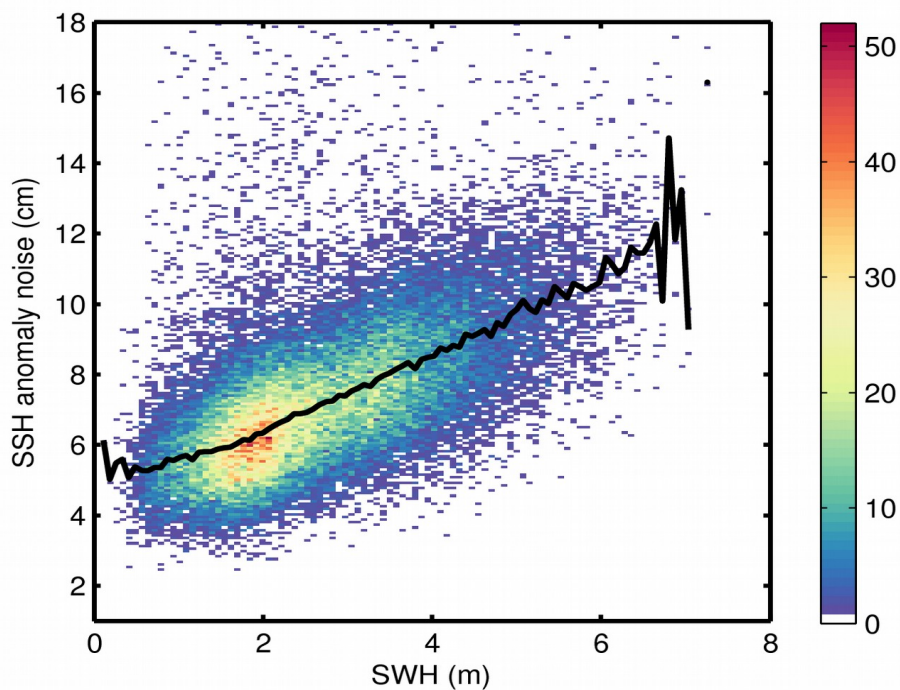
Figure 9. 2D histogram showing flag-valid SSH anomaly noise as a function of SWH for 01/06/2019. The black line denotes the median SSH anomaly noise as a function of SWH.
