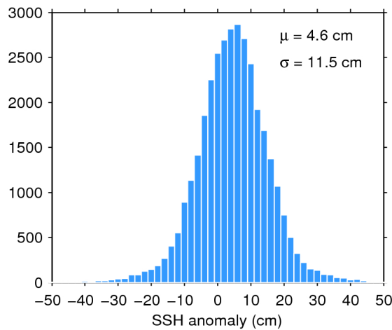
Figure 11. Histogram of science-valid SSH anomaly over oceans and lakes for 01/06/2019. The mean ( \mu ) and standard deviation ( \sigma ) are also shown. Note that values outside [-50 50] cm are excluded from the histogram for the sake of readability but not from the computation of \mu and \sigma .
