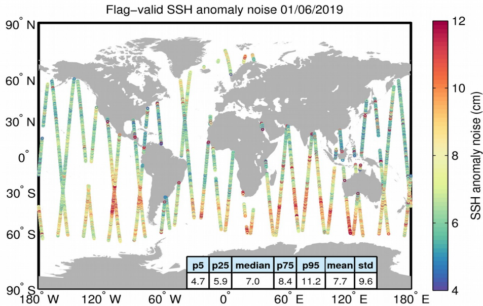
Figure 8. Geographical distribution of flag-valid 20-Hz SSH anomaly measurement noise over oceans and lakes for 01/06/2019. The statistical values shown in the table refer to the SSH anomaly noise and are calculated over all measurements shown in the figure.
