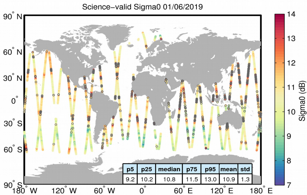
Figure 27. Geographical distribution of science-valid sigma0 data over oceans and lakes for 01/06/2019. The statistical values shown in the table refer to the sigma0 in dB and are calculated over all measurements shown in the figure. Gray circles denote records that have been rejected based on the editing criteria described in Table 4.
