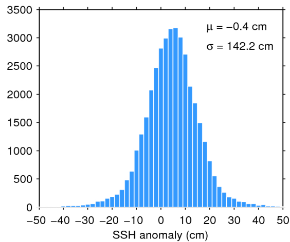
Figure 7. Histogram of flag-valid SSH anomaly over oceans and lakes for 01/06/2019. The mean ( \mu ) and standard deviation ( \sigma ) are also shown. Note that values outside [-50 50] cm are excluded from the histogram for the sake of readability but not from the computation of \mu and \sigma .
