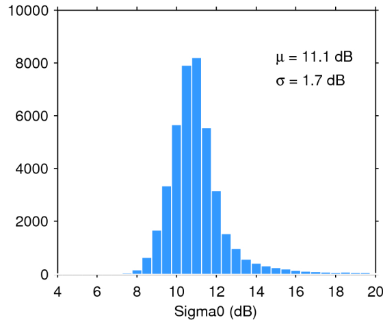
Figure 25. Histogram of flag-valid sigma0 over oceans and lakes for 01/06/2019. The mean ( \mu ) and standard deviation ( \sigma ) are also shown. Note that values outside [4 20] dB are excluded from the histogram for the sake of readability but not from the computation of \mu and \sigma .
