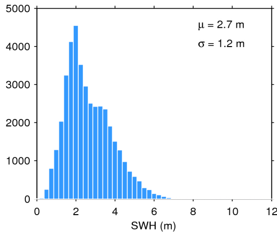
Figure 20. Histogram of science-valid SWH over oceans and lakes for 01/06/2019. The mean ( \mu ) and standard deviation ( \sigma ) are also shown. Note that values larger than 12 m are excluded from the histogram for the sake of readability but not from the computation of \mu and \sigma .
