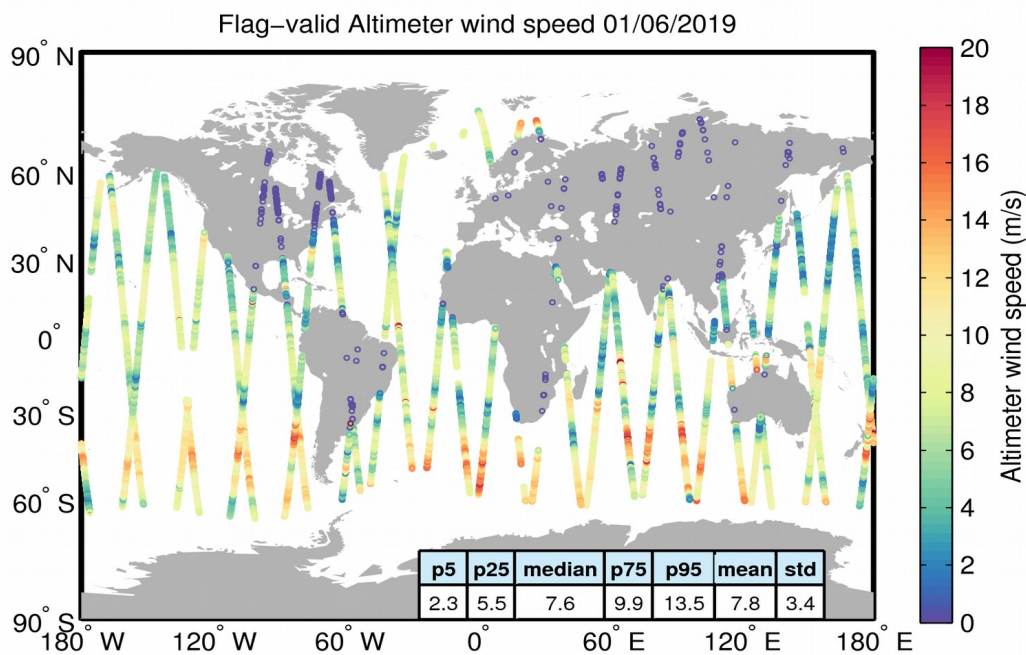
Figure 31. Geographical distribution of flag-valid wind data over oceans and lakes for 01/06/2019. The statistical values shown in the table refer to the wind in m/s and are calculated over all measurements shown in the figure.
