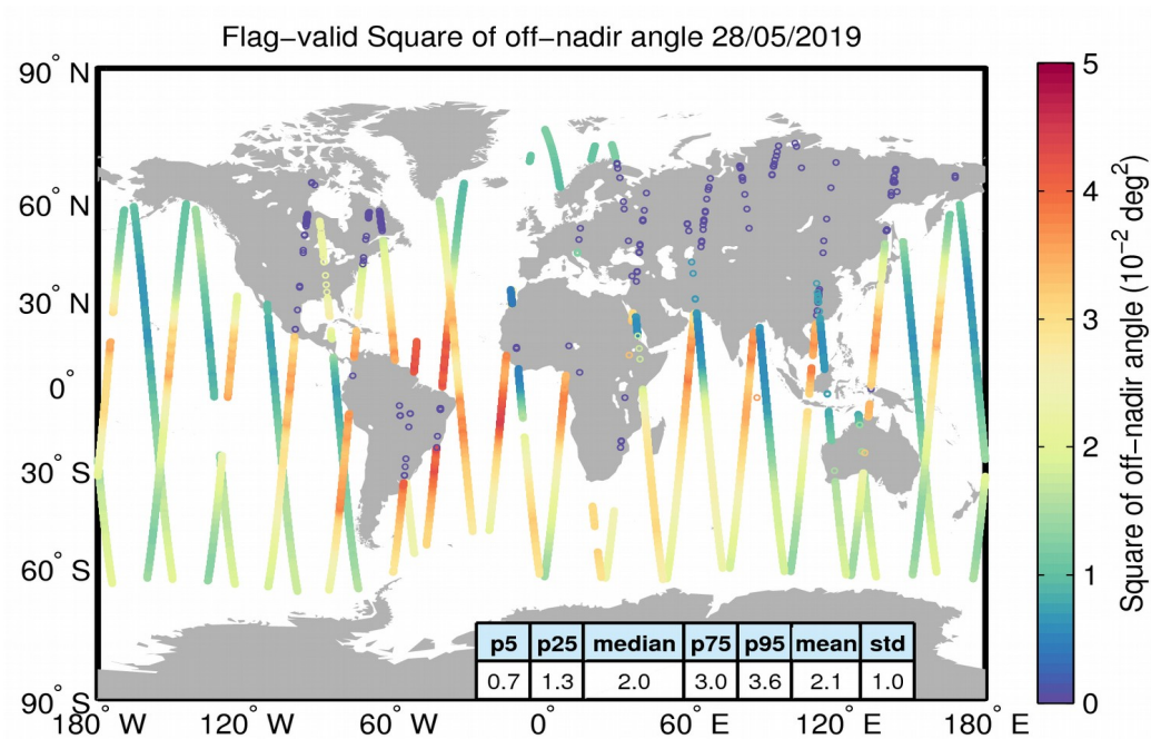
Figure 37. Geographical distribution of flag-valid mispointing data over oceans and lakes for 28/05/2019. The statistical values shown in the table refer to the mispointing in 10^{-2} \text{deg}^2 and are calculated over all measurements shown in the figure.
