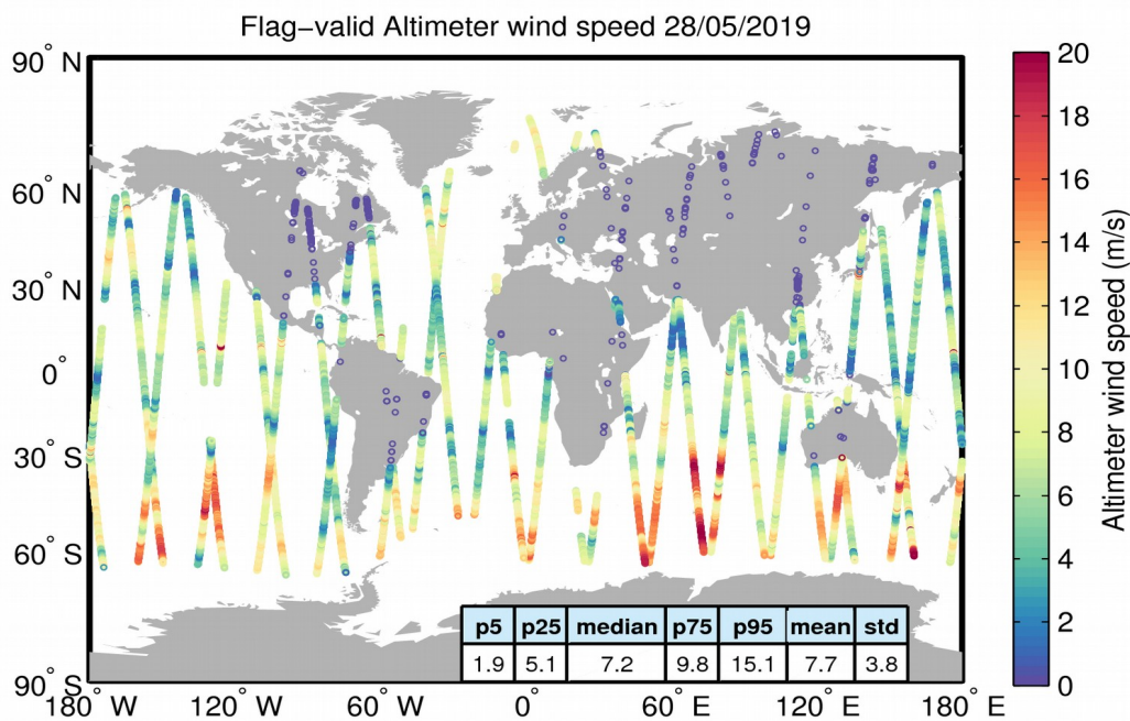
Figure 31. Geographical distribution of flag-valid wind data over oceans and lakes for 28/05/2019. The statistical values shown in the table refer to the wind in m/s and are calculated over all measurements shown in the figure.
