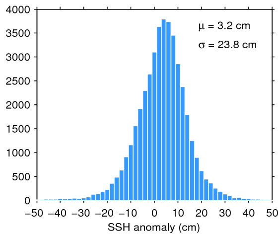
Figure 7. Histogram of flag-valid SSH anomaly over oceans and lakes for 28/05/2019. The mean ( \mu ) and standard deviation ( \sigma ) are also shown. Note that values outside [-50 50] cm are excluded from the histogram for the sake of readability but not from the computation of \mu and \sigma .
