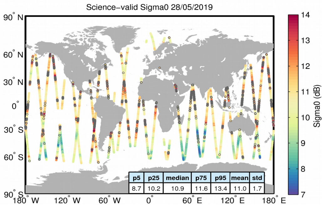
Figure 27. Geographical distribution of science-valid sigma0 data over oceans and lakes for 28/05/2019. The statistical values shown in the table refer to the sigma0 in dB and are calculated over all measurements shown in the figure. Gray circles denote records that have been rejected based on the editing criteria described in Table 4.
