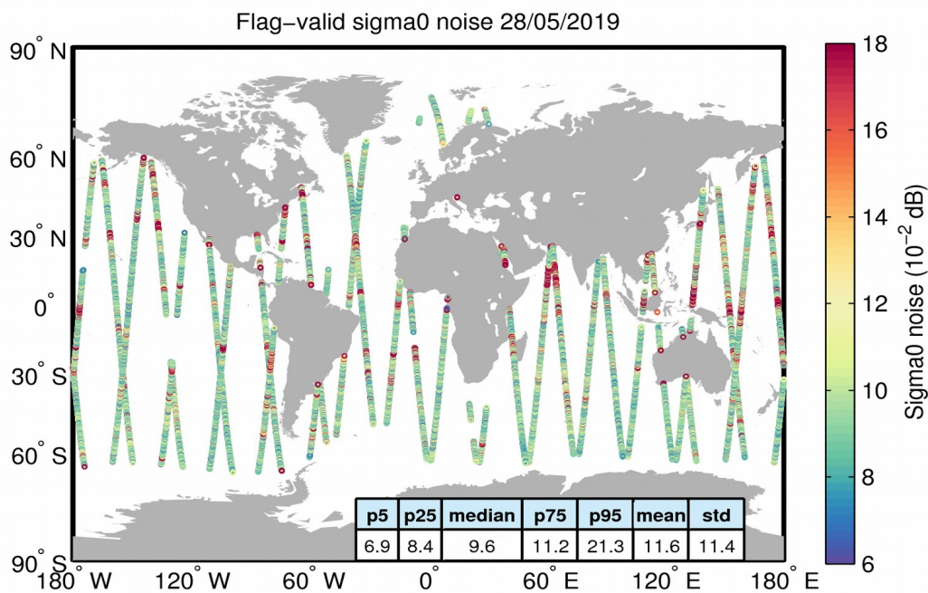
Figure 26. Geographical distribution of flag-valid 20-Hz sigma0 measurement noise over oceans and lakes for 28/05/2019. The statistical values shown in the table refer to the sigma0 noise and are calculated over all measurements shown in the figure.
