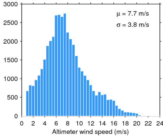
Figure 33. Histogram of flag-valid wind over oceans and lakes for 28/05/2019. The mean ( \mu ) and standard deviation ( \sigma ) are also shown. Note that values larger than 24 m/s are excluded from the histogram for the sake of readability but not from the computation of \mu and \sigma .
