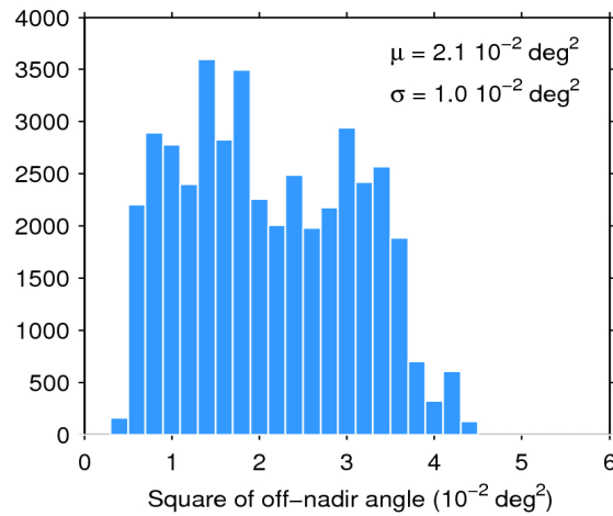
Figure 39. Histogram of flag-valid mispointing over oceans and lakes for 28/05/2019. The mean ( \mu ) and standard deviation ( \sigma ) are also shown. Note that values larger than 6 \cdot 10^{-2} \text{ deg}^2 are excluded from the histogram for the sake of readability but not from the computation of \mu and \sigma .
