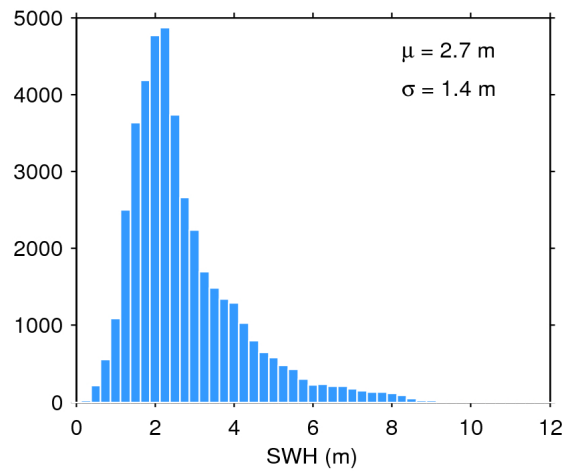
Figure 17. Histogram of flag-valid SWH over oceans and lakes for 28/05/2019. The mean ( \mu ) and standard deviation ( \sigma ) are also shown. Note that values larger than 12 m are excluded from the histogram for the sake of readability but not from the computation of \mu and \sigma .
