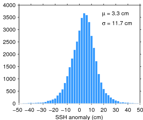
Figure 11. Histogram of science-valid SSH anomaly over oceans and lakes for 28/05/2019. The mean ( \mu ) and standard deviation ( \sigma ) are also shown. Note that values outside [-50 50] cm are excluded from the histogram for the sake of readability but not from the computation of \mu and \sigma .
