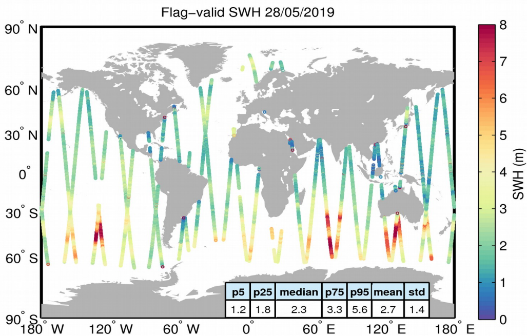
Figure 15. Geographical distribution of flag-valid SWH data over oceans and lakes for 28/05/2019. The statistical values shown in the table refer to the SWH in m and are calculated over all measurements shown in the figure.
