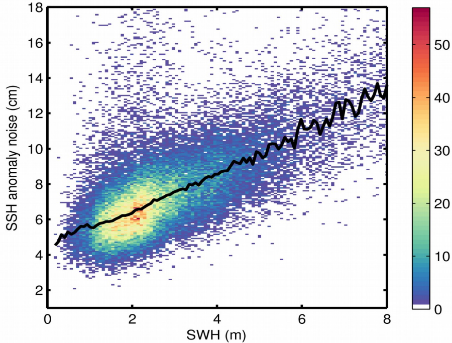
Figure 9. 2D histogram showing flag-valid SSH anomaly noise as a function of SWH for 28/05/2019. The black line denotes the median SSH anomaly noise as a function of SWH.
