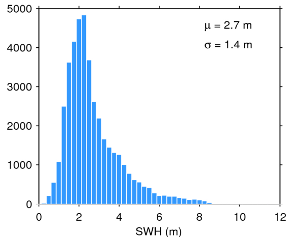
Figure 20. Histogram of science-valid SWH over oceans and lakes for 28/05/2019. The mean ( \mu ) and standard deviation ( \sigma ) are also shown. Note that values larger than 12 m are excluded from the histogram for the sake of readability but not from the computation of \mu and \sigma .
