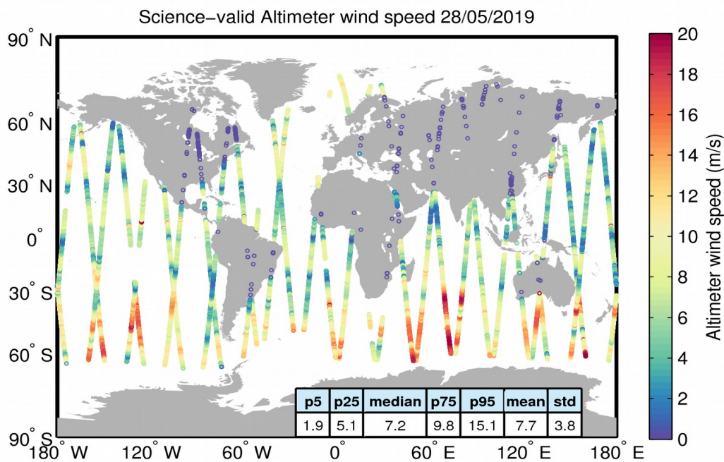
Figure 34. Geographical distribution of science-valid wind data over oceans and lakes for 28/05/2019. The statistical values shown in the table refer to the wind in m/s and are calculated over all measurements shown in the figure. Gray circles denote records that have been rejected based on the editing criteria described in Table 5.
