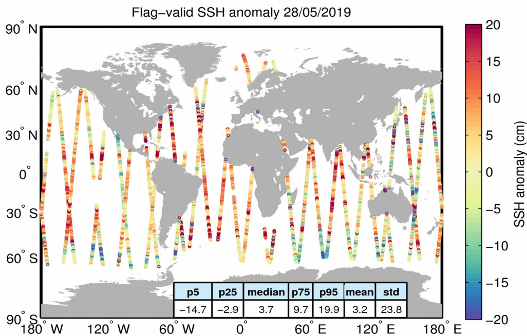
Figure 5. Geographical distribution of flag-valid 1-Hz SSH anomaly data over oceans and lakes for 28/05/2019. The statistical values shown in the table refer to the SSH anomaly in cm and are calculated over all measurements shown in the figure.
