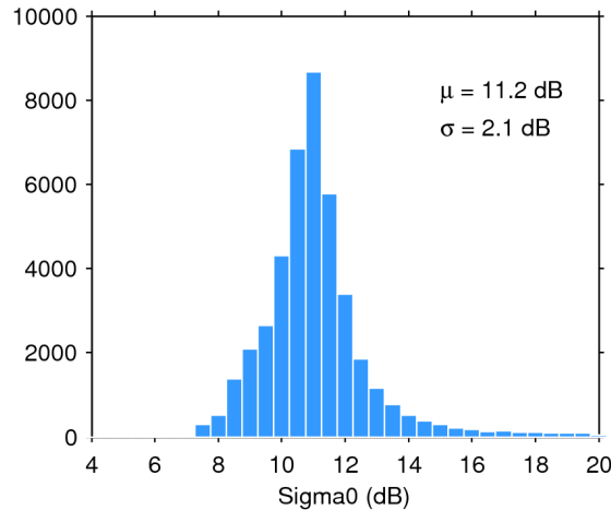
Figure 25. Histogram of flag-valid sigma0 over oceans and lakes for 28/05/2019. The mean ( \mu ) and standard deviation ( \sigma ) are also shown. Note that values outside [4 20] dB are excluded from the histogram for the sake of readability but not from the computation of \mu and \sigma .
