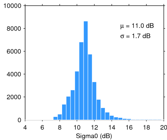
Figure 28. Histogram of science-valid sigma0 over oceans and lakes for 28/05/2019. The mean ( \mu ) and standard deviation ( \sigma ) are also shown. Note that values outside [4 20] dB are excluded from the histogram for the sake of readability but not from the computation of \mu and \sigma .
