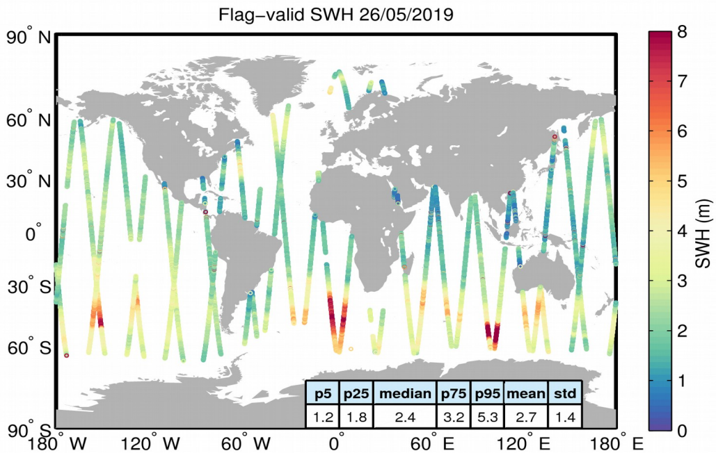
Figure 15. Geographical distribution of flag-valid SWH data over oceans and lakes for 26/05/2019. The statistical values shown in the table refer to the SWH in m and are calculated over all measurements shown in the figure.
