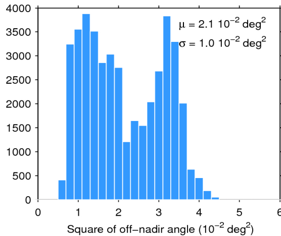
Figure 39. Histogram of flag-valid mispointing over oceans and lakes for 26/05/2019. The mean ( \mu ) and standard deviation ( \sigma ) are also shown. Note that values larger than 6 \cdot 10^{-2} \text{ deg}^2 are excluded from the histogram for the sake of readability but not from the computation of \mu and \sigma .
