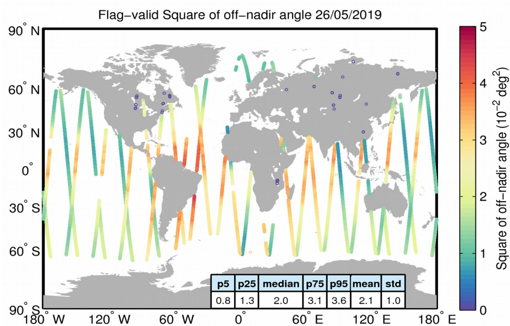
Figure 37. Geographical distribution of flag-valid mispointing data over oceans and lakes for 26/05/2019. The statistical values shown in the table refer to the mispointing in 10^{-2} deg 2 and are calculated over all measurements shown in the figure.
