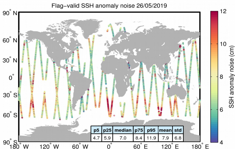
Figure 8. Geographical distribution of flag-valid 20-Hz SSH anomaly measurement noise over oceans and lakes for 26/05/2019. The statistical values shown in the table refer to the SSH anomaly noise and are calculated over all measurements shown in the figure.
