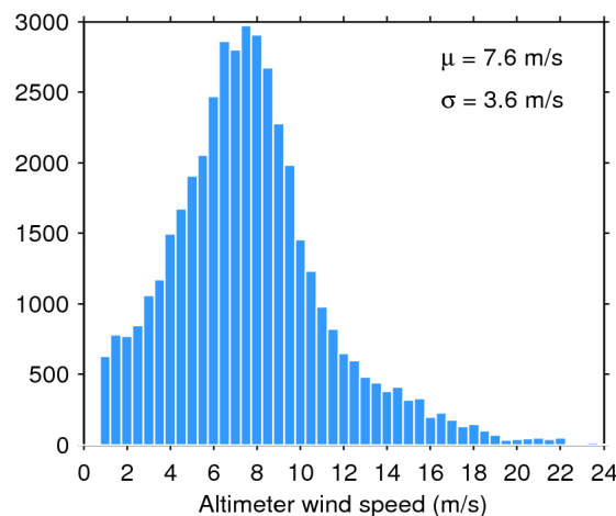
Figure 35. Histogram of science-valid wind over oceans and lakes for 26/05/2019. The mean ( \mu ) and standard deviation ( \sigma ) are also shown. Note that values larger than 24 m/s are excluded from the histogram for the sake of readability but not from the computation of \mu and \sigma .
