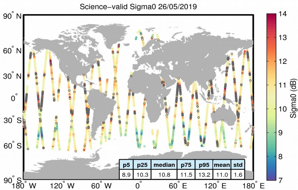
Figure 27. Geographical distribution of science-valid sigma0 data over oceans and lakes for 26/05/2019. The statistical values shown in the table refer to the sigma0 in dB and are calculated over all measurements shown in the figure. Gray circles denote records that have been rejected based on the editing criteria described in Table 4.
