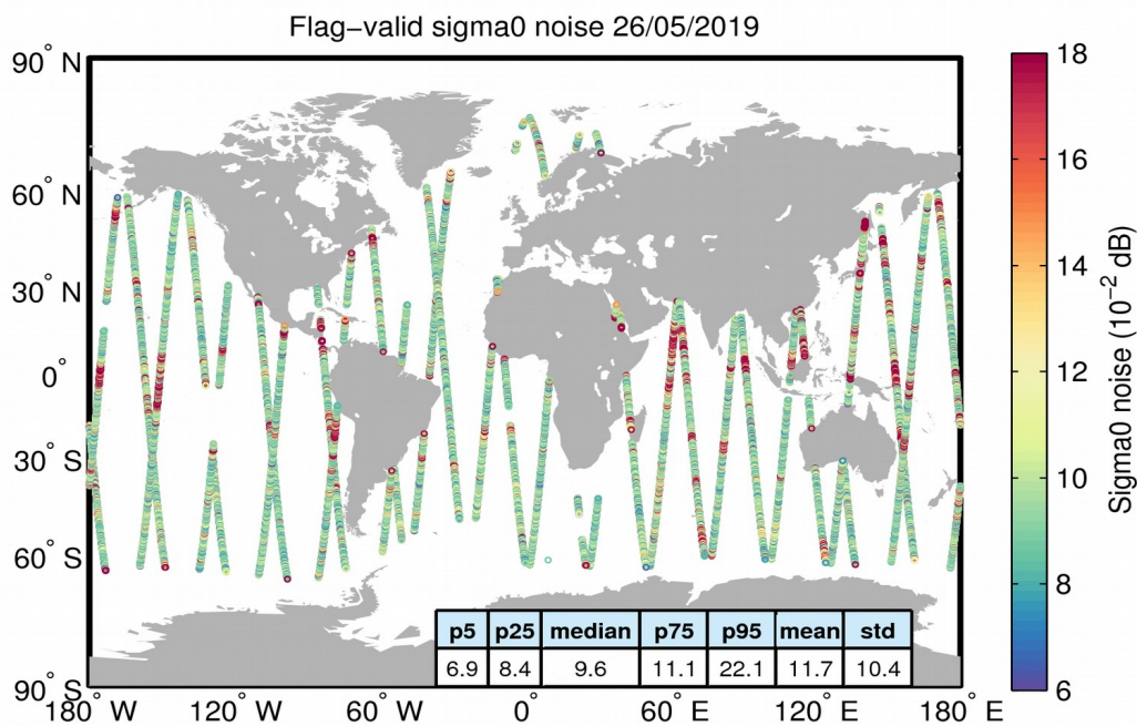
Figure 26. Geographical distribution of flag-valid 20-Hz sigma0 measurement noise over oceans and lakes for 26/05/2019. The statistical values shown in the table refer to the sigma0 noise and are calculated over all measurements shown in the figure.
