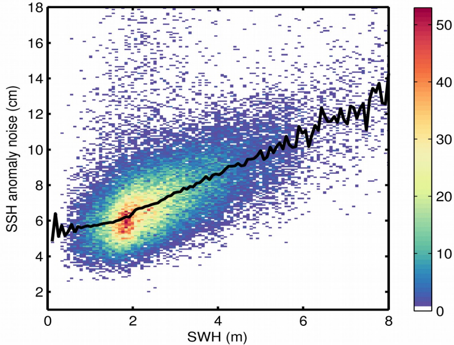
Figure 9. 2D histogram showing flag-valid SSH anomaly noise as a function of SWH for 26/05/2019. The black line denotes the median SSH anomaly noise as a function of SWH.
