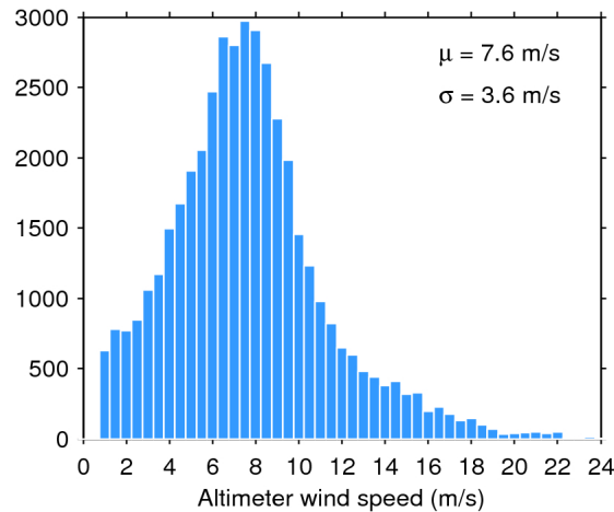
Figure 33. Histogram of flag-valid wind over oceans and lakes for 26/05/2019. The mean ( \mu ) and standard deviation ( \sigma ) are also shown. Note that values larger than 24 m/s are excluded from the histogram for the sake of readability but not from the computation of \mu and \sigma .
