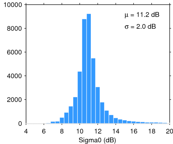
Figure 25. Histogram of flag-valid sigma0 over oceans and lakes for 26/05/2019. The mean ( \mu ) and standard deviation ( \sigma ) are also shown. Note that values outside [4 20] dB are excluded from the histogram for the sake of readability but not from the computation of \mu and \sigma .
