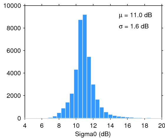
Figure 28. Histogram of science-valid sigma0 over oceans and lakes for 26/05/2019. The mean ( \mu ) and standard deviation ( \sigma ) are also shown. Note that values outside [4 20] dB are excluded from the histogram for the sake of readability but not from the computation of \mu and \sigma .
