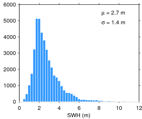
Figure 17. Histogram of flag-valid SWH over oceans and lakes for 26/05/2019. The mean ( \mu ) and standard deviation ( \sigma ) are also shown. Note that values larger than 12 m are excluded from the histogram for the sake of readability but not from the computation of \mu and \sigma .
