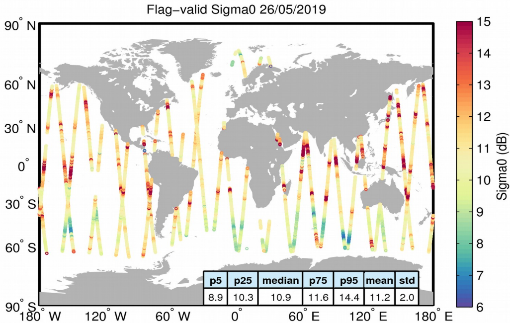
Figure 23. Geographical distribution of flag-valid sigma0 data over oceans and lakes for 26/05/2019. The statistical values shown in the table refer to the sigma0 in dB and are calculated over all measurements shown in the figure.
