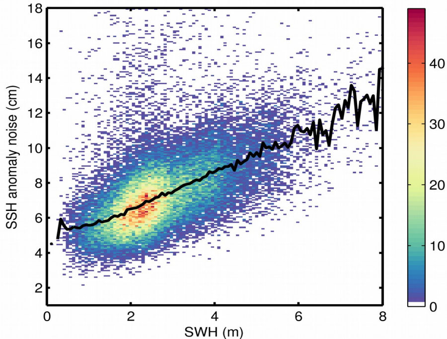
Figure 9. 2D histogram showing flag-valid SSH anomaly noise as a function of SWH for 25/05/2019. The black line denotes the median SSH anomaly noise as a function of SWH.
