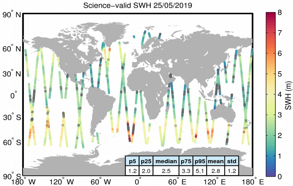
Figure 19. Geographical distribution of science-valid SWH data over oceans and lakes for 25/05/2019. The statistical values shown in the table refer to the SWH in m and are calculated over all measurements shown in the figure. Gray circles denote records that have been rejected based on the editing criteria described in Table 3.
