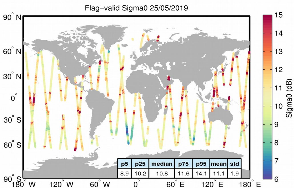
Figure 23. Geographical distribution of flag-valid sigma0 data over oceans and lakes for 25/05/2019. The statistical values shown in the table refer to the sigma0 in dB and are calculated over all measurements shown in the figure.
