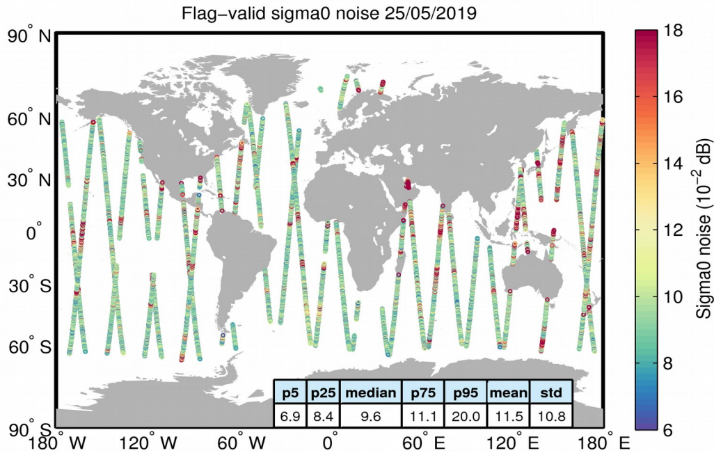
Figure 26. Geographical distribution of flag-valid 20-Hz sigma0 measurement noise over oceans and lakes for 25/05/2019. The statistical values shown in the table refer to the sigma0 noise and are calculated over all measurements shown in the figure.
