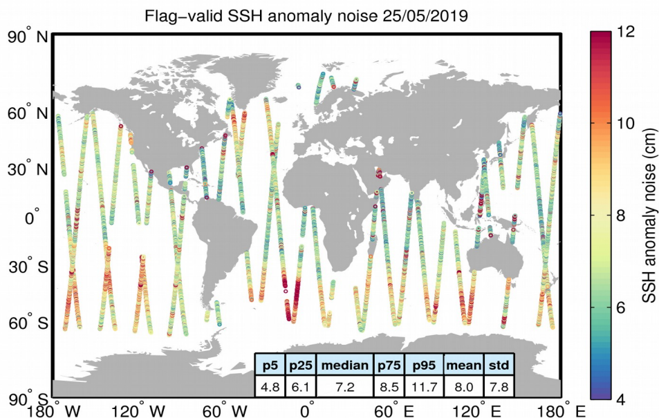
Figure 8. Geographical distribution of flag-valid 20-Hz SSH anomaly measurement noise over oceans and lakes for 25/05/2019. The statistical values shown in the table refer to the SSH anomaly noise and are calculated over all measurements shown in the figure.
