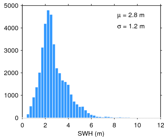
Figure 20. Histogram of science-valid SWH over oceans and lakes for 25/05/2019. The mean ( \mu ) and standard deviation ( \sigma ) are also shown. Note that values larger than 12 m are excluded from the histogram for the sake of readability but not from the computation of \mu and \sigma .
