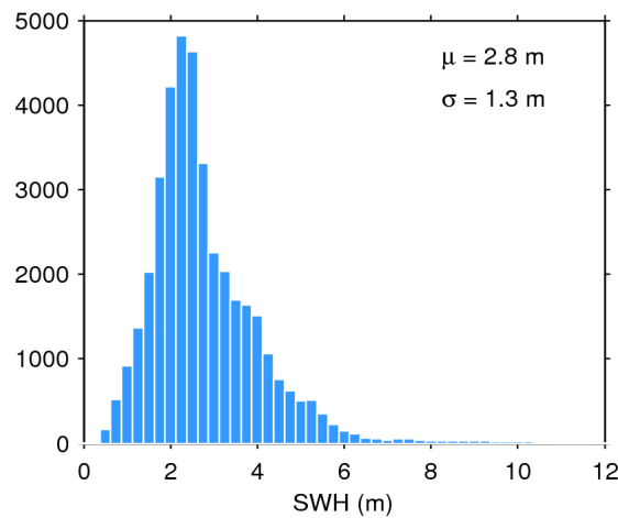
Figure 17. Histogram of flag-valid SWH over oceans and lakes for 25/05/2019. The mean ( \mu ) and standard deviation ( \sigma ) are also shown. Note that values larger than 12 m are excluded from the histogram for the sake of readability but not from the computation of \mu and \sigma .
