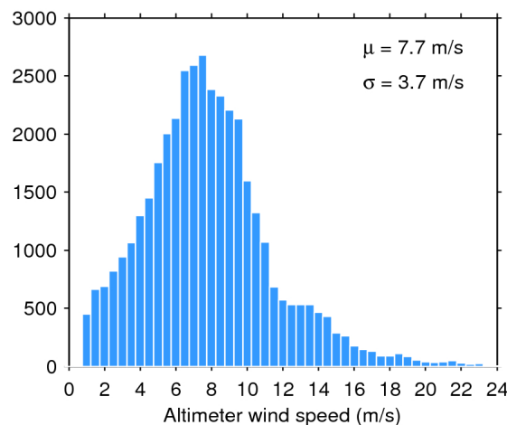
Figure 35. Histogram of science-valid wind over oceans and lakes for 25/05/2019. The mean ( \mu ) and standard deviation ( \sigma ) are also shown. Note that values larger than 24 m/s are excluded from the histogram for the sake of readability but not from the computation of \mu and \sigma .
