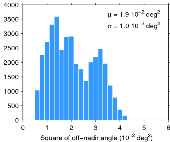
Figure 39. Histogram of flag-valid mispointing over oceans and lakes for 25/05/2019. The mean ( \mu ) and standard deviation ( \sigma ) are also shown. Note that values larger than 6 \cdot 10^{-2} \text{ deg}^2 are excluded from the histogram for the sake of readability but not from the computation of \mu and \sigma .
