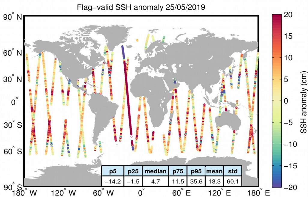
Figure 5. Geographical distribution of flag-valid 1-Hz SSH anomaly data over oceans and lakes for 25/05/2019. The statistical values shown in the table refer to the SSH anomaly in cm and are calculated over all measurements shown in the figure.
