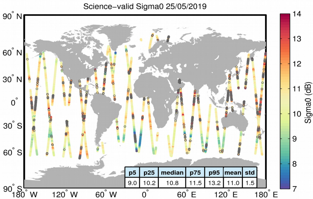
Figure 27. Geographical distribution of science-valid sigma0 data over oceans and lakes for 25/05/2019. The statistical values shown in the table refer to the sigma0 in dB and are calculated over all measurements shown in the figure. Gray circles denote records that have been rejected based on the editing criteria described in Table 4.
