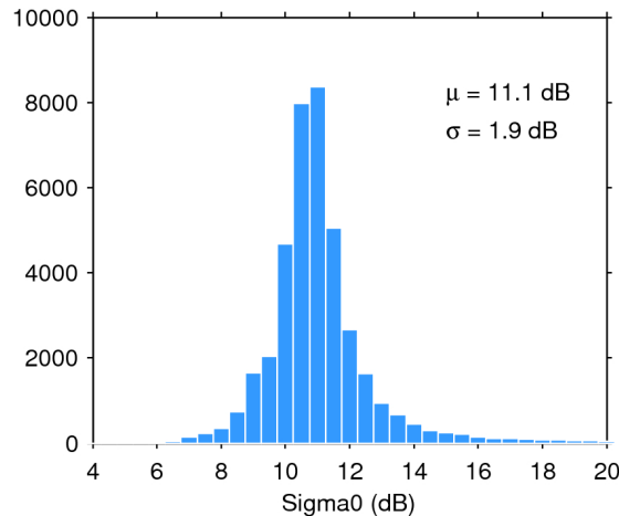
Figure 25. Histogram of flag-valid sigma0 over oceans and lakes for 25/05/2019. The mean ( \mu ) and standard deviation ( \sigma ) are also shown. Note that values outside [4 20] dB are excluded from the histogram for the sake of readability but not from the computation of \mu and \sigma .
