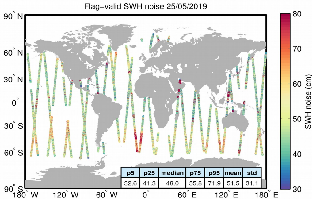
Figure 18. Geographical distribution of flag-valid 20-Hz SWH measurement noise over oceans and lakes for 25/05/2019. The statistical values shown in the figure refer to the SWH noise and are calculated over all measurements shown in the figure.
