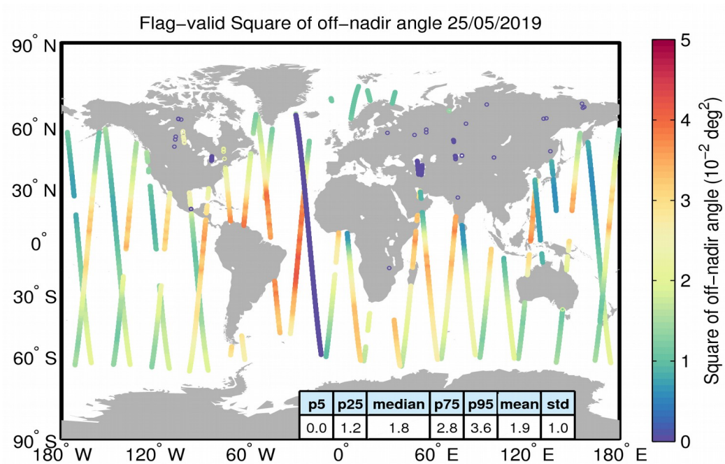
Figure 37. Geographical distribution of flag-valid mispointing data over oceans and lakes for 25/05/2019. The statistical values shown in the table refer to the mispointing in 10^{-2} \text{ deg}^2 and are calculated over all measurements shown in the figure.
