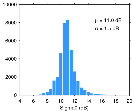
Figure 28. Histogram of science-valid sigma0 over oceans and lakes for 25/05/2019. The mean ( \mu ) and standard deviation ( \sigma ) are also shown. Note that values outside [4 20] dB are excluded from the histogram for the sake of readability but not from the computation of \mu and \sigma .
