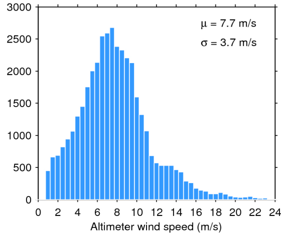
Figure 33. Histogram of flag-valid wind over oceans and lakes for 25/05/2019. The mean ( \mu ) and standard deviation ( \sigma ) are also shown. Note that values larger than 24 m/s are excluded from the histogram for the sake of readability but not from the computation of \mu and \sigma .
