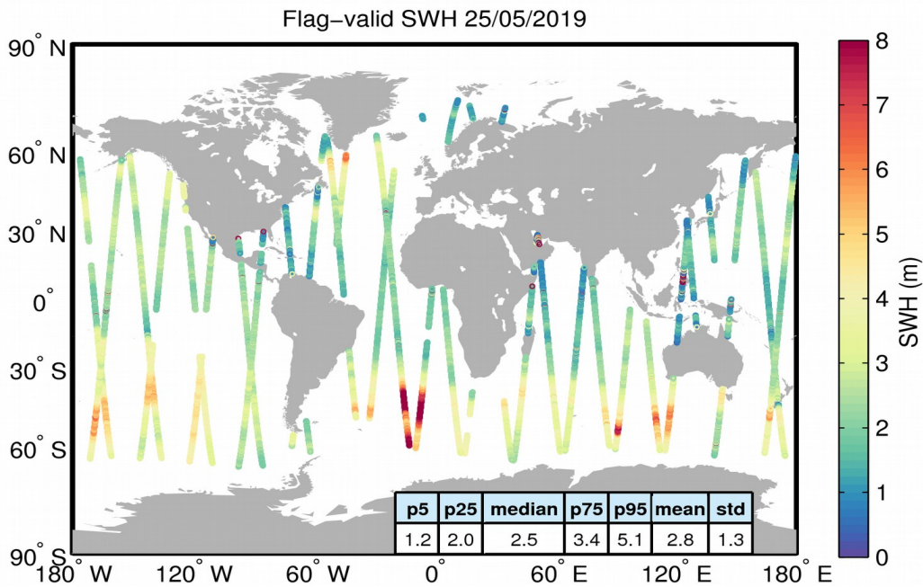
Figure 15. Geographical distribution of flag-valid SWH data over oceans and lakes for 25/05/2019. The statistical values shown in the table refer to the SWH in m and are calculated over all measurements shown in the figure.
