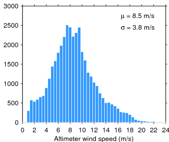
Figure 35. Histogram of science-valid wind over oceans and lakes for 23/05/2019. The mean ( \mu ) and standard deviation ( \sigma ) are also shown. Note that values larger than 24 m/s are excluded from the histogram for the sake of readability but not from the computation of \mu and \sigma .
