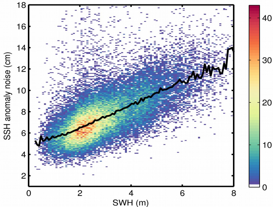
Figure 9. 2D histogram showing flag-valid SSH anomaly noise as a function of SWH for 23/05/2019. The black line denotes the median SSH anomaly noise as a function of SWH.
