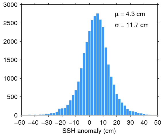
Figure 11. Histogram of science-valid SSH anomaly over oceans and lakes for 23/05/2019. The mean ( \mu ) and standard deviation ( \sigma ) are also shown. Note that values outside [-50 50] cm are excluded from the histogram for the sake of readability but not from the computation of \mu and \sigma .
