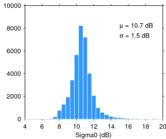
Figure 28. Histogram of science-valid sigma0 over oceans and lakes for 23/05/2019. The mean ( \mu ) and standard deviation ( \sigma ) are also shown. Note that values outside [4 20] dB are excluded from the histogram for the sake of readability but not from the computation of \mu and \sigma .
