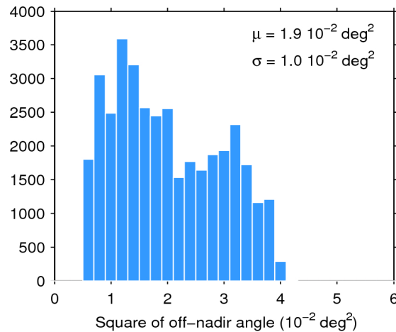
Figure 39. Histogram of flag-valid mispointing over oceans and lakes for 23/05/2019. The mean ( \mu ) and standard deviation ( \sigma ) are also shown. Note that values larger than 6 \cdot 10^{-2} \text{ deg}^2 are excluded from the histogram for the sake of readability but not from the computation of \mu and \sigma .
