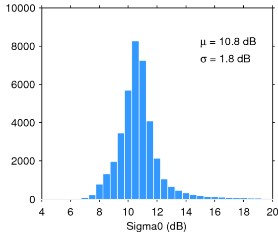
Figure 25. Histogram of flag-valid sigma0 over oceans and lakes for 23/05/2019. The mean ( \mu ) and standard deviation ( \sigma ) are also shown. Note that values outside [4 20] dB are excluded from the histogram for the sake of readability but not from the computation of \mu and \sigma .
