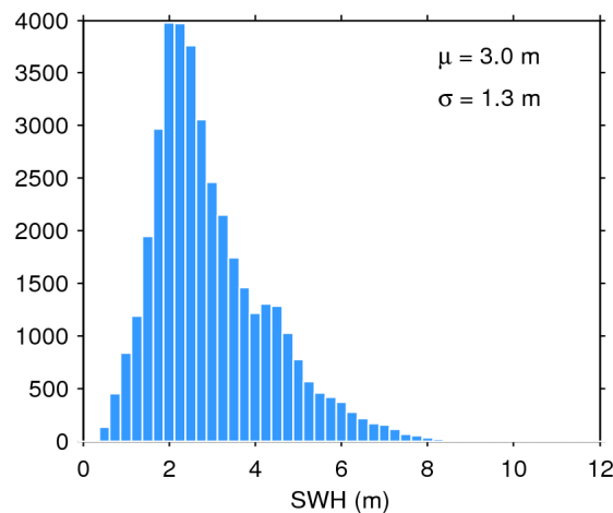
Figure 20. Histogram of science-valid SWH over oceans and lakes for 23/05/2019. The mean ( \mu ) and standard deviation ( \sigma ) are also shown. Note that values larger than 12 m are excluded from the histogram for the sake of readability but not from the computation of \mu and \sigma .
