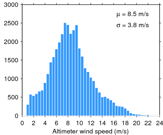
Figure 33. Histogram of flag-valid wind over oceans and lakes for 23/05/2019. The mean ( \mu ) and standard deviation ( \sigma ) are also shown. Note that values larger than 24 m/s are excluded from the histogram for the sake of readability but not from the computation of \mu and \sigma .
