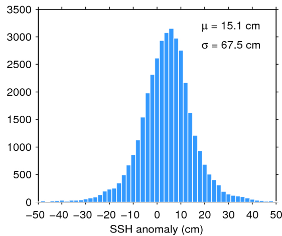
Figure 7. Histogram of flag-valid SSH anomaly over oceans and lakes for 23/05/2019. The mean ( \mu ) and standard deviation ( \sigma ) are also shown. Note that values outside [-50\ 50] cm are excluded from the histogram for the sake of readability but not from the computation of \mu and \sigma .
