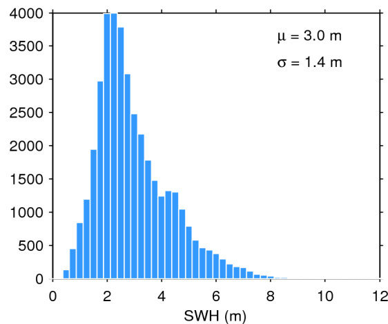
Figure 17. Histogram of flag-valid SWH over oceans and lakes for 23/05/2019. The mean ( \mu ) and standard deviation ( \sigma ) are also shown. Note that values larger than 12 m are excluded from the histogram for the sake of readability but not from the computation of \mu and \sigma .
