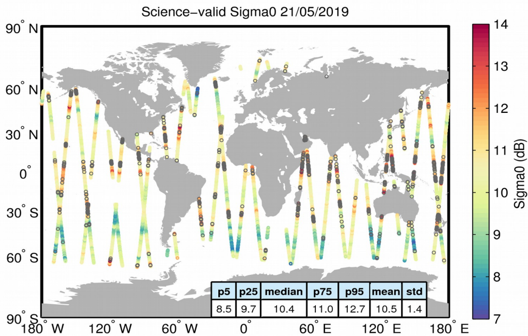
Figure 27. Geographical distribution of science-valid sigma0 data over oceans and lakes for 21/05/2019. The statistical values shown in the table refer to the sigma0 in dB and are calculated over all measurements shown in the figure. Gray circles denote records that have been rejected based on the editing criteria described in Table 4.
