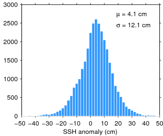
Figure 11. Histogram of science-valid SSH anomaly over oceans and lakes for 21/05/2019. The mean ( \mu ) and standard deviation ( \sigma ) are also shown. Note that values outside [-50 50] cm are excluded from the histogram for the sake of readability but not from the computation of \mu and \sigma .
