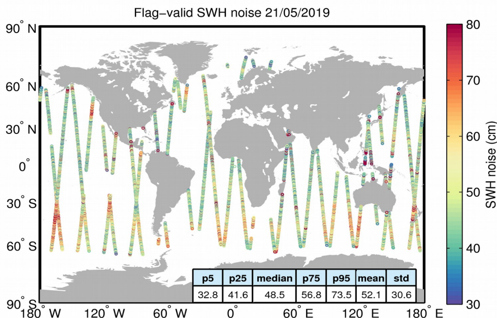
Figure 18. Geographical distribution of flag-valid 20-Hz SWH measurement noise over oceans and lakes for 21/05/2019. The statistical values shown in the figure refer to the SWH noise and are calculated over all measurements shown in the figure.
