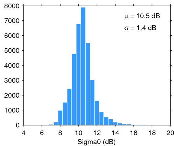
Figure 28. Histogram of science-valid sigma0 over oceans and lakes for 21/05/2019. The mean ( \mu ) and standard deviation ( \sigma ) are also shown. Note that values outside [4 20] dB are excluded from the histogram for the sake of readability but not from the computation of \mu and \sigma .
