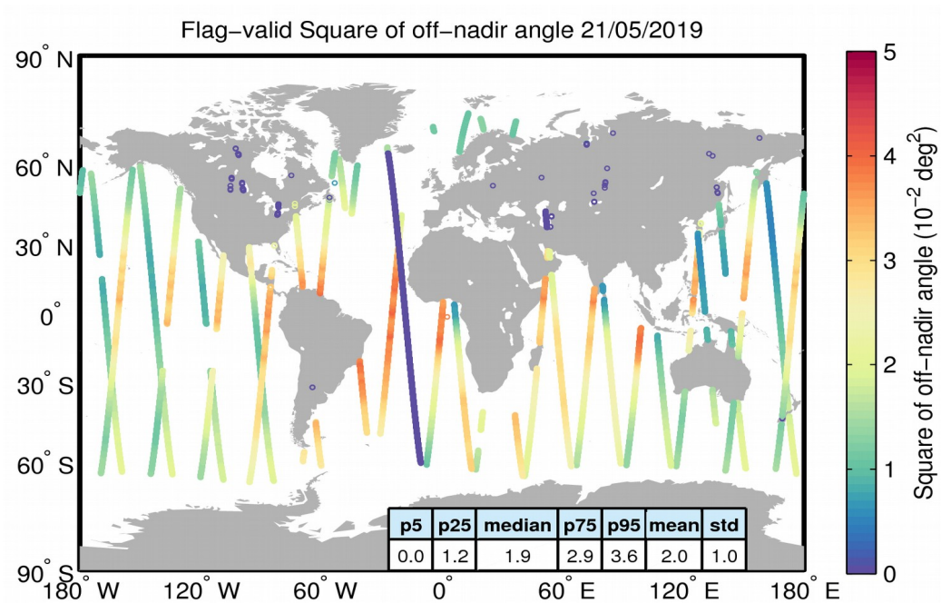
Figure 37. Geographical distribution of flag-valid mispointing data over oceans and lakes for 21/05/2019. The statistical values shown in the table refer to the mispointing in 10^{-2} deg 2 and are calculated over all measurements shown in the figure.
