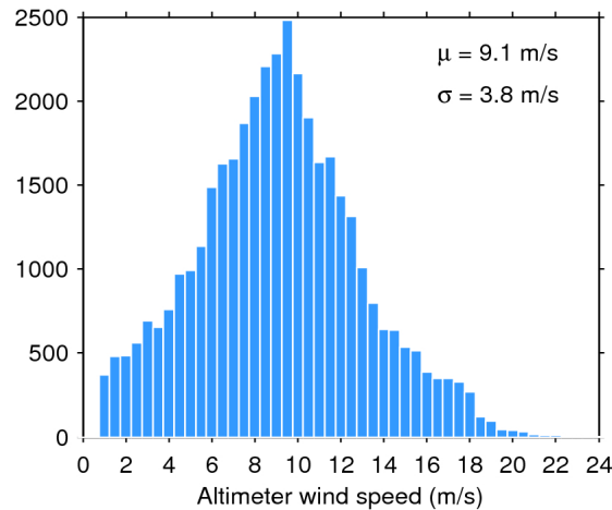
Figure 33. Histogram of flag-valid wind over oceans and lakes for 21/05/2019. The mean ( \mu ) and standard deviation ( \sigma ) are also shown. Note that values larger than 24 m/s are excluded from the histogram for the sake of readability but not from the computation of \mu and \sigma .
