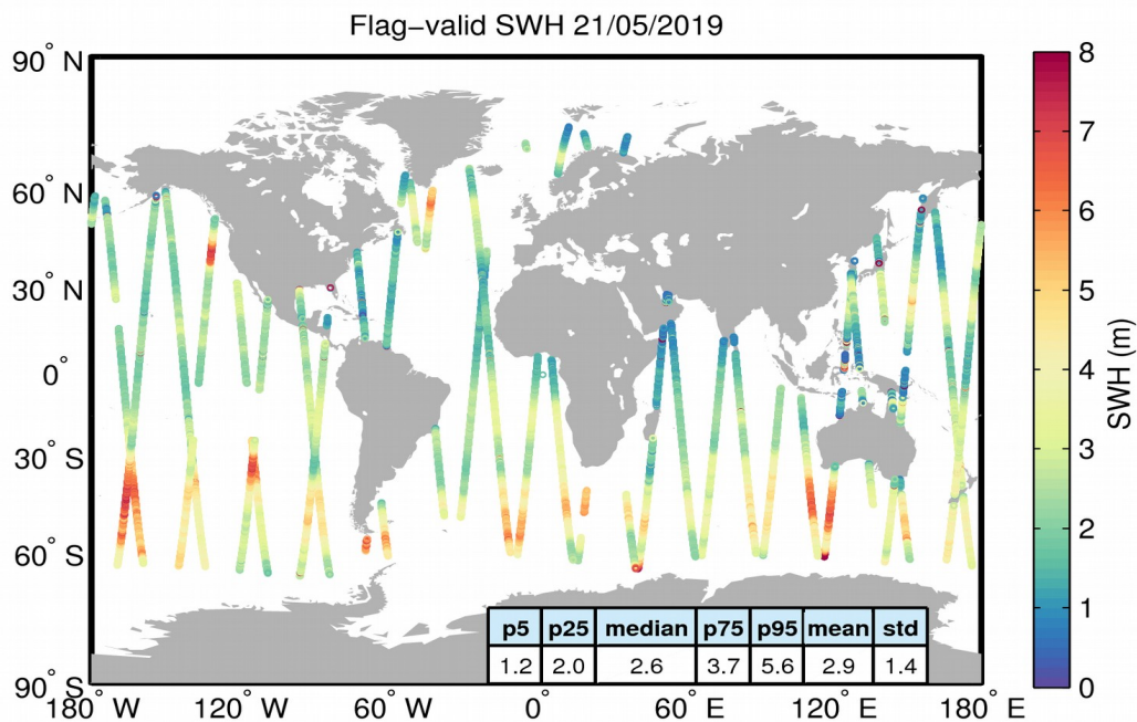
Figure 15. Geographical distribution of flag-valid SWH data over oceans and lakes for 21/05/2019. The statistical values shown in the table refer to the SWH in m and are calculated over all measurements shown in the figure.
