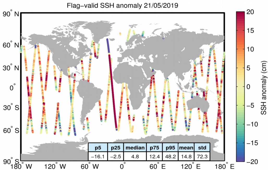
Figure 5. Geographical distribution of flag-valid 1-Hz SSH anomaly data over oceans and lakes for 21/05/2019. The statistical values shown in the table refer to the SSH anomaly in cm and are calculated over all measurements shown in the figure.
