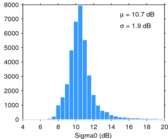
Figure 25. Histogram of flag-valid sigma0 over oceans and lakes for 21/05/2019. The mean ( \mu ) and standard deviation ( \sigma ) are also shown. Note that values outside [4 20] dB are excluded from the histogram for the sake of readability but not from the computation of \mu and \sigma .
