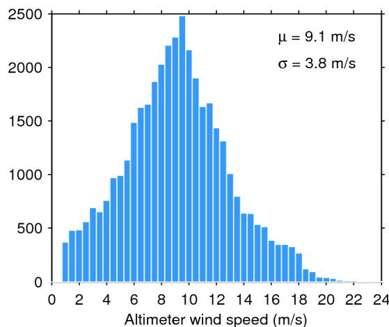
Figure 35. Histogram of science-valid wind over oceans and lakes for 21/05/2019. The mean ( \mu ) and standard deviation ( \sigma ) are also shown. Note that values larger than 24 m/s are excluded from the histogram for the sake of readability but not from the computation of \mu and \sigma .
