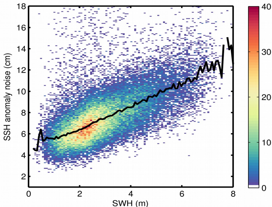
Figure 9. 2D histogram showing flag-valid SSH anomaly noise as a function of SWH for 21/05/2019. The black line denotes the median SSH anomaly noise as a function of SWH.
