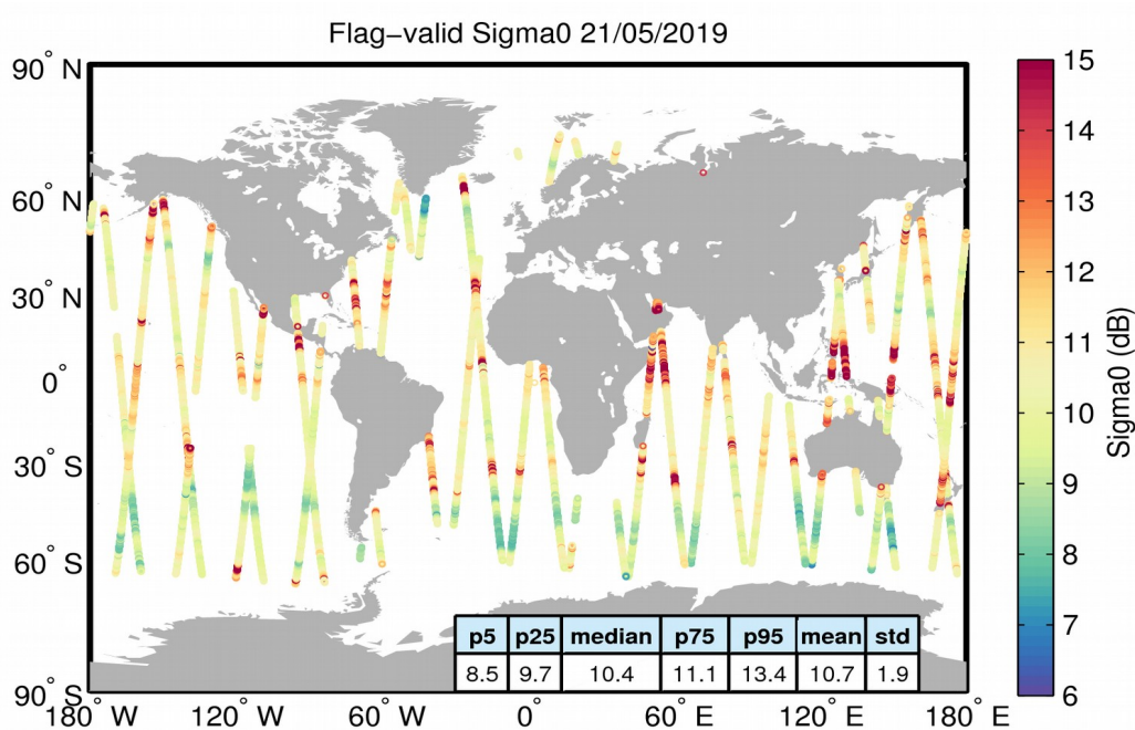
Figure 23. Geographical distribution of flag-valid sigma0 data over oceans and lakes for 21/05/2019. The statistical values shown in the table refer to the sigma0 in dB and are calculated over all measurements shown in the figure.
