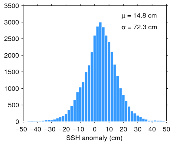
Figure 7. Histogram of flag-valid SSH anomaly over oceans and lakes for 21/05/2019. The mean ( \mu ) and standard deviation ( \sigma ) are also shown. Note that values outside [-50 50] cm are excluded from the histogram for the sake of readability but not from the computation of \mu and \sigma .
