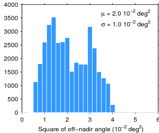
Figure 39. Histogram of flag-valid mispointing over oceans and lakes for 21/05/2019. The mean ( \mu ) and standard deviation ( \sigma ) are also shown. Note that values larger than 6 \cdot 10^{-2} \text{ deg}^2 are excluded from the histogram for the sake of readability but not from the computation of \mu and \sigma .
