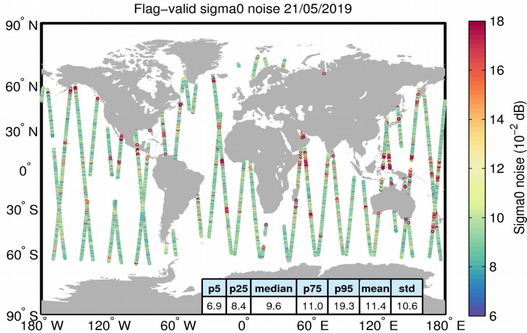
Figure 26. Geographical distribution of flag-valid 20-Hz sigma0 measurement noise over oceans and lakes for 21/05/2019. The statistical values shown in the table refer to the sigma0 noise and are calculated over all measurements shown in the figure.
