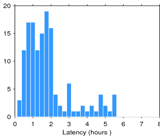
Figure 2. Histogram of the data latency for 20/05/2019. The y-axis denotes the number of files that are made available with a delay of x-hours with respect to the mean time of the records stored in the file.
