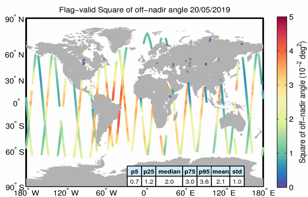
Figure 37. Geographical distribution of flag-valid mispointing data over oceans and lakes for 20/05/2019. The statistical values shown in the table refer to the mispointing in 10^{-2} \text{ deg}^2 and are calculated over all measurements shown in the figure.
