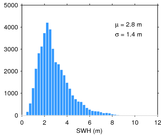
Figure 17. Histogram of flag-valid SWH over oceans and lakes for 20/05/2019. The mean ( \mu ) and standard deviation ( \sigma ) are also shown. Note that values larger than 12 m are excluded from the histogram for the sake of readability but not from the computation of \mu and \sigma .
