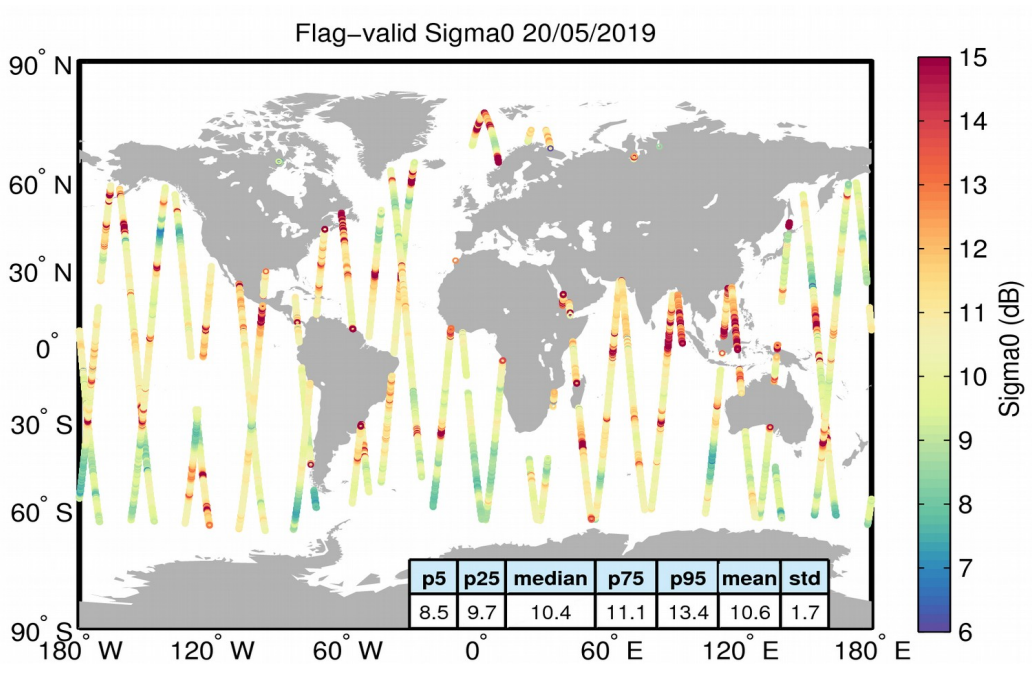
Figure 23. Geographical distribution of flag-valid sigma0 data over oceans and lakes for 20/05/2019. The statistical values shown in the table refer to the sigma0 in dB and are calculated over all measurements shown in the figure.
