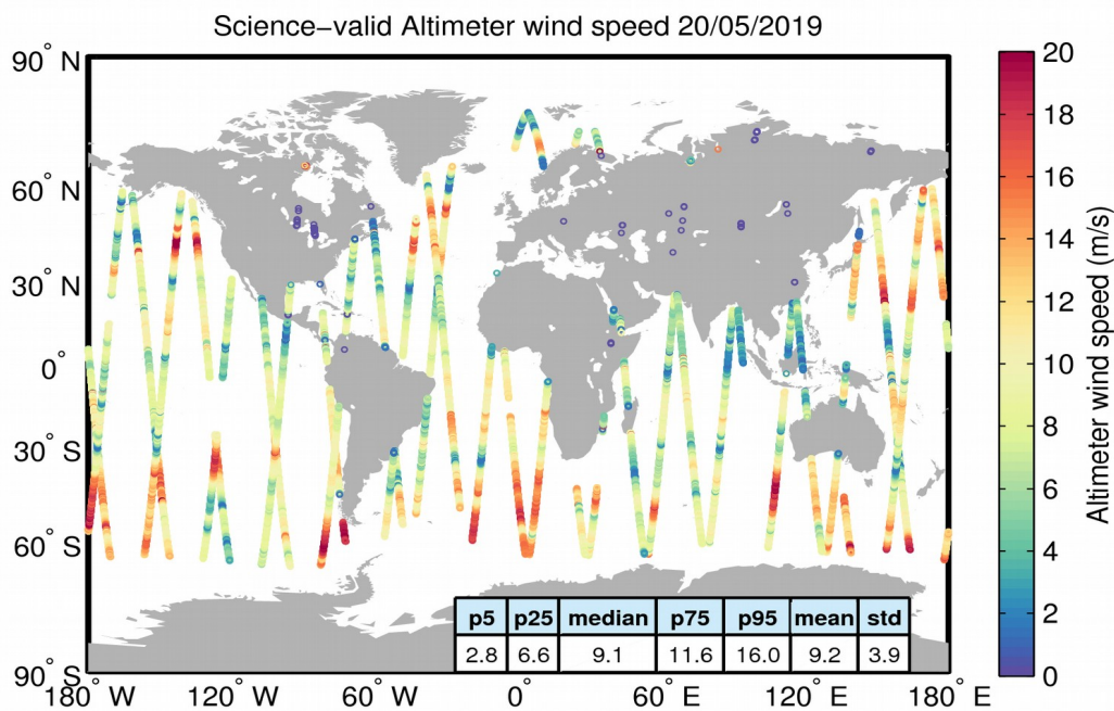
Figure 34. Geographical distribution of science-valid wind data over oceans and lakes for 20/05/2019. The statistical values shown in the table refer to the wind in m/s and are calculated over all measurements shown in the figure. Gray circles denote records that have been rejected based on the editing criteria described in Table 5.
