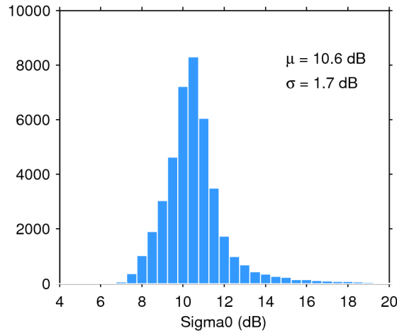
Figure 25. Histogram of flag-valid sigma0 over oceans and lakes for 20/05/2019. The mean ( \mu ) and standard deviation ( \sigma ) are also shown. Note that values outside [4 20] dB are excluded from the histogram for the sake of readability but not from the computation of \mu and \sigma .
