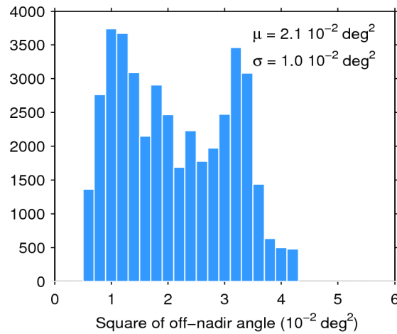
Figure 39. Histogram of flag-valid mispointing over oceans and lakes for 20/05/2019. The mean ( \mu ) and standard deviation ( \sigma ) are also shown. Note that values larger than 6 \cdot 10^{-2} \text{ deg}^2 are excluded from the histogram for the sake of readability but not from the computation of \mu and \sigma .
