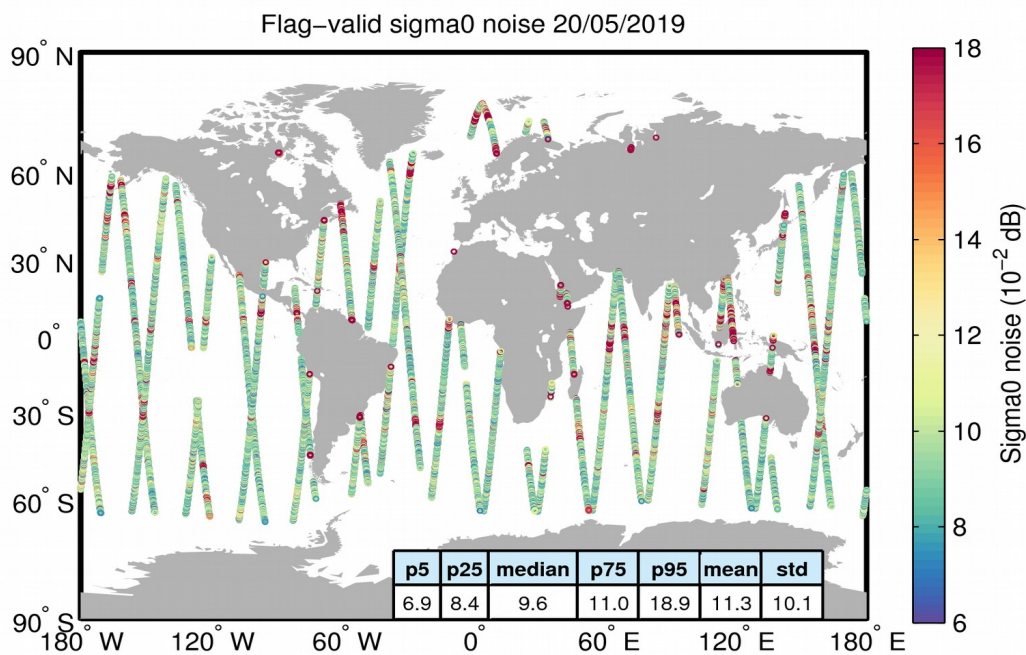
Figure 26. Geographical distribution of flag-valid 20-Hz sigma0 measurement noise over oceans and lakes for 20/05/2019. The statistical values shown in the table refer to the sigma0 noise and are calculated over all measurements shown in the figure.
