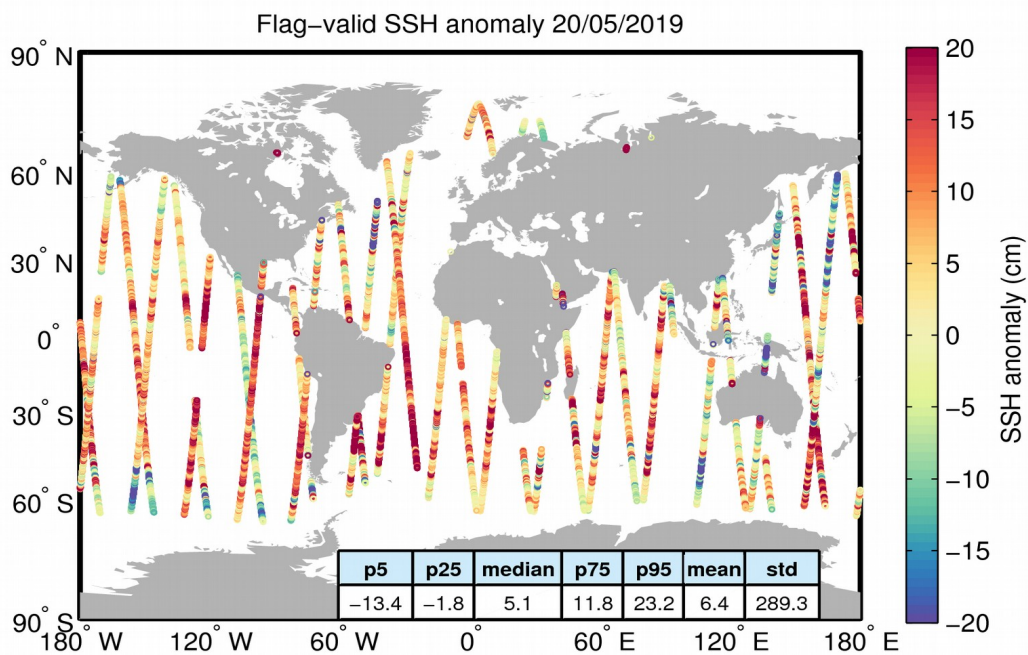
Figure 5. Geographical distribution of flag-valid 1-Hz SSH anomaly data over oceans and lakes for 20/05/2019. The statistical values shown in the table refer to the SSH anomaly in cm and are calculated over all measurements shown in the figure.
