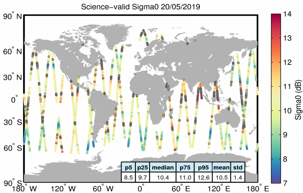
Figure 27. Geographical distribution of science-valid sigma0 data over oceans and lakes for 20/05/2019. The statistical values shown in the table refer to the sigma0 in dB and are calculated over all measurements shown in the figure. Gray circles denote records that have been rejected based on the editing criteria described in Table 4.
