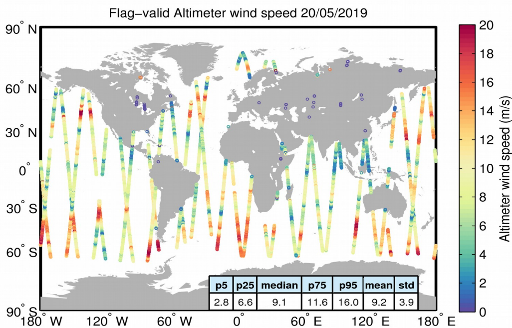
Figure 31. Geographical distribution of flag-valid wind data over oceans and lakes for 20/05/2019. The statistical values shown in the table refer to the wind in m/s and are calculated over all measurements shown in the figure.
