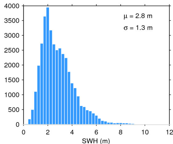
Figure 20. Histogram of science-valid SWH over oceans and lakes for 19/05/2019. The mean ( \mu ) and standard deviation ( \sigma ) are also shown. Note that values larger than 12 m are excluded from the histogram for the sake of readability but not from the computation of \mu and \sigma .
