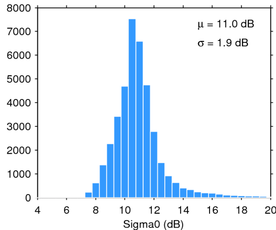
Figure 25. Histogram of flag-valid sigma0 over oceans and lakes for 19/05/2019. The mean ( \mu ) and standard deviation ( \sigma ) are also shown. Note that values outside [4 20] dB are excluded from the histogram for the sake of readability but not from the computation of \mu and \sigma .
