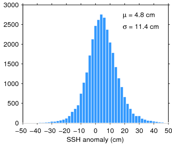
Figure 11. Histogram of science-valid SSH anomaly over oceans and lakes for 19/05/2019. The mean ( \mu ) and standard deviation ( \sigma ) are also shown. Note that values outside [-50 50] cm are excluded from the histogram for the sake of readability but not from the computation of \mu and \sigma .
