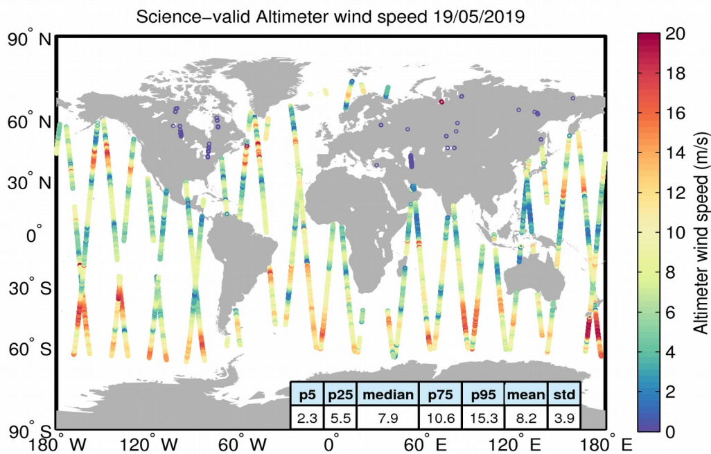
Figure 34. Geographical distribution of science-valid wind data over oceans and lakes for 19/05/2019. The statistical values shown in the table refer to the wind in m/s and are calculated over all measurements shown in the figure. Gray circles denote records that have been rejected based on the editing criteria described in Table 5.
