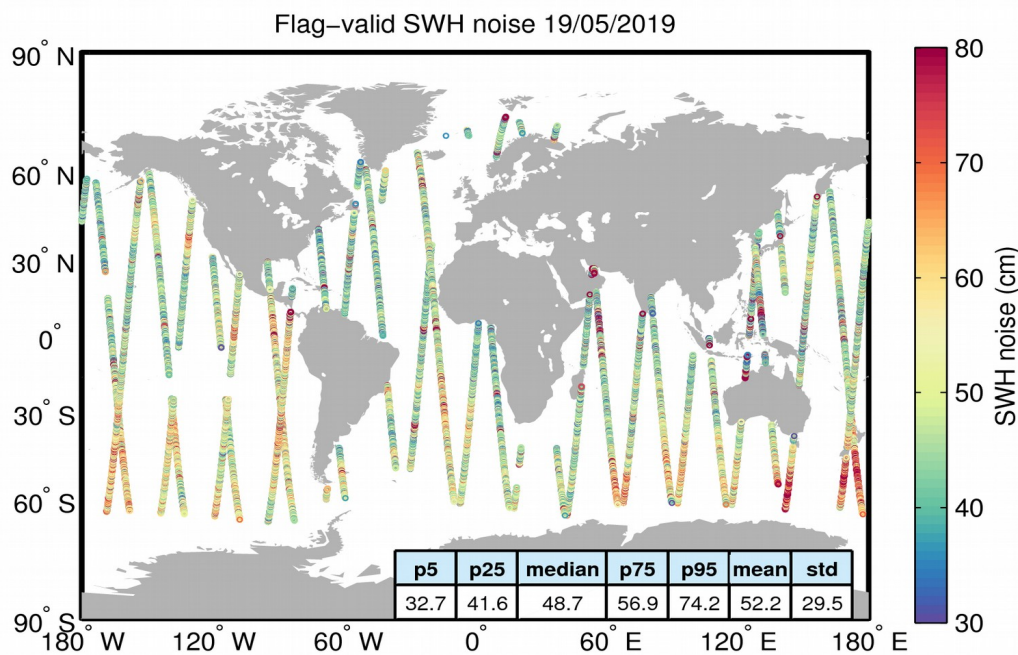
Figure 18. Geographical distribution of flag-valid 20-Hz SWH measurement noise over oceans and lakes for 19/05/2019. The statistical values shown in the figure refer to the SWH noise and are calculated over all measurements shown in the figure.
