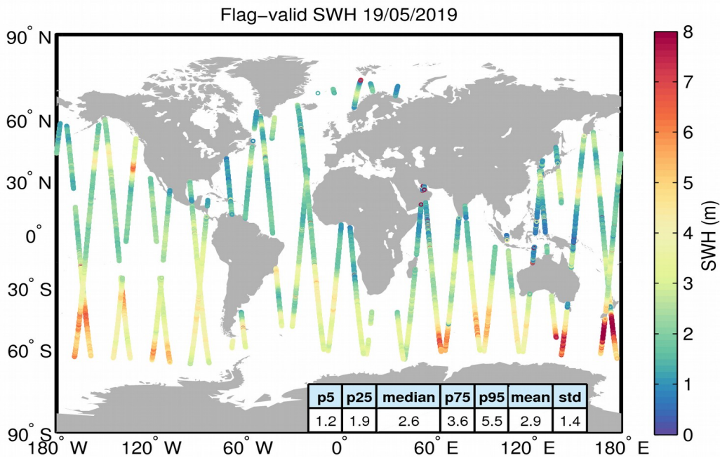
Figure 15. Geographical distribution of flag-valid SWH data over oceans and lakes for 19/05/2019. The statistical values shown in the table refer to the SWH in m and are calculated over all measurements shown in the figure.
