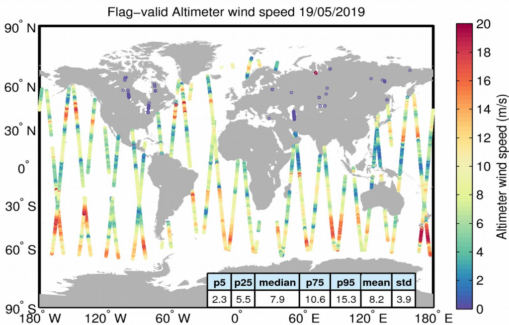
Figure 31. Geographical distribution of flag-valid wind data over oceans and lakes for 19/05/2019. The statistical values shown in the table refer to the wind in m/s and are calculated over all measurements shown in the figure.
