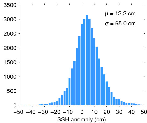
Figure 7. Histogram of flag-valid SSH anomaly over oceans and lakes for 19/05/2019. The mean ( \mu ) and standard deviation ( \sigma ) are also shown. Note that values outside [-50\ 50] cm are excluded from the histogram for the sake of readability but not from the computation of \mu and \sigma .
