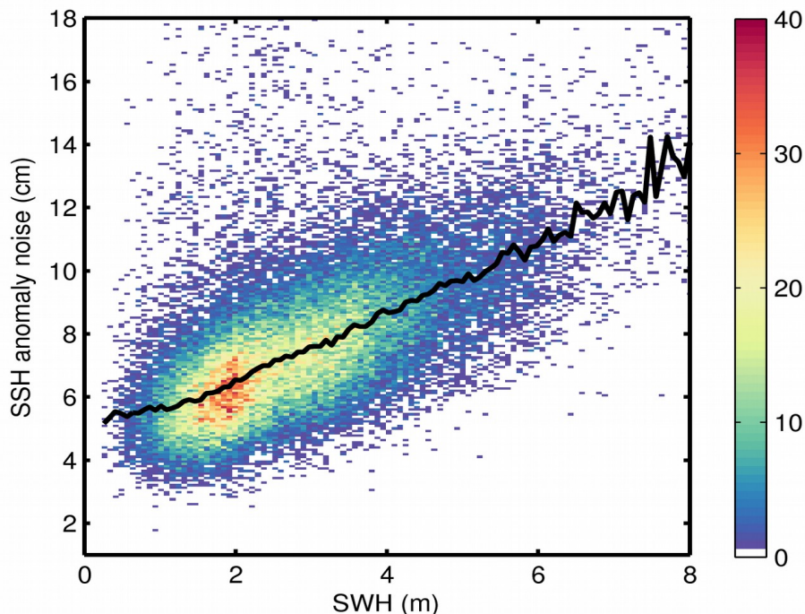
Figure 9. 2D histogram showing flag-valid SSH anomaly noise as a function of SWH for 19/05/2019. The black line denotes the median SSH anomaly noise as a function of SWH.
