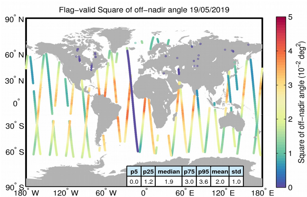
Figure 37. Geographical distribution of flag-valid mispointing data over oceans and lakes for 19/05/2019. The statistical values shown in the table refer to the mispointing in 10^{-2} deg 2 and are calculated over all measurements shown in the figure.
