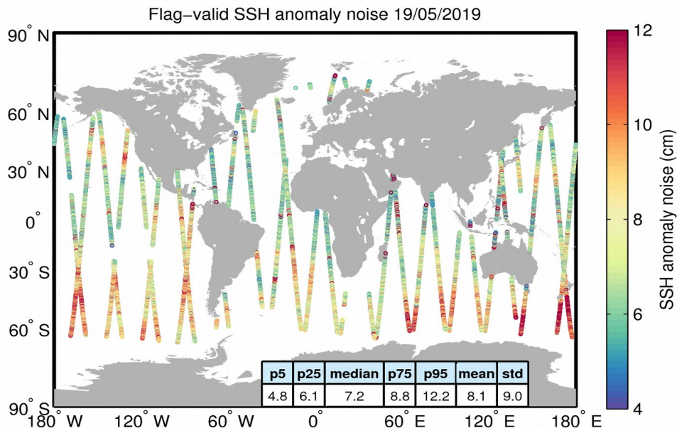
Figure 8. Geographical distribution of flag-valid 20-Hz SSH anomaly measurement noise over oceans and lakes for 19/05/2019. The statistical values shown in the table refer to the SSH anomaly noise and are calculated over all measurements shown in the figure.
