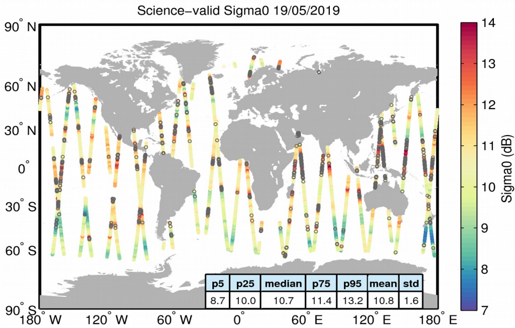
Figure 27. Geographical distribution of science-valid sigma0 data over oceans and lakes for 19/05/2019. The statistical values shown in the table refer to the sigma0 in dB and are calculated over all measurements shown in the figure. Gray circles denote records that have been rejected based on the editing criteria described in Table 4.
