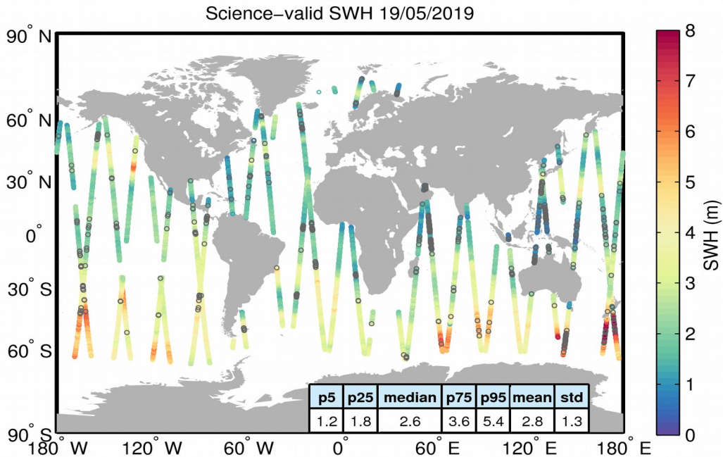
Figure 19. Geographical distribution of science-valid SWH data over oceans and lakes for 19/05/2019. The statistical values shown in the table refer to the SWH in m and are calculated over all measurements shown in the figure. Gray circles denote records that have been rejected based on the editing criteria described in Table 3.
