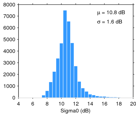
Figure 28. Histogram of science-valid sigma0 over oceans and lakes for 19/05/2019. The mean ( \mu ) and standard deviation ( \sigma ) are also shown. Note that values outside [4 20] dB are excluded from the histogram for the sake of readability but not from the computation of \mu and \sigma .
