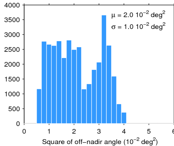
Figure 39. Histogram of flag-valid mispointing over oceans and lakes for 19/05/2019. The mean ( \mu ) and standard deviation ( \sigma ) are also shown. Note that values larger than 6 \cdot 10^{-2} \text{ deg}^2 are excluded from the histogram for the sake of readability but not from the computation of \mu and \sigma .
