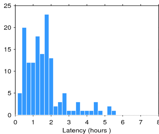
Figure 2. Histogram of the data latency for 19/05/2019. The y-axis denotes the number of files that are made available with a delay of x-hours with respect to the mean time of the records stored in the file.
