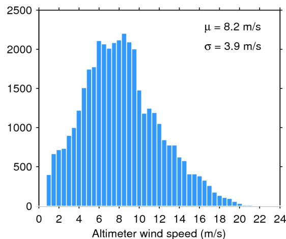
Figure 35. Histogram of science-valid wind over oceans and lakes for 19/05/2019. The mean ( \mu ) and standard deviation ( \sigma ) are also shown. Note that values larger than 24 m/s are excluded from the histogram for the sake of readability but not from the computation of \mu and \sigma .
