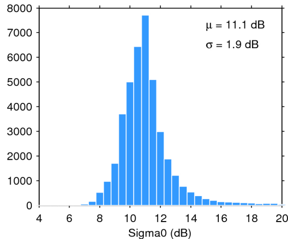
Figure 25. Histogram of flag-valid sigma0 over oceans and lakes for 17/05/2019. The mean ( \mu ) and standard deviation ( \sigma ) are also shown. Note that values outside [4 20] dB are excluded from the histogram for the sake of readability but not from the computation of \mu and \sigma .
