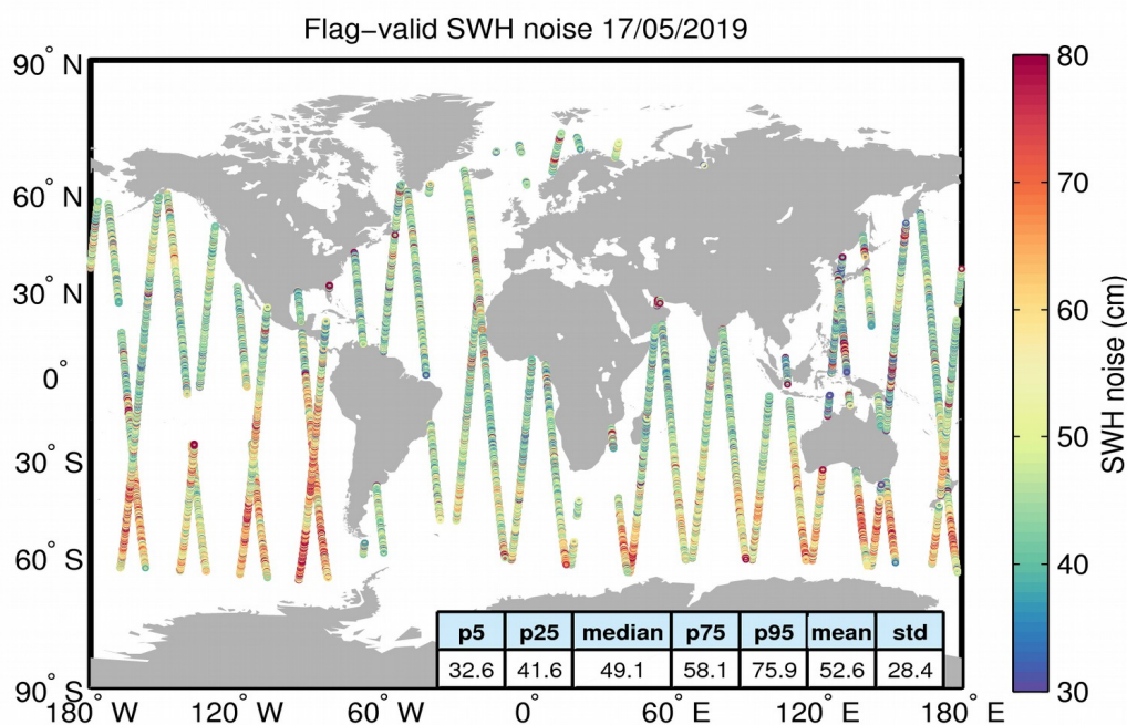
Figure 18. Geographical distribution of flag-valid 20-Hz SWH measurement noise over oceans and lakes for 17/05/2019. The statistical values shown in the figure refer to the SWH noise and are calculated over all measurements shown in the figure.
