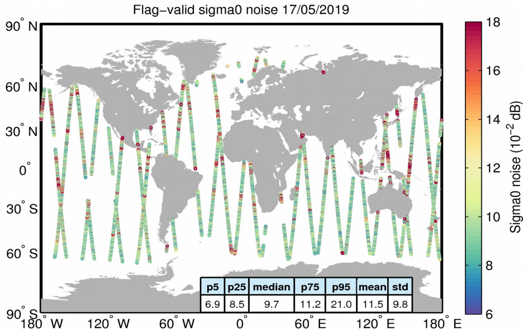
Figure 26. Geographical distribution of flag-valid 20-Hz sigma0 measurement noise over oceans and lakes for 17/05/2019. The statistical values shown in the table refer to the sigma0 noise and are calculated over all measurements shown in the figure.
