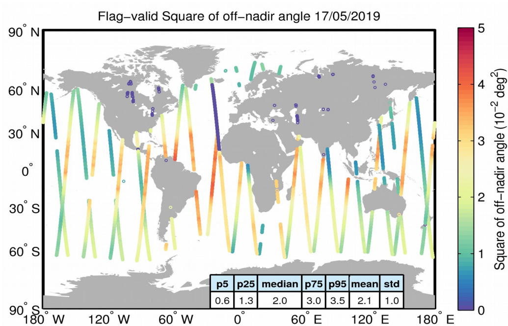
Figure 37. Geographical distribution of flag-valid mispointing data over oceans and lakes for 17/05/2019. The statistical values shown in the table refer to the mispointing in 10^{-2} deg 2 and are calculated over all measurements shown in the figure.
