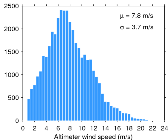
Figure 35. Histogram of science-valid wind over oceans and lakes for 17/05/2019. The mean ( \mu ) and standard deviation ( \sigma ) are also shown. Note that values larger than 24 m/s are excluded from the histogram for the sake of readability but not from the computation of \mu and \sigma .
