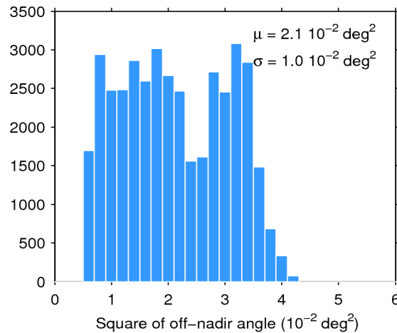
Figure 39. Histogram of flag-valid mispointing over oceans and lakes for 17/05/2019. The mean ( \mu ) and standard deviation ( \sigma ) are also shown. Note that values larger than 6 \cdot 10^{-2} \text{ deg}^2 are excluded from the histogram for the sake of readability but not from the computation of \mu and \sigma .
