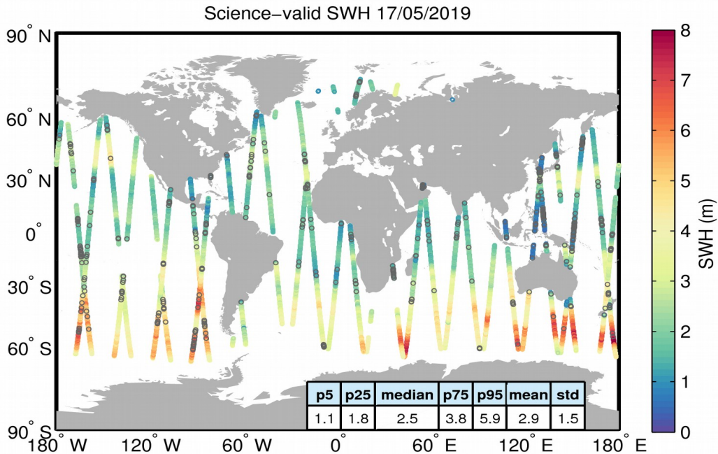
Figure 19. Geographical distribution of science-valid SWH data over oceans and lakes for 17/05/2019. The statistical values shown in the table refer to the SWH in m and are calculated over all measurements shown in the figure. Gray circles denote records that have been rejected based on the editing criteria described in Table 3.
