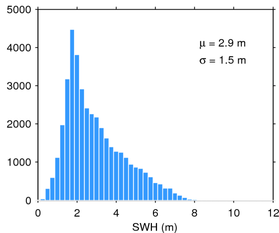
Figure 20. Histogram of science-valid SWH over oceans and lakes for 17/05/2019. The mean ( \mu ) and standard deviation ( \sigma ) are also shown. Note that values larger than 12 m are excluded from the histogram for the sake of readability but not from the computation of \mu and \sigma .
