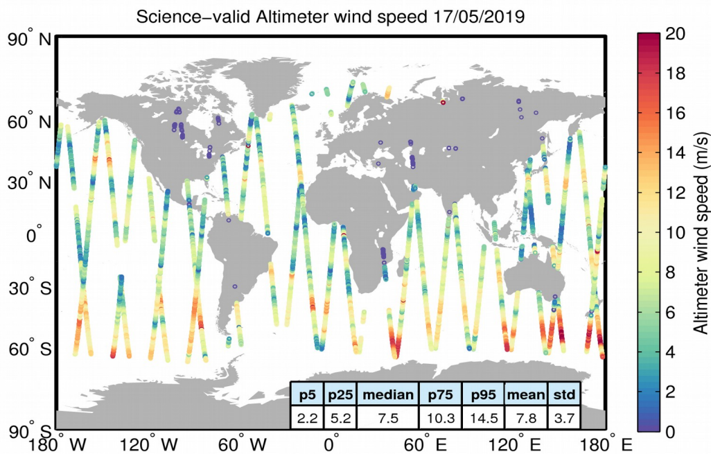
Figure 34. Geographical distribution of science-valid wind data over oceans and lakes for 17/05/2019. The statistical values shown in the table refer to the wind in m/s and are calculated over all measurements shown in the figure. Gray circles denote records that have been rejected based on the editing criteria described in Table 5.
