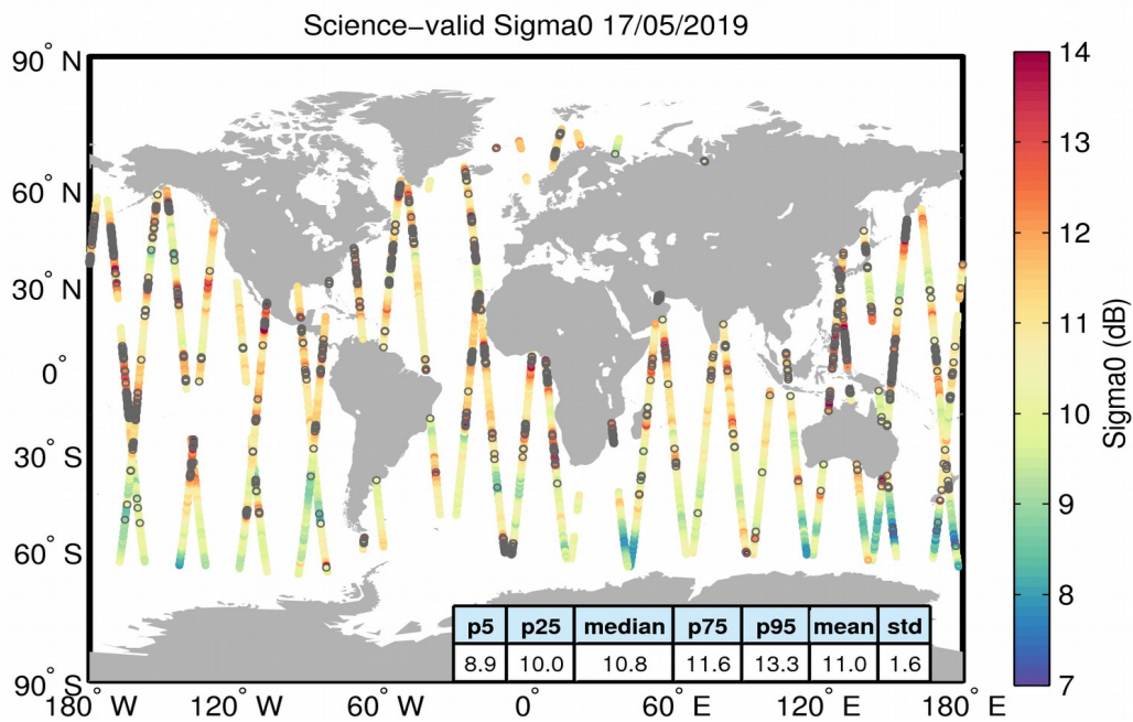
Figure 27. Geographical distribution of science-valid sigma0 data over oceans and lakes for 17/05/2019. The statistical values shown in the table refer to the sigma0 in dB and are calculated over all measurements shown in the figure. Gray circles denote records that have been rejected based on the editing criteria described in Table 4.
