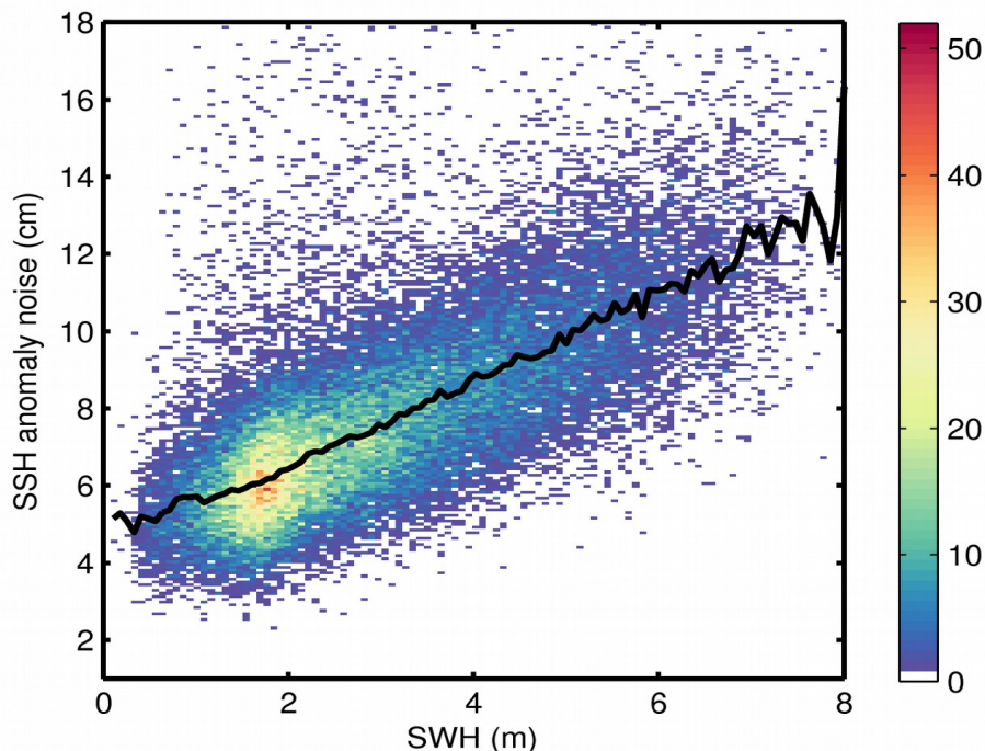
Figure 9. 2D histogram showing flag-valid SSH anomaly noise as a function of SWH for 17/05/2019. The black line denotes the median SSH anomaly noise as a function of SWH.
