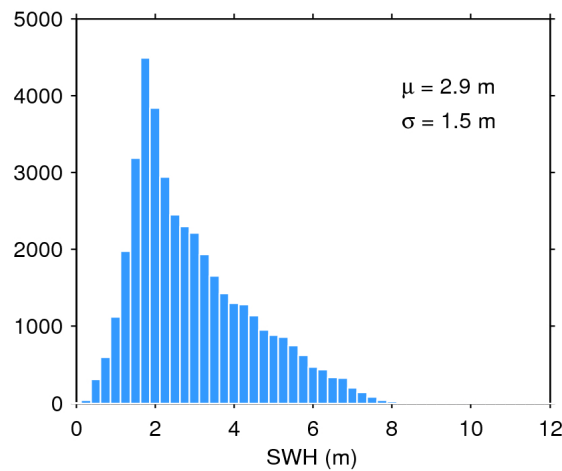
Figure 17. Histogram of flag-valid SWH over oceans and lakes for 17/05/2019. The mean ( \mu ) and standard deviation ( \sigma ) are also shown. Note that values larger than 12 m are excluded from the histogram for the sake of readability but not from the computation of \mu and \sigma .
