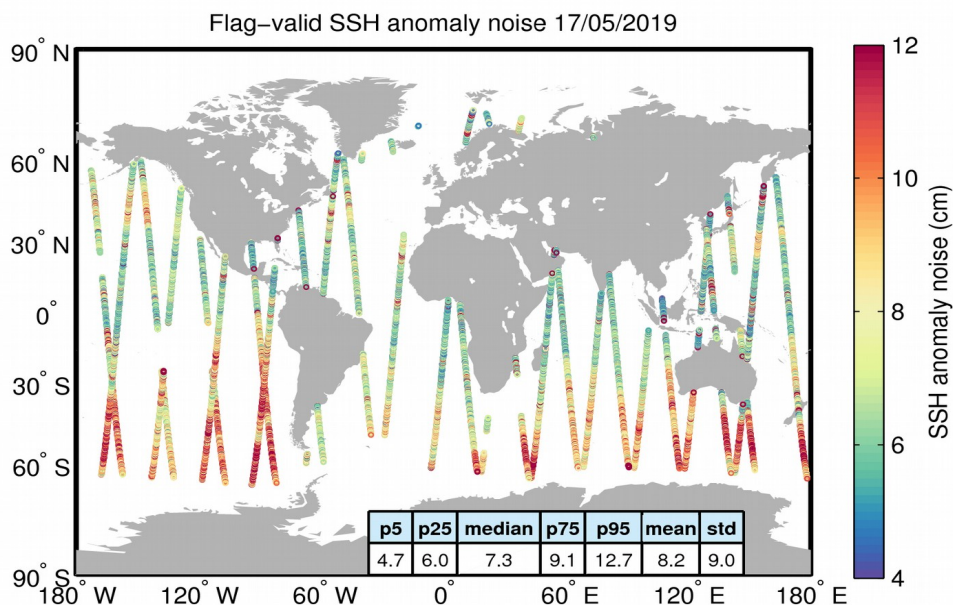
Figure 8. Geographical distribution of flag-valid 20-Hz SSH anomaly measurement noise over oceans and lakes for 17/05/2019. The statistical values shown in the table refer to the SSH anomaly noise and are calculated over all measurements shown in the figure.
