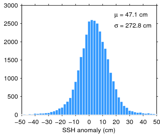
Figure 7. Histogram of flag-valid SSH anomaly over oceans and lakes for 17/05/2019. The mean ( \mu ) and standard deviation ( \sigma ) are also shown. Note that values outside [-50\ 50] cm are excluded from the histogram for the sake of readability but not from the computation of \mu and \sigma .
