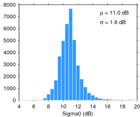
Figure 28. Histogram of science-valid sigma0 over oceans and lakes for 17/05/2019. The mean ( \mu ) and standard deviation ( \sigma ) are also shown. Note that values outside [4 20] dB are excluded from the histogram for the sake of readability but not from the computation of \mu and \sigma .
