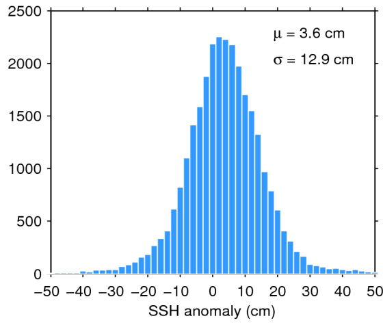
Figure 11. Histogram of science-valid SSH anomaly over oceans and lakes for 17/05/2019. The mean ( \mu ) and standard deviation ( \sigma ) are also shown. Note that values outside [-50 50] cm are excluded from the histogram for the sake of readability but not from the computation of \mu and \sigma .
