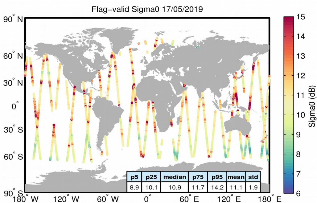
Figure 23. Geographical distribution of flag-valid sigma0 data over oceans and lakes for 17/05/2019. The statistical values shown in the table refer to the sigma0 in dB and are calculated over all measurements shown in the figure.
