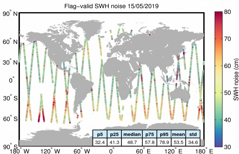
Figure 18. Geographical distribution of flag-valid 20-Hz SWH measurement noise over oceans and lakes for 15/05/2019. The statistical values shown in the figure refer to the SWH noise and are calculated over all measurements shown in the figure.
