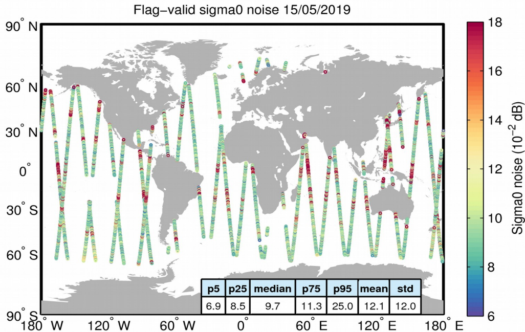
Figure 26. Geographical distribution of flag-valid 20-Hz sigma0 measurement noise over oceans and lakes for 15/05/2019. The statistical values shown in the table refer to the sigma0 noise and are calculated over all measurements shown in the figure.
