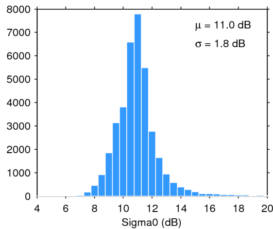
Figure 28. Histogram of science-valid sigma0 over oceans and lakes for 15/05/2019. The mean ( \mu ) and standard deviation ( \sigma ) are also shown. Note that values outside [4 20] dB are excluded from the histogram for the sake of readability but not from the computation of \mu and \sigma .
