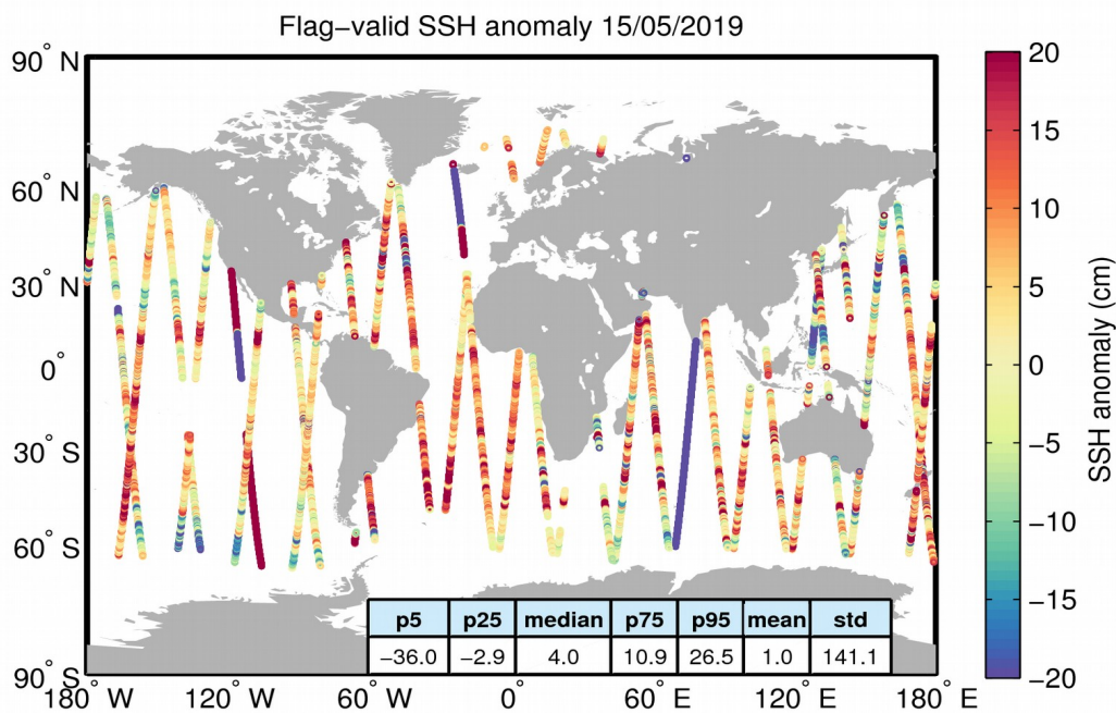
Figure 5. Geographical distribution of flag-valid 1-Hz SSH anomaly data over oceans and lakes for 15/05/2019. The statistical values shown in the table refer to the SSH anomaly in cm and are calculated over all measurements shown in the figure.
