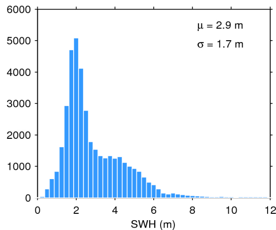
Figure 17. Histogram of flag-valid SWH over oceans and lakes for 15/05/2019. The mean ( \mu ) and standard deviation ( \sigma ) are also shown. Note that values larger than 12 m are excluded from the histogram for the sake of readability but not from the computation of \mu and \sigma .
