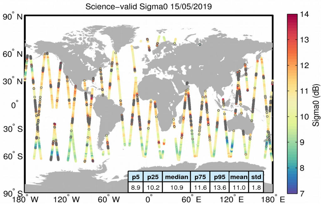
Figure 27. Geographical distribution of science-valid sigma0 data over oceans and lakes for 15/05/2019. The statistical values shown in the table refer to the sigma0 in dB and are calculated over all measurements shown in the figure. Gray circles denote records that have been rejected based on the editing criteria described in Table 4.
