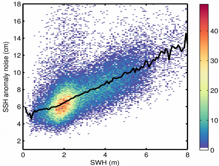
Figure 9. 2D histogram showing flag-valid SSH anomaly noise as a function of SWH for 15/05/2019. The black line denotes the median SSH anomaly noise as a function of SWH.
