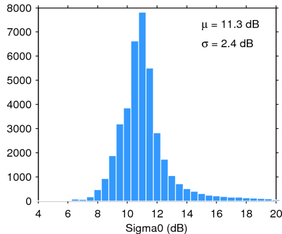
Figure 25. Histogram of flag-valid sigma0 over oceans and lakes for 15/05/2019. The mean ( \mu ) and standard deviation ( \sigma ) are also shown. Note that values outside [4 20] dB are excluded from the histogram for the sake of readability but not from the computation of \mu and \sigma .
