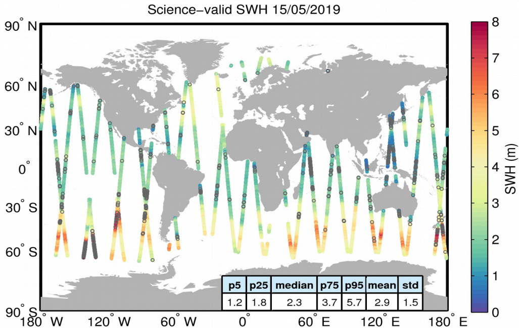
Figure 19. Geographical distribution of science-valid SWH data over oceans and lakes for 15/05/2019. The statistical values shown in the table refer to the SWH in m and are calculated over all measurements shown in the figure. Gray circles denote records that have been rejected based on the editing criteria described in Table 3.
