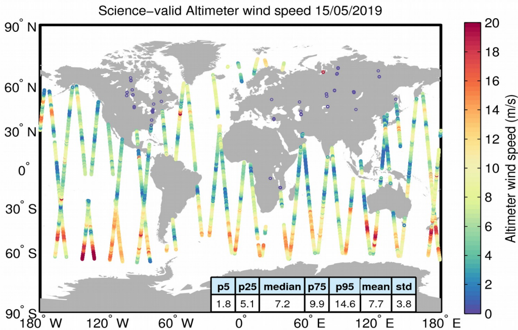
Figure 34. Geographical distribution of science-valid wind data over oceans and lakes for 15/05/2019. The statistical values shown in the table refer to the wind in m/s and are calculated over all measurements shown in the figure. Gray circles denote records that have been rejected based on the editing criteria described in Table 5.
