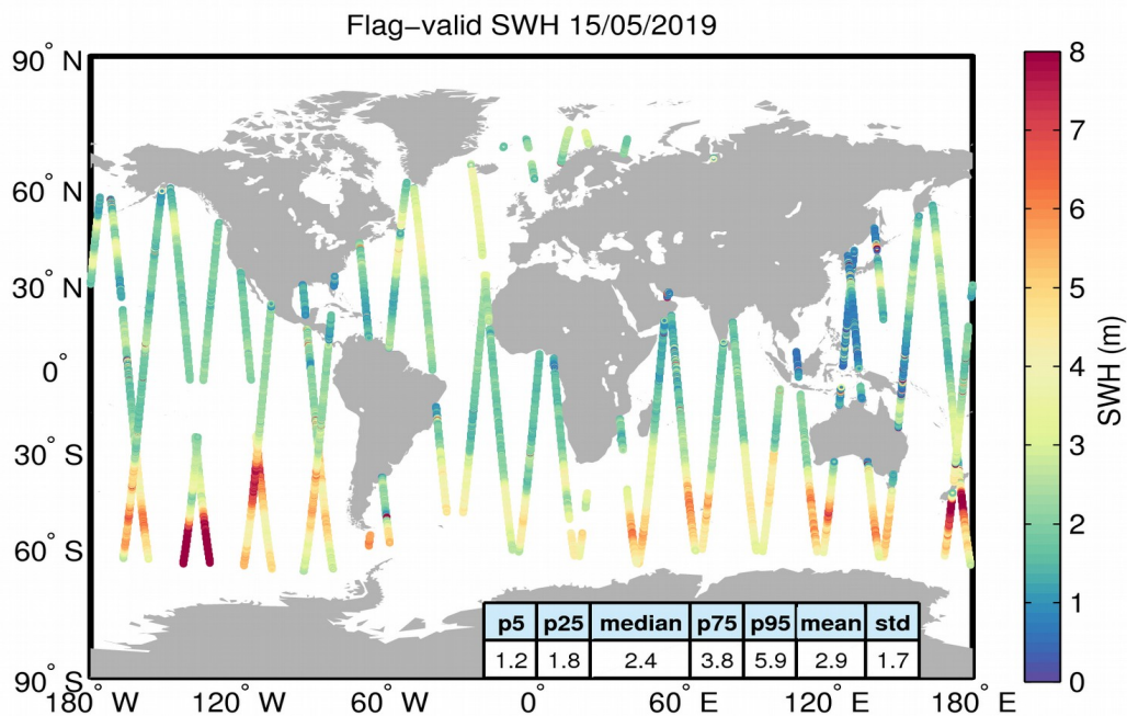
Figure 15. Geographical distribution of flag-valid SWH data over oceans and lakes for 15/05/2019. The statistical values shown in the table refer to the SWH in m and are calculated over all measurements shown in the figure.
