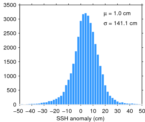
Figure 7. Histogram of flag-valid SSH anomaly over oceans and lakes for 15/05/2019. The mean ( \mu ) and standard deviation ( \sigma ) are also shown. Note that values outside [-50 50] cm are excluded from the histogram for the sake of readability but not from the computation of \mu and \sigma .
