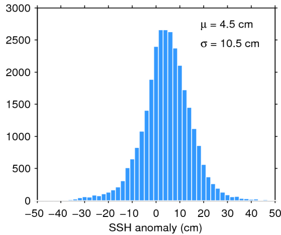
Figure 11. Histogram of science-valid SSH anomaly over oceans and lakes for 15/05/2019. The mean ( \mu ) and standard deviation ( \sigma ) are also shown. Note that values outside [-50 50] cm are excluded from the histogram for the sake of readability but not from the computation of \mu and \sigma .
