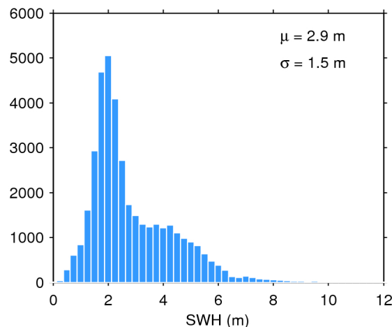
Figure 20. Histogram of science-valid SWH over oceans and lakes for 15/05/2019. The mean ( \mu ) and standard deviation ( \sigma ) are also shown. Note that values larger than 12 m are excluded from the histogram for the sake of readability but not from the computation of \mu and \sigma .
