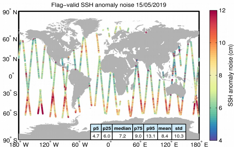
Figure 8. Geographical distribution of flag-valid 20-Hz SSH anomaly measurement noise over oceans and lakes for 15/05/2019. The statistical values shown in the table refer to the SSH anomaly noise and are calculated over all measurements shown in the figure.
