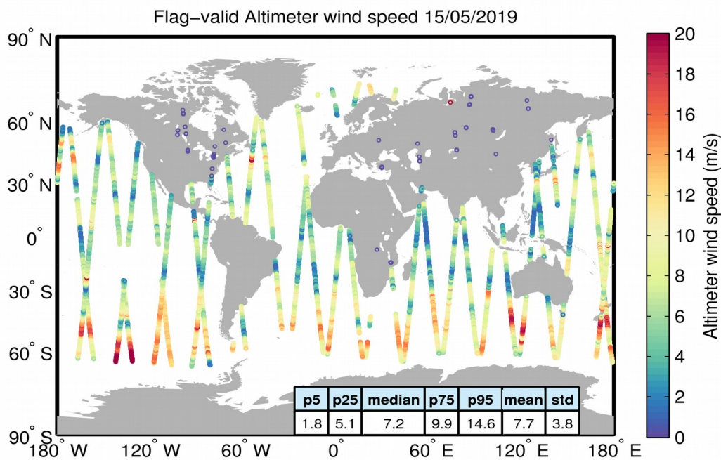
Figure 31. Geographical distribution of flag-valid wind data over oceans and lakes for 15/05/2019. The statistical values shown in the table refer to the wind in m/s and are calculated over all measurements shown in the figure.
