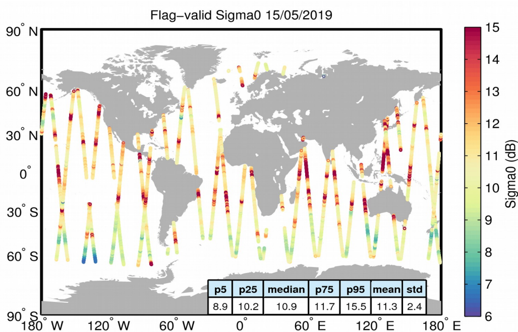
Figure 23. Geographical distribution of flag-valid sigma0 data over oceans and lakes for 15/05/2019. The statistical values shown in the table refer to the sigma0 in dB and are calculated over all measurements shown in the figure.
