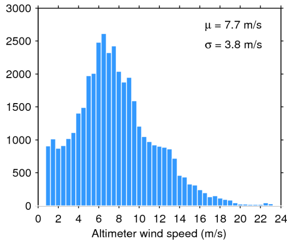
Figure 33. Histogram of flag-valid wind over oceans and lakes for 15/05/2019. The mean ( \mu ) and standard deviation ( \sigma ) are also shown. Note that values larger than 24 m/s are excluded from the histogram for the sake of readability but not from the computation of \mu and \sigma .
