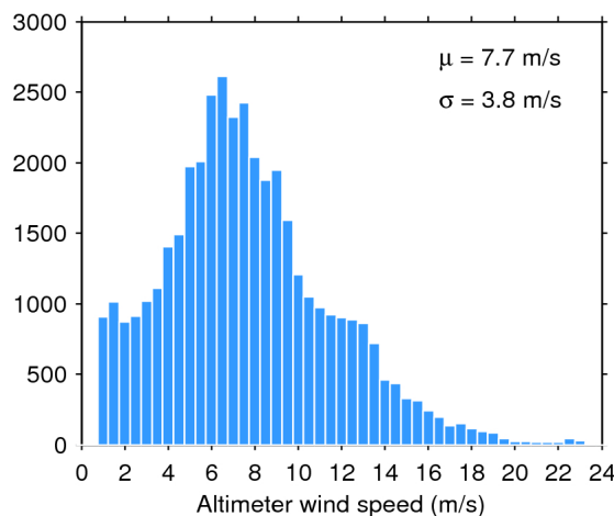
Figure 35. Histogram of science-valid wind over oceans and lakes for 15/05/2019. The mean ( \mu ) and standard deviation ( \sigma ) are also shown. Note that values larger than 24 m/s are excluded from the histogram for the sake of readability but not from the computation of \mu and \sigma .
