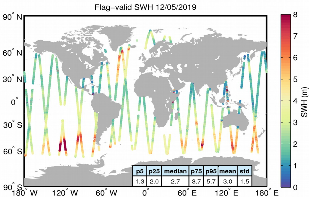
Figure 15. Geographical distribution of flag-valid SWH data over oceans and lakes for 12/05/2019. The statistical values shown in the table refer to the SWH in m and are calculated over all measurements shown in the figure.
