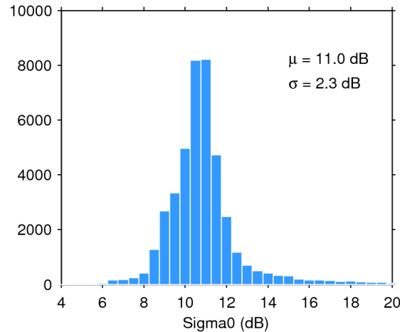
Figure 25. Histogram of flag-valid sigma0 over oceans and lakes for 12/05/2019. The mean ( \mu ) and standard deviation ( \sigma ) are also shown. Note that values outside [4 20] dB are excluded from the histogram for the sake of readability but not from the computation of \mu and \sigma .
