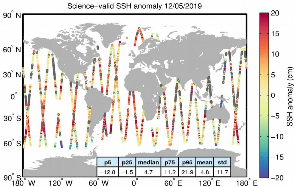
Figure 10. Geographical distribution of science-valid SSH anomaly data over oceans and lakes for 12/05/2019. The statistical values shown in the table refer to the SSH anomaly in cm and are calculated over all measurements shown in the figure. Gray circles denote records that have been rejected based on the editing criteria described in Table 2.
