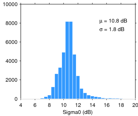
Figure 28. Histogram of science-valid sigma0 over oceans and lakes for 12/05/2019. The mean ( \mu ) and standard deviation ( \sigma ) are also shown. Note that values outside [4 20] dB are excluded from the histogram for the sake of readability but not from the computation of \mu and \sigma .
