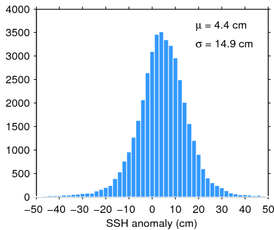
Figure 7. Histogram of flag-valid SSH anomaly over oceans and lakes for 12/05/2019. The mean ( \mu ) and standard deviation ( \sigma ) are also shown. Note that values outside [-50 50] cm are excluded from the histogram for the sake of readability but not from the computation of \mu and \sigma .
