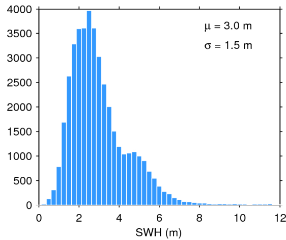
Figure 17. Histogram of flag-valid SWH over oceans and lakes for 12/05/2019. The mean ( \mu ) and standard deviation ( \sigma ) are also shown. Note that values larger than 12 m are excluded from the histogram for the sake of readability but not from the computation of \mu and \sigma .
