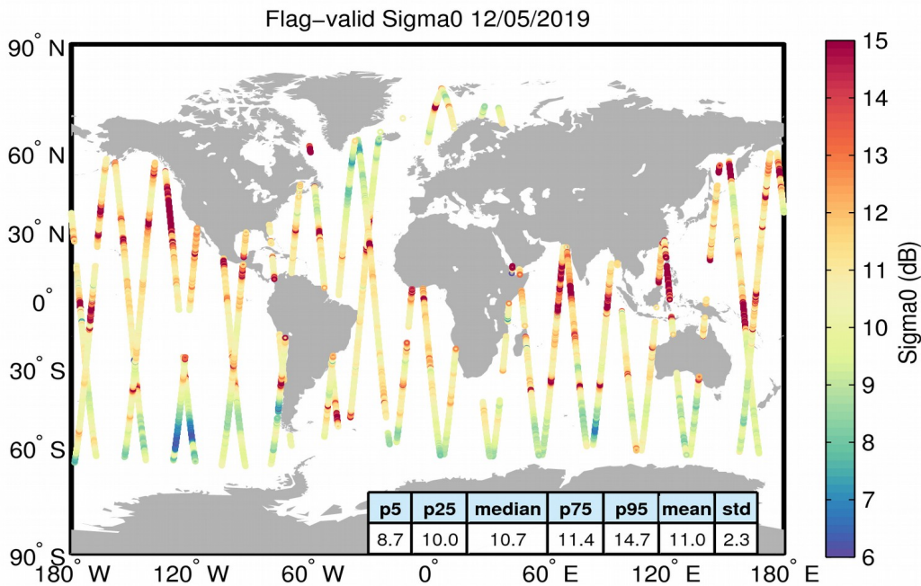
Figure 23. Geographical distribution of flag-valid sigma0 data over oceans and lakes for 12/05/2019. The statistical values shown in the table refer to the sigma0 in dB and are calculated over all measurements shown in the figure.
