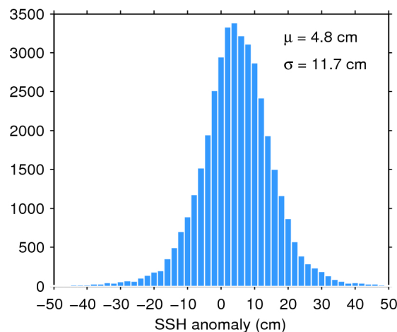
Figure 11. Histogram of science-valid SSH anomaly over oceans and lakes for 12/05/2019. The mean ( \mu ) and standard deviation ( \sigma ) are also shown. Note that values outside [-50 50] cm are excluded from the histogram for the sake of readability but not from the computation of \mu and \sigma .
