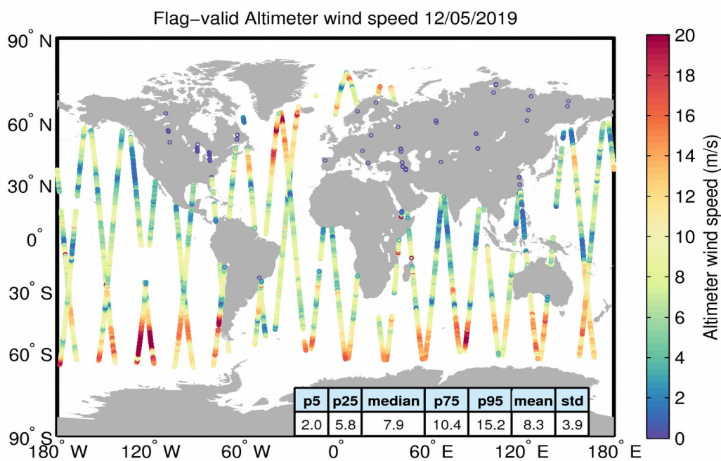
Figure 31. Geographical distribution of flag-valid wind data over oceans and lakes for 12/05/2019. The statistical values shown in the table refer to the wind in m/s and are calculated over all measurements shown in the figure.
