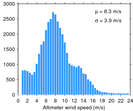
Figure 33. Histogram of flag-valid wind over oceans and lakes for 12/05/2019. The mean ( \mu ) and standard deviation ( \sigma ) are also shown. Note that values larger than 24 m/s are excluded from the histogram for the sake of readability but not from the computation of \mu and \sigma .
