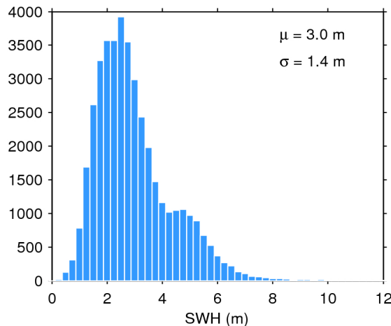
Figure 20. Histogram of science-valid SWH over oceans and lakes for 12/05/2019. The mean ( \mu ) and standard deviation ( \sigma ) are also shown. Note that values larger than 12 m are excluded from the histogram for the sake of readability but not from the computation of \mu and \sigma .
