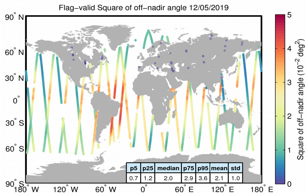
Figure 37. Geographical distribution of flag-valid mispointing data over oceans and lakes for 12/05/2019. The statistical values shown in the table refer to the mispointing in 10^{-2} \text{ deg}^2 and are calculated over all measurements shown in the figure.
