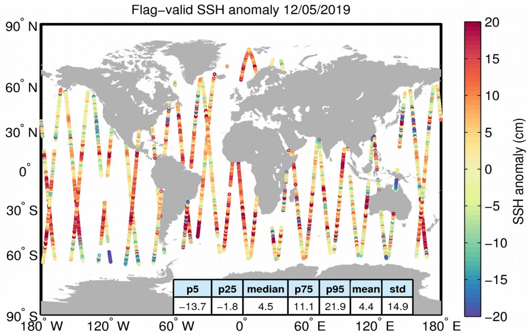
Figure 5. Geographical distribution of flag-valid 1-Hz SSH anomaly data over oceans and lakes for 12/05/2019. The statistical values shown in the table refer to the SSH anomaly in cm and are calculated over all measurements shown in the figure.
