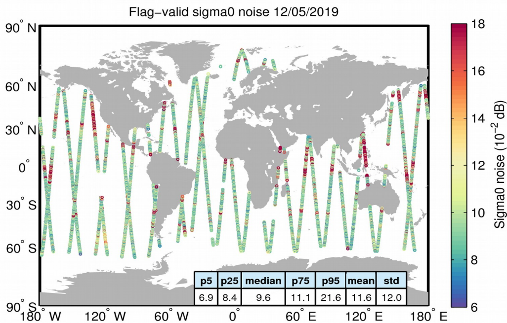
Figure 26. Geographical distribution of flag-valid 20-Hz sigma0 measurement noise over oceans and lakes for 12/05/2019. The statistical values shown in the table refer to the sigma0 noise and are calculated over all measurements shown in the figure.
