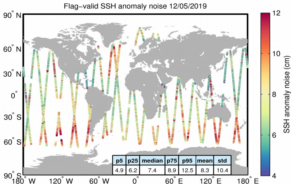
Figure 8. Geographical distribution of flag-valid 20-Hz SSH anomaly measurement noise over oceans and lakes for 12/05/2019. The statistical values shown in the table refer to the SSH anomaly noise and are calculated over all measurements shown in the figure.
