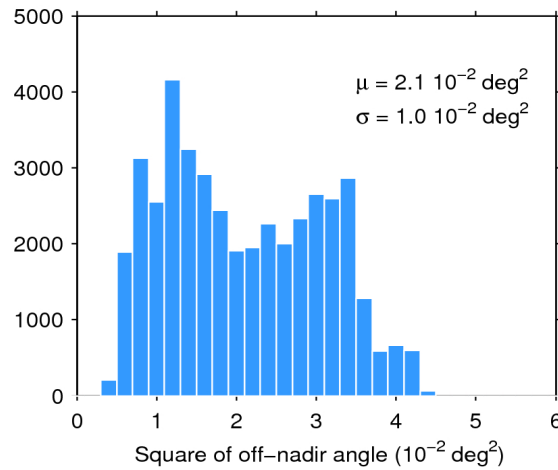
Figure 39. Histogram of flag-valid mispointing over oceans and lakes for 12/05/2019. The mean ( \mu ) and standard deviation ( \sigma ) are also shown. Note that values larger than 6 \cdot 10^{-2} \text{ deg}^2 are excluded from the histogram for the sake of readability but not from the computation of \mu and \sigma .
