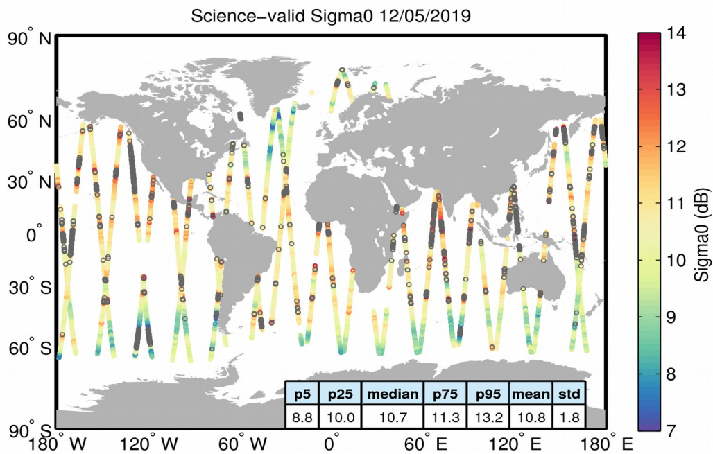
Figure 27. Geographical distribution of science-valid sigma0 data over oceans and lakes for 12/05/2019. The statistical values shown in the table refer to the sigma0 in dB and are calculated over all measurements shown in the figure. Gray circles denote records that have been rejected based on the editing criteria described in Table 4.
