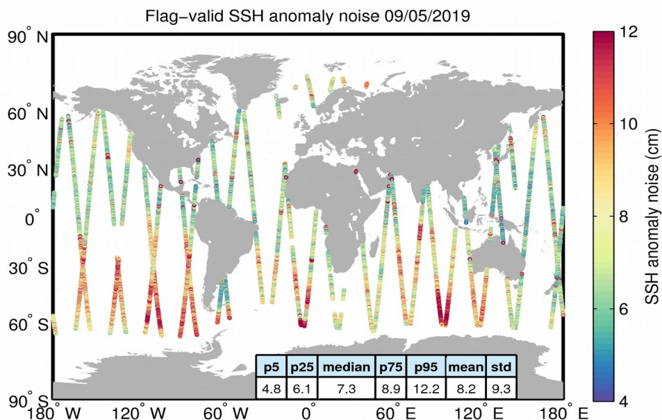
Figure 8. Geographical distribution of flag-valid 20-Hz SSH anomaly measurement noise over oceans and lakes for 09/05/2019. The statistical values shown in the table refer to the SSH anomaly noise and are calculated over all measurements shown in the figure.
