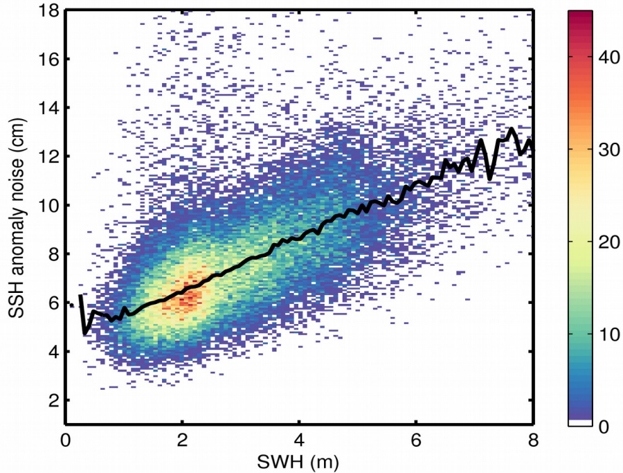
Figure 9. 2D histogram showing flag-valid SSH anomaly noise as a function of SWH for 09/05/2019. The black line denotes the median SSH anomaly noise as a function of SWH.
