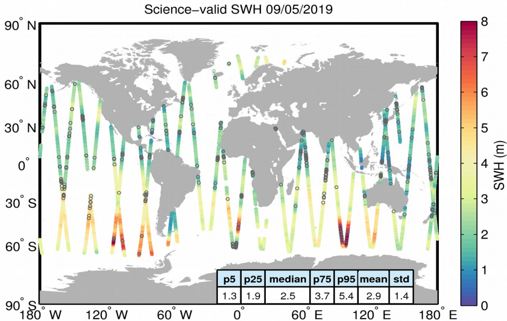
Figure 19. Geographical distribution of science-valid SWH data over oceans and lakes for 09/05/2019. The statistical values shown in the table refer to the SWH in m and are calculated over all measurements shown in the figure. Gray circles denote records that have been rejected based on the editing criteria described in Table 3.
