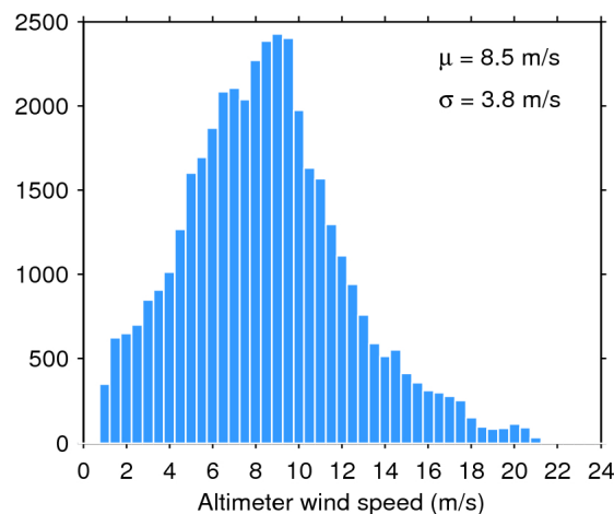
Figure 35. Histogram of science-valid wind over oceans and lakes for 09/05/2019. The mean ( \mu ) and standard deviation ( \sigma ) are also shown. Note that values larger than 24 m/s are excluded from the histogram for the sake of readability but not from the computation of \mu and \sigma .
