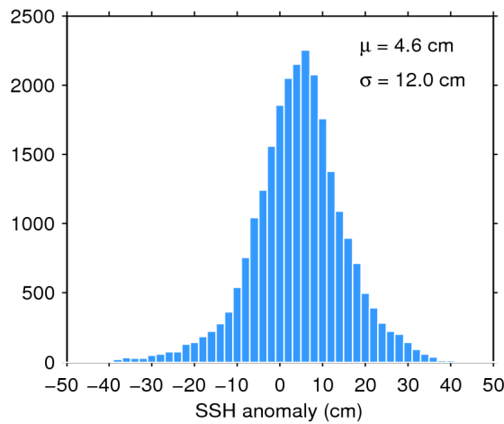
Figure 11. Histogram of science-valid SSH anomaly over oceans and lakes for 09/05/2019. The mean ( \mu ) and standard deviation ( \sigma ) are also shown. Note that values outside [-50 50] cm are excluded from the histogram for the sake of readability but not from the computation of \mu and \sigma .
