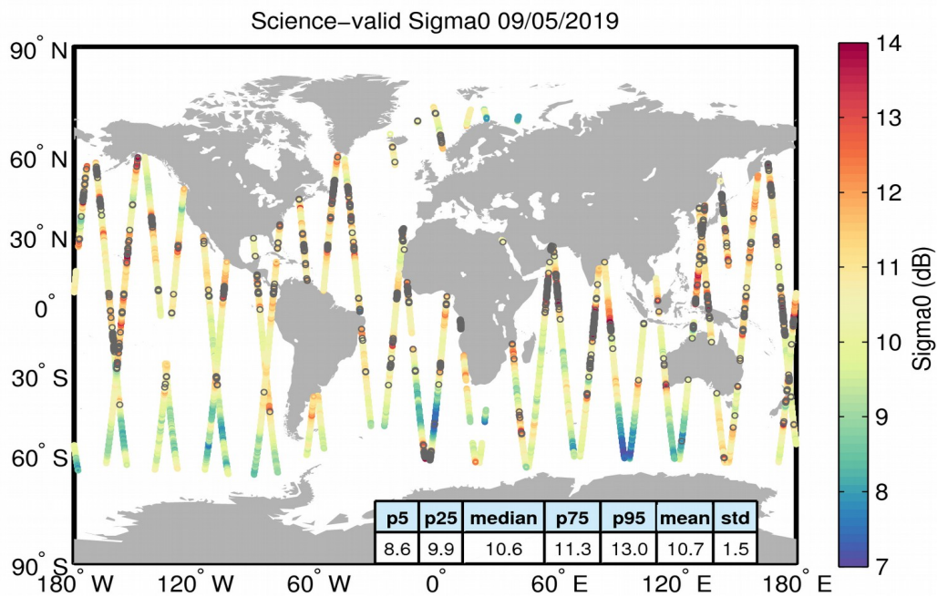
Figure 27. Geographical distribution of science-valid sigma0 data over oceans and lakes for 09/05/2019. The statistical values shown in the table refer to the sigma0 in dB and are calculated over all measurements shown in the figure. Gray circles denote records that have been rejected based on the editing criteria described in Table 4.
