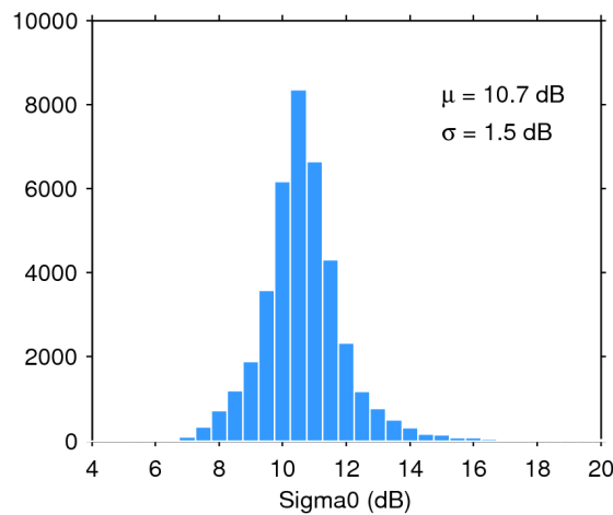
Figure 28. Histogram of science-valid sigma0 over oceans and lakes for 09/05/2019. The mean ( \mu ) and standard deviation ( \sigma ) are also shown. Note that values outside [4 20] dB are excluded from the histogram for the sake of readability but not from the computation of \mu and \sigma .
