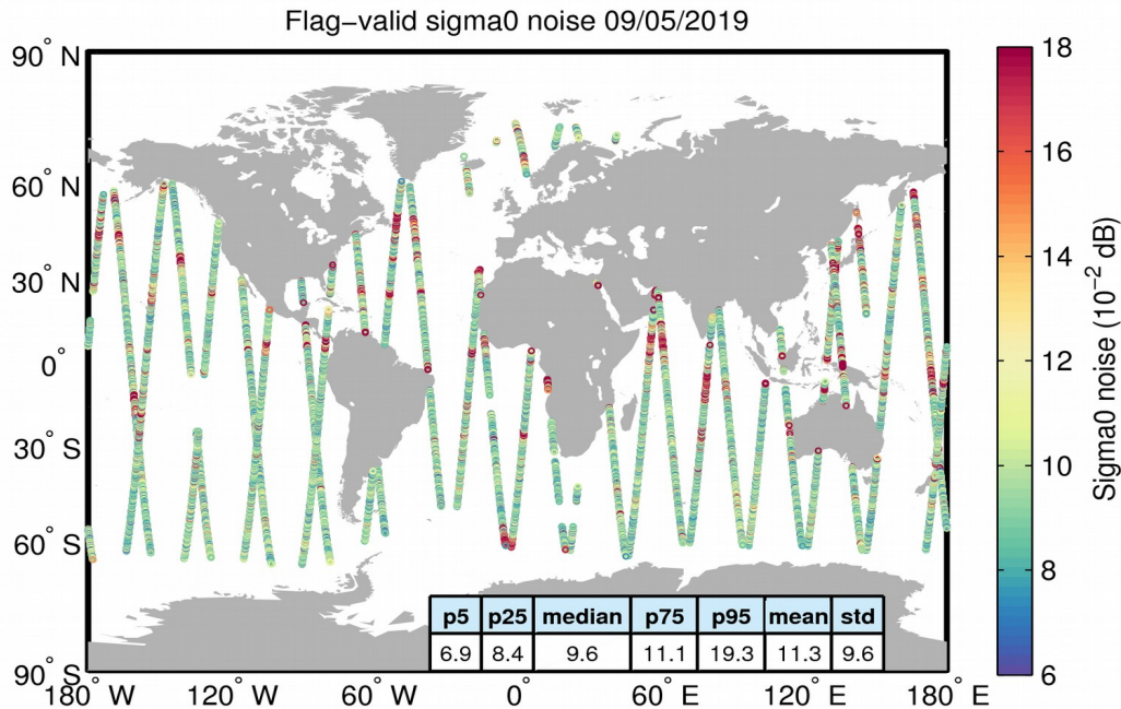
Figure 26. Geographical distribution of flag-valid 20-Hz sigma0 measurement noise over oceans and lakes for 09/05/2019. The statistical values shown in the table refer to the sigma0 noise and are calculated over all measurements shown in the figure.
