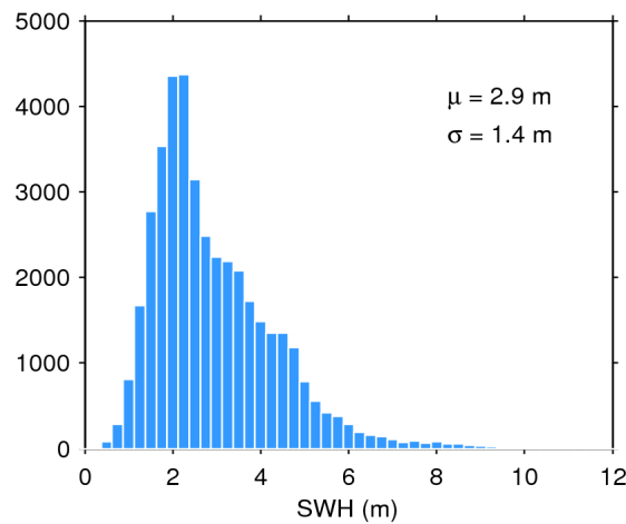
Figure 17. Histogram of flag-valid SWH over oceans and lakes for 09/05/2019. The mean ( \mu ) and standard deviation ( \sigma ) are also shown. Note that values larger than 12 m are excluded from the histogram for the sake of readability but not from the computation of \mu and \sigma .
