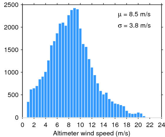
Figure 33. Histogram of flag-valid wind over oceans and lakes for 09/05/2019. The mean ( \mu ) and standard deviation ( \sigma ) are also shown. Note that values larger than 24 m/s are excluded from the histogram for the sake of readability but not from the computation of \mu and \sigma .
