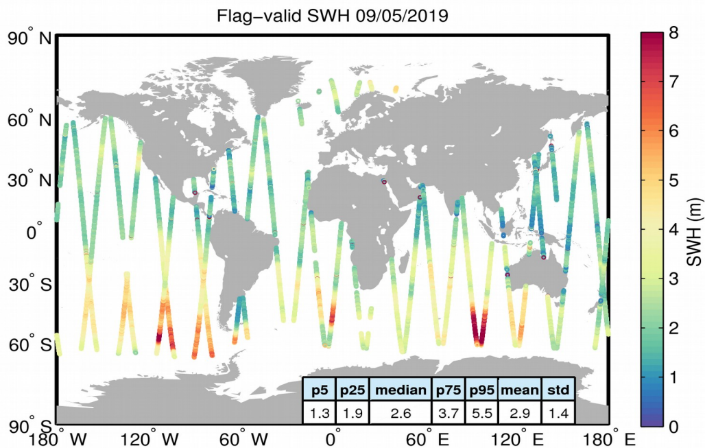
Figure 15. Geographical distribution of flag-valid SWH data over oceans and lakes for 09/05/2019. The statistical values shown in the table refer to the SWH in m and are calculated over all measurements shown in the figure.
