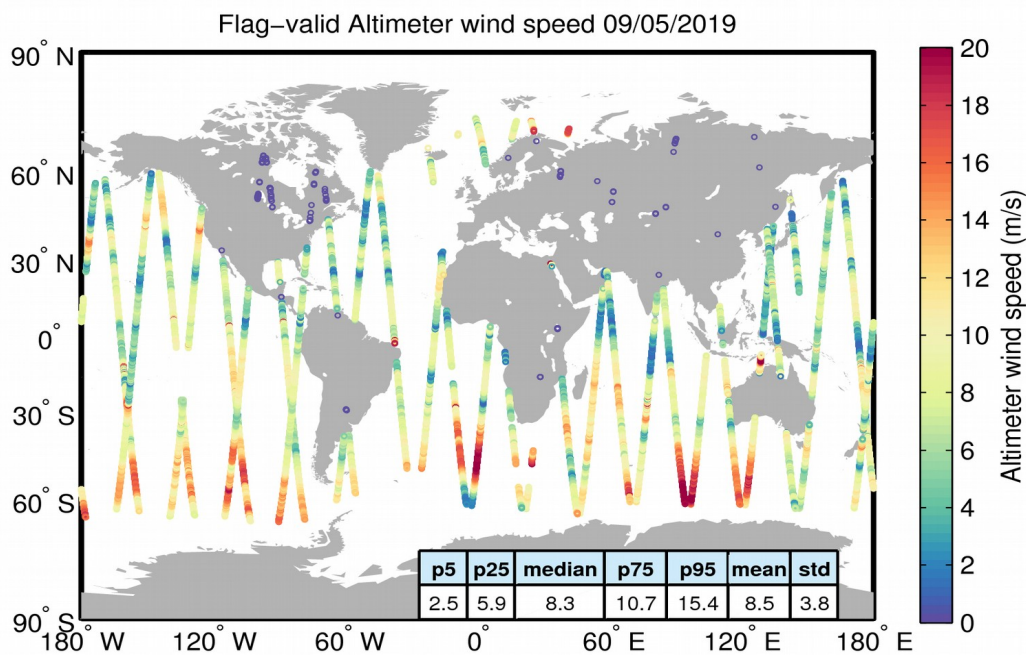
Figure 31. Geographical distribution of flag-valid wind data over oceans and lakes for 09/05/2019. The statistical values shown in the table refer to the wind in m/s and are calculated over all measurements shown in the figure.
