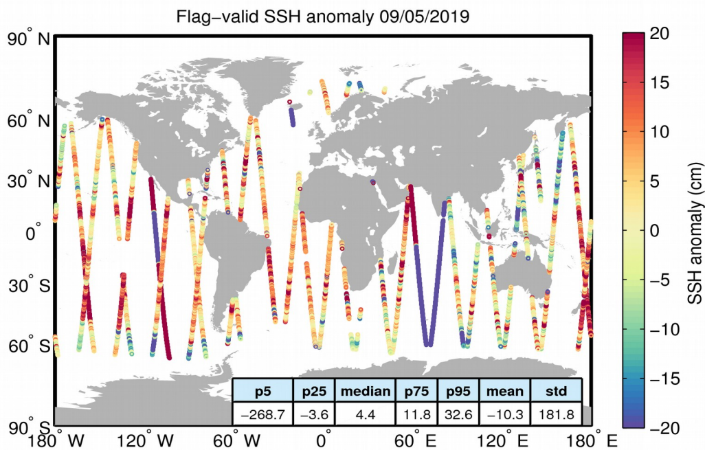
Figure 5. Geographical distribution of flag-valid 1-Hz SSH anomaly data over oceans and lakes for 09/05/2019. The statistical values shown in the table refer to the SSH anomaly in cm and are calculated over all measurements shown in the figure.
