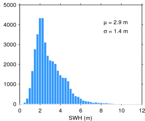
Figure 20. Histogram of science-valid SWH over oceans and lakes for 09/05/2019. The mean ( \mu ) and standard deviation ( \sigma ) are also shown. Note that values larger than 12 m are excluded from the histogram for the sake of readability but not from the computation of \mu and \sigma .
