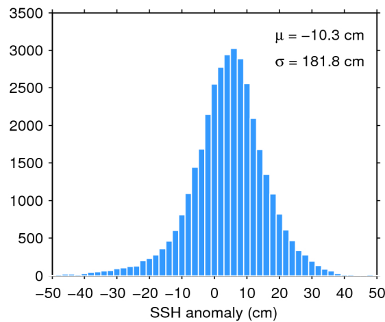
Figure 7. Histogram of flag-valid SSH anomaly over oceans and lakes for 09/05/2019. The mean ( \mu ) and standard deviation ( \sigma ) are also shown. Note that values outside [-50\ 50] cm are excluded from the histogram for the sake of readability but not from the computation of \mu and \sigma .
