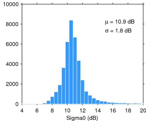
Figure 25. Histogram of flag-valid sigma0 over oceans and lakes for 09/05/2019. The mean ( \mu ) and standard deviation ( \sigma ) are also shown. Note that values outside [4 20] dB are excluded from the histogram for the sake of readability but not from the computation of \mu and \sigma .
