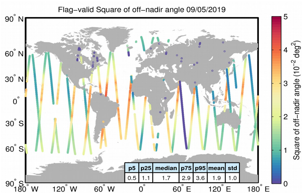
Figure 37. Geographical distribution of flag-valid mispointing data over oceans and lakes for 09/05/2019. The statistical values shown in the table refer to the mispointing in 10^{-2} deg 2 and are calculated over all measurements shown in the figure.
