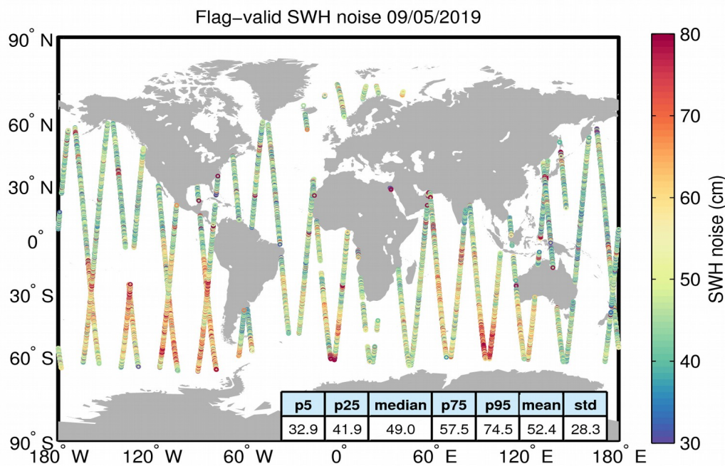
Figure 18. Geographical distribution of flag-valid 20-Hz SWH measurement noise over oceans and lakes for 09/05/2019. The statistical values shown in the figure refer to the SWH noise and are calculated over all measurements shown in the figure.
