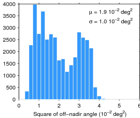
Figure 39. Histogram of flag-valid mispointing over oceans and lakes for 09/05/2019. The mean ( \mu ) and standard deviation ( \sigma ) are also shown. Note that values larger than 6 \cdot 10^{-2} \text{ deg}^2 are excluded from the histogram for the sake of readability but not from the computation of \mu and \sigma .
