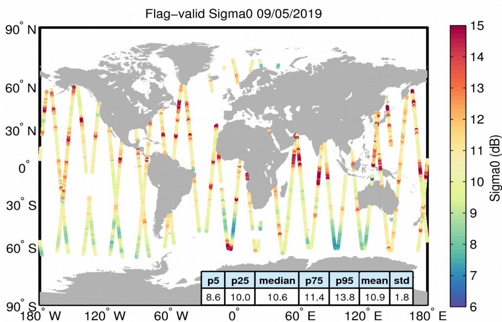
Figure 23. Geographical distribution of flag-valid sigma0 data over oceans and lakes for 09/05/2019. The statistical values shown in the table refer to the sigma0 in dB and are calculated over all measurements shown in the figure.
