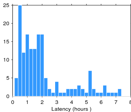
Figure 2. Histogram of the data latency for 09/05/2019. The y-axis denotes the number of files that are made available with a delay of x-hours with respect to the mean time of the records stored in the file.
