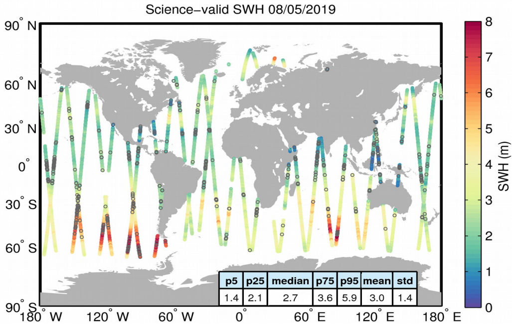
Figure 19. Geographical distribution of science-valid SWH data over oceans and lakes for 08/05/2019. The statistical values shown in the table refer to the SWH in m and are calculated over all measurements shown in the figure. Gray circles denote records that have been rejected based on the editing criteria described in Table 3.
