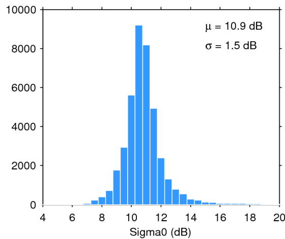
Figure 28. Histogram of science-valid sigma0 over oceans and lakes for 08/05/2019. The mean ( \mu ) and standard deviation ( \sigma ) are also shown. Note that values outside [4 20] dB are excluded from the histogram for the sake of readability but not from the computation of \mu and \sigma .
