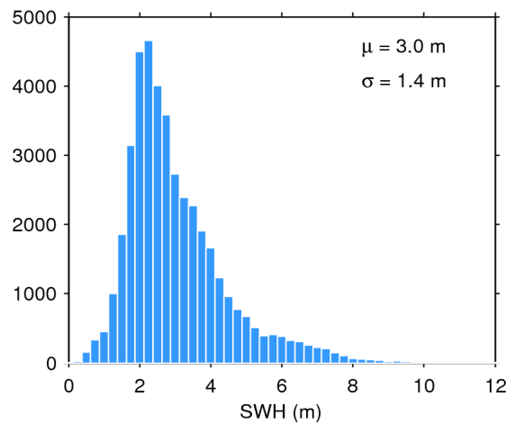
Figure 17. Histogram of flag-valid SWH over oceans and lakes for 08/05/2019. The mean ( \mu ) and standard deviation ( \sigma ) are also shown. Note that values larger than 12 m are excluded from the histogram for the sake of readability but not from the computation of \mu and \sigma .
