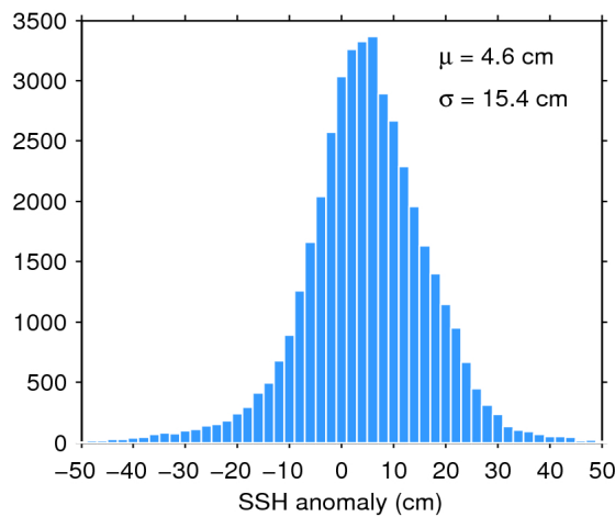
Figure 7. Histogram of flag-valid SSH anomaly over oceans and lakes for 08/05/2019. The mean ( \mu ) and standard deviation ( \sigma ) are also shown. Note that values outside [-50\ 50] cm are excluded from the histogram for the sake of readability but not from the computation of \mu and \sigma .
