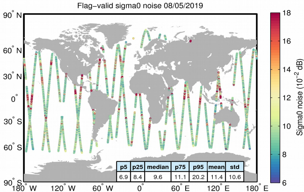
Figure 26. Geographical distribution of flag-valid 20-Hz sigma0 measurement noise over oceans and lakes for 08/05/2019. The statistical values shown in the table refer to the sigma0 noise and are calculated over all measurements shown in the figure.
