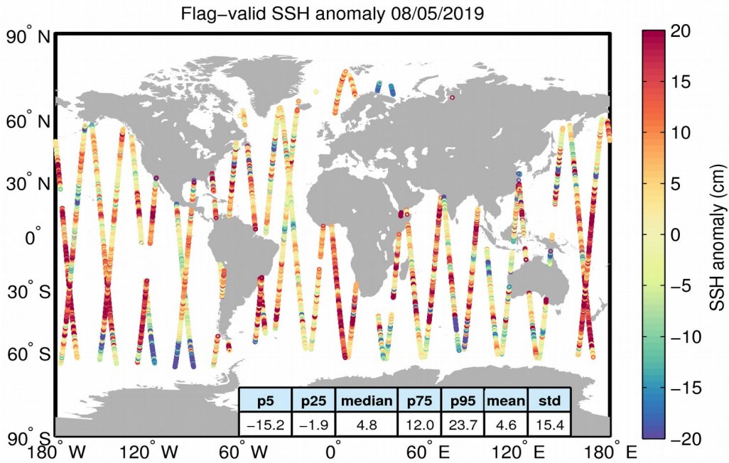
Figure 5. Geographical distribution of flag-valid 1-Hz SSH anomaly data over oceans and lakes for 08/05/2019. The statistical values shown in the table refer to the SSH anomaly in cm and are calculated over all measurements shown in the figure.
