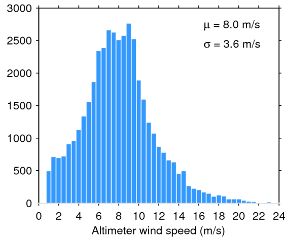
Figure 33. Histogram of flag-valid wind over oceans and lakes for 08/05/2019. The mean ( \mu ) and standard deviation ( \sigma ) are also shown. Note that values larger than 24 m/s are excluded from the histogram for the sake of readability but not from the computation of \mu and \sigma .
