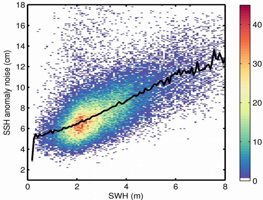
Figure 9. 2D histogram showing flag-valid SSH anomaly noise as a function of SWH for 08/05/2019. The black line denotes the median SSH anomaly noise as a function of SWH.
