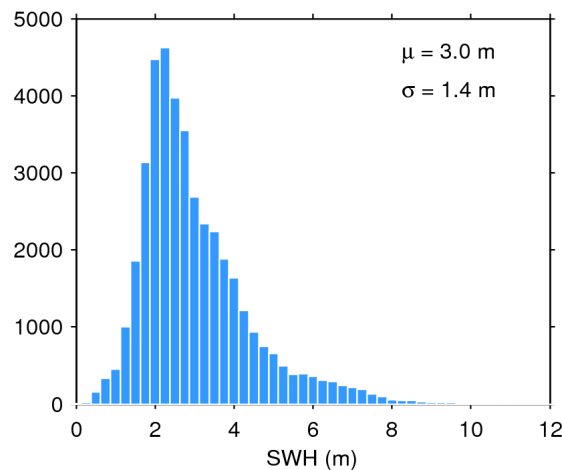
Figure 20. Histogram of science-valid SWH over oceans and lakes for 08/05/2019. The mean ( \mu ) and standard deviation ( \sigma ) are also shown. Note that values larger than 12 m are excluded from the histogram for the sake of readability but not from the computation of \mu and \sigma .
