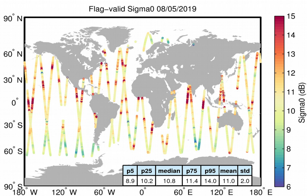
Figure 23. Geographical distribution of flag-valid sigma0 data over oceans and lakes for 08/05/2019. The statistical values shown in the table refer to the sigma0 in dB and are calculated over all measurements shown in the figure.
