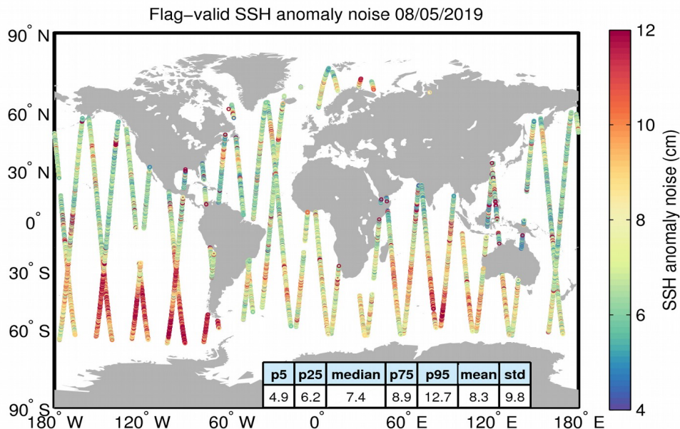
Figure 8. Geographical distribution of flag-valid 20-Hz SSH anomaly measurement noise over oceans and lakes for 08/05/2019. The statistical values shown in the table refer to the SSH anomaly noise and are calculated over all measurements shown in the figure.
