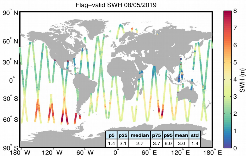
Figure 15. Geographical distribution of flag-valid SWH data over oceans and lakes for 08/05/2019. The statistical values shown in the table refer to the SWH in m and are calculated over all measurements shown in the figure.
