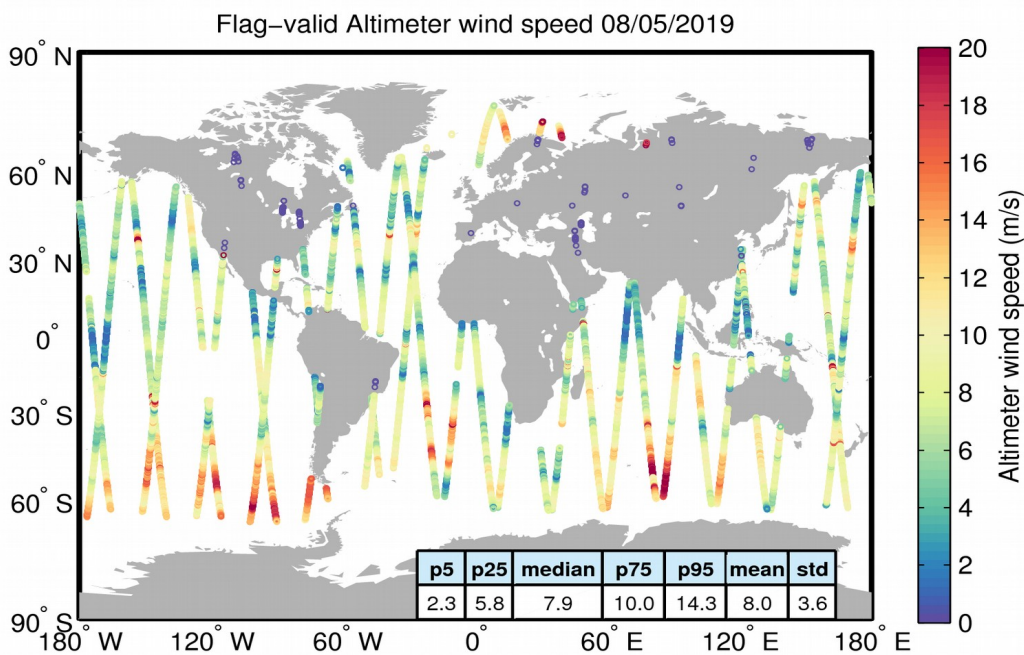
Figure 31. Geographical distribution of flag-valid wind data over oceans and lakes for 08/05/2019. The statistical values shown in the table refer to the wind in m/s and are calculated over all measurements shown in the figure.
