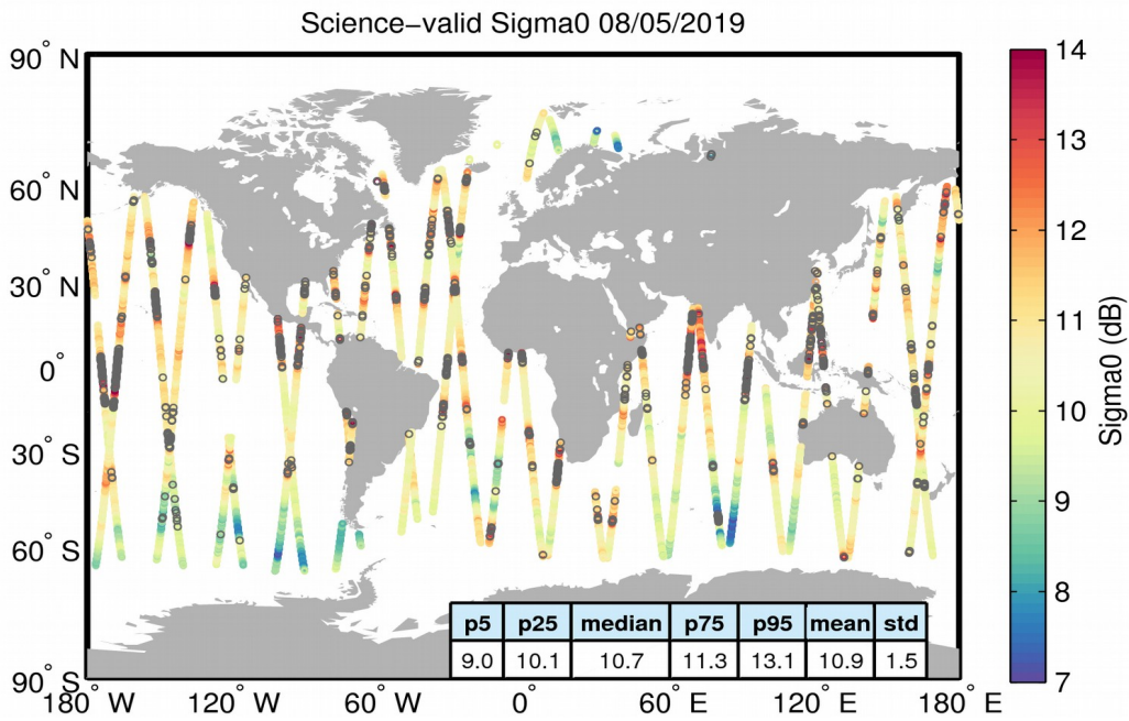
Figure 27. Geographical distribution of science-valid sigma0 data over oceans and lakes for 08/05/2019. The statistical values shown in the table refer to the sigma0 in dB and are calculated over all measurements shown in the figure. Gray circles denote records that have been rejected based on the editing criteria described in Table 4.
