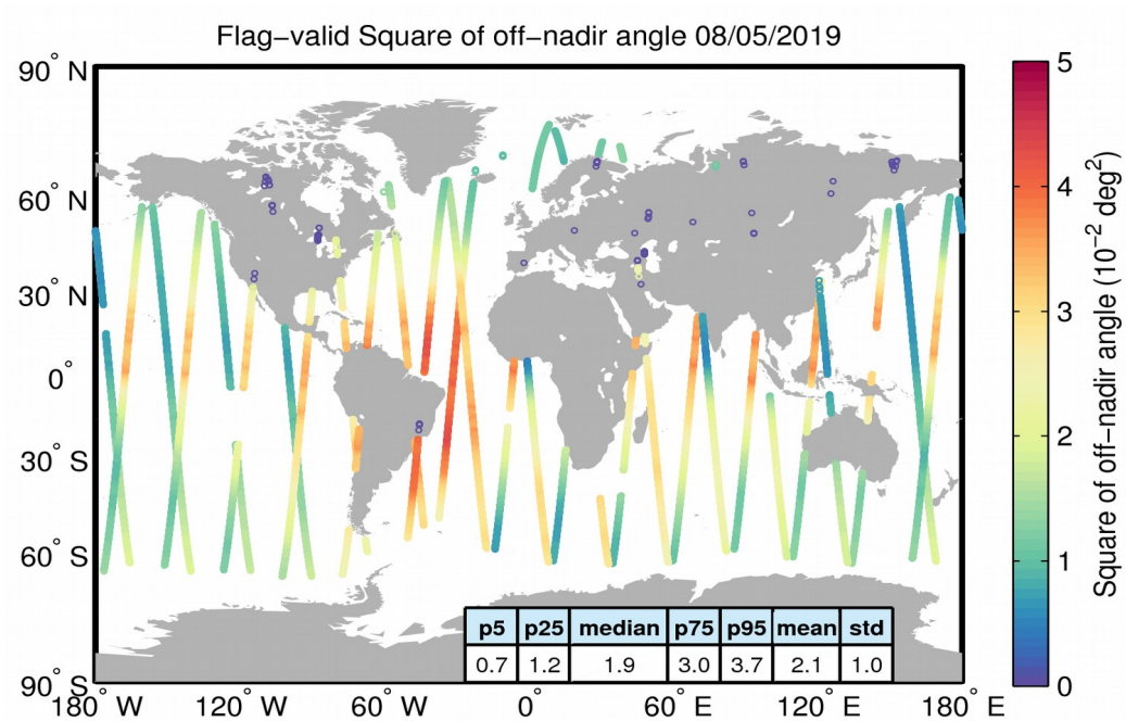
Figure 37. Geographical distribution of flag-valid mispointing data over oceans and lakes for 08/05/2019. The statistical values shown in the table refer to the mispointing in 10^{-2} \text{ deg}^2 and are calculated over all measurements shown in the figure.
