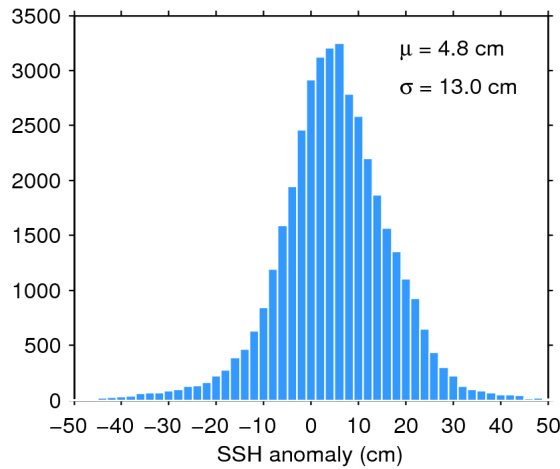
Figure 11. Histogram of science-valid SSH anomaly over oceans and lakes for 08/05/2019. The mean ( \mu ) and standard deviation ( \sigma ) are also shown. Note that values outside [-50 50] cm are excluded from the histogram for the sake of readability but not from the computation of \mu and \sigma .
