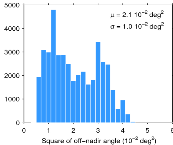
Figure 39. Histogram of flag-valid mispointing over oceans and lakes for 08/05/2019. The mean ( \mu ) and standard deviation ( \sigma ) are also shown. Note that values larger than 6 \cdot 10^{-2} \text{ deg}^2 are excluded from the histogram for the sake of readability but not from the computation of \mu and \sigma .
