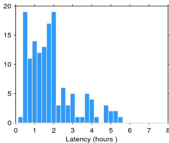
Figure 2. Histogram of the data latency for 08/05/2019. The y-axis denotes the number of files that are made available with a delay of x-hours with respect to the mean time of the records stored in the file.
