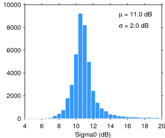
Figure 25. Histogram of flag-valid sigma0 over oceans and lakes for 08/05/2019. The mean ( \mu ) and standard deviation ( \sigma ) are also shown. Note that values outside [4 20] dB are excluded from the histogram for the sake of readability but not from the computation of \mu and \sigma .
