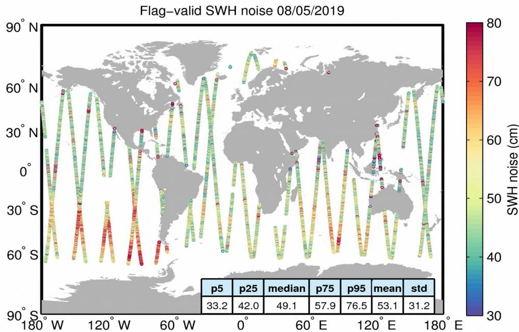
Figure 18. Geographical distribution of flag-valid 20-Hz SWH measurement noise over oceans and lakes for 08/05/2019. The statistical values shown in the table refer to the SWH noise and are calculated over all measurements shown in the figure.
