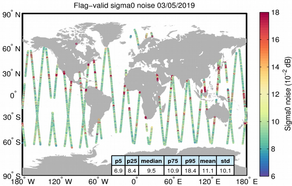
Figure 26. Geographical distribution of flag-valid 20-Hz sigma0 measurement noise over oceans and lakes for 03/05/2019. The statistical values shown in the table refer to the sigma0 noise and are calculated over all measurements shown in the figure.
