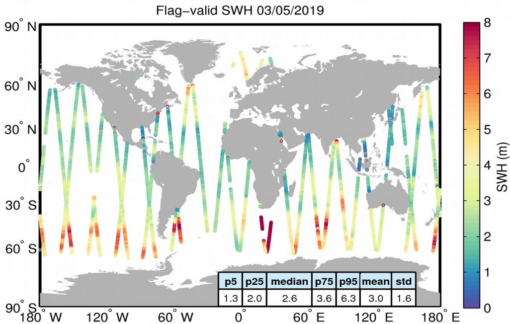
Figure 15. Geographical distribution of flag-valid SWH data over oceans and lakes for 03/05/2019. The statistical values shown in the table refer to the SWH in m and are calculated over all measurements shown in the figure.
