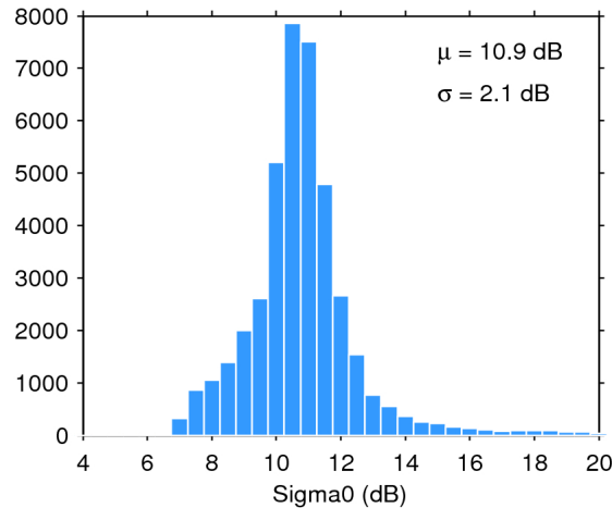
Figure 25. Histogram of flag-valid sigma0 over oceans and lakes for 03/05/2019. The mean ( \mu ) and standard deviation ( \sigma ) are also shown. Note that values outside [4 20] dB are excluded from the histogram for the sake of readability but not from the computation of \mu and \sigma .
