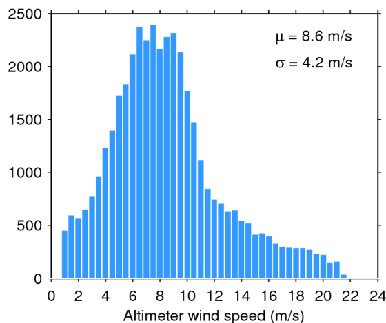
Figure 35. Histogram of science-valid wind over oceans and lakes for 03/05/2019. The mean ( \mu ) and standard deviation ( \sigma ) are also shown. Note that values larger than 24 m/s are excluded from the histogram for the sake of readability but not from the computation of \mu and \sigma .
