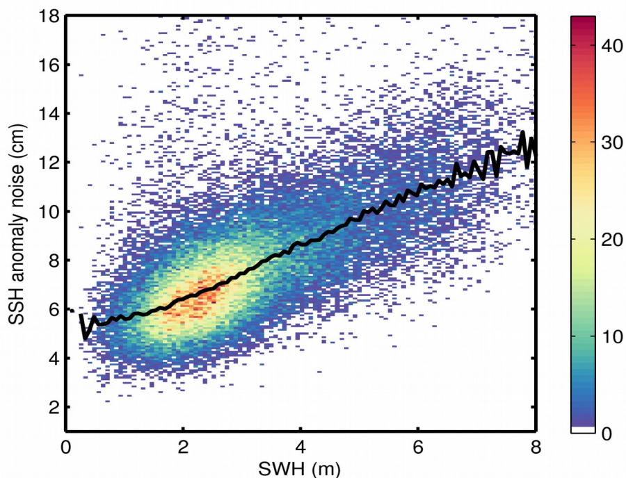
Figure 9. 2D histogram showing flag-valid SSH anomaly noise as a function of SWH for 03/05/2019. The black line denotes the median SSH anomaly noise as a function of SWH.
