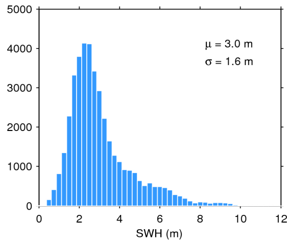
Figure 17. Histogram of flag-valid SWH over oceans and lakes for 03/05/2019. The mean ( \mu ) and standard deviation ( \sigma ) are also shown. Note that values larger than 12 m are excluded from the histogram for the sake of readability but not from the computation of \mu and \sigma .
