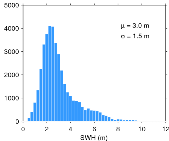
Figure 20. Histogram of science-valid SWH over oceans and lakes for 03/05/2019. The mean ( \mu ) and standard deviation ( \sigma ) are also shown. Note that values larger than 12 m are excluded from the histogram for the sake of readability but not from the computation of \mu and \sigma .
