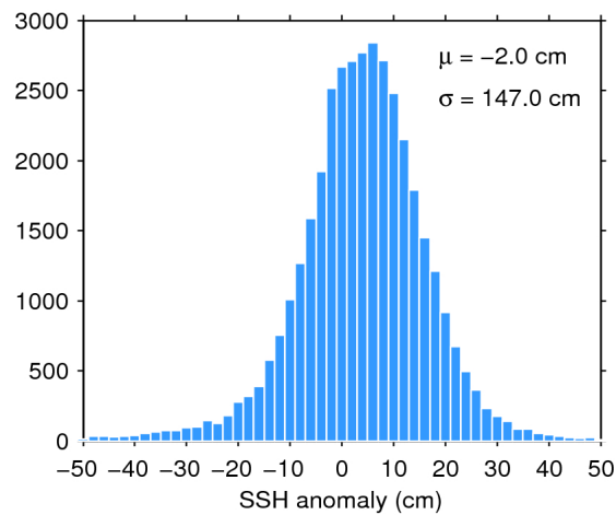
Figure 7. Histogram of flag-valid SSH anomaly over oceans and lakes for 03/05/2019. The mean ( \mu ) and standard deviation ( \sigma ) are also shown. Note that values outside [-50 50] cm are excluded from the histogram for the sake of readability but not from the computation of \mu and \sigma .
