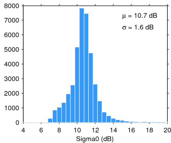
Figure 28. Histogram of science-valid sigma0 over oceans and lakes for 03/05/2019. The mean ( \mu ) and standard deviation ( \sigma ) are also shown. Note that values outside [4 20] dB are excluded from the histogram for the sake of readability but not from the computation of \mu and \sigma .
