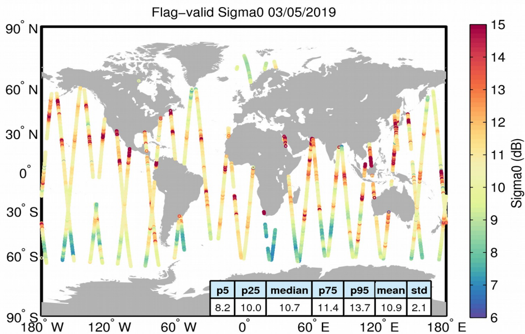
Figure 23. Geographical distribution of flag-valid sigma0 data over oceans and lakes for 03/05/2019. The statistical values shown in the table refer to the sigma0 in dB and are calculated over all measurements shown in the figure.
