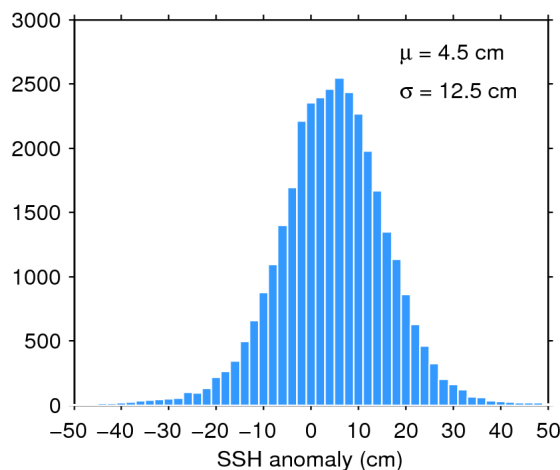
Figure 11. Histogram of science-valid SSH anomaly over oceans and lakes for 03/05/2019. The mean ( \mu ) and standard deviation ( \sigma ) are also shown. Note that values outside [-50 50] cm are excluded from the histogram for the sake of readability but not from the computation of \mu and \sigma .
