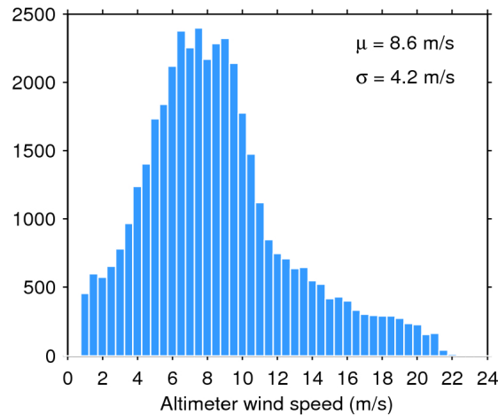
Figure 33. Histogram of flag-valid wind over oceans and lakes for 03/05/2019. The mean ( \mu ) and standard deviation ( \sigma ) are also shown. Note that values larger than 24 m/s are excluded from the histogram for the sake of readability but not from the computation of \mu and \sigma .
