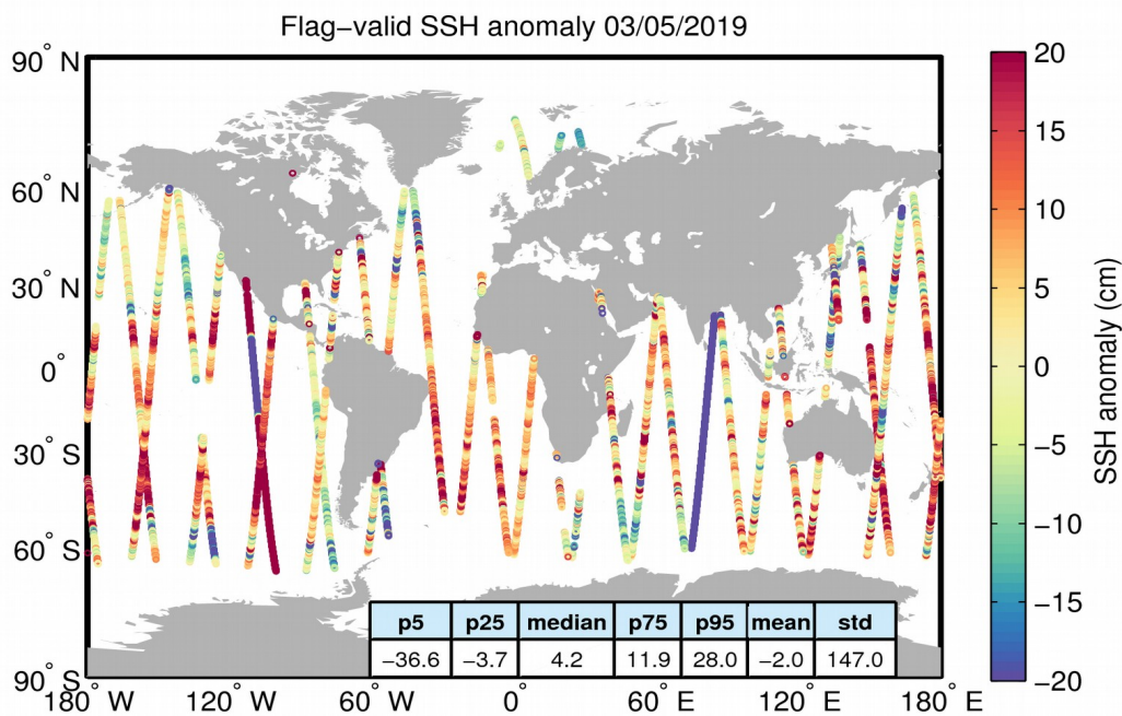
Figure 5. Geographical distribution of flag-valid 1-Hz SSH anomaly data over oceans and lakes for 03/05/2019. The statistical values shown in the table refer to the SSH anomaly in cm and are calculated over all measurements shown in the figure.
