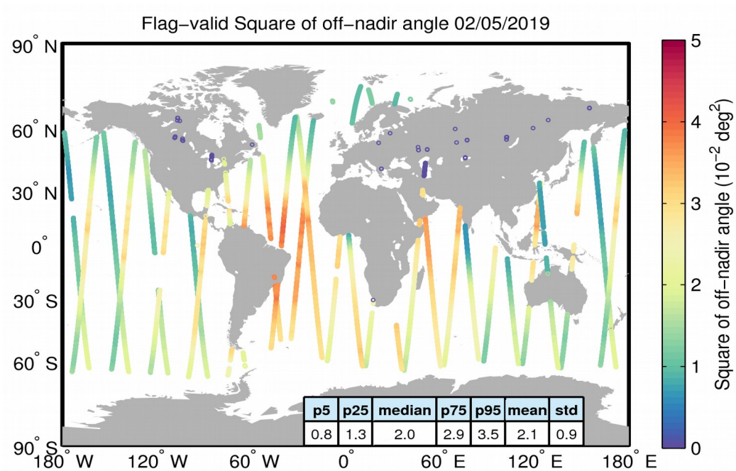
Figure 37. Geographical distribution of flag-valid mispointing data over oceans and lakes for 02/05/2019. The statistical values shown in the table refer to the mispointing in 10^{-2} \text{ deg}^2 and are calculated over all measurements shown in the figure.
