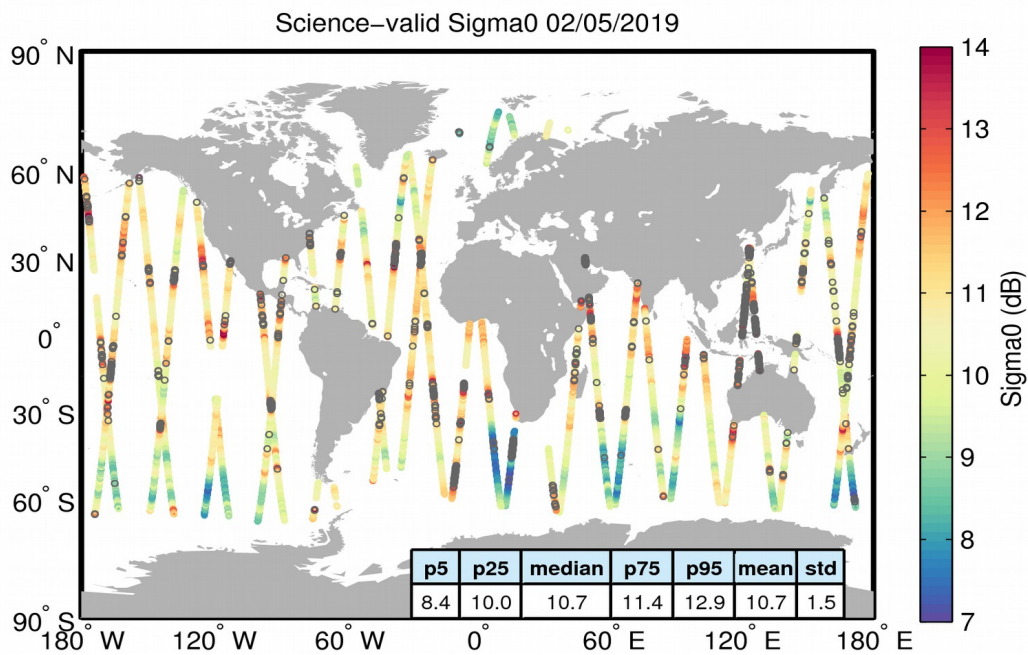
Figure 27. Geographical distribution of science-valid sigma0 data over oceans and lakes for 02/05/2019. The statistical values shown in the table refer to the sigma0 in dB and are calculated over all measurements shown in the figure. Gray circles denote records that have been rejected based on the editing criteria described in Table 4.
