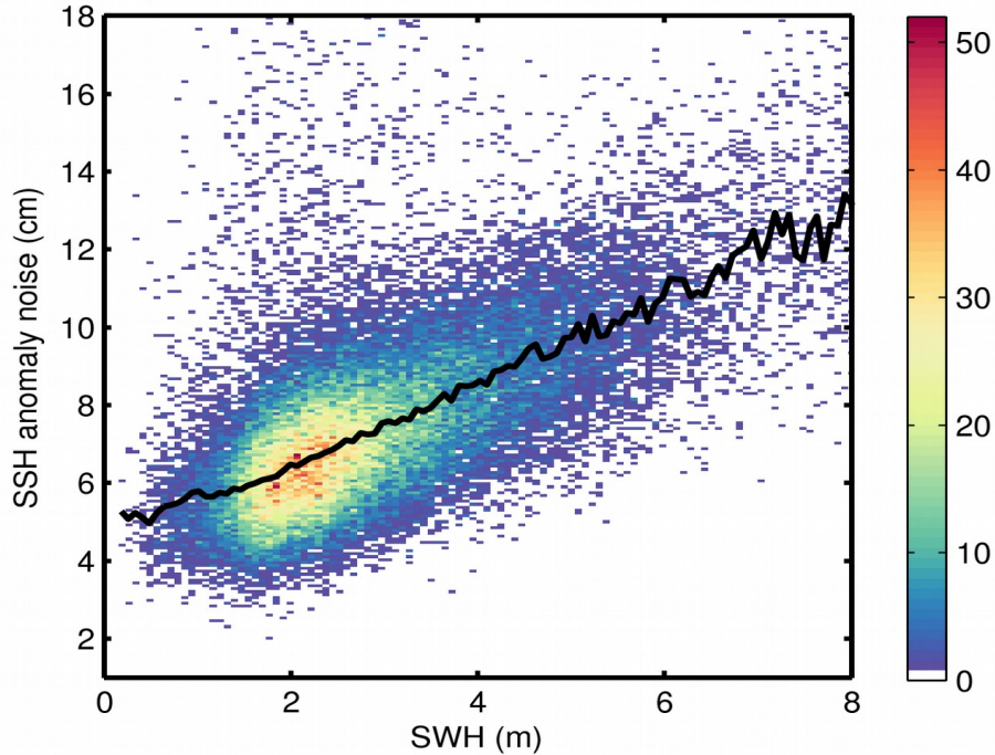
Figure 9. 2D histogram showing flag-valid SSH anomaly noise as a function of SWH for 02/05/2019. The black line denotes the median SSH anomaly noise as a function of SWH.
