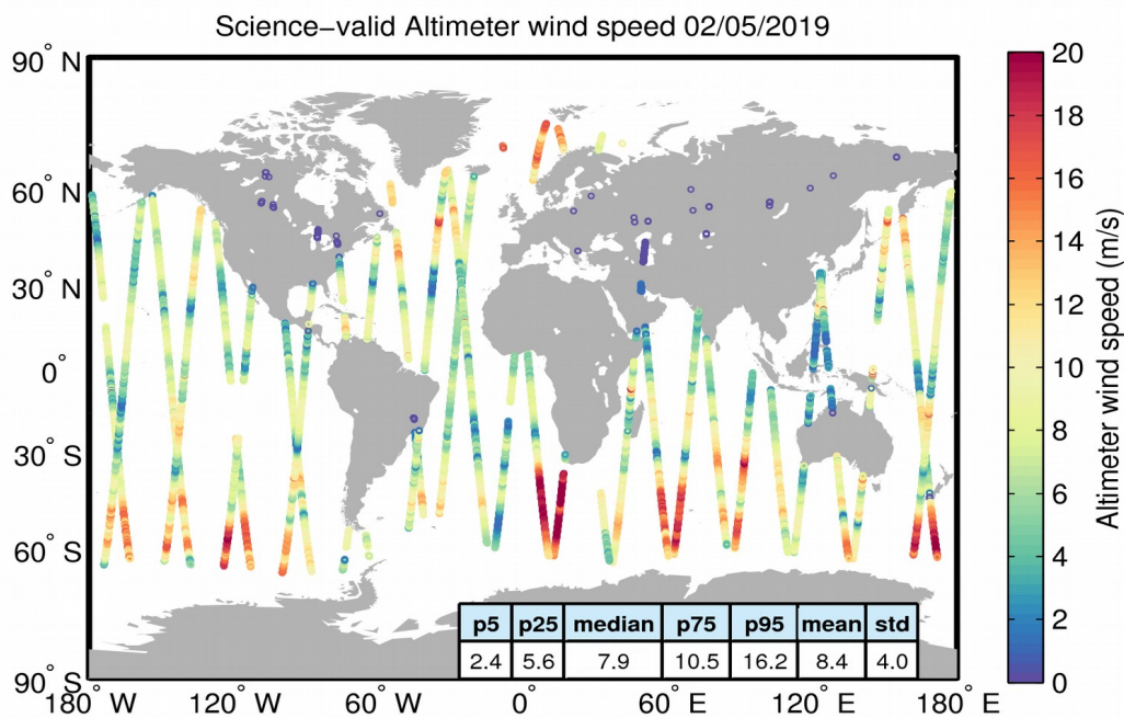
Figure 34. Geographical distribution of science-valid wind data over oceans and lakes for 02/05/2019. The statistical values shown in the table refer to the wind in m/s and are calculated over all measurements shown in the figure. Gray circles denote records that have been rejected based on the editing criteria described in Table 5.
