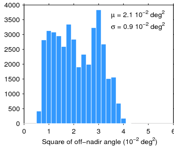
Figure 39. Histogram of flag-valid mispointing over oceans and lakes for 02/05/2019. The mean ( \mu ) and standard deviation ( \sigma ) are also shown. Note that values larger than 6 \cdot 10^{-2} \text{ deg}^2 are excluded from the histogram for the sake of readability but not from the computation of \mu and \sigma .
