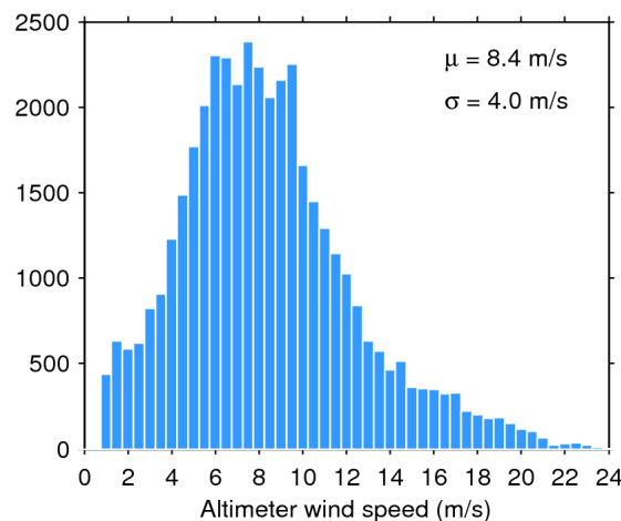
Figure 35. Histogram of science-valid wind over oceans and lakes for 02/05/2019. The mean ( \mu ) and standard deviation ( \sigma ) are also shown. Note that values larger than 24 m/s are excluded from the histogram for the sake of readability but not from the computation of \mu and \sigma .
