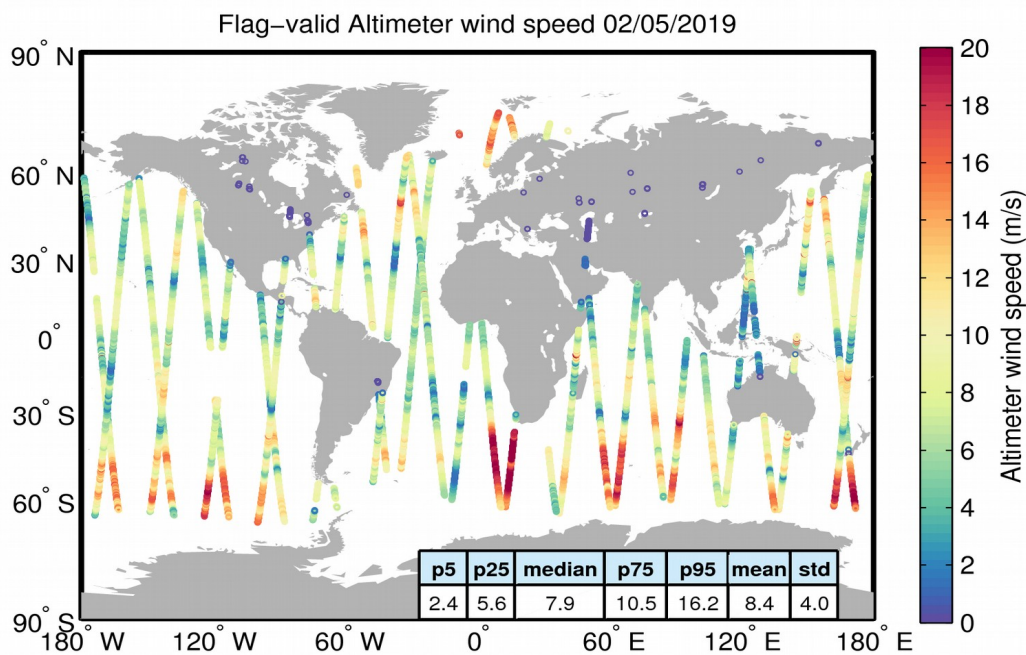
Figure 31. Geographical distribution of flag-valid wind data over oceans and lakes for 02/05/2019. The statistical values shown in the table refer to the wind in m/s and are calculated over all measurements shown in the figure.
