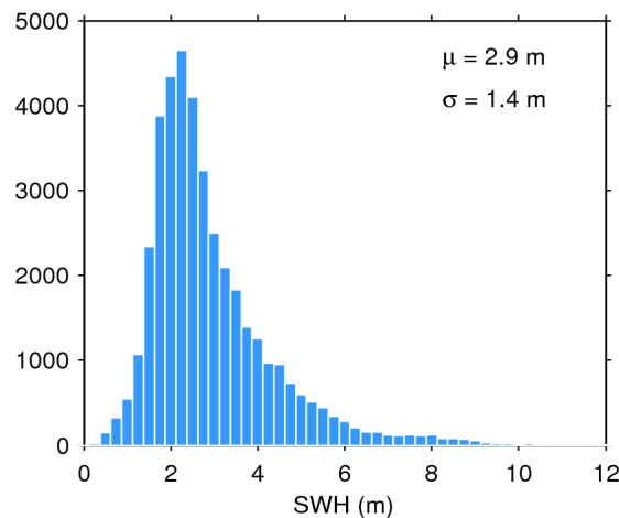
Figure 20. Histogram of science-valid SWH over oceans and lakes for 02/05/2019. The mean ( \mu ) and standard deviation ( \sigma ) are also shown. Note that values larger than 12 m are excluded from the histogram for the sake of readability but not from the computation of \mu and \sigma .
