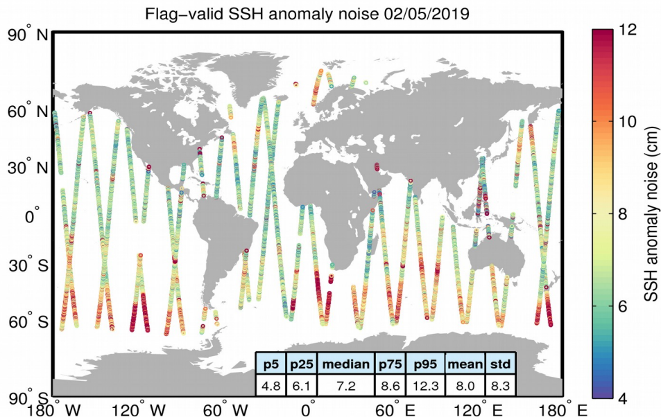
Figure 8. Geographical distribution of flag-valid 20-Hz SSH anomaly measurement noise over oceans and lakes for 02/05/2019. The statistical values shown in the table refer to the SSH anomaly noise and are calculated over all measurements shown in the figure.
