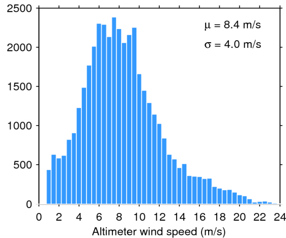
Figure 33. Histogram of flag-valid wind over oceans and lakes for 02/05/2019. The mean ( \mu ) and standard deviation ( \sigma ) are also shown. Note that values larger than 24 m/s are excluded from the histogram for the sake of readability but not from the computation of \mu and \sigma .
