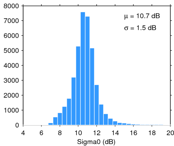
Figure 28. Histogram of science-valid sigma0 over oceans and lakes for 02/05/2019. The mean ( \mu ) and standard deviation ( \sigma ) are also shown. Note that values outside [4 20] dB are excluded from the histogram for the sake of readability but not from the computation of \mu and \sigma .
