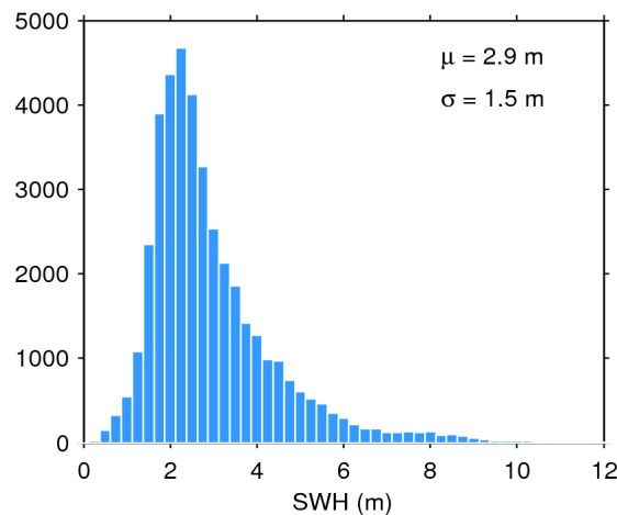
Figure 17. Histogram of flag-valid SWH over oceans and lakes for 02/05/2019. The mean ( \mu ) and standard deviation ( \sigma ) are also shown. Note that values larger than 12 m are excluded from the histogram for the sake of readability but not from the computation of \mu and \sigma .
