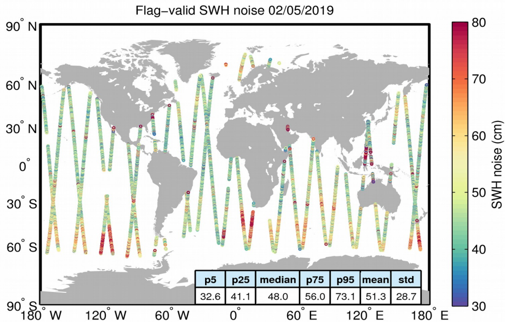
Figure 18. Geographical distribution of flag-valid 20-Hz SWH measurement noise over oceans and lakes for 02/05/2019. The statistical values shown in the table refer to the SWH noise and are calculated over all measurements shown in the figure.
