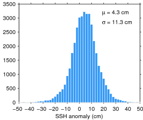
Figure 11. Histogram of science-valid SSH anomaly over oceans and lakes for 02/05/2019. The mean ( \mu ) and standard deviation ( \sigma ) are also shown. Note that values outside [-50 50] cm are excluded from the histogram for the sake of readability but not from the computation of \mu and \sigma .
