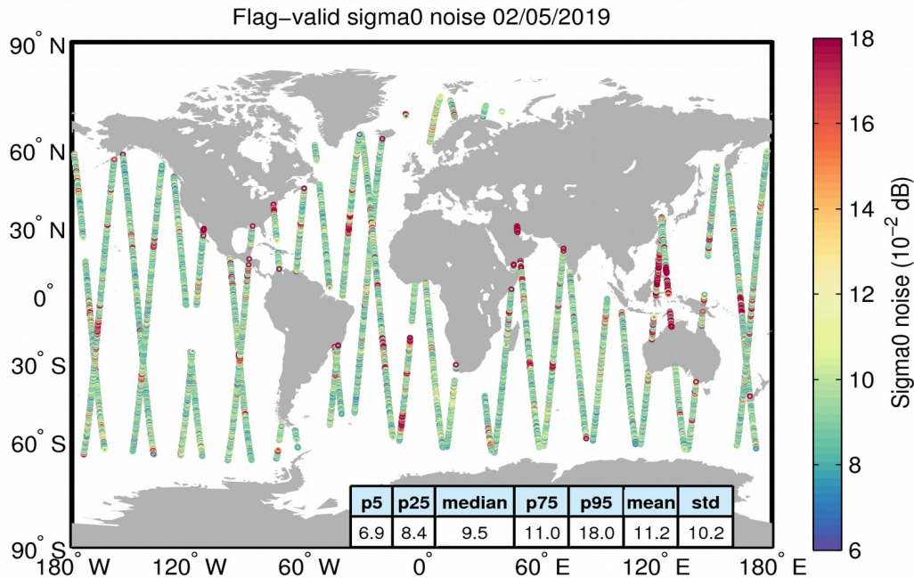
Figure 26. Geographical distribution of flag-valid 20-Hz sigma0 measurement noise over oceans and lakes for 02/05/2019. The statistical values shown in the table refer to the sigma0 noise and are calculated over all measurements shown in the figure.
