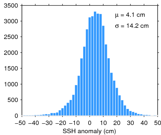
Figure 7. Histogram of flag-valid SSH anomaly over oceans and lakes for 02/05/2019. The mean ( \mu ) and standard deviation ( \sigma ) are also shown. Note that values outside [-50\ 50] cm are excluded from the histogram for the sake of readability but not from the computation of \mu and \sigma .
