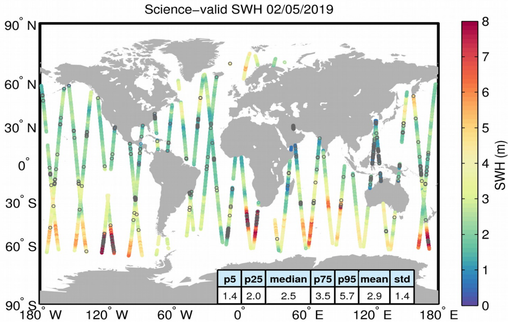
Figure 19. Geographical distribution of science-valid SWH data over oceans and lakes for 02/05/2019. The statistical values shown in the table refer to the SWH in m and are calculated over all measurements shown in the figure. Gray circles denote records that have been rejected based on the editing criteria described in Table 3.
