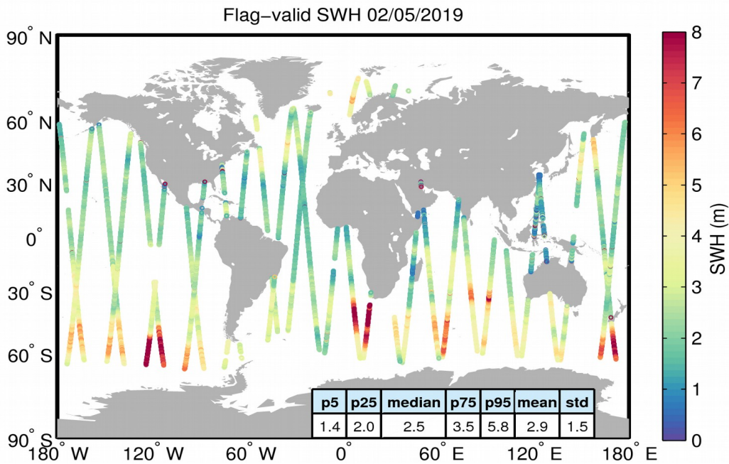
Figure 15. Geographical distribution of flag-valid SWH data over oceans and lakes for 02/05/2019. The statistical values shown in the table refer to the SWH in m and are calculated over all measurements shown in the figure.
