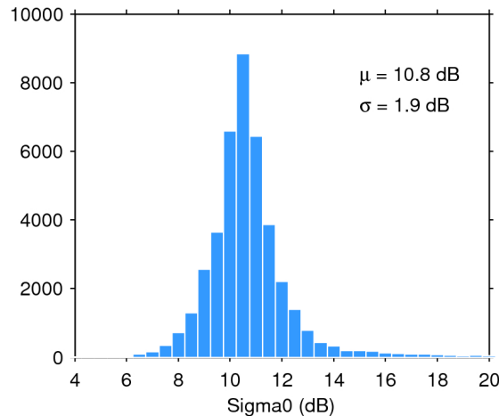
Figure 25. Histogram of flag-valid sigma0 over oceans and lakes for 01/05/2019. The mean ( \mu ) and standard deviation ( \sigma ) are also shown. Note that values outside [4 20] dB are excluded from the histogram for the sake of readability but not from the computation of \mu and \sigma .
