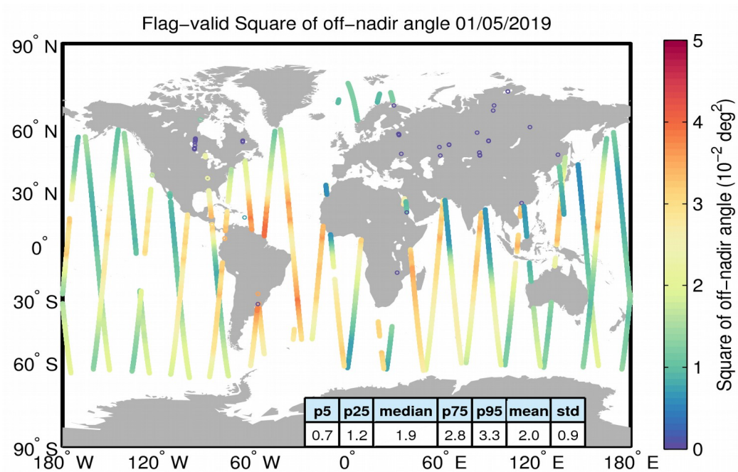
Figure 37. Geographical distribution of flag-valid mispointing data over oceans and lakes for 01/05/2019. The statistical values shown in the table refer to the mispointing in 10^{-2} \text{ deg}^2 and are calculated over all measurements shown in the figure.
