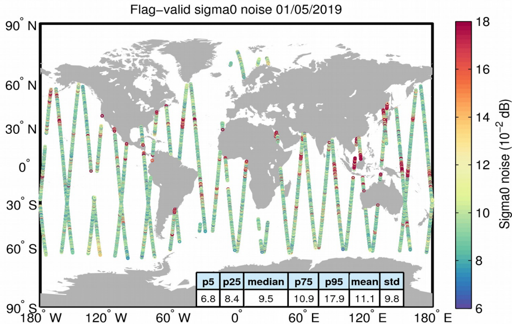
Figure 26. Geographical distribution of flag-valid 20-Hz sigma0 measurement noise over oceans and lakes for 01/05/2019. The statistical values shown in the table refer to the sigma0 noise and are calculated over all measurements shown in the figure.
