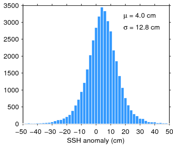
Figure 11. Histogram of science-valid SSH anomaly over oceans and lakes for 01/05/2019. The mean ( \mu ) and standard deviation ( \sigma ) are also shown. Note that values outside [-50 50] cm are excluded from the histogram for the sake of readability but not from the computation of \mu and \sigma .
