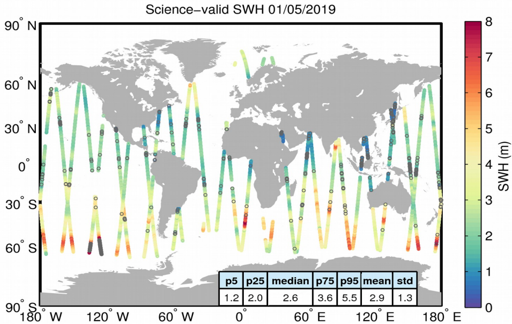
Figure 19. Geographical distribution of science-valid SWH data over oceans and lakes for 01/05/2019. The statistical values shown in the table refer to the SWH in m and are calculated over all measurements shown in the figure. Gray circles denote records that have been rejected based on the editing criteria described in Table 3.
