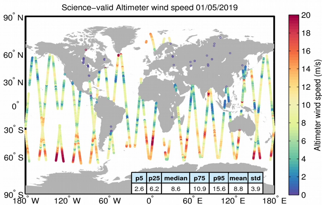
Figure 34. Geographical distribution of science-valid wind data over oceans and lakes for 01/05/2019. The statistical values shown in the table refer to the wind in m/s and are calculated over all measurements shown in the figure. Gray circles denote records that have been rejected based on the editing criteria described in Table 5.
