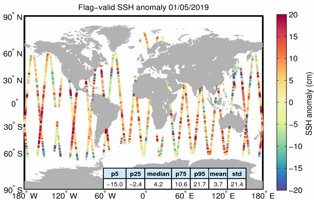
Figure 5. Geographical distribution of flag-valid 1-Hz SSH anomaly data over oceans and lakes for 01/05/2019. The statistical values shown in the table refer to the SSH anomaly in cm and are calculated over all measurements shown in the figure.
