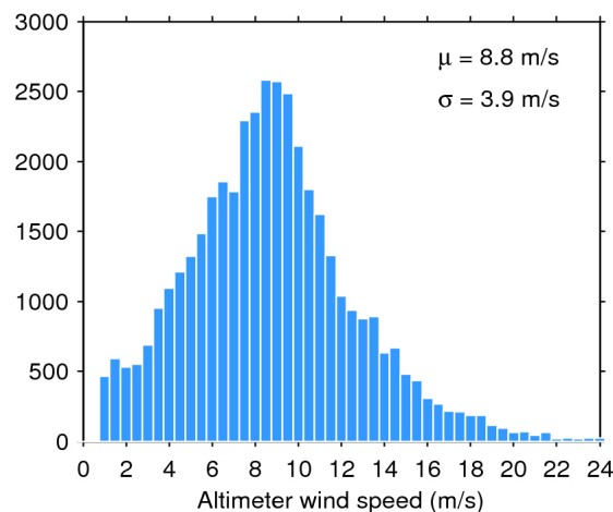
Figure 35. Histogram of science-valid wind over oceans and lakes for 01/05/2019. The mean ( \mu ) and standard deviation ( \sigma ) are also shown. Note that values larger than 24 m/s are excluded from the histogram for the sake of readability but not from the computation of \mu and \sigma .
