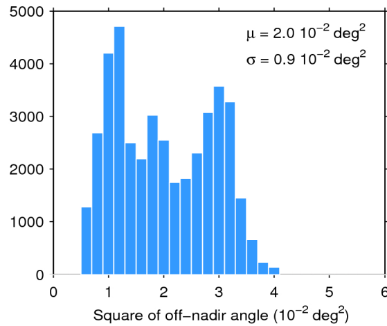
Figure 39. Histogram of flag-valid mispointing over oceans and lakes for 01/05/2019. The mean ( \mu ) and standard deviation ( \sigma ) are also shown. Note that values larger than 6 \cdot 10^{-2} \text{ deg}^2 are excluded from the histogram for the sake of readability but not from the computation of \mu and \sigma .
