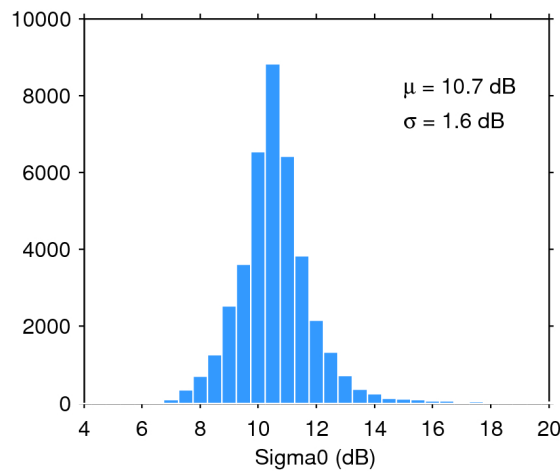
Figure 28. Histogram of science-valid sigma0 over oceans and lakes for 01/05/2019. The mean ( \mu ) and standard deviation ( \sigma ) are also shown. Note that values outside [4 20] dB are excluded from the histogram for the sake of readability but not from the computation of \mu and \sigma .
