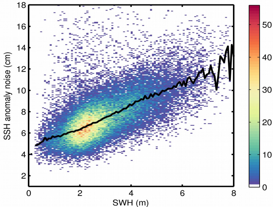
Figure 9. 2D histogram showing flag-valid SSH anomaly noise as a function of SWH for 01/05/2019. The black line denotes the median SSH anomaly noise as a function of SWH.
