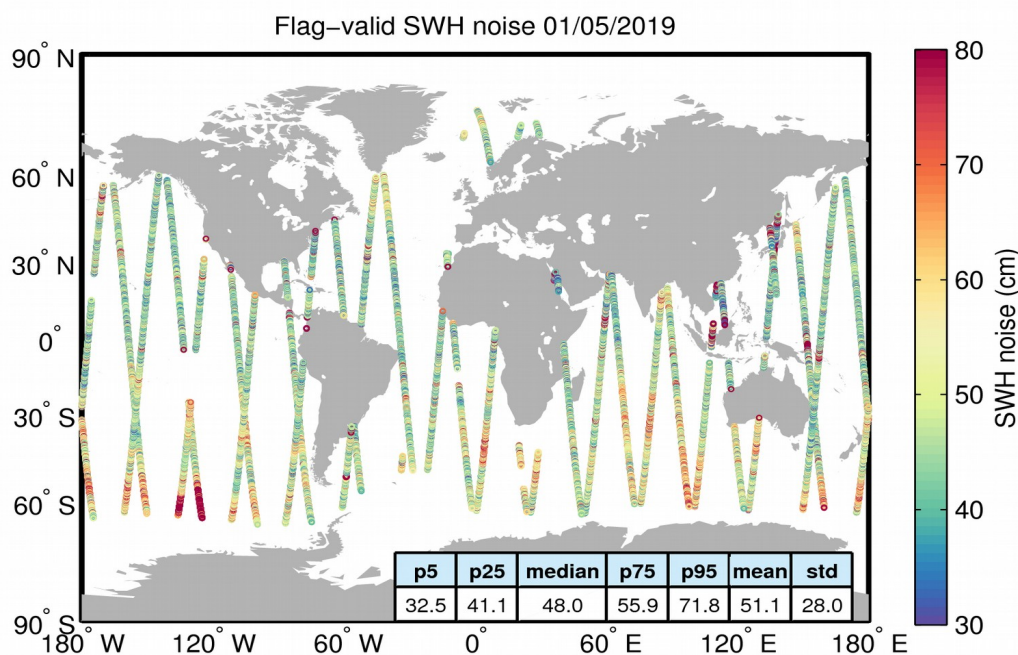
Figure 18. Geographical distribution of flag-valid 20-Hz SWH measurement noise over oceans and lakes for 01/05/2019. The statistical values shown in the table refer to the SWH noise and are calculated over all measurements shown in the figure.
