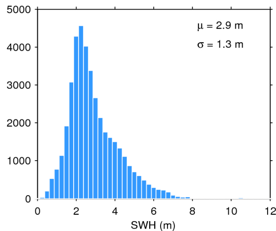
Figure 20. Histogram of science-valid SWH over oceans and lakes for 01/05/2019. The mean ( \mu ) and standard deviation ( \sigma ) are also shown. Note that values larger than 12 m are excluded from the histogram for the sake of readability but not from the computation of \mu and \sigma .
