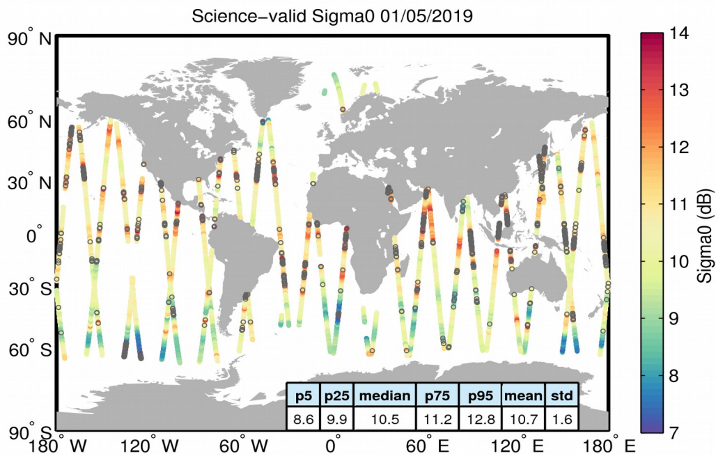
Figure 27. Geographical distribution of science-valid sigma0 data over oceans and lakes for 01/05/2019. The statistical values shown in the table refer to the sigma0 in dB and are calculated over all measurements shown in the figure. Gray circles denote records that have been rejected based on the editing criteria described in Table 4.
