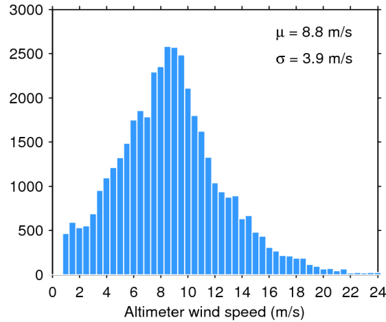
Figure 33. Histogram of flag-valid wind over oceans and lakes for 01/05/2019. The mean ( \mu ) and standard deviation ( \sigma ) are also shown. Note that values larger than 24 m/s are excluded from the histogram for the sake of readability but not from the computation of \mu and \sigma .
