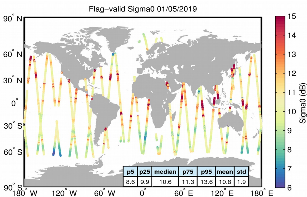
Figure 23. Geographical distribution of flag-valid sigma0 data over oceans and lakes for 01/05/2019. The statistical values shown in the table refer to the sigma0 in dB and are calculated over all measurements shown in the figure.
