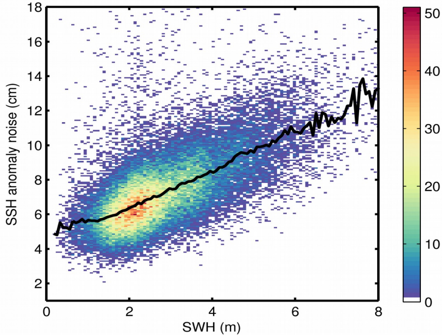
Figure 9. 2D histogram showing flag-valid SSH anomaly noise as a function of SWH for 30/04/2019. The black line denotes the median SSH anomaly noise as a function of SWH.
