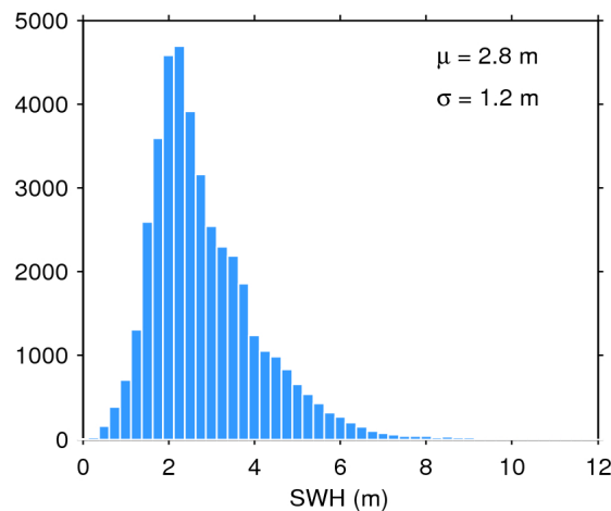
Figure 20. Histogram of science-valid SWH over oceans and lakes for 30/04/2019. The mean ( \mu ) and standard deviation ( \sigma ) are also shown. Note that values larger than 12 m are excluded from the histogram for the sake of readability but not from the computation of \mu and \sigma .
