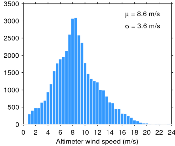
Figure 33. Histogram of flag-valid wind over oceans and lakes for 30/04/2019. The mean ( \mu ) and standard deviation ( \sigma ) are also shown. Note that values larger than 24 m/s are excluded from the histogram for the sake of readability but not from the computation of \mu and \sigma .
