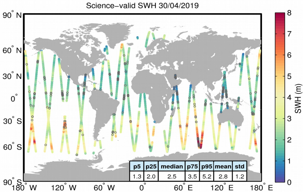
Figure 19. Geographical distribution of science-valid SWH data over oceans and lakes for 30/04/2019. The statistical values shown in the table refer to the SWH in m and are calculated over all measurements shown in the figure. Gray circles denote records that have been rejected based on the editing criteria described in Table 3.
