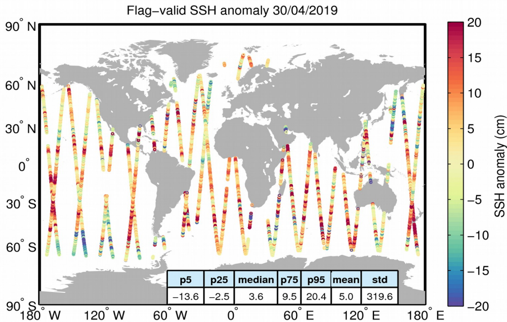
Figure 5. Geographical distribution of flag-valid 1-Hz SSH anomaly data over oceans and lakes for 30/04/2019. The statistical values shown in the table refer to the SSH anomaly in cm and are calculated over all measurements shown in the figure.
