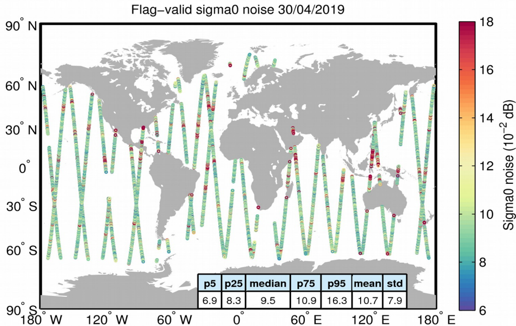
Figure 26. Geographical distribution of flag-valid 20-Hz sigma0 measurement noise over oceans and lakes for 30/04/2019. The statistical values shown in the table refer to the sigma0 noise and are calculated over all measurements shown in the figure.
