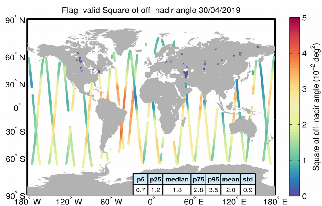
Figure 37. Geographical distribution of flag-valid mispointing data over oceans and lakes for 30/04/2019. The statistical values shown in the table refer to the mispointing in 10^{-2} deg 2 and are calculated over all measurements shown in the figure.
