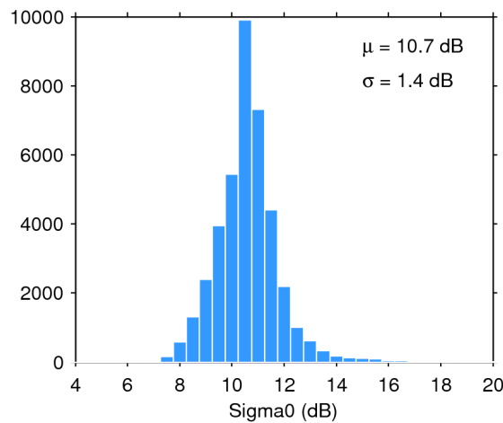
Figure 28. Histogram of science-valid sigma0 over oceans and lakes for 30/04/2019. The mean ( \mu ) and standard deviation ( \sigma ) are also shown. Note that values outside [4 20] dB are excluded from the histogram for the sake of readability but not from the computation of \mu and \sigma .
