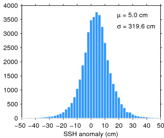
Figure 7. Histogram of flag-valid SSH anomaly over oceans and lakes for 30/04/2019. The mean ( \mu ) and standard deviation ( \sigma ) are also shown. Note that values outside [-50\ 50] cm are excluded from the histogram for the sake of readability but not from the computation of \mu and \sigma .
