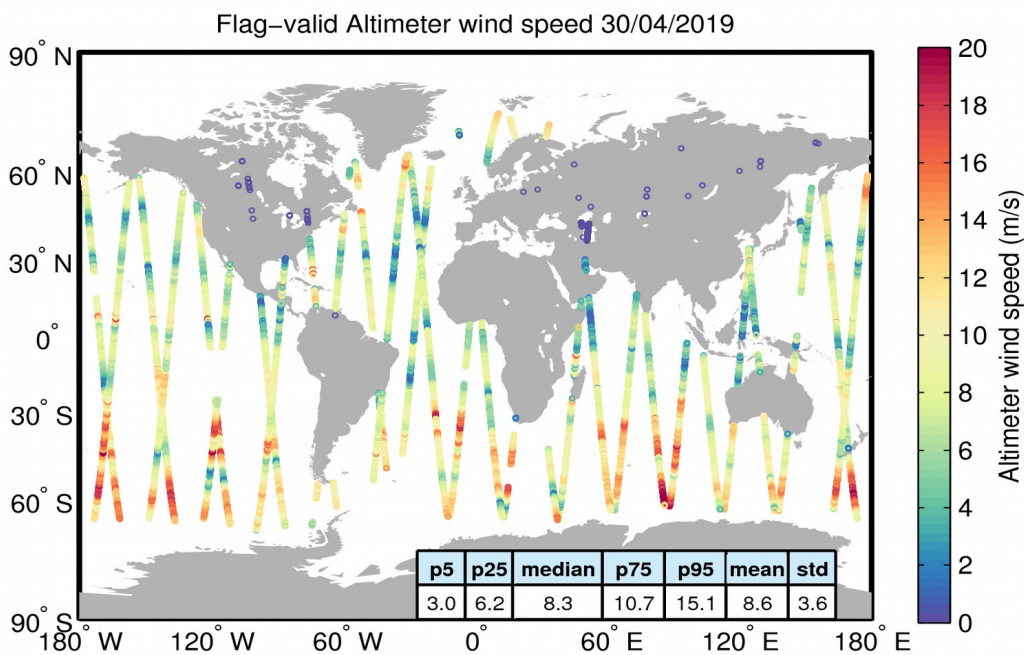
Figure 31. Geographical distribution of flag-valid wind data over oceans and lakes for 30/04/2019. The statistical values shown in the table refer to the wind in m/s and are calculated over all measurements shown in the figure.
