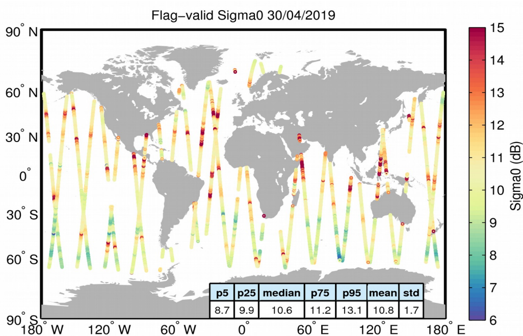
Figure 23. Geographical distribution of flag-valid sigma0 data over oceans and lakes for 30/04/2019. The statistical values shown in the table refer to the sigma0 in dB and are calculated over all measurements shown in the figure.
