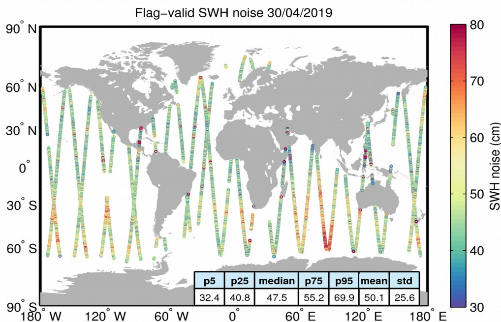
Figure 18. Geographical distribution of flag-valid 20-Hz SWH measurement noise over oceans and lakes for 30/04/2019. The statistical values shown in the figure refer to the SWH noise and are calculated over all measurements shown in the figure.
