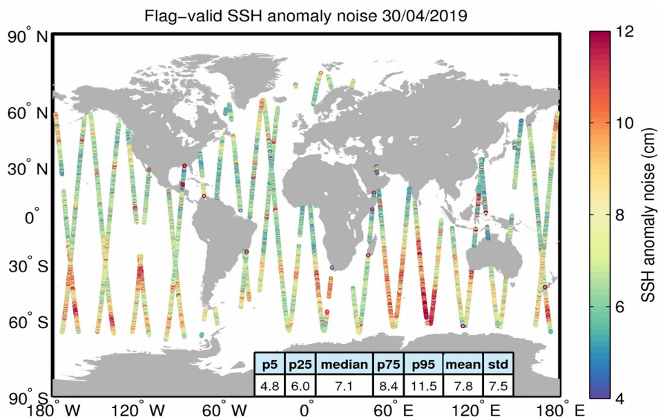
Figure 8. Geographical distribution of flag-valid 20-Hz SSH anomaly measurement noise over oceans and lakes for 30/04/2019. The statistical values shown in the table refer to the SSH anomaly noise and are calculated over all measurements shown in the figure.
