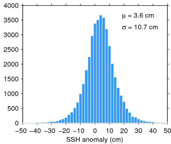
Figure 11. Histogram of science-valid SSH anomaly over oceans and lakes for 30/04/2019. The mean ( \mu ) and standard deviation ( \sigma ) are also shown. Note that values outside [-50 50] cm are excluded from the histogram for the sake of readability but not from the computation of \mu and \sigma .
