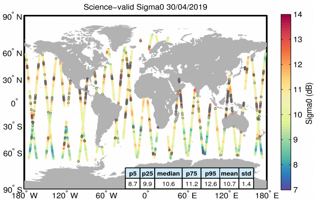
Figure 27. Geographical distribution of science-valid sigma0 data over oceans and lakes for 30/04/2019. The statistical values shown in the table refer to the sigma0 in dB and are calculated over all measurements shown in the figure. Gray circles denote records that have been rejected based on the editing criteria described in Table 4.
