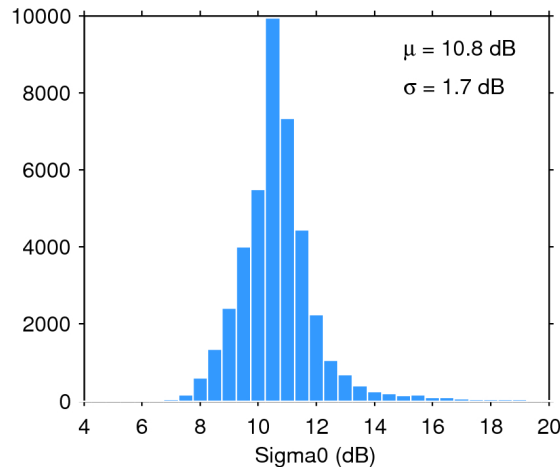
Figure 25. Histogram of flag-valid sigma0 over oceans and lakes for 30/04/2019. The mean ( \mu ) and standard deviation ( \sigma ) are also shown. Note that values outside [4 20] dB are excluded from the histogram for the sake of readability but not from the computation of \mu and \sigma .
