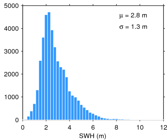
Figure 17. Histogram of flag-valid SWH over oceans and lakes for 30/04/2019. The mean ( \mu ) and standard deviation ( \sigma ) are also shown. Note that values larger than 12 m are excluded from the histogram for the sake of readability but not from the computation of \mu and \sigma .
