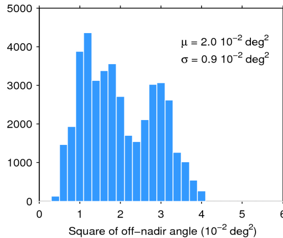
Figure 39. Histogram of flag-valid mispointing over oceans and lakes for 30/04/2019. The mean ( \mu ) and standard deviation ( \sigma ) are also shown. Note that values larger than 6 \cdot 10^{-2} \text{ deg}^2 are excluded from the histogram for the sake of readability but not from the computation of \mu and \sigma .
