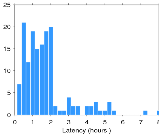
Figure 2. Histogram of the data latency for 29/04/2019. The y-axis denotes the number of files that are made available with a delay of x-hours with respect to the mean time of the records stored in the file.
