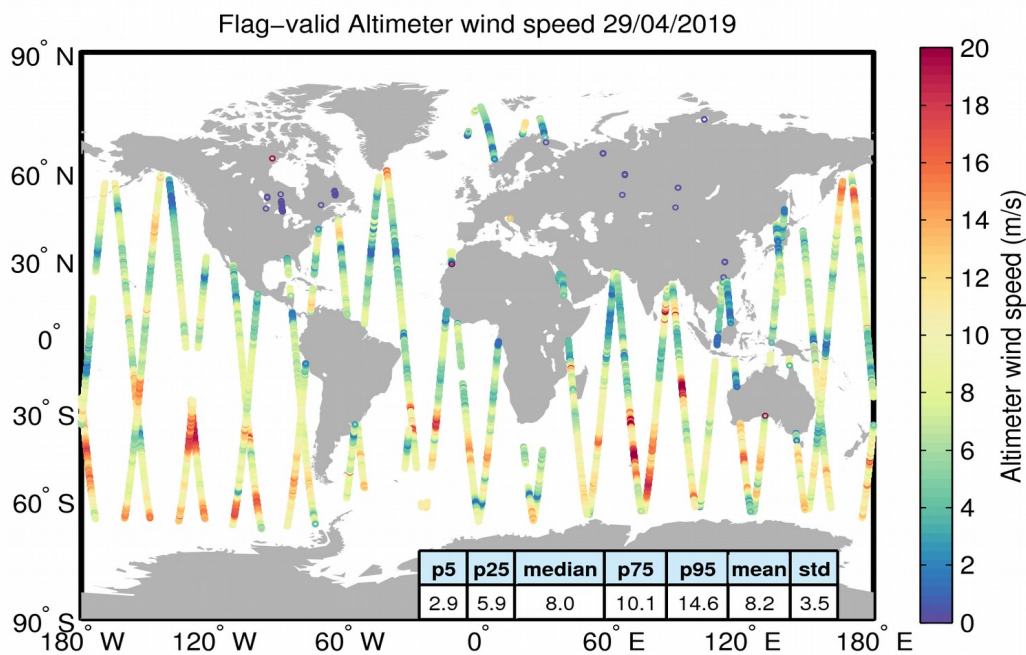
Figure 31. Geographical distribution of flag-valid wind data over oceans and lakes for 29/04/2019. The statistical values shown in the table refer to the wind in m/s and are calculated over all measurements shown in the figure.
