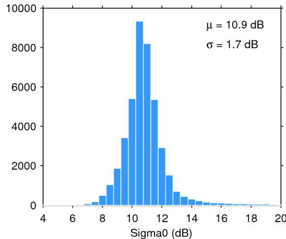
Figure 25. Histogram of flag-valid sigma0 over oceans and lakes for 29/04/2019. The mean ( \mu ) and standard deviation ( \sigma ) are also shown. Note that values outside [4 20] dB are excluded from the histogram for the sake of readability but not from the computation of \mu and \sigma .
