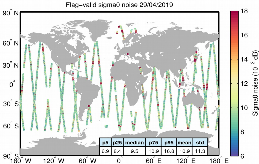
Figure 26. Geographical distribution of flag-valid 20-Hz sigma0 measurement noise over oceans and lakes for 29/04/2019. The statistical values shown in the table refer to the sigma0 noise and are calculated over all measurements shown in the figure.
