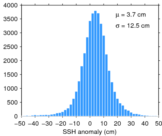
Figure 11. Histogram of science-valid SSH anomaly over oceans and lakes for 29/04/2019. The mean ( \mu ) and standard deviation ( \sigma ) are also shown. Note that values outside [-50 50] cm are excluded from the histogram for the sake of readability but not from the computation of \mu and \sigma .
