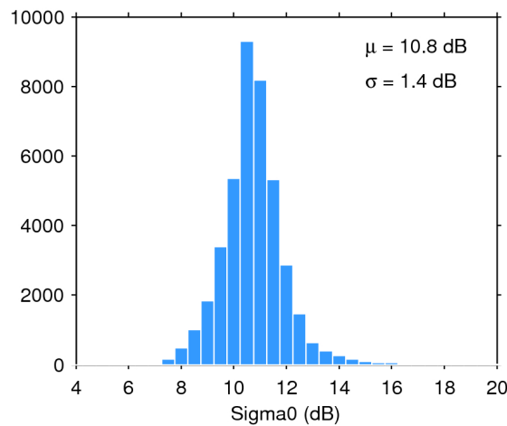
Figure 28. Histogram of science-valid sigma0 over oceans and lakes for 29/04/2019. The mean ( \mu ) and standard deviation ( \sigma ) are also shown. Note that values outside [4 20] dB are excluded from the histogram for the sake of readability but not from the computation of \mu and \sigma .
