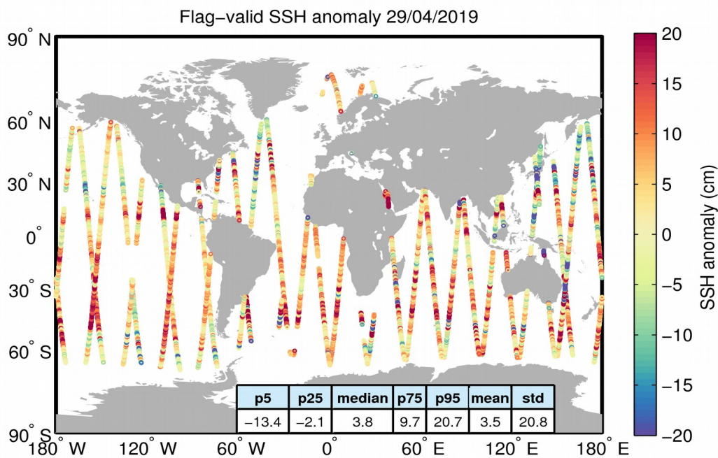
Figure 5. Geographical distribution of flag-valid 1-Hz SSH anomaly data over oceans and lakes for 29/04/2019. The statistical values shown in the table refer to the SSH anomaly in cm and are calculated over all measurements shown in the figure.
