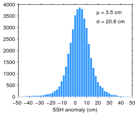
Figure 7. Histogram of flag-valid SSH anomaly over oceans and lakes for 29/04/2019. The mean ( \mu ) and standard deviation ( \sigma ) are also shown. Note that values outside [-50 50] cm are excluded from the histogram for the sake of readability but not from the computation of \mu and \sigma .
