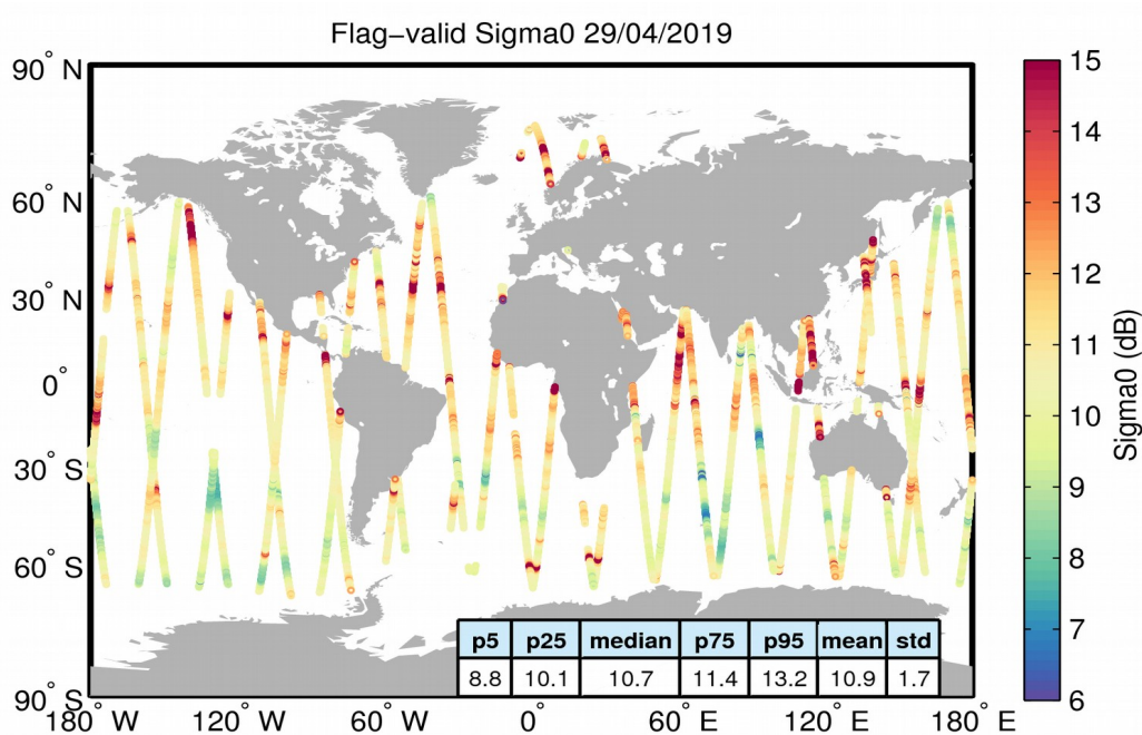
Figure 23. Geographical distribution of flag-valid sigma0 data over oceans and lakes for 29/04/2019. The statistical values shown in the table refer to the sigma0 in dB and are calculated over all measurements shown in the figure.
