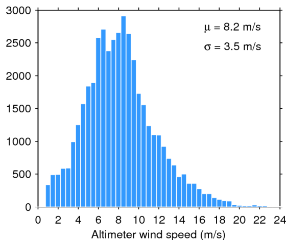
Figure 35. Histogram of science-valid wind over oceans and lakes for 29/04/2019. The mean ( \mu ) and standard deviation ( \sigma ) are also shown. Note that values larger than 24 m/s are excluded from the histogram for the sake of readability but not from the computation of \mu and \sigma .
