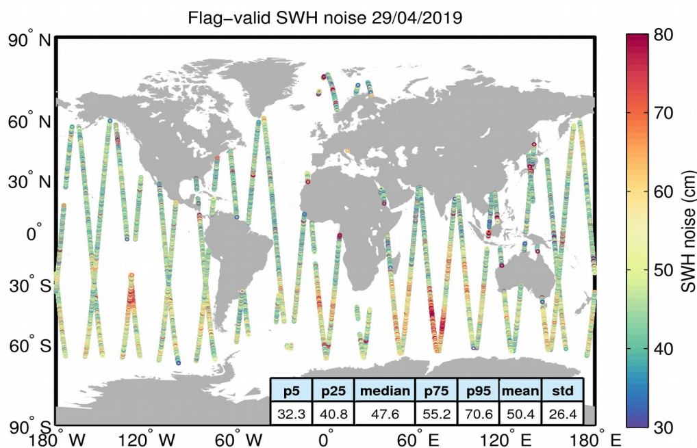
Figure 18. Geographical distribution of flag-valid 20-Hz SWH measurement noise over oceans and lakes for 29/04/2019. The statistical values shown in the figure refer to the SWH noise and are calculated over all measurements shown in the figure.
