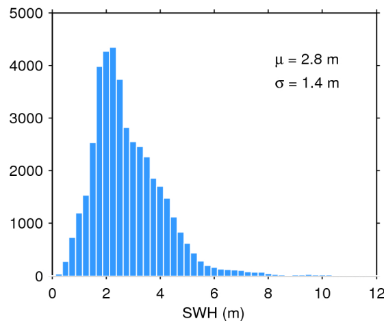
Figure 17. Histogram of flag-valid SWH over oceans and lakes for 29/04/2019. The mean ( \mu ) and standard deviation ( \sigma ) are also shown. Note that values larger than 12 m are excluded from the histogram for the sake of readability but not from the computation of \mu and \sigma .
