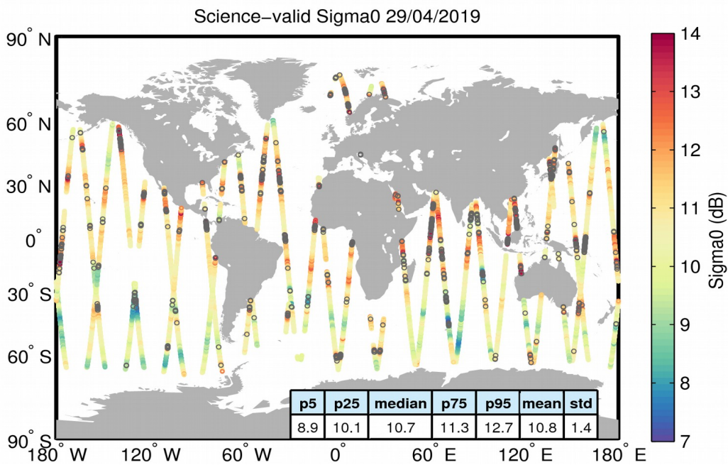
Figure 27. Geographical distribution of science-valid sigma0 data over oceans and lakes for 29/04/2019. The statistical values shown in the table refer to the sigma0 in dB and are calculated over all measurements shown in the figure. Gray circles denote records that have been rejected based on the editing criteria described in Table 4.
