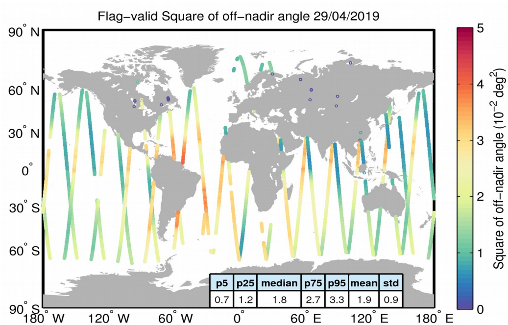
Figure 37. Geographical distribution of flag-valid mispointing data over oceans and lakes for 29/04/2019. The statistical values shown in the table refer to the mispointing in 10^{-2} \text{ deg}^2 and are calculated over all measurements shown in the figure.
