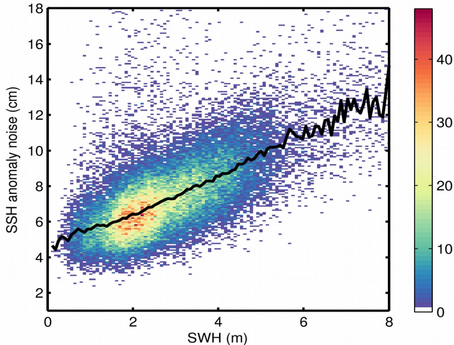
Figure 9. 2D histogram showing flag-valid SSH anomaly noise as a function of SWH for 29/04/2019. The black line denotes the median SSH anomaly noise as a function of SWH.
