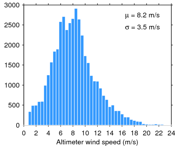
Figure 33. Histogram of flag-valid wind over oceans and lakes for 29/04/2019. The mean ( \mu ) and standard deviation ( \sigma ) are also shown. Note that values larger than 24 m/s are excluded from the histogram for the sake of readability but not from the computation of \mu and \sigma .
