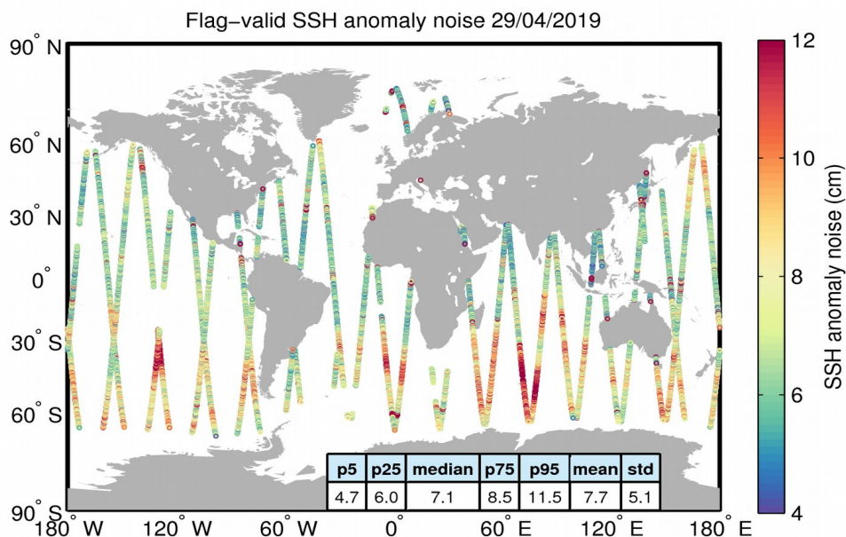
Figure 8. Geographical distribution of flag-valid 20-Hz SSH anomaly measurement noise over oceans and lakes for 29/04/2019. The statistical values shown in the table refer to the SSH anomaly noise and are calculated over all measurements shown in the figure.
