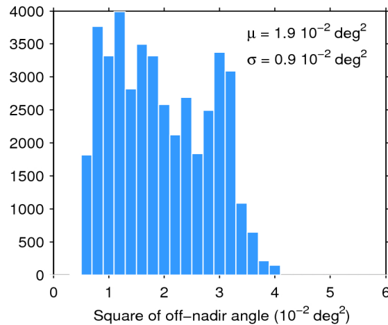
Figure 39. Histogram of flag-valid mispointing over oceans and lakes for 29/04/2019. The mean ( \mu ) and standard deviation ( \sigma ) are also shown. Note that values larger than 6 \cdot 10^{-2} \text{ deg}^2 are excluded from the histogram for the sake of readability but not from the computation of \mu and \sigma .
