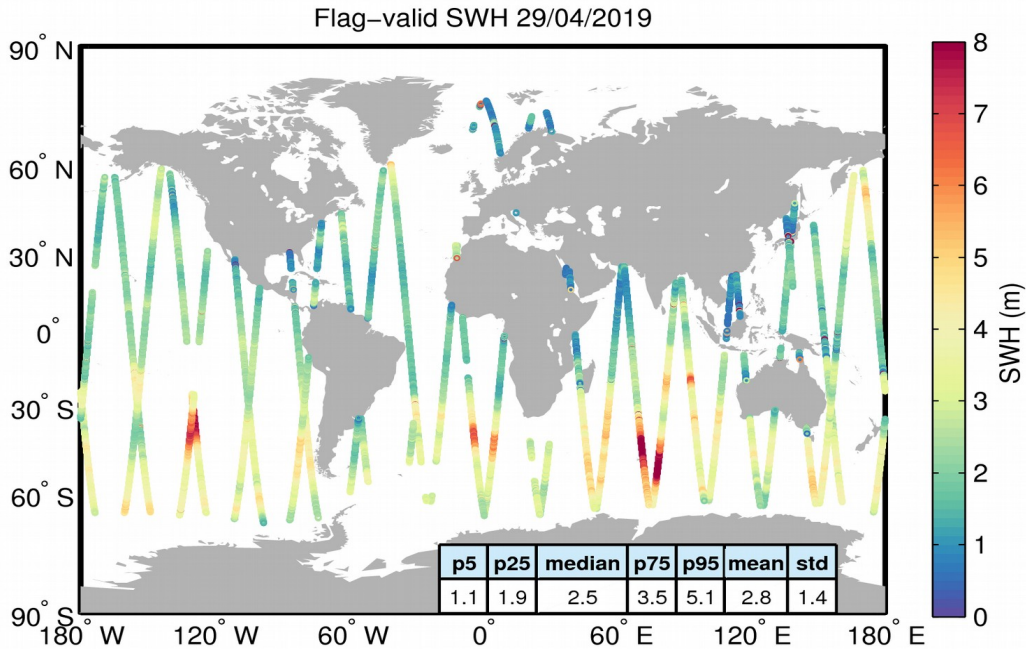
Figure 15. Geographical distribution of flag-valid SWH data over oceans and lakes for 29/04/2019. The statistical values shown in the table refer to the SWH in m and are calculated over all measurements shown in the figure.
