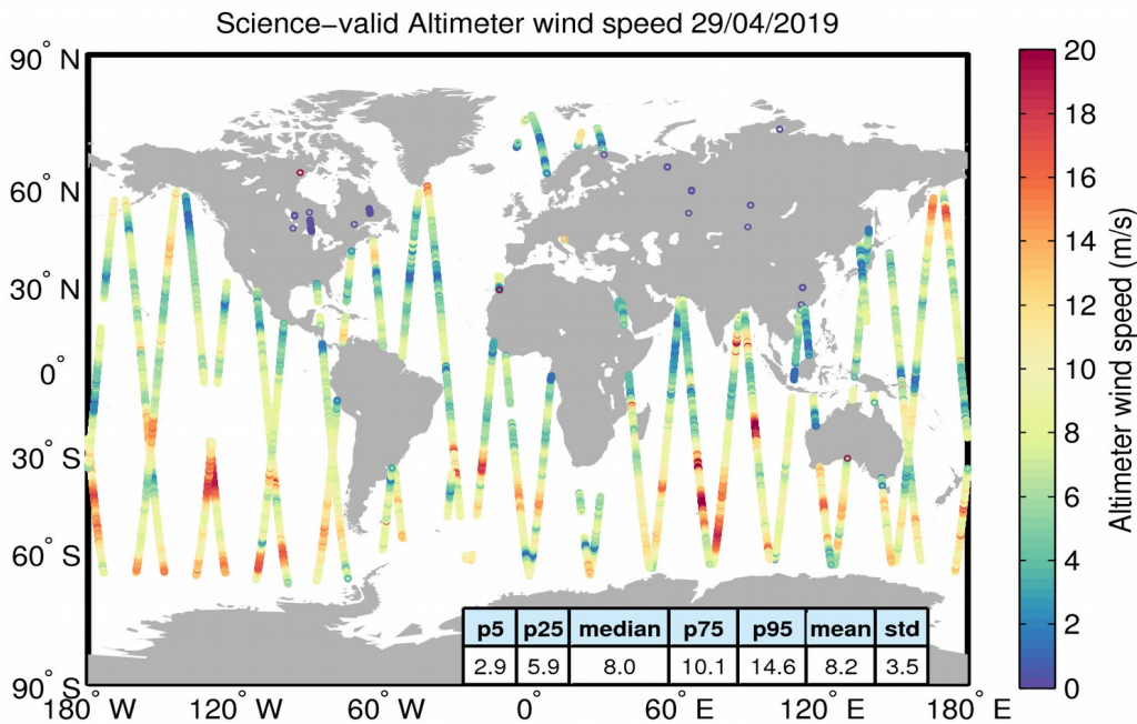
Figure 34. Geographical distribution of science-valid wind data over oceans and lakes for 29/04/2019. The statistical values shown in the table refer to the wind in m/s and are calculated over all measurements shown in the figure. Gray circles denote records that have been rejected based on the editing criteria described in Table 5.
