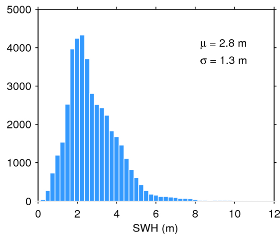
Figure 20. Histogram of science-valid SWH over oceans and lakes for 29/04/2019. The mean ( \mu ) and standard deviation ( \sigma ) are also shown. Note that values larger than 12 m are excluded from the histogram for the sake of readability but not from the computation of \mu and \sigma .
