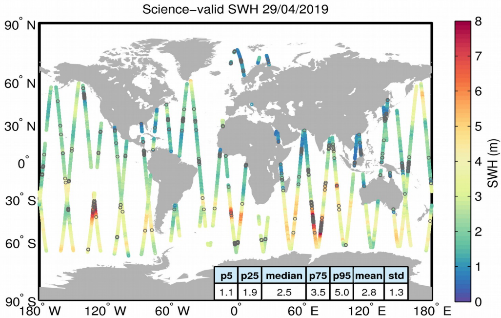
Figure 19. Geographical distribution of science-valid SWH data over oceans and lakes for 29/04/2019. The statistical values shown in the table refer to the SWH in m and are calculated over all measurements shown in the figure. Gray circles denote records that have been rejected based on the editing criteria described in Table 3.
