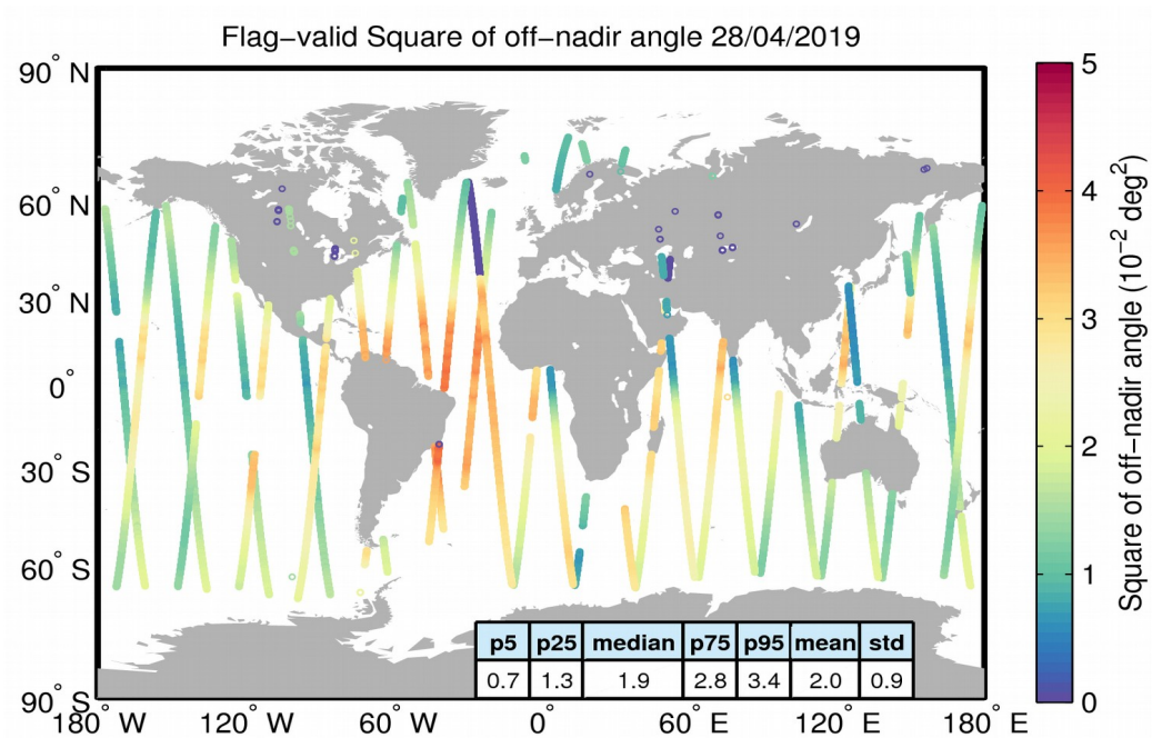
Figure 37. Geographical distribution of flag-valid mispointing data over oceans and lakes for 28/04/2019. The statistical values shown in the table refer to the mispointing in 10^{-2} deg 2 and are calculated over all measurements shown in the figure.
