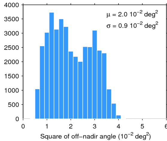
Figure 39. Histogram of flag-valid mispointing over oceans and lakes for 28/04/2019. The mean ( \mu ) and standard deviation ( \sigma ) are also shown. Note that values larger than 6 \cdot 10^{-2} \text{ deg}^2 are excluded from the histogram for the sake of readability but not from the computation of \mu and \sigma .
