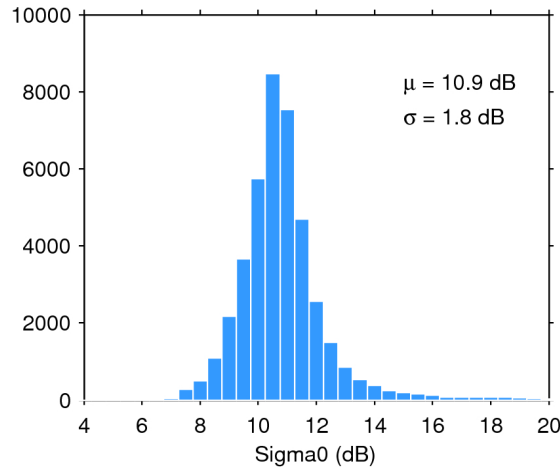
Figure 25. Histogram of flag-valid sigma0 over oceans and lakes for 28/04/2019. The mean ( \mu ) and standard deviation ( \sigma ) are also shown. Note that values outside [4 20] dB are excluded from the histogram for the sake of readability but not from the computation of \mu and \sigma .
