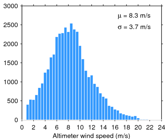
Figure 35. Histogram of science-valid wind over oceans and lakes for 28/04/2019. The mean ( \mu ) and standard deviation ( \sigma ) are also shown. Note that values larger than 24 m/s are excluded from the histogram for the sake of readability but not from the computation of \mu and \sigma .
