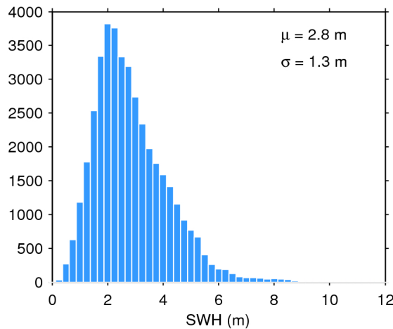
Figure 20. Histogram of science-valid SWH over oceans and lakes for 28/04/2019. The mean ( \mu ) and standard deviation ( \sigma ) are also shown. Note that values larger than 12 m are excluded from the histogram for the sake of readability but not from the computation of \mu and \sigma .
