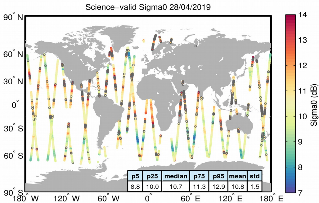
Figure 27. Geographical distribution of science-valid sigma0 data over oceans and lakes for 28/04/2019. The statistical values shown in the table refer to the sigma0 in dB and are calculated over all measurements shown in the figure. Gray circles denote records that have been rejected based on the editing criteria described in Table 4.
