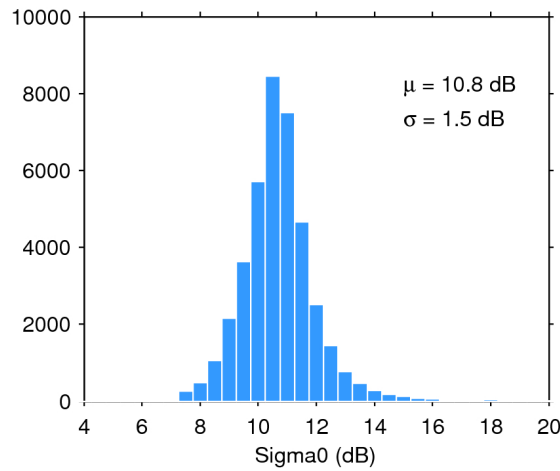
Figure 28. Histogram of science-valid sigma0 over oceans and lakes for 28/04/2019. The mean ( \mu ) and standard deviation ( \sigma ) are also shown. Note that values outside [4 20] dB are excluded from the histogram for the sake of readability but not from the computation of \mu and \sigma .
