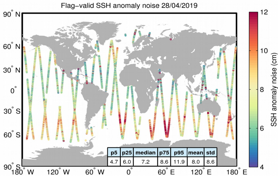
Figure 8. Geographical distribution of flag-valid 20-Hz SSH anomaly measurement noise over oceans and lakes for 28/04/2019. The statistical values shown in the table refer to the SSH anomaly noise and are calculated over all measurements shown in the figure.
