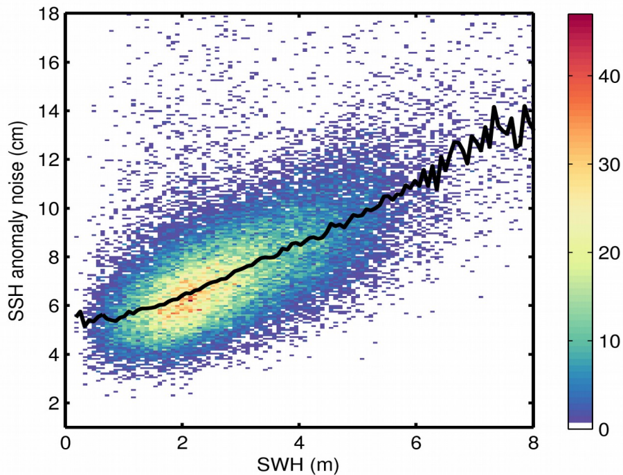
Figure 9. 2D histogram showing flag-valid SSH anomaly noise as a function of SWH for 28/04/2019. The black line denotes the median SSH anomaly noise as a function of SWH.
