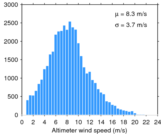
Figure 33. Histogram of flag-valid wind over oceans and lakes for 28/04/2019. The mean ( \mu ) and standard deviation ( \sigma ) are also shown. Note that values larger than 24 m/s are excluded from the histogram for the sake of readability but not from the computation of \mu and \sigma .
