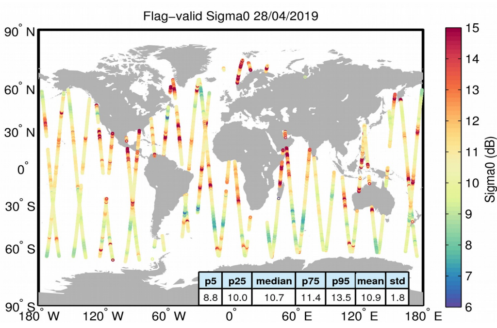
Figure 23. Geographical distribution of flag-valid sigma0 data over oceans and lakes for 28/04/2019. The statistical values shown in the table refer to the sigma0 in dB and are calculated over all measurements shown in the figure.
