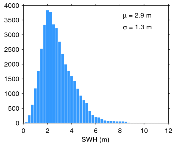
Figure 17. Histogram of flag-valid SWH over oceans and lakes for 28/04/2019. The mean ( \mu ) and standard deviation ( \sigma ) are also shown. Note that values larger than 12 m are excluded from the histogram for the sake of readability but not from the computation of \mu and \sigma .
