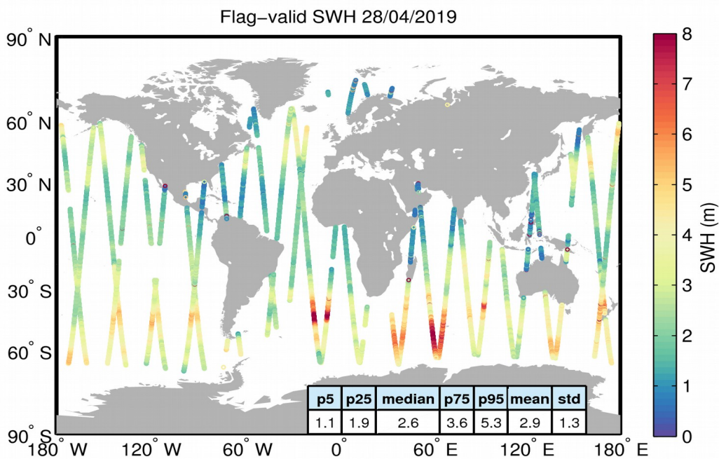
Figure 15. Geographical distribution of flag-valid SWH data over oceans and lakes for 28/04/2019. The statistical values shown in the table refer to the SWH in m and are calculated over all measurements shown in the figure.
