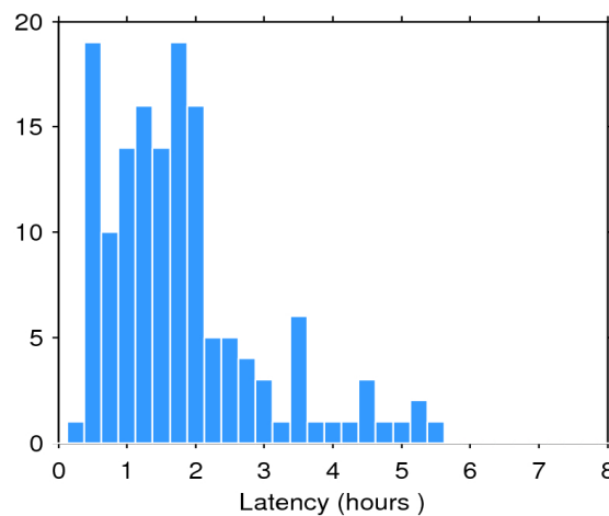
Figure 2. Histogram of the data latency for 28/04/2019. The y-axis denotes the number of files that are made available with a delay of x-hours with respect to the mean time of the records stored in the file.
