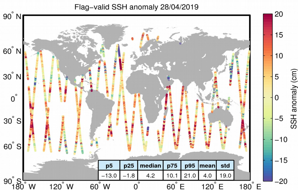
Figure 5. Geographical distribution of flag-valid 1-Hz SSH anomaly data over oceans and lakes for 28/04/2019. The statistical values shown in the table refer to the SSH anomaly in cm and are calculated over all measurements shown in the figure.
