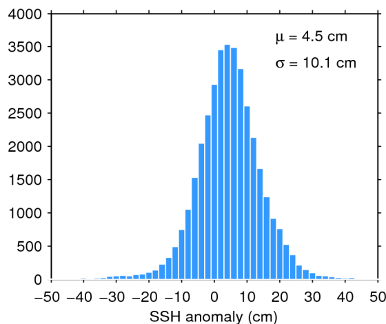
Figure 11. Histogram of science-valid SSH anomaly over oceans and lakes for 28/04/2019. The mean ( \mu ) and standard deviation ( \sigma ) are also shown. Note that values outside [-50 50] cm are excluded from the histogram for the sake of readability but not from the computation of \mu and \sigma .
