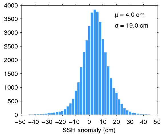
Figure 7. Histogram of flag-valid SSH anomaly over oceans and lakes for 28/04/2019. The mean ( \mu ) and standard deviation ( \sigma ) are also shown. Note that values outside [-50 50] cm are excluded from the histogram for the sake of readability but not from the computation of \mu and \sigma .
