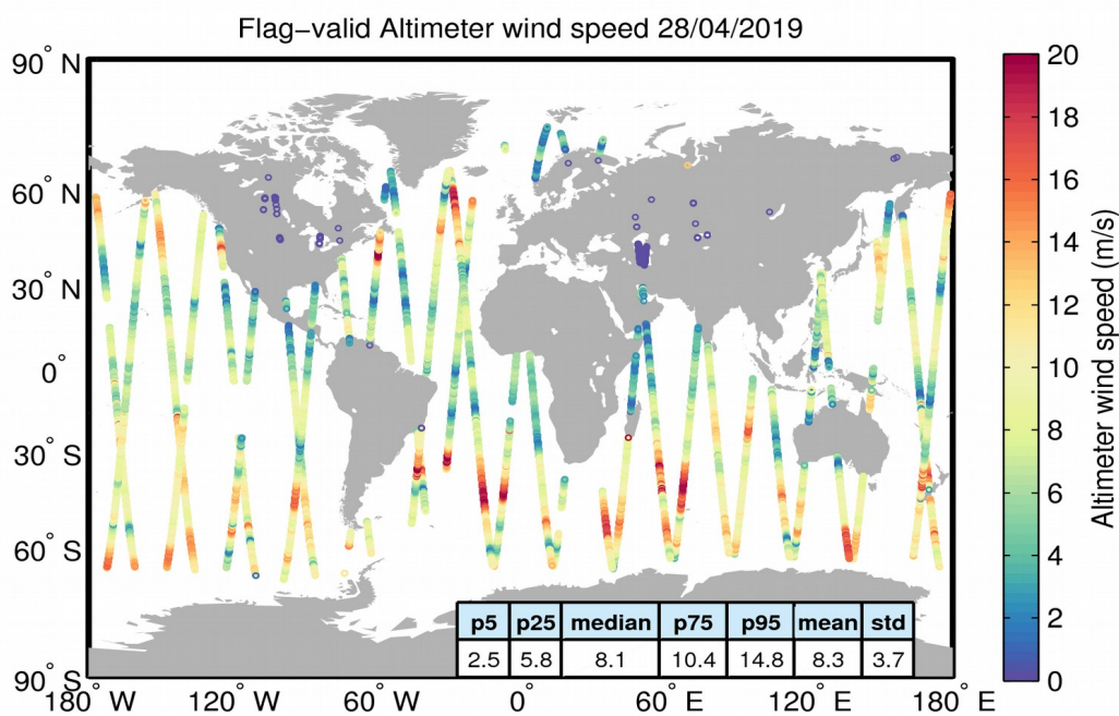
Figure 31. Geographical distribution of flag-valid wind data over oceans and lakes for 28/04/2019. The statistical values shown in the table refer to the wind in m/s and are calculated over all measurements shown in the figure.
