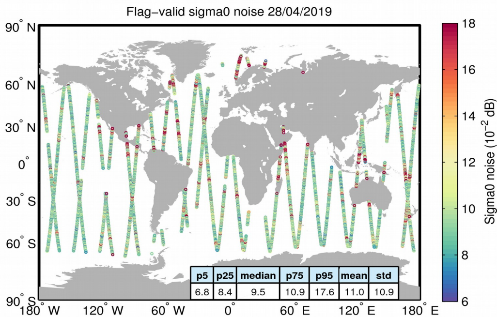
Figure 26. Geographical distribution of flag-valid 20-Hz sigma0 measurement noise over oceans and lakes for 28/04/2019. The statistical values shown in the table refer to the sigma0 noise and are calculated over all measurements shown in the figure.
