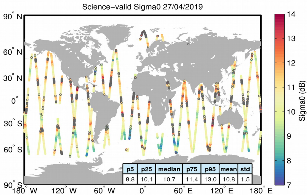
Figure 27. Geographical distribution of science-valid sigma0 data over oceans and lakes for 27/04/2019. The statistical values shown in the table refer to the sigma0 in dB and are calculated over all measurements shown in the figure. Gray circles denote records that have been rejected based on the editing criteria described in Table 4.
