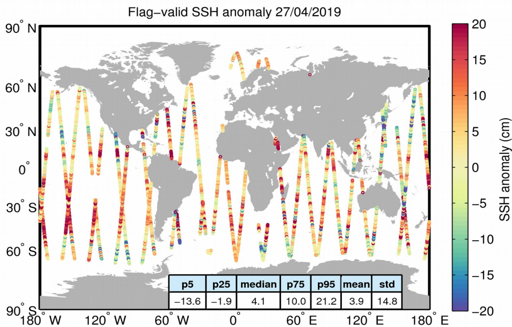
Figure 5. Geographical distribution of flag-valid 1-Hz SSH anomaly data over oceans and lakes for 27/04/2019. The statistical values shown in the table refer to the SSH anomaly in cm and are calculated over all measurements shown in the figure.
