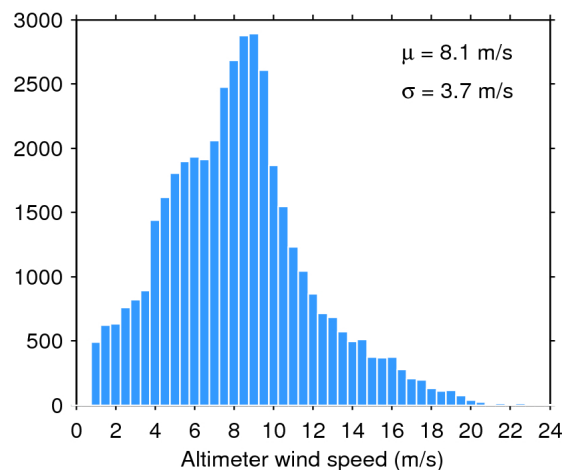
Figure 35. Histogram of science-valid wind over oceans and lakes for 27/04/2019. The mean ( \mu ) and standard deviation ( \sigma ) are also shown. Note that values larger than 24 m/s are excluded from the histogram for the sake of readability but not from the computation of \mu and \sigma .
