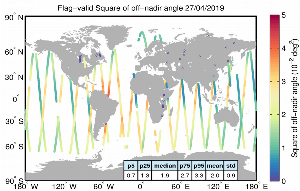
Figure 37. Geographical distribution of flag-valid mispointing data over oceans and lakes for 27/04/2019. The statistical values shown in the table refer to the mispointing in 10^{-2} \text{ deg}^2 and are calculated over all measurements shown in the figure.
