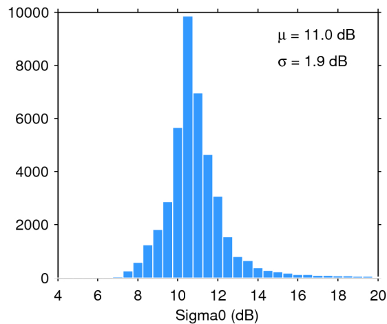
Figure 25. Histogram of flag-valid sigma0 over oceans and lakes for 27/04/2019. The mean ( \mu ) and standard deviation ( \sigma ) are also shown. Note that values outside [4 20] dB are excluded from the histogram for the sake of readability but not from the computation of \mu and \sigma .
