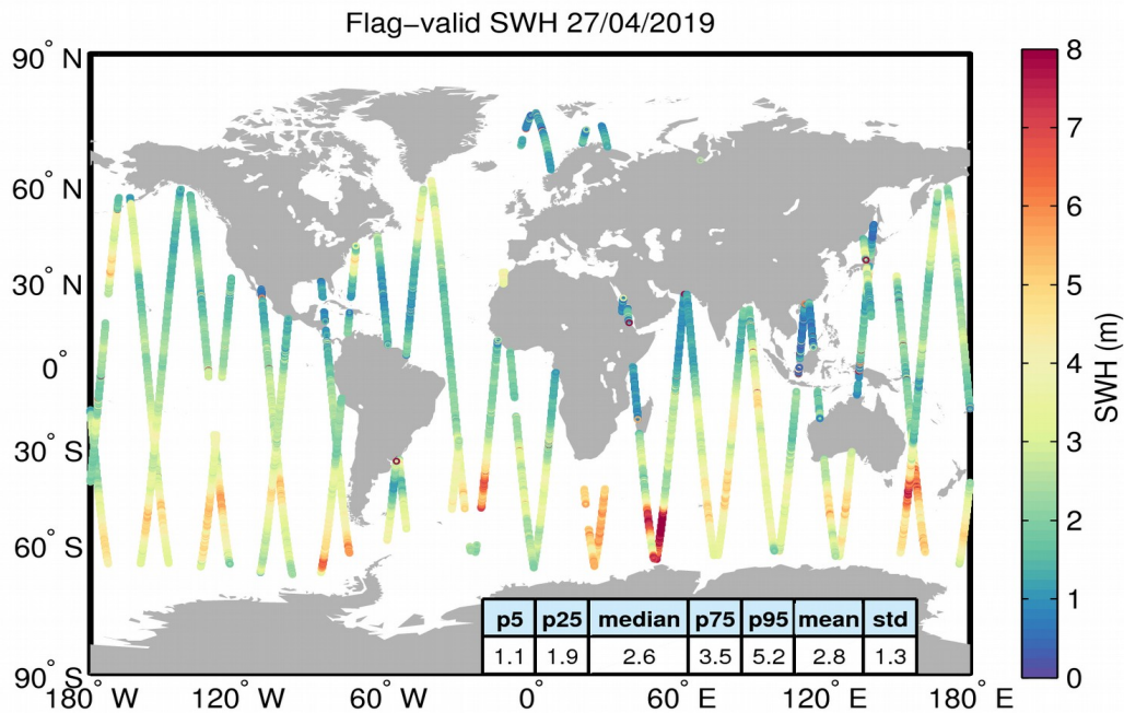
Figure 15. Geographical distribution of flag-valid SWH data over oceans and lakes for 27/04/2019. The statistical values shown in the table refer to the SWH in m and are calculated over all measurements shown in the figure.
