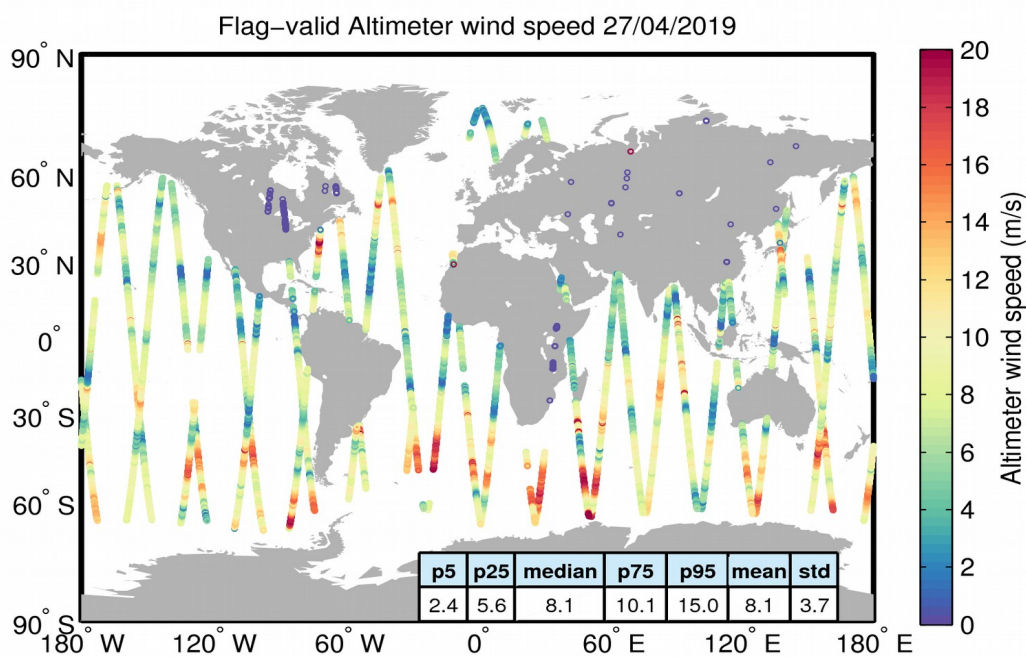
Figure 31. Geographical distribution of flag-valid wind data over oceans and lakes for 27/04/2019. The statistical values shown in the table refer to the wind in m/s and are calculated over all measurements shown in the figure.
