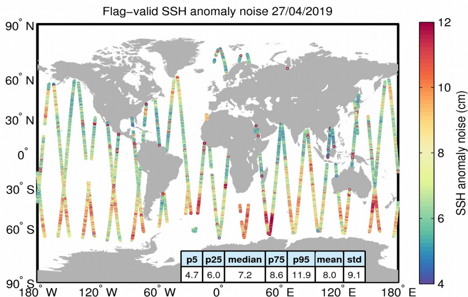
Figure 8. Geographical distribution of flag-valid 20-Hz SSH anomaly measurement noise over oceans and lakes for 27/04/2019. The statistical values shown in the table refer to the SSH anomaly noise and are calculated over all measurements shown in the figure.
