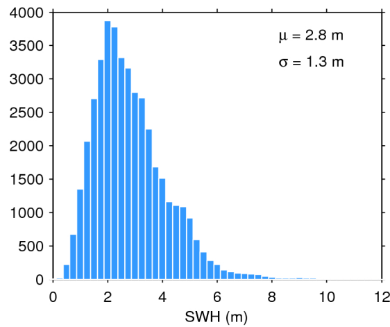
Figure 17. Histogram of flag-valid SWH over oceans and lakes for 27/04/2019. The mean ( \mu ) and standard deviation ( \sigma ) are also shown. Note that values larger than 12 m are excluded from the histogram for the sake of readability but not from the computation of \mu and \sigma .
