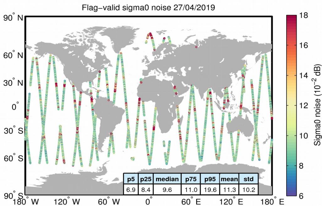
Figure 26. Geographical distribution of flag-valid 20-Hz sigma0 measurement noise over oceans and lakes for 27/04/2019. The statistical values shown in the table refer to the sigma0 noise and are calculated over all measurements shown in the figure.
