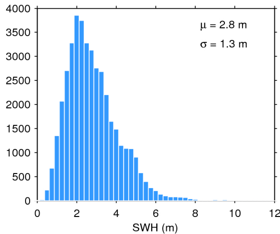
Figure 20. Histogram of science-valid SWH over oceans and lakes for 27/04/2019. The mean ( \mu ) and standard deviation ( \sigma ) are also shown. Note that values larger than 12 m are excluded from the histogram for the sake of readability but not from the computation of \mu and \sigma .
