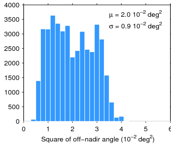
Figure 39. Histogram of flag-valid mispointing over oceans and lakes for 27/04/2019. The mean ( \mu ) and standard deviation ( \sigma ) are also shown. Note that values larger than 6 \cdot 10^{-2} \text{ deg}^2 are excluded from the histogram for the sake of readability but not from the computation of \mu and \sigma .
