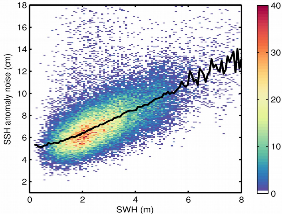
Figure 9. 2D histogram showing flag-valid SSH anomaly noise as a function of SWH for 27/04/2019. The black line denotes the median SSH anomaly noise as a function of SWH.
