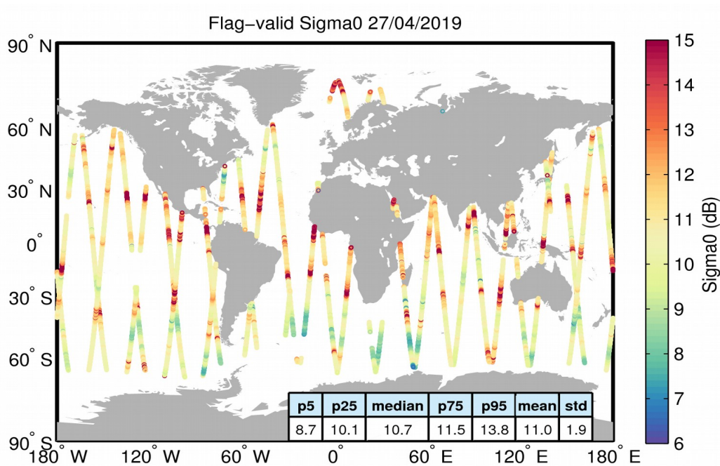
Figure 23. Geographical distribution of flag-valid sigma0 data over oceans and lakes for 27/04/2019. The statistical values shown in the table refer to the sigma0 in dB and are calculated over all measurements shown in the figure.
