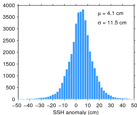
Figure 11. Histogram of science-valid SSH anomaly over oceans and lakes for 27/04/2019. The mean ( \mu ) and standard deviation ( \sigma ) are also shown. Note that values outside [-50 50] cm are excluded from the histogram for the sake of readability but not from the computation of \mu and \sigma .
