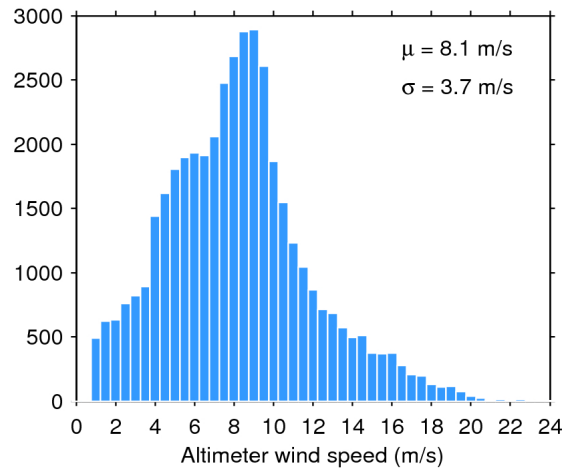
Figure 33. Histogram of flag-valid wind over oceans and lakes for 27/04/2019. The mean ( \mu ) and standard deviation ( \sigma ) are also shown. Note that values larger than 24 m/s are excluded from the histogram for the sake of readability but not from the computation of \mu and \sigma .
