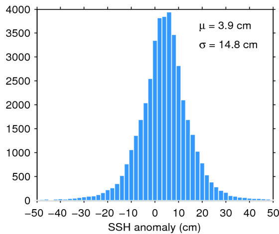
Figure 7. Histogram of flag-valid SSH anomaly over oceans and lakes for 27/04/2019. The mean ( \mu ) and standard deviation ( \sigma ) are also shown. Note that values outside [-50 50] cm are excluded from the histogram for the sake of readability but not from the computation of \mu and \sigma .
