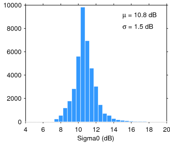
Figure 28. Histogram of science-valid sigma0 over oceans and lakes for 27/04/2019. The mean ( \mu ) and standard deviation ( \sigma ) are also shown. Note that values outside [4 20] dB are excluded from the histogram for the sake of readability but not from the computation of \mu and \sigma .
