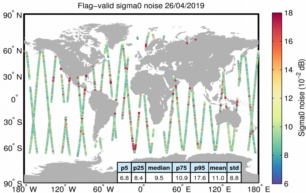
Figure 26. Geographical distribution of flag-valid 20-Hz sigma0 measurement noise over oceans and lakes for 26/04/2019. The statistical values shown in the table refer to the sigma0 noise and are calculated over all measurements shown in the figure.
