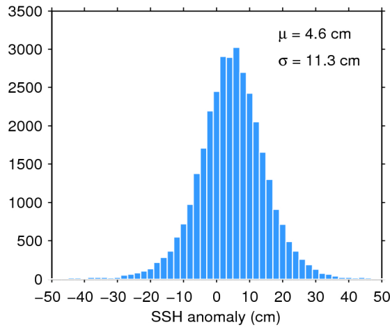
Figure 11. Histogram of science-valid SSH anomaly over oceans and lakes for 26/04/2019. The mean ( \mu ) and standard deviation ( \sigma ) are also shown. Note that values outside [-50 50] cm are excluded from the histogram for the sake of readability but not from the computation of \mu and \sigma .
