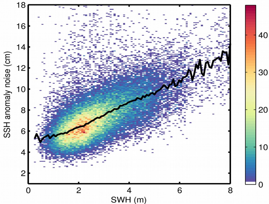
Figure 9. 2D histogram showing flag-valid SSH anomaly noise as a function of SWH for 26/04/2019. The black line denotes the median SSH anomaly noise as a function of SWH.
