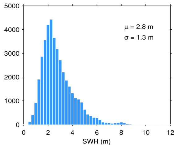
Figure 17. Histogram of flag-valid SWH over oceans and lakes for 26/04/2019. The mean ( \mu ) and standard deviation ( \sigma ) are also shown. Note that values larger than 12 m are excluded from the histogram for the sake of readability but not from the computation of \mu and \sigma .
