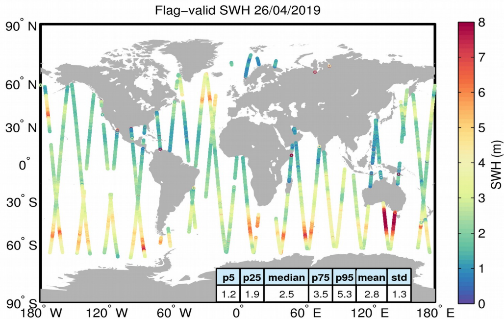
Figure 15. Geographical distribution of flag-valid SWH data over oceans and lakes for 26/04/2019. The statistical values shown in the table refer to the SWH in m and are calculated over all measurements shown in the figure.
