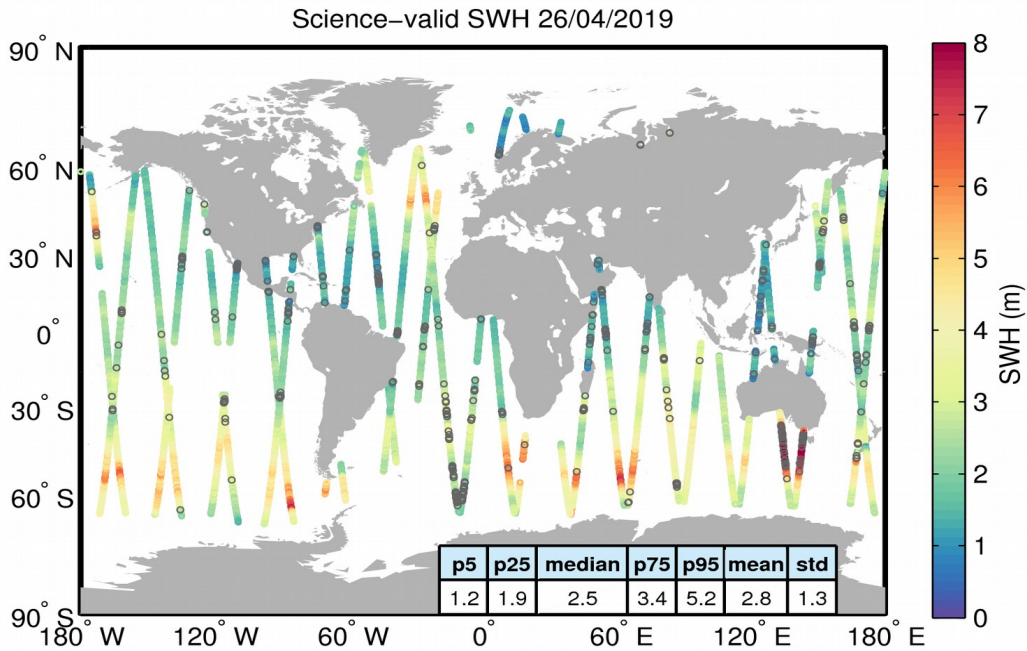
Figure 19. Geographical distribution of science-valid SWH data over oceans and lakes for 26/04/2019. The statistical values shown in the table refer to the SWH in m and are calculated over all measurements shown in the figure. Gray circles denote records that have been rejected based on the editing criteria described in Table 3.
