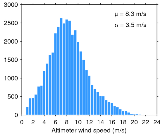
Figure 33. Histogram of flag-valid wind over oceans and lakes for 26/04/2019. The mean ( \mu ) and standard deviation ( \sigma ) are also shown. Note that values larger than 24 m/s are excluded from the histogram for the sake of readability but not from the computation of \mu and \sigma .
