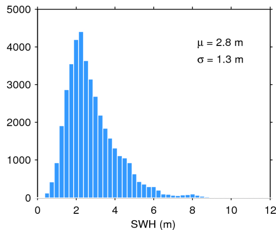
Figure 20. Histogram of science-valid SWH over oceans and lakes for 26/04/2019. The mean ( \mu ) and standard deviation ( \sigma ) are also shown. Note that values larger than 12 m are excluded from the histogram for the sake of readability but not from the computation of \mu and \sigma .
