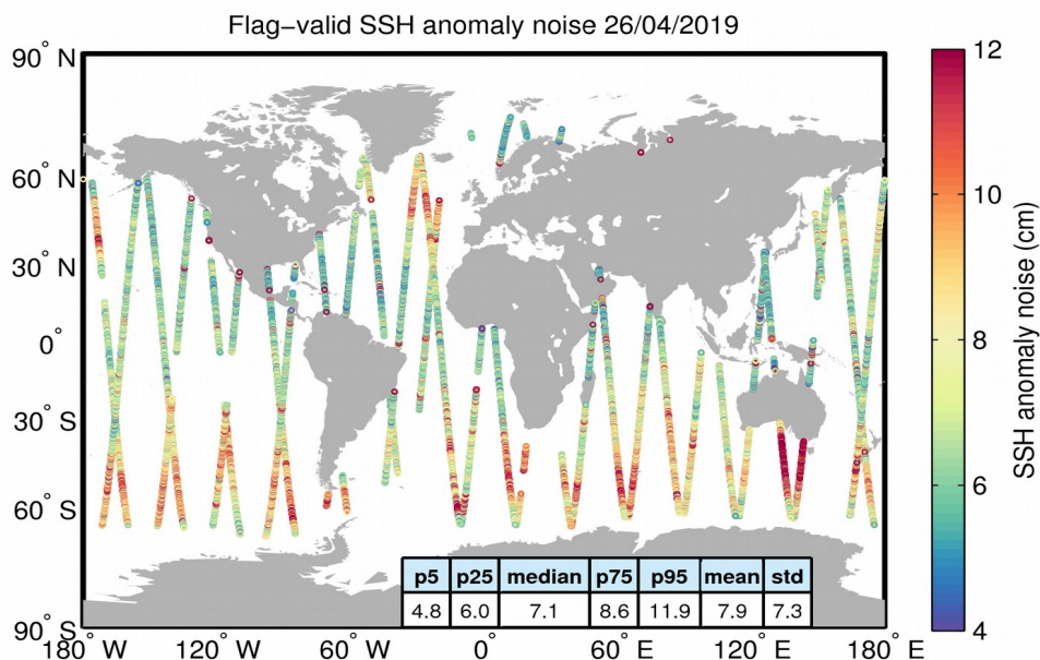
Figure 8. Geographical distribution of flag-valid 20-Hz SSH anomaly measurement noise over oceans and lakes for 26/04/2019. The statistical values shown in the table refer to the SSH anomaly noise and are calculated over all measurements shown in the figure.
