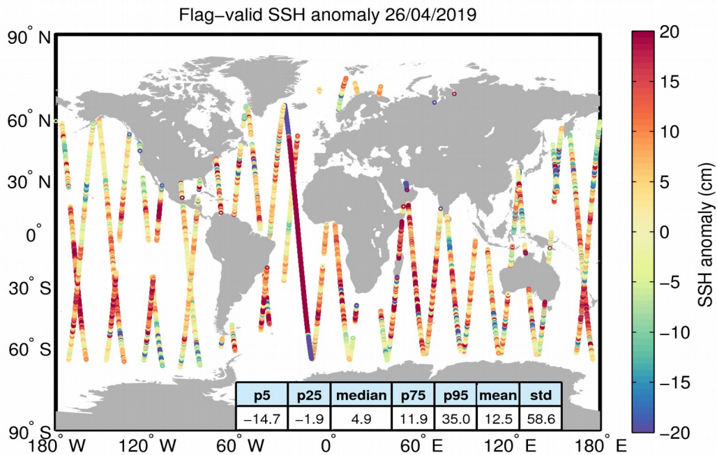
Figure 5. Geographical distribution of flag-valid 1-Hz SSH anomaly data over oceans and lakes for 26/04/2019. The statistical values shown in the table refer to the SSH anomaly in cm and are calculated over all measurements shown in the figure.
