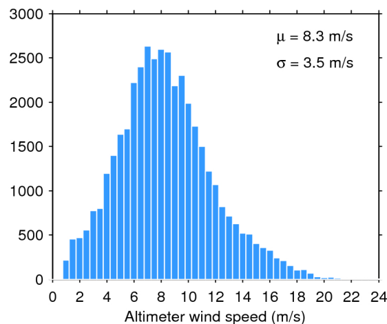
Figure 35. Histogram of science-valid wind over oceans and lakes for 26/04/2019. The mean ( \mu ) and standard deviation ( \sigma ) are also shown. Note that values larger than 24 m/s are excluded from the histogram for the sake of readability but not from the computation of \mu and \sigma .
