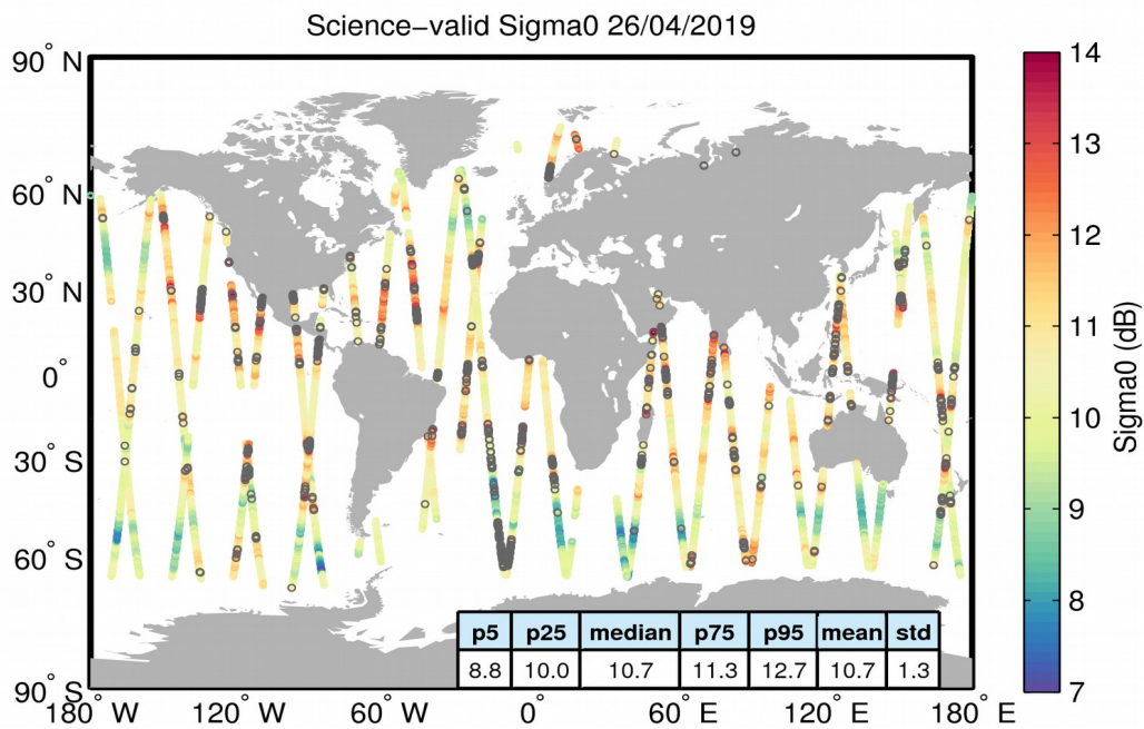
Figure 27. Geographical distribution of science-valid sigma0 data over oceans and lakes for 26/04/2019. The statistical values shown in the table refer to the sigma0 in dB and are calculated over all measurements shown in the figure. Gray circles denote records that have been rejected based on the editing criteria described in Table 4.
