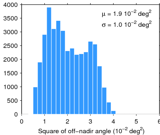
Figure 39. Histogram of flag-valid mispointing over oceans and lakes for 26/04/2019. The mean ( \mu ) and standard deviation ( \sigma ) are also shown. Note that values larger than 6 \cdot 10^{-2} \text{ deg}^2 are excluded from the histogram for the sake of readability but not from the computation of \mu and \sigma .
