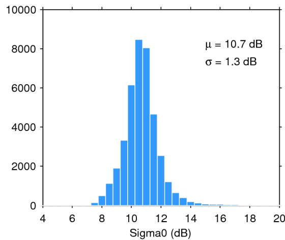
Figure 28. Histogram of science-valid sigma0 over oceans and lakes for 26/04/2019. The mean ( \mu ) and standard deviation ( \sigma ) are also shown. Note that values outside [4 20] dB are excluded from the histogram for the sake of readability but not from the computation of \mu and \sigma .
