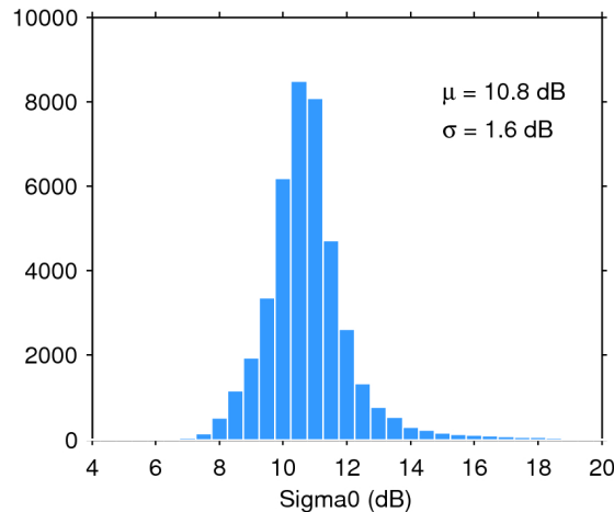
Figure 25. Histogram of flag-valid sigma0 over oceans and lakes for 26/04/2019. The mean ( \mu ) and standard deviation ( \sigma ) are also shown. Note that values outside [4 20] dB are excluded from the histogram for the sake of readability but not from the computation of \mu and \sigma .
