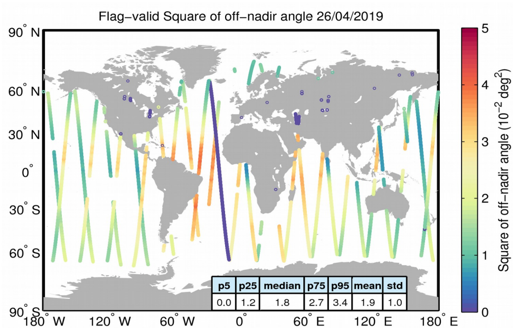
Figure 37. Geographical distribution of flag-valid mispointing data over oceans and lakes for 26/04/2019. The statistical values shown in the table refer to the mispointing in 10^{-2} \text{deg}^2 and are calculated over all measurements shown in the figure.
