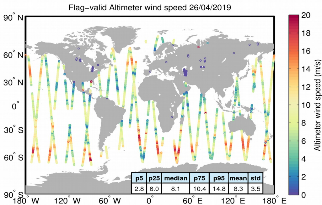
Figure 31. Geographical distribution of flag-valid wind data over oceans and lakes for 26/04/2019. The statistical values shown in the table refer to the wind in m/s and are calculated over all measurements shown in the figure.
