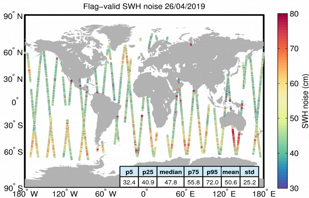
Figure 18. Geographical distribution of flag-valid 20-Hz SWH measurement noise over oceans and lakes for 26/04/2019. The statistical values shown in the figure refer to the SWH noise and are calculated over all measurements shown in the figure.
