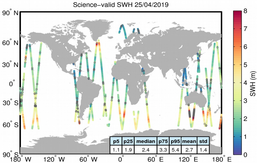
Figure 19. Geographical distribution of science-valid SWH data over oceans and lakes for 25/04/2019. The statistical values shown in the table refer to the SWH in m and are calculated over all measurements shown in the figure. Gray circles denote records that have been rejected based on the editing criteria described in Table 3.
