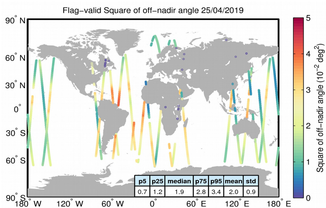
Figure 37. Geographical distribution of flag-valid mispointing data over oceans and lakes for 25/04/2019. The statistical values shown in the table refer to the mispointing in 10^{-2} deg 2 and are calculated over all measurements shown in the figure.
