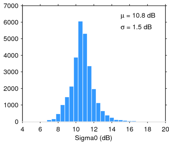
Figure 28. Histogram of science-valid sigma0 over oceans and lakes for 25/04/2019. The mean ( \mu ) and standard deviation ( \sigma ) are also shown. Note that values outside [4 20] dB are excluded from the histogram for the sake of readability but not from the computation of \mu and \sigma .
