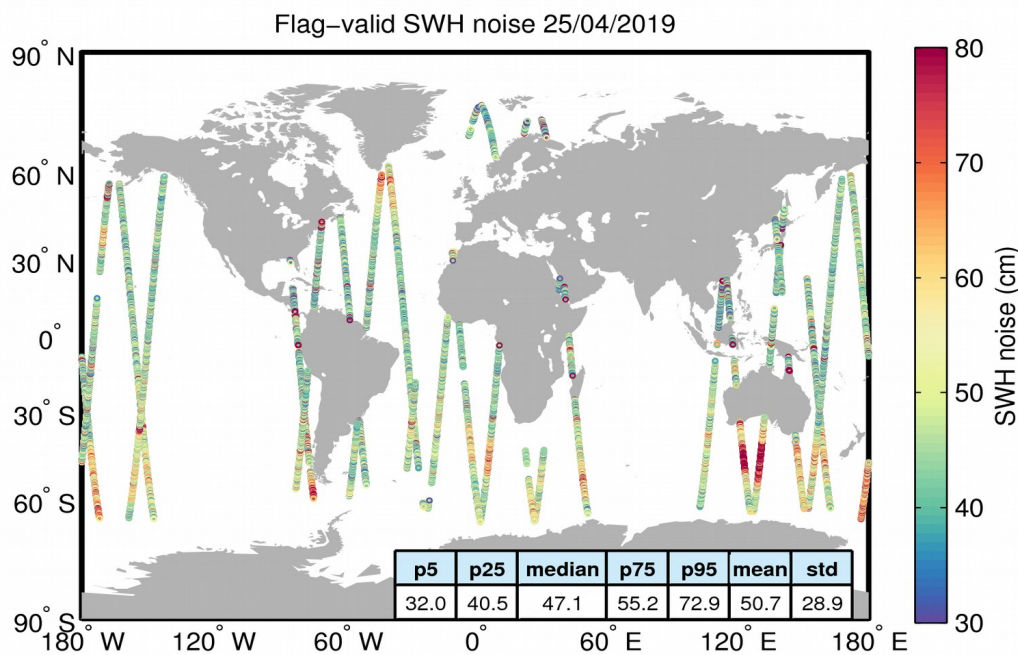
Figure 18. Geographical distribution of flag-valid 20-Hz SWH measurement noise over oceans and lakes for 25/04/2019. The statistical values shown in the table refer to the SWH noise and are calculated over all measurements shown in the figure.
