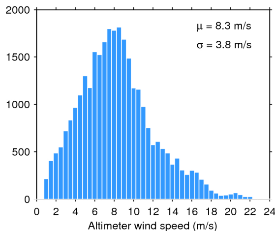
Figure 35. Histogram of science-valid wind over oceans and lakes for 25/04/2019. The mean ( \mu ) and standard deviation ( \sigma ) are also shown. Note that values larger than 24 m/s are excluded from the histogram for the sake of readability but not from the computation of \mu and \sigma .
