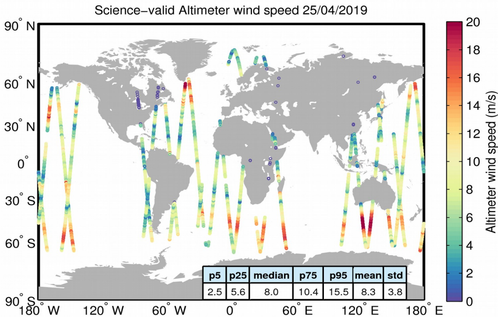
Figure 34. Geographical distribution of science-valid wind data over oceans and lakes for 25/04/2019. The statistical values shown in the table refer to the wind in m/s and are calculated over all measurements shown in the figure. Gray circles denote records that have been rejected based on the editing criteria described in Table 5.
