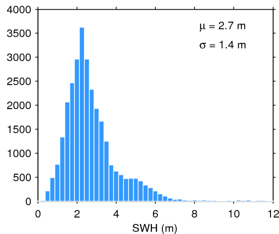
Figure 20. Histogram of science-valid SWH over oceans and lakes for 25/04/2019. The mean ( \mu ) and standard deviation ( \sigma ) are also shown. Note that values larger than 12 m are excluded from the histogram for the sake of readability but not from the computation of \mu and \sigma .
