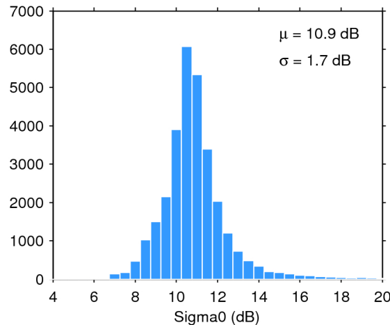
Figure 25. Histogram of flag-valid sigma0 over oceans and lakes for 25/04/2019. The mean ( \mu ) and standard deviation ( \sigma ) are also shown. Note that values outside [4 20] dB are excluded from the histogram for the sake of readability but not from the computation of \mu and \sigma .
