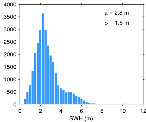
Figure 17. Histogram of flag-valid SWH over oceans and lakes for 25/04/2019. The mean ( \mu ) and standard deviation ( \sigma ) are also shown. Note that values larger than 12 m are excluded from the histogram for the sake of readability but not from the computation of \mu and \sigma .
