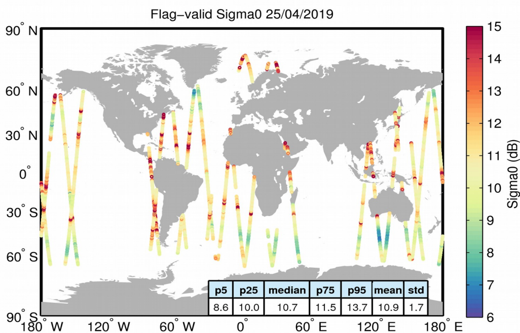
Figure 23. Geographical distribution of flag-valid sigma0 data over oceans and lakes for 25/04/2019. The statistical values shown in the table refer to the sigma0 in dB and are calculated over all measurements shown in the figure.
