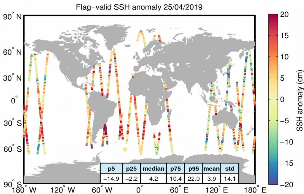
Figure 5. Geographical distribution of flag-valid 1-Hz SSH anomaly data over oceans and lakes for 25/04/2019. The statistical values shown in the table refer to the SSH anomaly in cm and are calculated over all measurements shown in the figure.
