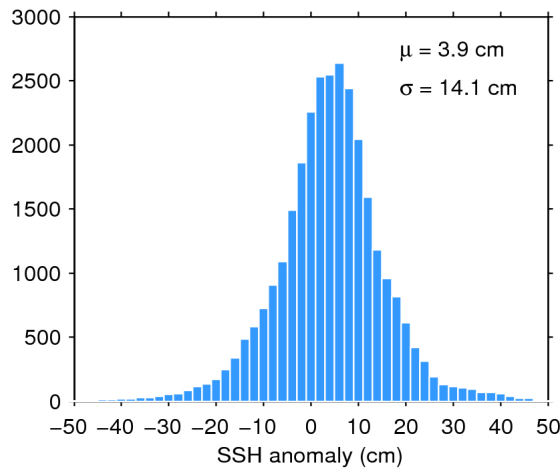
Figure 7. Histogram of flag-valid SSH anomaly over oceans and lakes for 25/04/2019. The mean ( \mu ) and standard deviation ( \sigma ) are also shown. Note that values outside [-50 50] cm are excluded from the histogram for the sake of readability but not from the computation of \mu and \sigma .
