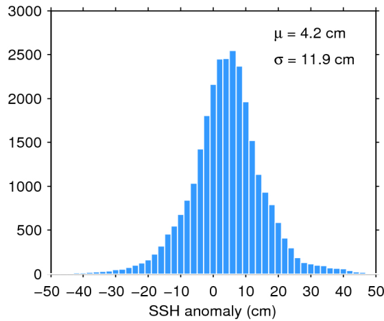
Figure 11. Histogram of science-valid SSH anomaly over oceans and lakes for 25/04/2019. The mean ( \mu ) and standard deviation ( \sigma ) are also shown. Note that values outside [-50 50] cm are excluded from the histogram for the sake of readability but not from the computation of \mu and \sigma .
