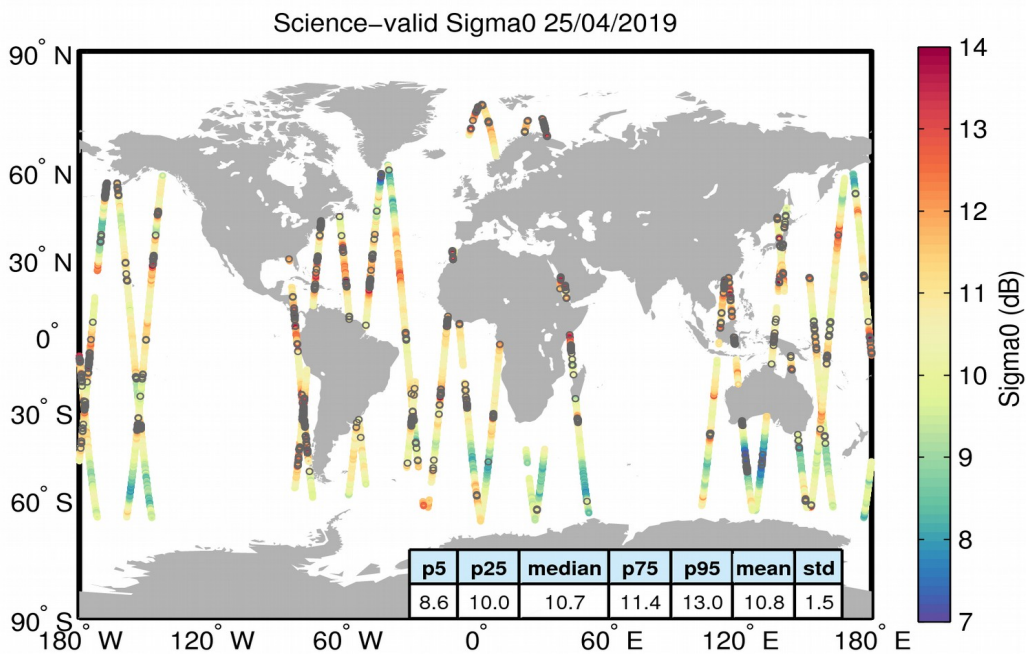
Figure 27. Geographical distribution of science-valid sigma0 data over oceans and lakes for 25/04/2019. The statistical values shown in the table refer to the sigma0 in dB and are calculated over all measurements shown in the figure. Gray circles denote records that have been rejected based on the editing criteria described in Table 4.
