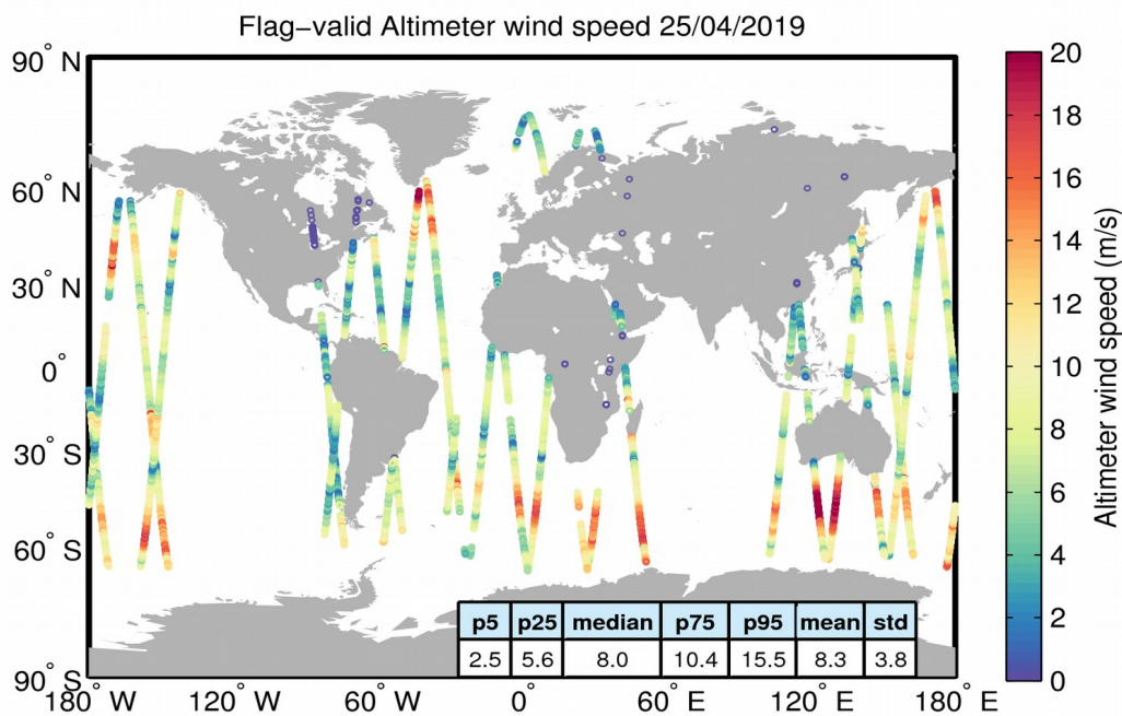
Figure 31. Geographical distribution of flag-valid wind data over oceans and lakes for 25/04/2019. The statistical values shown in the table refer to the wind in m/s and are calculated over all measurements shown in the figure.
