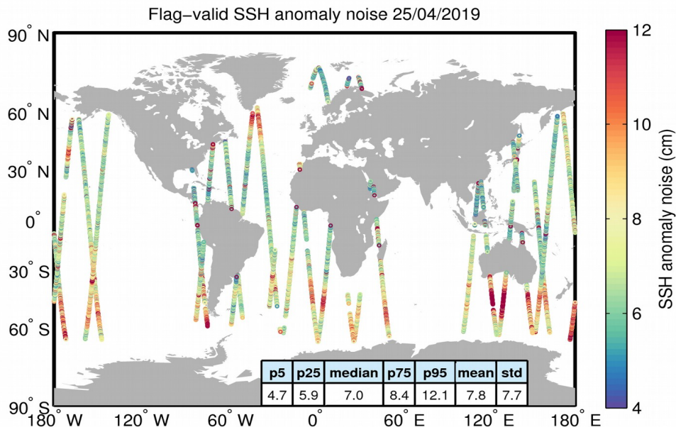
Figure 8. Geographical distribution of flag-valid 20-Hz SSH anomaly measurement noise over oceans and lakes for 25/04/2019. The statistical values shown in the table refer to the SSH anomaly noise and are calculated over all measurements shown in the figure.
