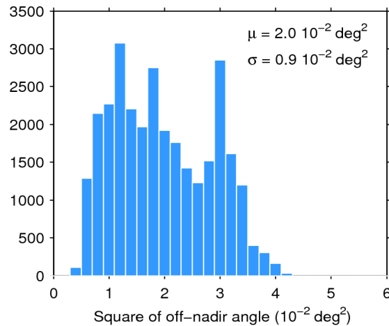
Figure 39. Histogram of flag-valid mispointing over oceans and lakes for 25/04/2019. The mean ( \mu ) and standard deviation ( \sigma ) are also shown. Note that values larger than 6 \cdot 10^{-2} \text{ deg}^2 are excluded from the histogram for the sake of readability but not from the computation of \mu and \sigma .
