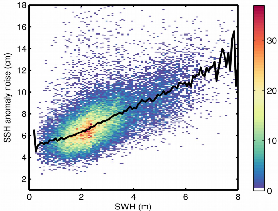
Figure 9. 2D histogram showing flag-valid SSH anomaly noise as a function of SWH for 25/04/2019. The black line denotes the median SSH anomaly noise as a function of SWH.
