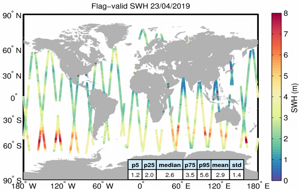
Figure 15. Geographical distribution of flag-valid SWH data over oceans and lakes for 23/04/2019. The statistical values shown in the table refer to the SWH in m and are calculated over all measurements shown in the figure.
