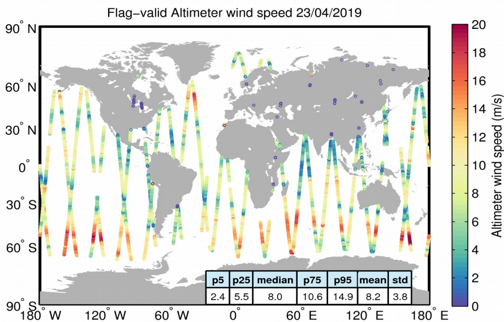
Figure 31. Geographical distribution of flag-valid wind data over oceans and lakes for 23/04/2019. The statistical values shown in the table refer to the wind in m/s and are calculated over all measurements shown in the figure.
