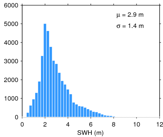
Figure 17. Histogram of flag-valid SWH over oceans and lakes for 23/04/2019. The mean ( \mu ) and standard deviation ( \sigma ) are also shown. Note that values larger than 12 m are excluded from the histogram for the sake of readability but not from the computation of \mu and \sigma .
