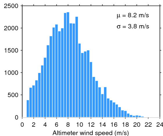
Figure 35. Histogram of science-valid wind over oceans and lakes for 23/04/2019. The mean ( \mu ) and standard deviation ( \sigma ) are also shown. Note that values larger than 24 m/s are excluded from the histogram for the sake of readability but not from the computation of \mu and \sigma .
