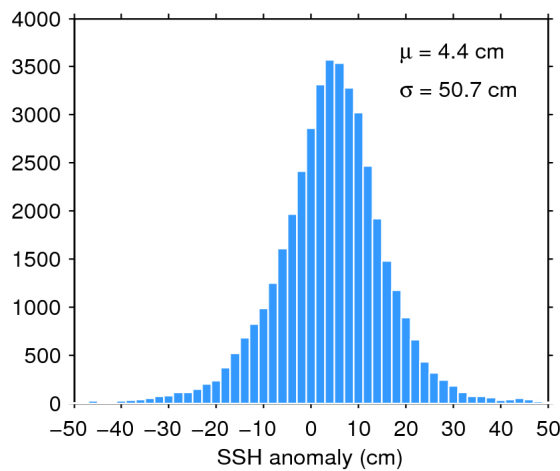
Figure 7. Histogram of flag-valid SSH anomaly over oceans and lakes for 23/04/2019. The mean ( \mu ) and standard deviation ( \sigma ) are also shown. Note that values outside [-50 50] cm are excluded from the histogram for the sake of readability but not from the computation of \mu and \sigma .
