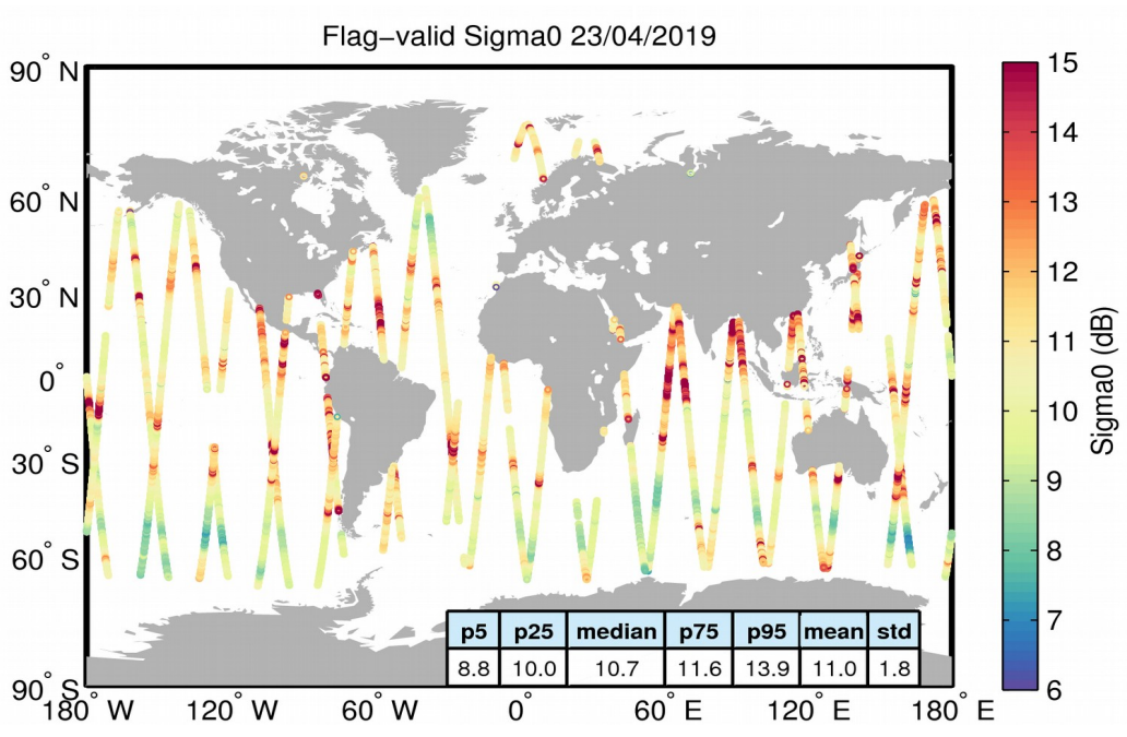
Figure 23. Geographical distribution of flag-valid sigma0 data over oceans and lakes for 23/04/2019. The statistical values shown in the table refer to the sigma0 in dB and are calculated over all measurements shown in the figure.
