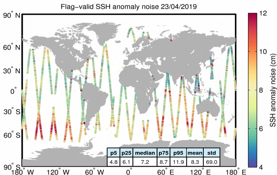
Figure 8. Geographical distribution of flag-valid 20-Hz SSH anomaly measurement noise over oceans and lakes for 23/04/2019. The statistical values shown in the table refer to the SSH anomaly noise and are calculated over all measurements shown in the figure.
