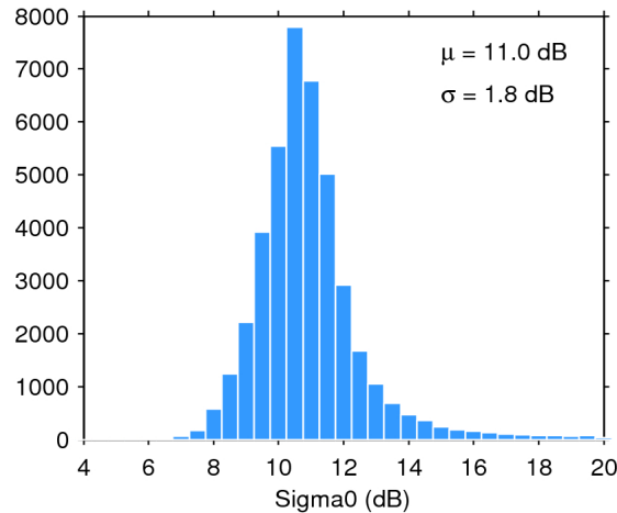
Figure 25. Histogram of flag-valid sigma0 over oceans and lakes for 23/04/2019. The mean ( \mu ) and standard deviation ( \sigma ) are also shown. Note that values outside [4 20] dB are excluded from the histogram for the sake of readability but not from the computation of \mu and \sigma .
