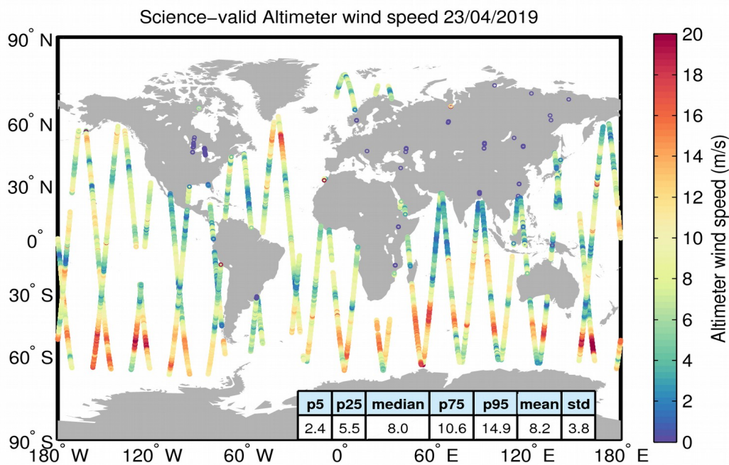
Figure 34. Geographical distribution of science-valid wind data over oceans and lakes for 23/04/2019. The statistical values shown in the table refer to the wind in m/s and are calculated over all measurements shown in the figure. Gray circles denote records that have been rejected based on the editing criteria described in Table 5.
