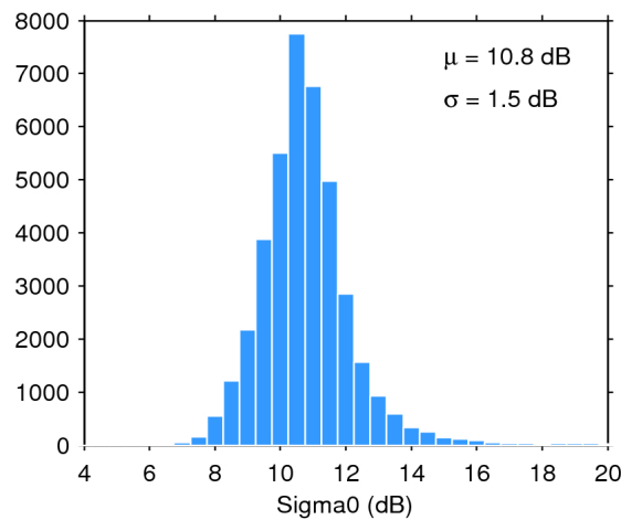
Figure 28. Histogram of science-valid sigma0 over oceans and lakes for 23/04/2019. The mean ( \mu ) and standard deviation ( \sigma ) are also shown. Note that values outside [4 20] dB are excluded from the histogram for the sake of readability but not from the computation of \mu and \sigma .
