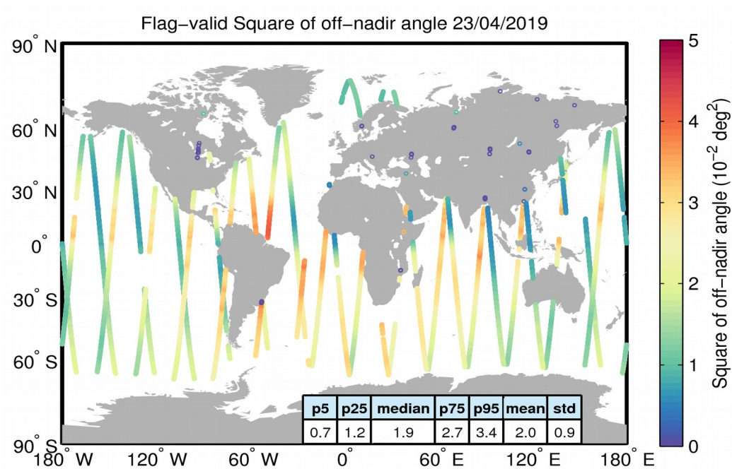
Figure 37. Geographical distribution of flag-valid mispointing data over oceans and lakes for 23/04/2019. The statistical values shown in the table refer to the mispointing in 10^{-2} \text{deg}^2 and are calculated over all measurements shown in the figure.
