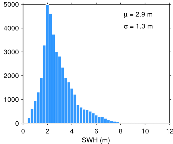
Figure 20. Histogram of science-valid SWH over oceans and lakes for 23/04/2019. The mean ( \mu ) and standard deviation ( \sigma ) are also shown. Note that values larger than 12 m are excluded from the histogram for the sake of readability but not from the computation of \mu and \sigma .
