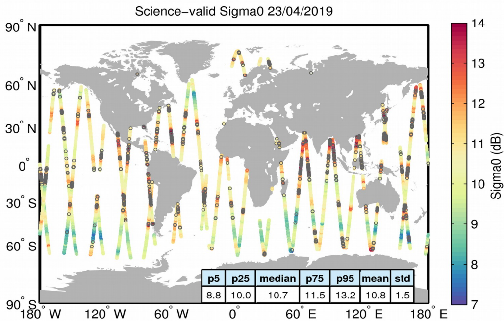
Figure 27. Geographical distribution of science-valid sigma0 data over oceans and lakes for 23/04/2019. The statistical values shown in the table refer to the sigma0 in dB and are calculated over all measurements shown in the figure. Gray circles denote records that have been rejected based on the editing criteria described in Table 4.
