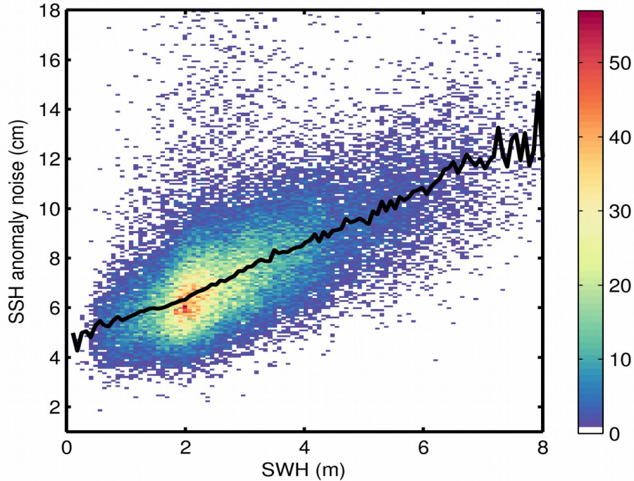
Figure 9. 2D histogram showing flag-valid SSH anomaly noise as a function of SWH for 23/04/2019. The black line denotes the median SSH anomaly noise as a function of SWH.
