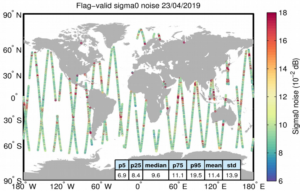
Figure 26. Geographical distribution of flag-valid 20-Hz sigma0 measurement noise over oceans and lakes for 23/04/2019. The statistical values shown in the table refer to the sigma0 noise and are calculated over all measurements shown in the figure.
