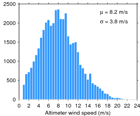
Figure 33. Histogram of flag-valid wind over oceans and lakes for 23/04/2019. The mean ( \mu ) and standard deviation ( \sigma ) are also shown. Note that values larger than 24 m/s are excluded from the histogram for the sake of readability but not from the computation of \mu and \sigma .
