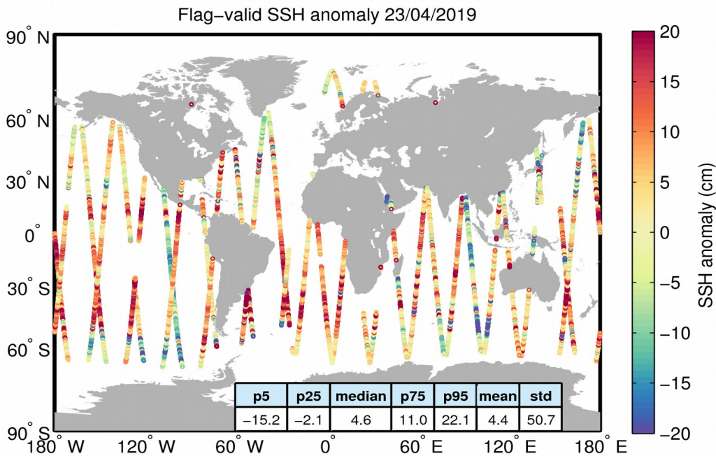
Figure 5. Geographical distribution of flag-valid 1-Hz SSH anomaly data over oceans and lakes for 23/04/2019. The statistical values shown in the table refer to the SSH anomaly in cm and are calculated over all measurements shown in the figure.
