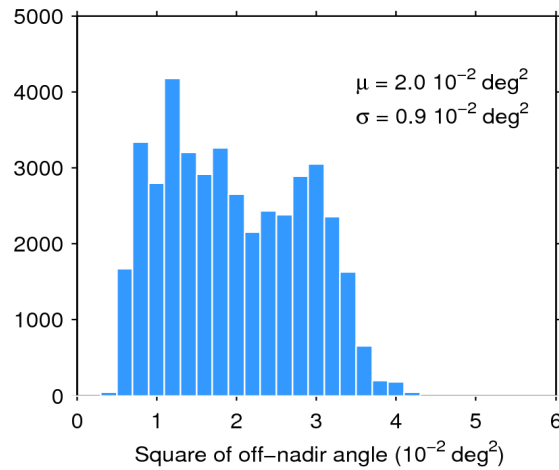
Figure 39. Histogram of flag-valid mispointing over oceans and lakes for 23/04/2019. The mean ( \mu ) and standard deviation ( \sigma ) are also shown. Note that values larger than 6 \cdot 10^{-2} \text{ deg}^2 are excluded from the histogram for the sake of readability but not from the computation of \mu and \sigma .
