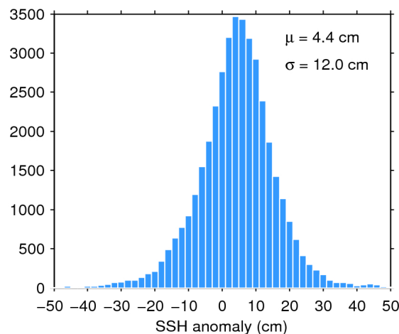
Figure 11. Histogram of science-valid SSH anomaly over oceans and lakes for 23/04/2019. The mean ( \mu ) and standard deviation ( \sigma ) are also shown. Note that values outside [-50 50] cm are excluded from the histogram for the sake of readability but not from the computation of \mu and \sigma .
