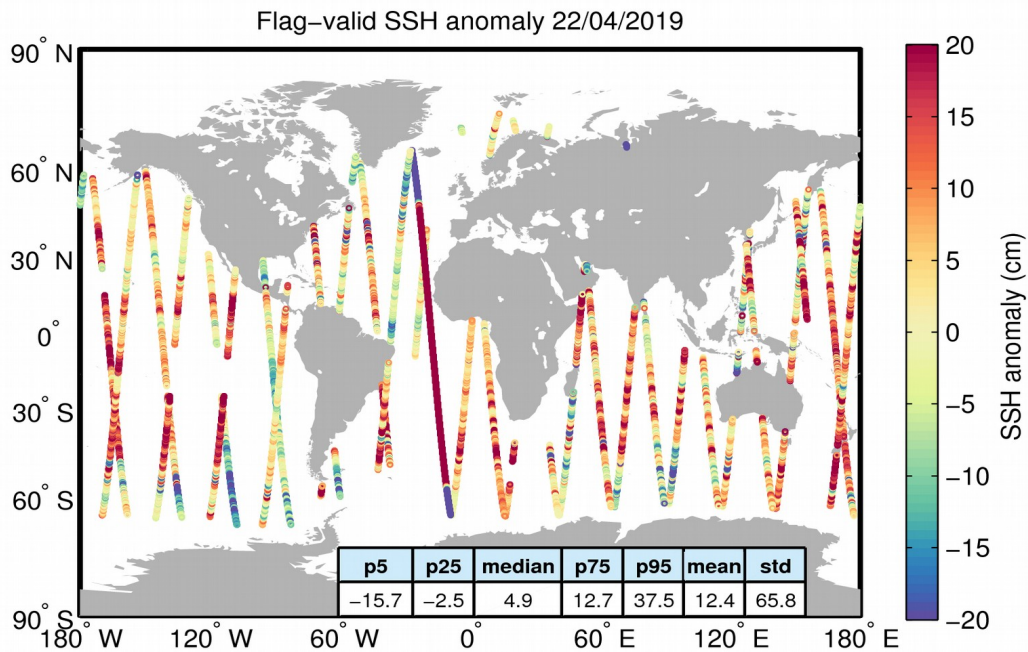
Figure 5. Geographical distribution of flag-valid 1-Hz SSH anomaly data over oceans and lakes for 22/04/2019. The statistical values shown in the table refer to the SSH anomaly in cm and are calculated over all measurements shown in the figure.
