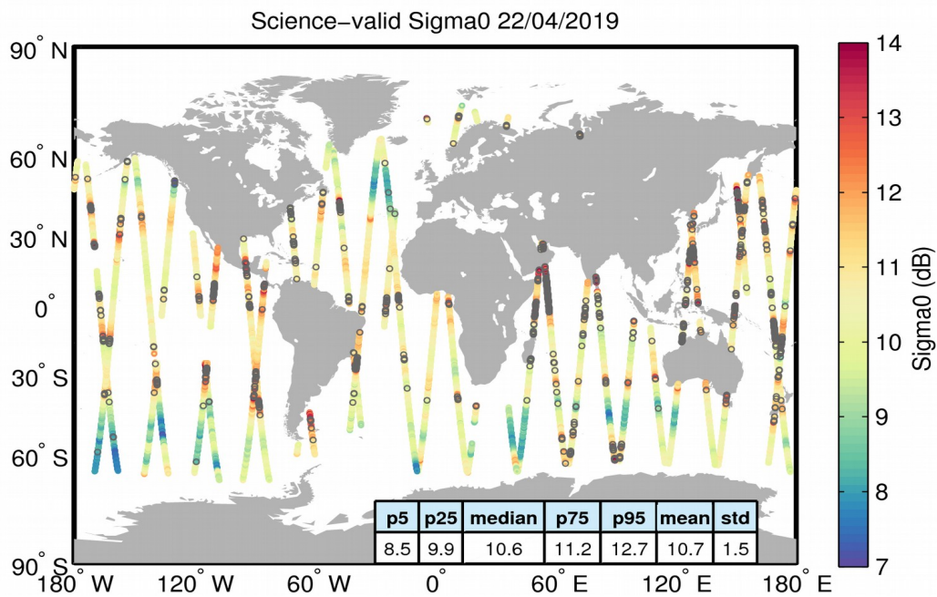
Figure 27. Geographical distribution of science-valid sigma0 data over oceans and lakes for 22/04/2019. The statistical values shown in the table refer to the sigma0 in dB and are calculated over all measurements shown in the figure. Gray circles denote records that have been rejected based on the editing criteria described in Table 4.
