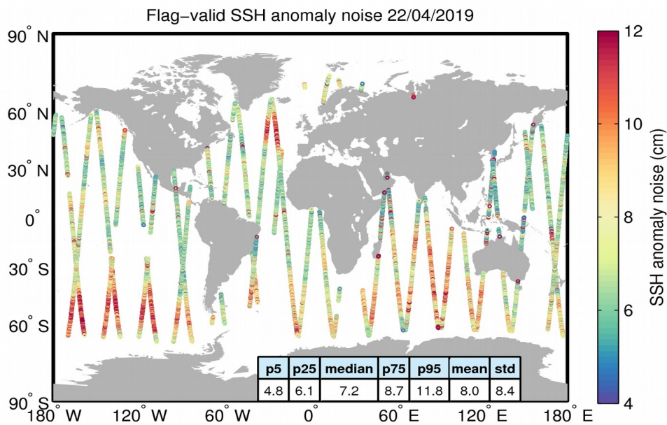
Figure 8. Geographical distribution of flag-valid 20-Hz SSH anomaly measurement noise over oceans and lakes for 22/04/2019. The statistical values shown in the table refer to the SSH anomaly noise and are calculated over all measurements shown in the figure.
