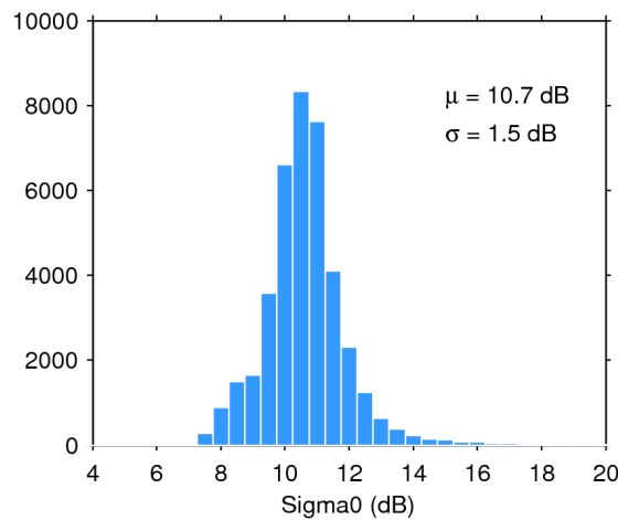
Figure 28. Histogram of science-valid sigma0 over oceans and lakes for 22/04/2019. The mean ( \mu ) and standard deviation ( \sigma ) are also shown. Note that values outside [4 20] dB are excluded from the histogram for the sake of readability but not from the computation of \mu and \sigma .
