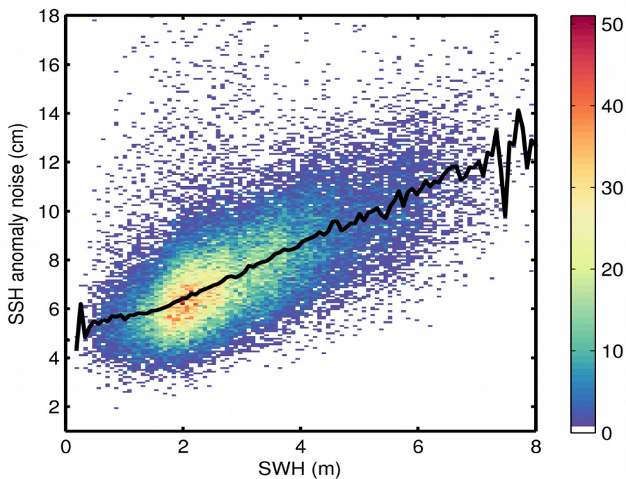
Figure 9. 2D histogram showing flag-valid SSH anomaly noise as a function of SWH for 22/04/2019. The black line denotes the median SSH anomaly noise as a function of SWH.
