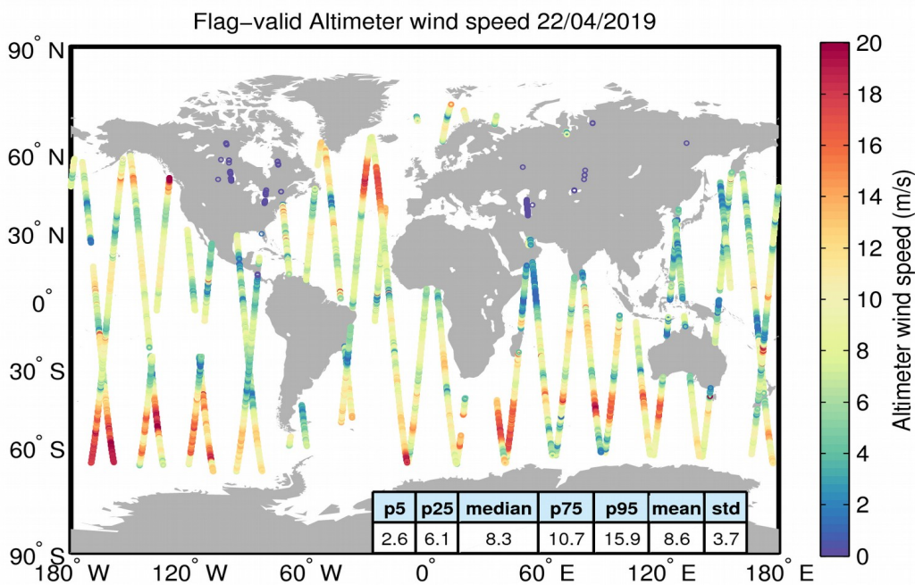
Figure 31. Geographical distribution of flag-valid wind data over oceans and lakes for 22/04/2019. The statistical values shown in the table refer to the wind in m/s and are calculated over all measurements shown in the figure.
