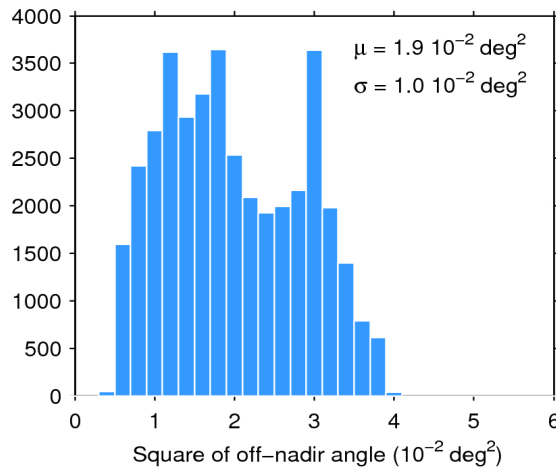
Figure 39. Histogram of flag-valid mispointing over oceans and lakes for 22/04/2019. The mean ( \mu ) and standard deviation ( \sigma ) are also shown. Note that values larger than 6 \cdot 10^{-2} \text{ deg}^2 are excluded from the histogram for the sake of readability but not from the computation of \mu and \sigma .
