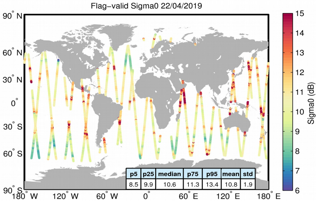
Figure 23. Geographical distribution of flag-valid sigma0 data over oceans and lakes for 22/04/2019. The statistical values shown in the table refer to the sigma0 in dB and are calculated over all measurements shown in the figure.
