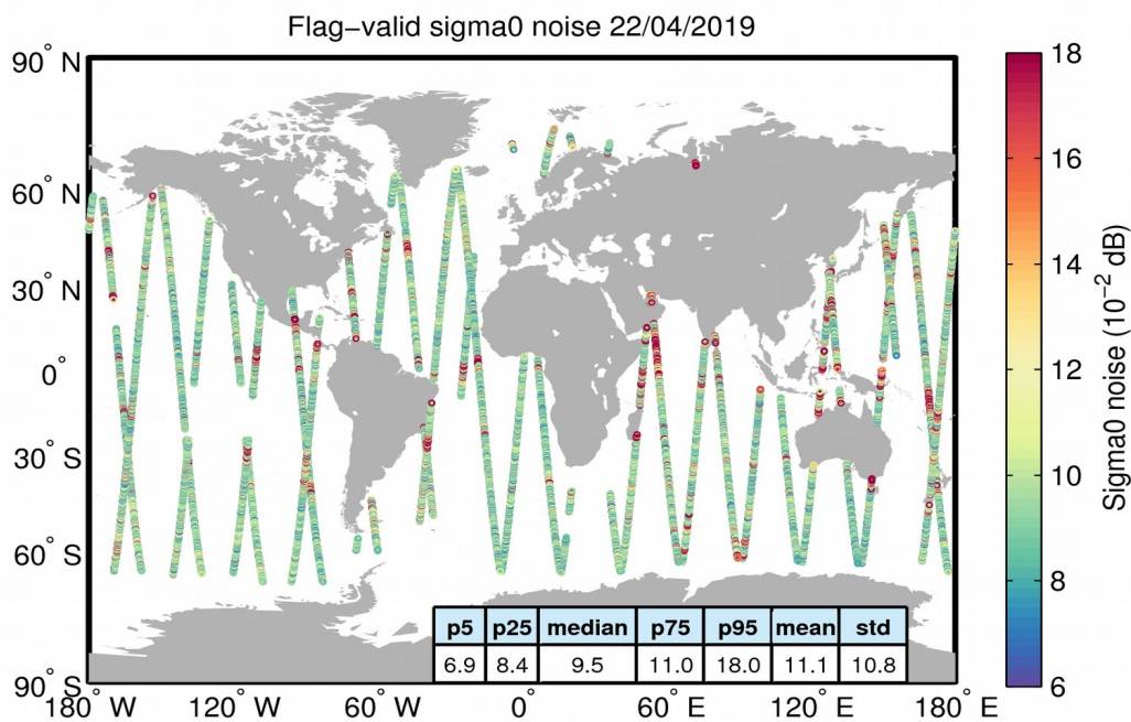
Figure 26. Geographical distribution of flag-valid 20-Hz sigma0 measurement noise over oceans and lakes for 22/04/2019. The statistical values shown in the table refer to the sigma0 noise and are calculated over all measurements shown in the figure.
