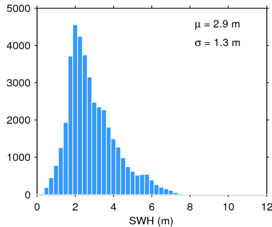
Figure 20. Histogram of science-valid SWH over oceans and lakes for 22/04/2019. The mean ( \mu ) and standard deviation ( \sigma ) are also shown. Note that values larger than 12 m are excluded from the histogram for the sake of readability but not from the computation of \mu and \sigma .
