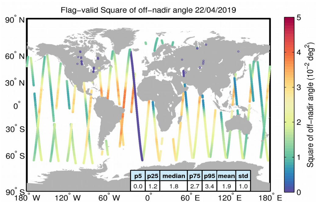
Figure 37. Geographical distribution of flag-valid mispointing data over oceans and lakes for 22/04/2019. The statistical values shown in the table refer to the mispointing in 10^{-2} deg 2 and are calculated over all measurements shown in the figure.
