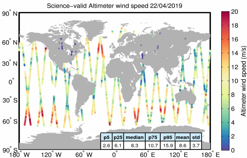
Figure 34. Geographical distribution of science-valid wind data over oceans and lakes for 22/04/2019. The statistical values shown in the table refer to the wind in m/s and are calculated over all measurements shown in the figure. Gray circles denote records that have been rejected based on the editing criteria described in Table 5.
