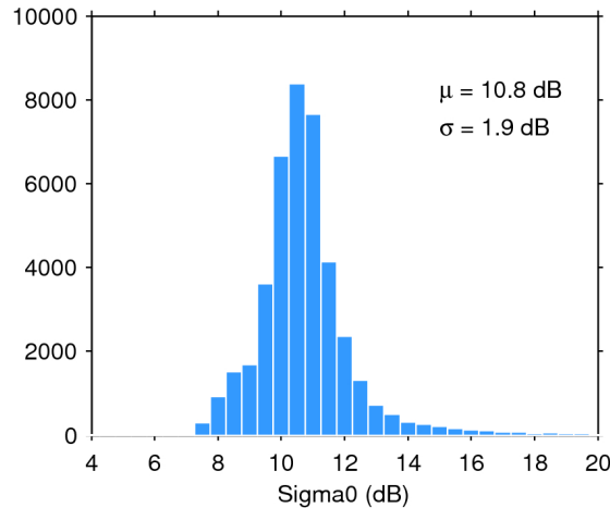
Figure 25. Histogram of flag-valid sigma0 over oceans and lakes for 22/04/2019. The mean ( \mu ) and standard deviation ( \sigma ) are also shown. Note that values outside [4 20] dB are excluded from the histogram for the sake of readability but not from the computation of \mu and \sigma .
