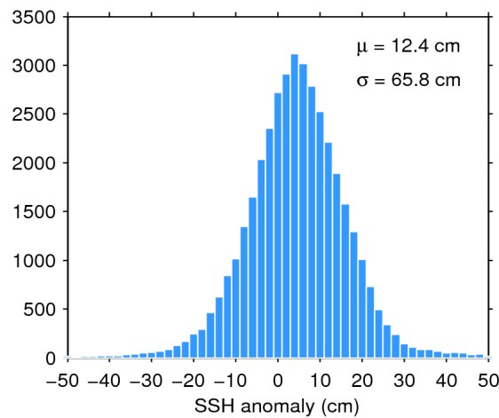
Figure 7. Histogram of flag-valid SSH anomaly over oceans and lakes for 22/04/2019. The mean ( \mu ) and standard deviation ( \sigma ) are also shown. Note that values outside [-50 50] cm are excluded from the histogram for the sake of readability but not from the computation of \mu and \sigma .
