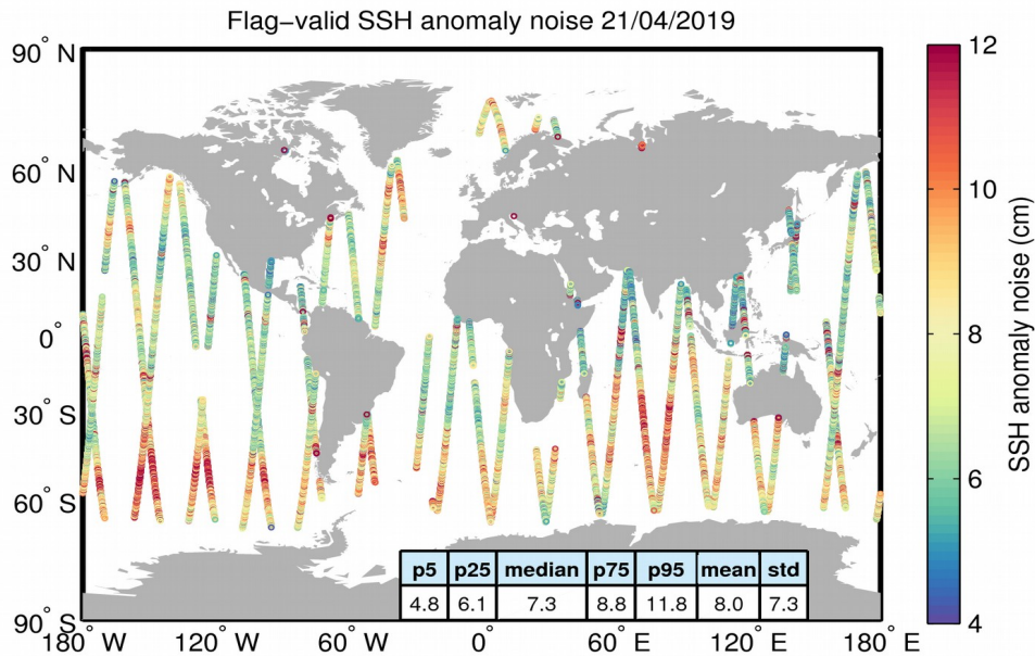
Figure 8. Geographical distribution of flag-valid 20-Hz SSH anomaly measurement noise over oceans and lakes for 21/04/2019. The statistical values shown in the table refer to the SSH anomaly noise and are calculated over all measurements shown in the figure.
