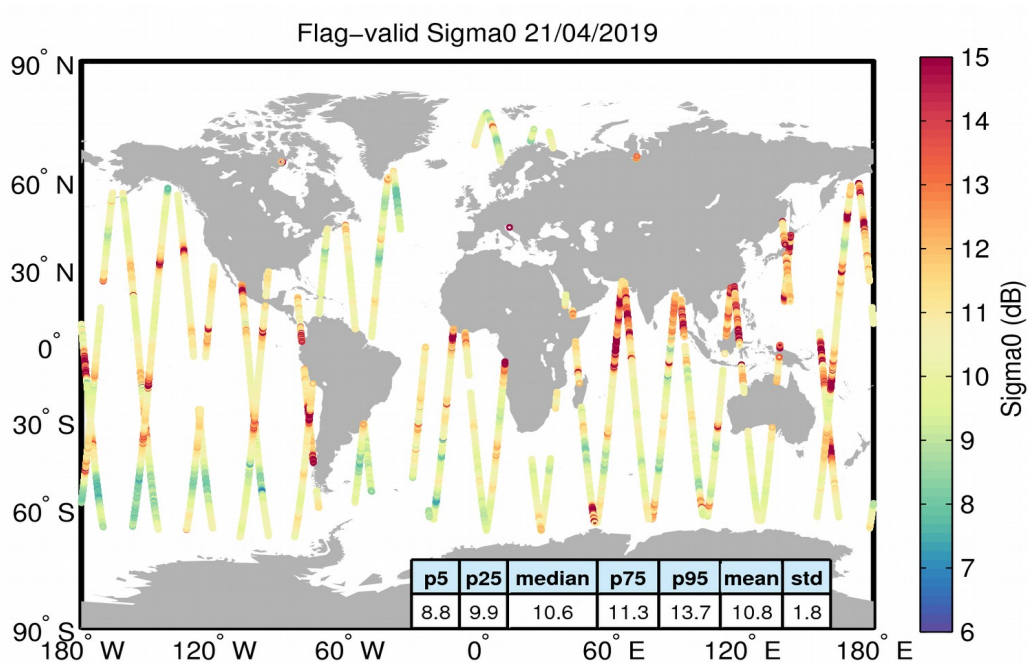
Figure 23. Geographical distribution of flag-valid sigma0 data over oceans and lakes for 21/04/2019. The statistical values shown in the table refer to the sigma0 in dB and are calculated over all measurements shown in the figure.
