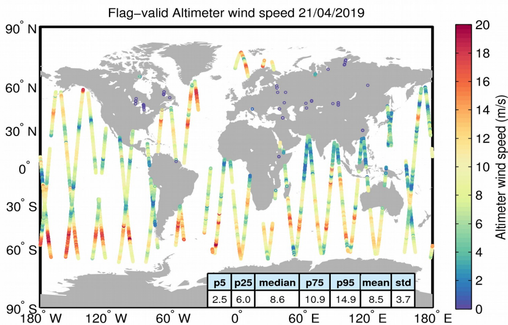
Figure 31. Geographical distribution of flag-valid wind data over oceans and lakes for 21/04/2019. The statistical values shown in the table refer to the wind in m/s and are calculated over all measurements shown in the figure.
