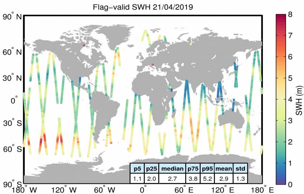
Figure 15. Geographical distribution of flag-valid SWH data over oceans and lakes for 21/04/2019. The statistical values shown in the table refer to the SWH in m and are calculated over all measurements shown in the figure.
