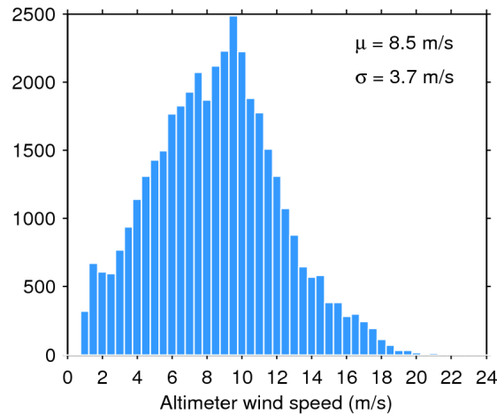
Figure 33. Histogram of flag-valid wind over oceans and lakes for 21/04/2019. The mean ( \mu ) and standard deviation ( \sigma ) are also shown. Note that values larger than 24 m/s are excluded from the histogram for the sake of readability but not from the computation of \mu and \sigma .
