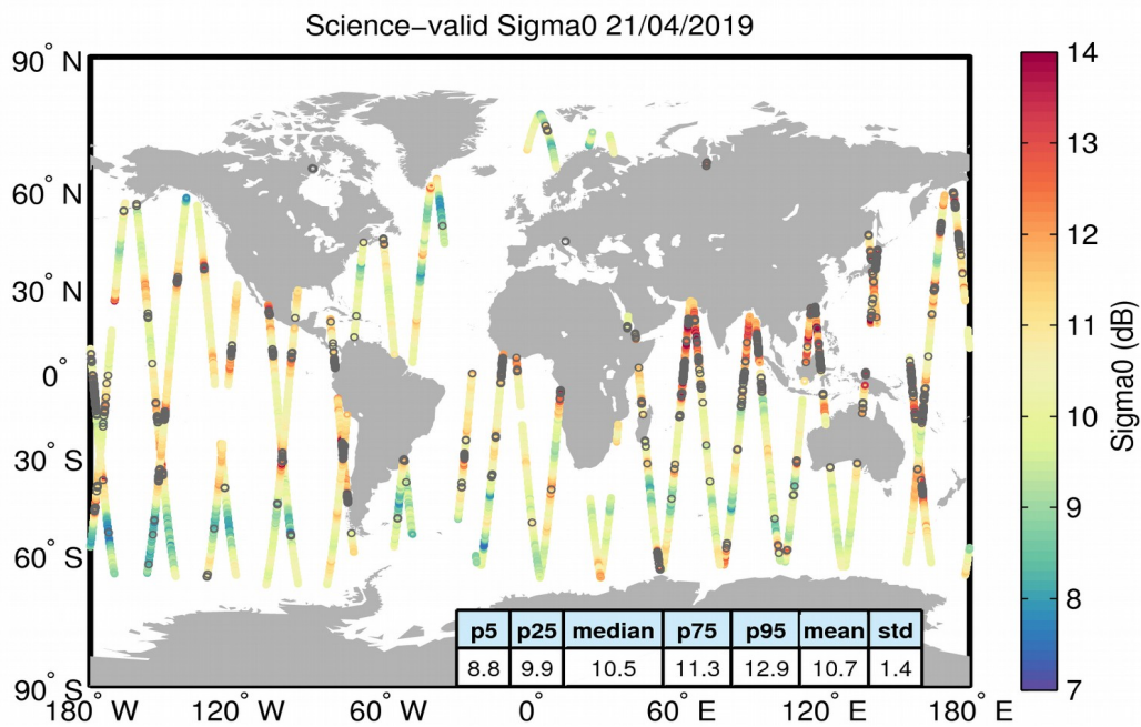
Figure 27. Geographical distribution of science-valid sigma0 data over oceans and lakes for 21/04/2019. The statistical values shown in the table refer to the sigma0 in dB and are calculated over all measurements shown in the figure. Gray circles denote records that have been rejected based on the editing criteria described in Table 4.
