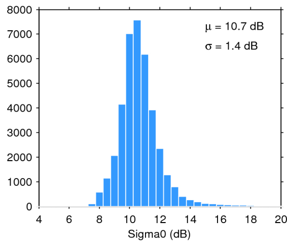
Figure 28. Histogram of science-valid sigma0 over oceans and lakes for 21/04/2019. The mean ( \mu ) and standard deviation ( \sigma ) are also shown. Note that values outside [4 20] dB are excluded from the histogram for the sake of readability but not from the computation of \mu and \sigma .
