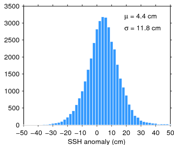
Figure 11. Histogram of science-valid SSH anomaly over oceans and lakes for 21/04/2019. The mean ( \mu ) and standard deviation ( \sigma ) are also shown. Note that values outside [-50 50] cm are excluded from the histogram for the sake of readability but not from the computation of \mu and \sigma .
