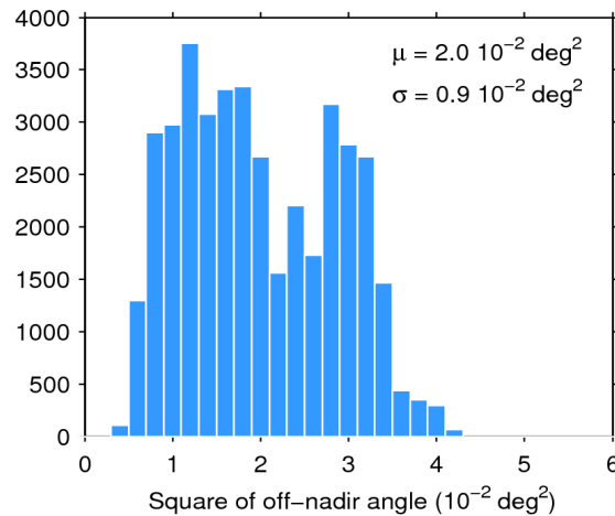
Figure 39. Histogram of flag-valid mispointing over oceans and lakes for 21/04/2019. The mean ( \mu ) and standard deviation ( \sigma ) are also shown. Note that values larger than 6 \cdot 10^{-2} \text{ deg}^2 are excluded from the histogram for the sake of readability but not from the computation of \mu and \sigma .
