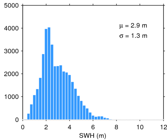
Figure 17. Histogram of flag-valid SWH over oceans and lakes for 21/04/2019. The mean ( \mu ) and standard deviation ( \sigma ) are also shown. Note that values larger than 12 m are excluded from the histogram for the sake of readability but not from the computation of \mu and \sigma .
