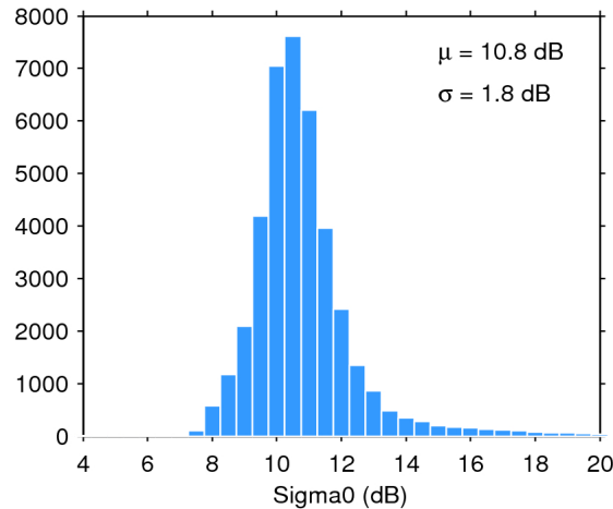
Figure 25. Histogram of flag-valid sigma0 over oceans and lakes for 21/04/2019. The mean ( \mu ) and standard deviation ( \sigma ) are also shown. Note that values outside [4 20] dB are excluded from the histogram for the sake of readability but not from the computation of \mu and \sigma .
