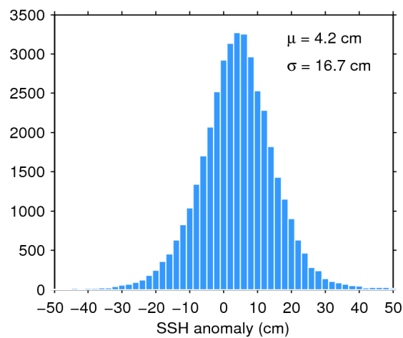
Figure 7. Histogram of flag-valid SSH anomaly over oceans and lakes for 21/04/2019. The mean ( \mu ) and standard deviation ( \sigma ) are also shown. Note that values outside [-50 50] cm are excluded from the histogram for the sake of readability but not from the computation of \mu and \sigma .
