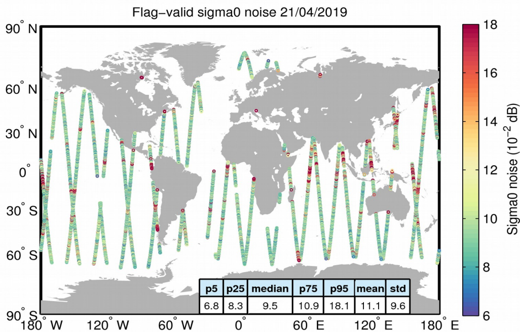
Figure 26. Geographical distribution of flag-valid 20-Hz sigma0 measurement noise over oceans and lakes for 21/04/2019. The statistical values shown in the table refer to the sigma0 noise and are calculated over all measurements shown in the figure.
