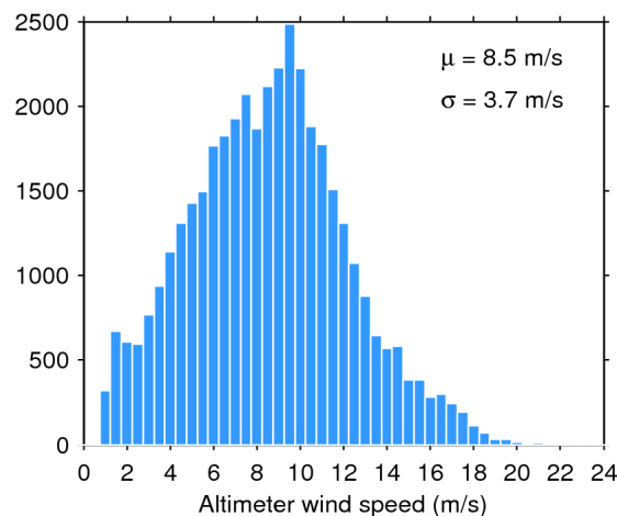
Figure 35. Histogram of science-valid wind over oceans and lakes for 21/04/2019. The mean ( \mu ) and standard deviation ( \sigma ) are also shown. Note that values larger than 24 m/s are excluded from the histogram for the sake of readability but not from the computation of \mu and \sigma .
