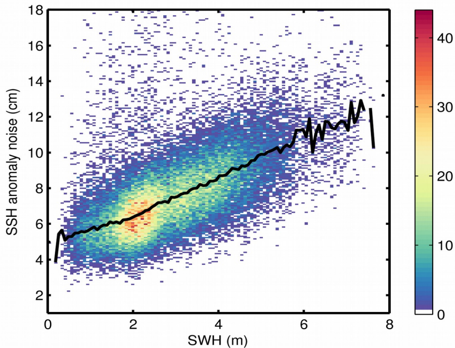
Figure 9. 2D histogram showing flag-valid SSH anomaly noise as a function of SWH for 21/04/2019. The black line denotes the median SSH anomaly noise as a function of SWH.
