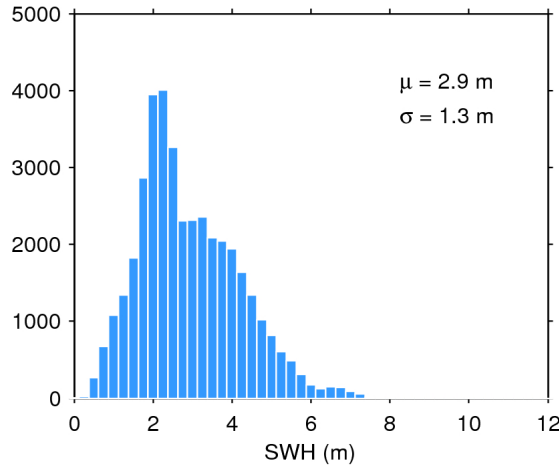
Figure 20. Histogram of science-valid SWH over oceans and lakes for 21/04/2019. The mean ( \mu ) and standard deviation ( \sigma ) are also shown. Note that values larger than 12 m are excluded from the histogram for the sake of readability but not from the computation of \mu and \sigma .
