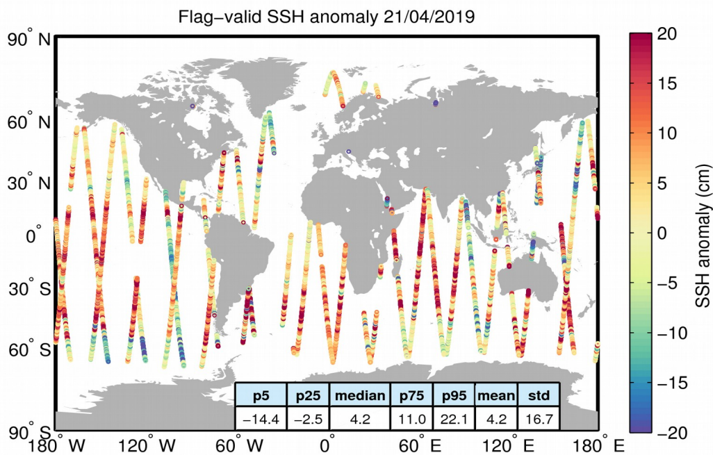
Figure 5. Geographical distribution of flag-valid 1-Hz SSH anomaly data over oceans and lakes for 21/04/2019. The statistical values shown in the table refer to the SSH anomaly in cm and are calculated over all measurements shown in the figure.
