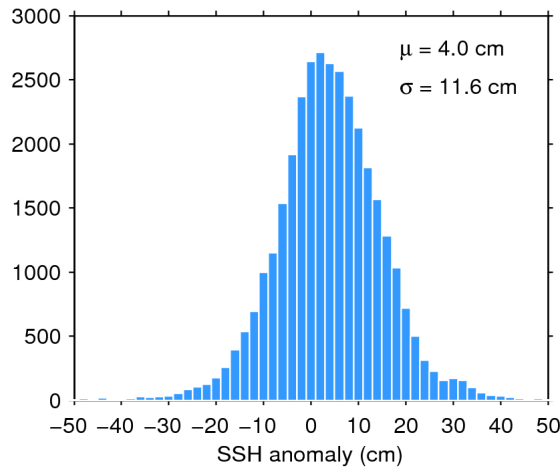
Figure 11. Histogram of science-valid SSH anomaly over oceans and lakes for 20/04/2019. The mean ( \mu ) and standard deviation ( \sigma ) are also shown. Note that values outside [-50 50] cm are excluded from the histogram for the sake of readability but not from the computation of \mu and \sigma .
