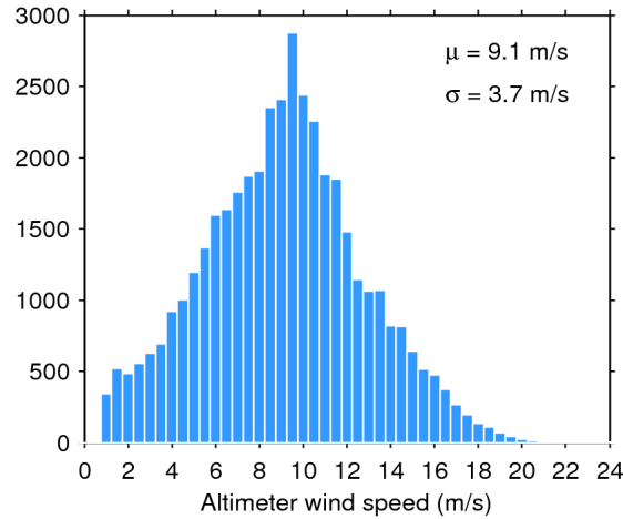
Figure 33. Histogram of flag-valid wind over oceans and lakes for 20/04/2019. The mean ( \mu ) and standard deviation ( \sigma ) are also shown. Note that values larger than 24 m/s are excluded from the histogram for the sake of readability but not from the computation of \mu and \sigma .
