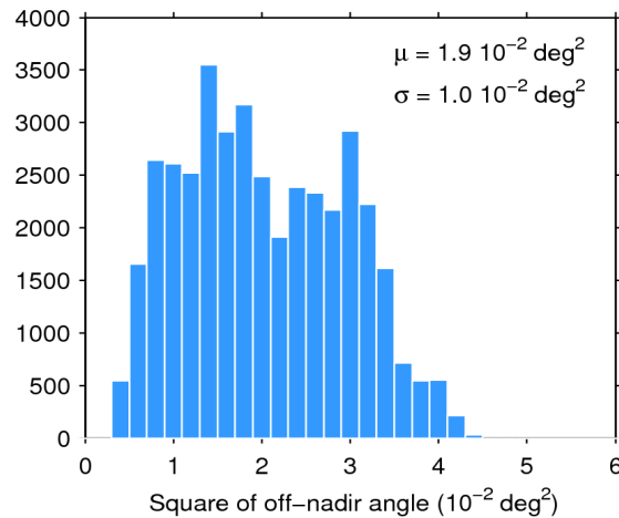
Figure 39. Histogram of flag-valid mispointing over oceans and lakes for 20/04/2019. The mean ( \mu ) and standard deviation ( \sigma ) are also shown. Note that values larger than 6 \cdot 10^{-2} \text{ deg}^2 are excluded from the histogram for the sake of readability but not from the computation of \mu and \sigma .
