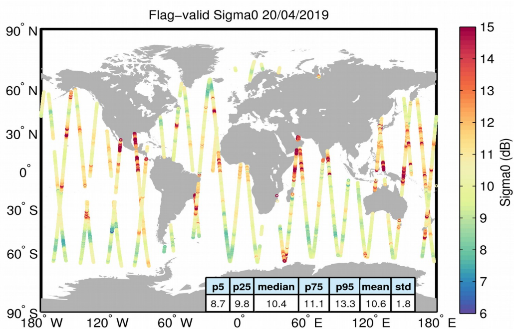
Figure 23. Geographical distribution of flag-valid sigma0 data over oceans and lakes for 20/04/2019. The statistical values shown in the table refer to the sigma0 in dB and are calculated over all measurements shown in the figure.
