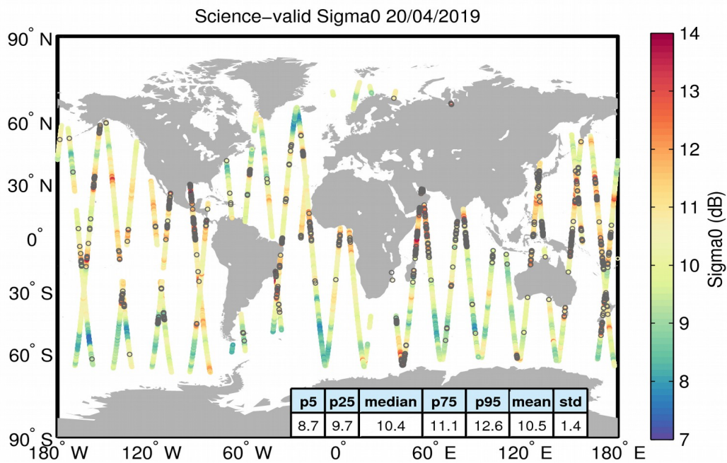
Figure 27. Geographical distribution of science-valid sigma0 data over oceans and lakes for 20/04/2019. The statistical values shown in the table refer to the sigma0 in dB and are calculated over all measurements shown in the figure. Gray circles denote records that have been rejected based on the editing criteria described in Table 4.
