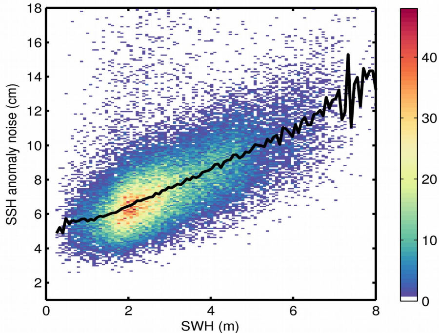
Figure 9. 2D histogram showing flag-valid SSH anomaly noise as a function of SWH for 20/04/2019. The black line denotes the median SSH anomaly noise as a function of SWH.
