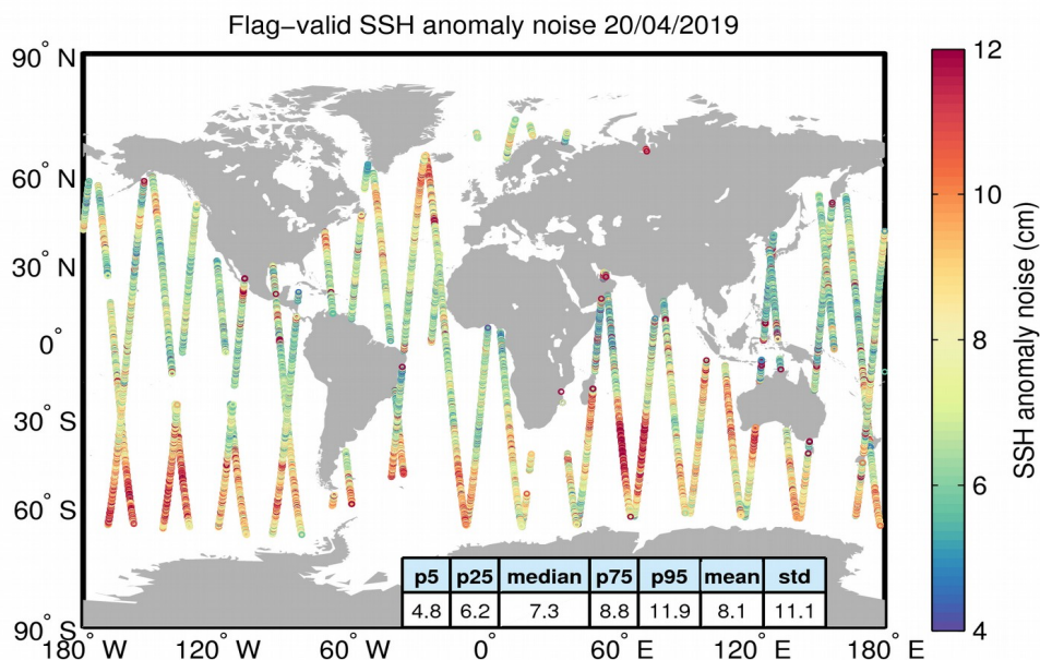
Figure 8. Geographical distribution of flag-valid 20-Hz SSH anomaly measurement noise over oceans and lakes for 20/04/2019. The statistical values shown in the table refer to the SSH anomaly noise and are calculated over all measurements shown in the figure.
