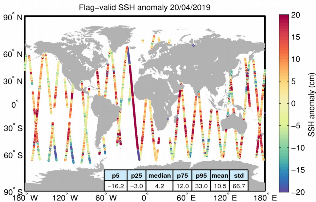
Figure 5. Geographical distribution of flag-valid 1-Hz SSH anomaly data over oceans and lakes for 20/04/2019. The statistical values shown in the table refer to the SSH anomaly in cm and are calculated over all measurements shown in the figure.
