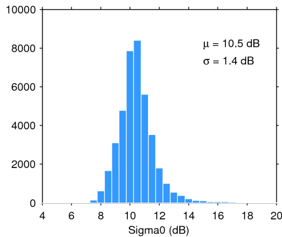
Figure 28. Histogram of science-valid sigma0 over oceans and lakes for 20/04/2019. The mean ( \mu ) and standard deviation ( \sigma ) are also shown. Note that values outside [4 20] dB are excluded from the histogram for the sake of readability but not from the computation of \mu and \sigma .
