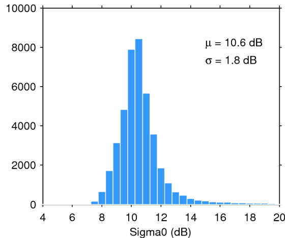
Figure 25. Histogram of flag-valid sigma0 over oceans and lakes for 20/04/2019. The mean ( \mu ) and standard deviation ( \sigma ) are also shown. Note that values outside [4 20] dB are excluded from the histogram for the sake of readability but not from the computation of \mu and \sigma .
