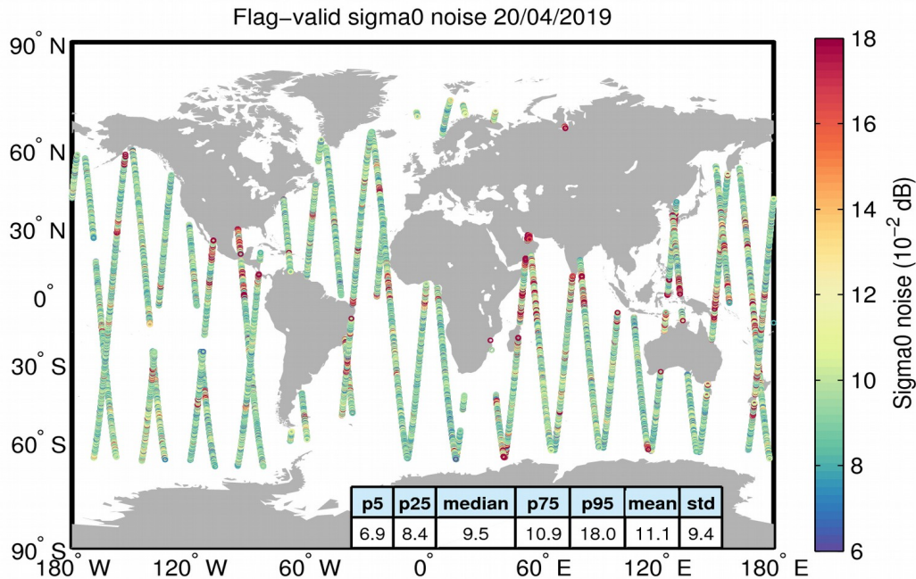
Figure 26. Geographical distribution of flag-valid 20-Hz sigma0 measurement noise over oceans and lakes for 20/04/2019. The statistical values shown in the table refer to the sigma0 noise and are calculated over all measurements shown in the figure.
