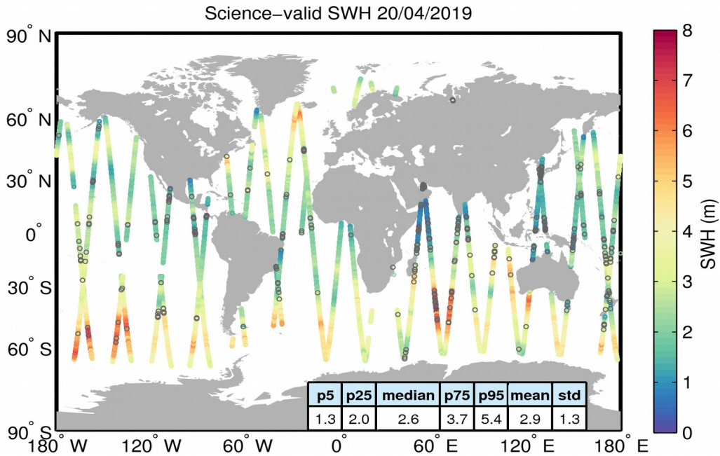
Figure 19. Geographical distribution of science-valid SWH data over oceans and lakes for 20/04/2019. The statistical values shown in the table refer to the SWH in m and are calculated over all measurements shown in the figure. Gray circles denote records that have been rejected based on the editing criteria described in Table 3.
