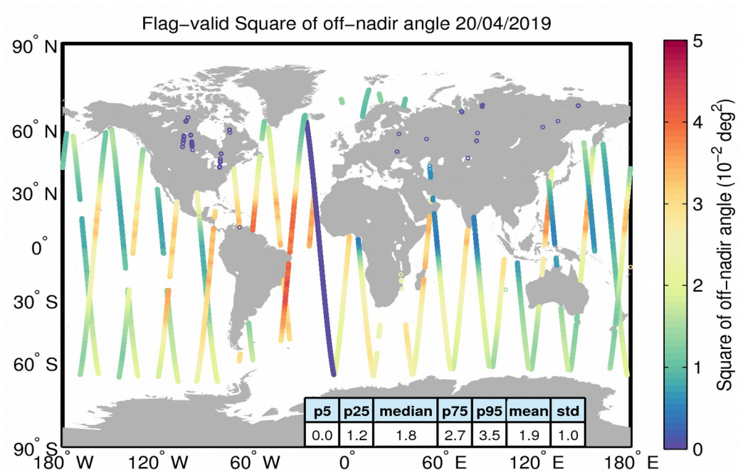
Figure 37. Geographical distribution of flag-valid mispointing data over oceans and lakes for 20/04/2019. The statistical values shown in the table refer to the mispointing in 10^{-2} \text{ deg}^2 and are calculated over all measurements shown in the figure.
