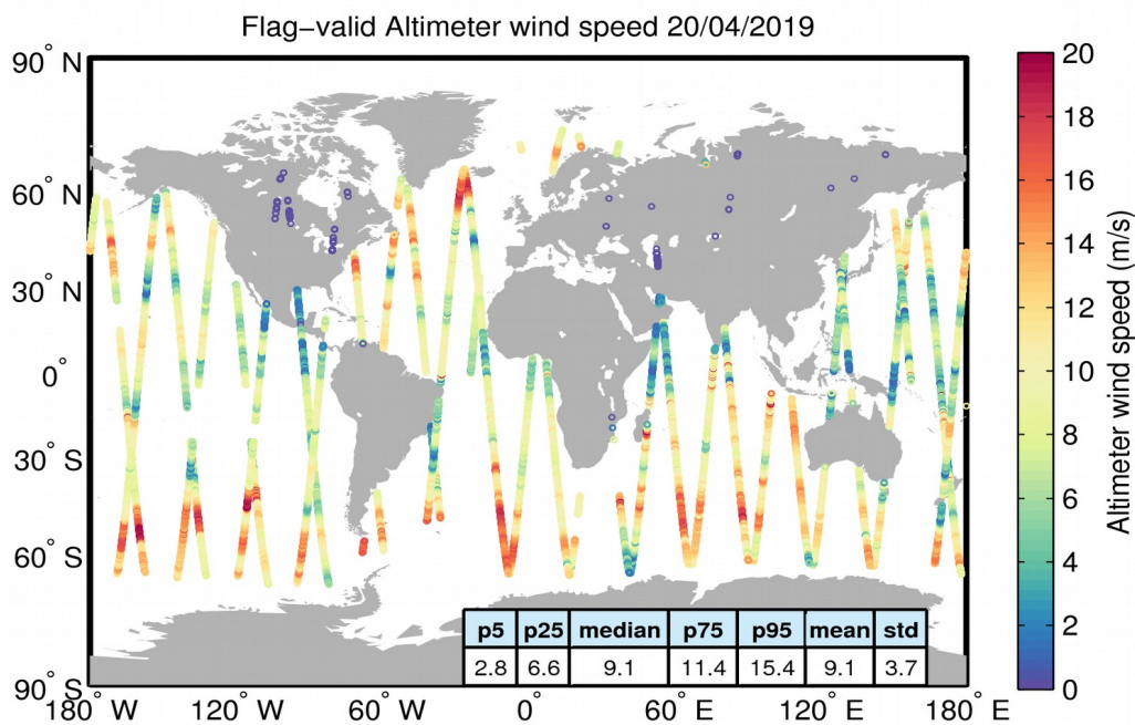
Figure 31. Geographical distribution of flag-valid wind data over oceans and lakes for 20/04/2019. The statistical values shown in the table refer to the wind in m/s and are calculated over all measurements shown in the figure.
