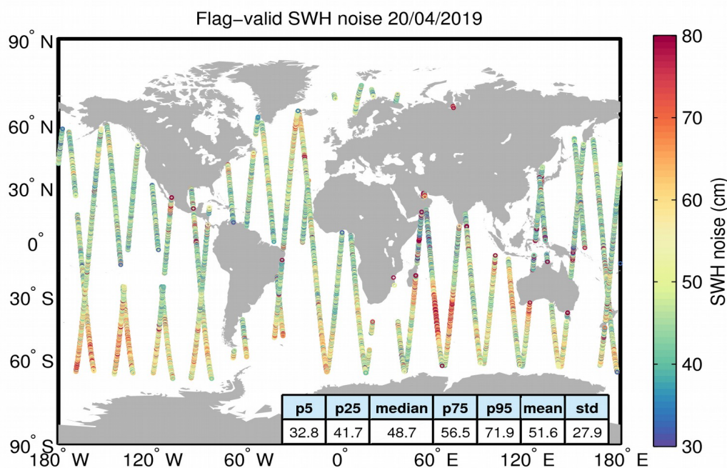
Figure 18. Geographical distribution of flag-valid 20-Hz SWH measurement noise over oceans and lakes for 20/04/2019. The statistical values shown in the table refer to the SWH noise and are calculated over all measurements shown in the figure.
