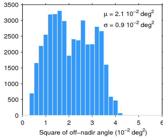
Figure 39. Histogram of flag-valid mispointing over oceans and lakes for 19/04/2019. The mean ( \mu ) and standard deviation ( \sigma ) are also shown. Note that values larger than 6 \cdot 10^{-2} \text{ deg}^2 are excluded from the histogram for the sake of readability but not from the computation of \mu and \sigma .
