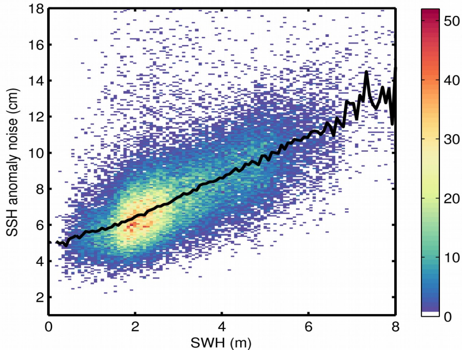
Figure 9. 2D histogram showing flag-valid SSH anomaly noise as a function of SWH for 19/04/2019. The black line denotes the median SSH anomaly noise as a function of SWH.
