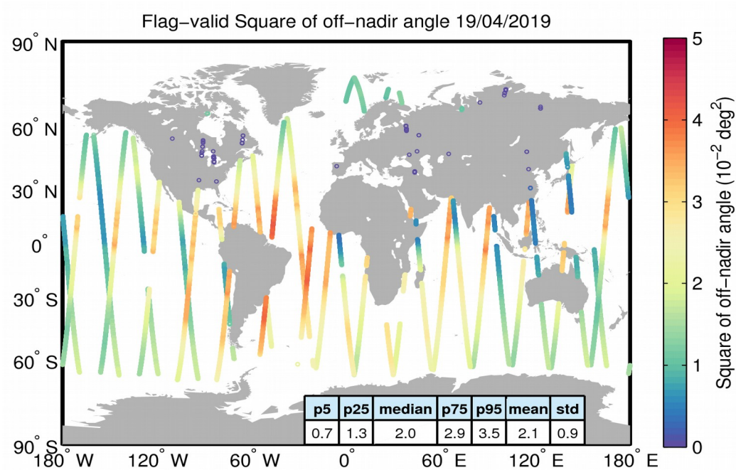
Figure 37. Geographical distribution of flag-valid mispointing data over oceans and lakes for 19/04/2019. The statistical values shown in the table refer to the mispointing in 10^{-2} deg 2 and are calculated over all measurements shown in the figure.
