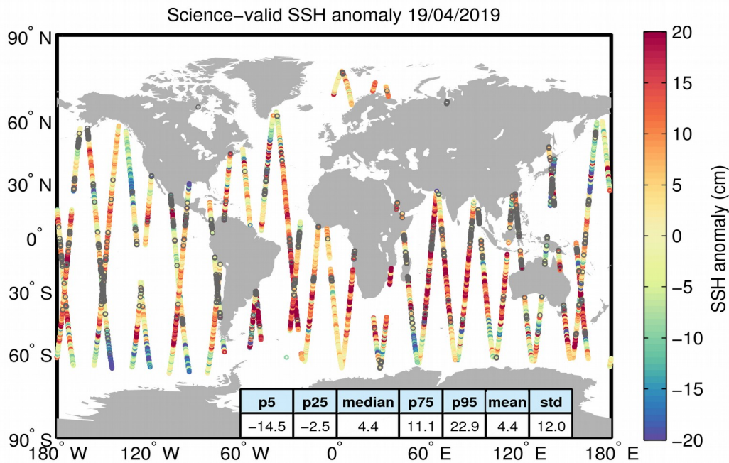
Figure 10. Geographical distribution of science-valid SSH anomaly data over oceans and lakes for 19/04/2019. The statistical values shown in the table refer to the SSH anomaly in cm and are calculated over all measurements shown in the figure. Gray circles denote records that have been rejected based on the editing criteria described in Table 2.
