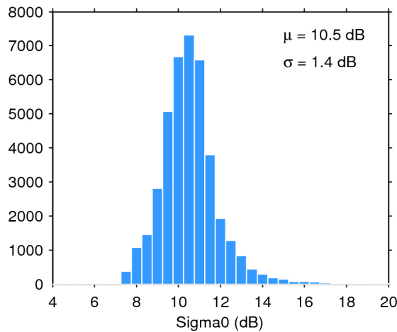
Figure 28. Histogram of science-valid sigma0 over oceans and lakes for 19/04/2019. The mean ( \mu ) and standard deviation ( \sigma ) are also shown. Note that values outside [4 20] dB are excluded from the histogram for the sake of readability but not from the computation of \mu and \sigma .
