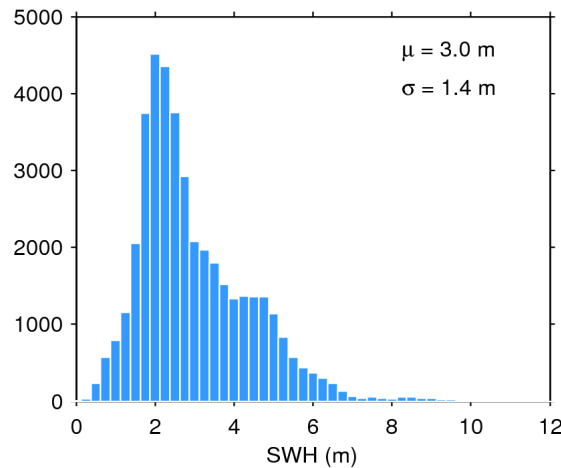
Figure 20. Histogram of science-valid SWH over oceans and lakes for 19/04/2019. The mean ( \mu ) and standard deviation ( \sigma ) are also shown. Note that values larger than 12 m are excluded from the histogram for the sake of readability but not from the computation of \mu and \sigma .
