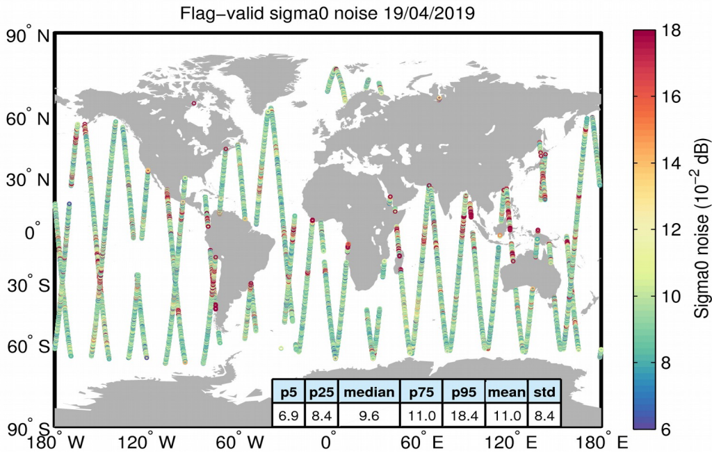
Figure 26. Geographical distribution of flag-valid 20-Hz sigma0 measurement noise over oceans and lakes for 19/04/2019. The statistical values shown in the table refer to the sigma0 noise and are calculated over all measurements shown in the figure.
