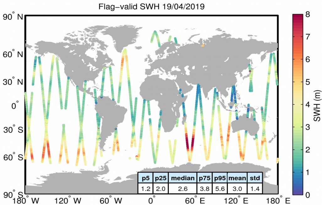
Figure 15. Geographical distribution of flag-valid SWH data over oceans and lakes for 19/04/2019. The statistical values shown in the table refer to the SWH in m and are calculated over all measurements shown in the figure.
