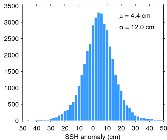
Figure 11. Histogram of science-valid SSH anomaly over oceans and lakes for 19/04/2019. The mean ( \mu ) and standard deviation ( \sigma ) are also shown. Note that values outside [-50 50] cm are excluded from the histogram for the sake of readability but not from the computation of \mu and \sigma .
