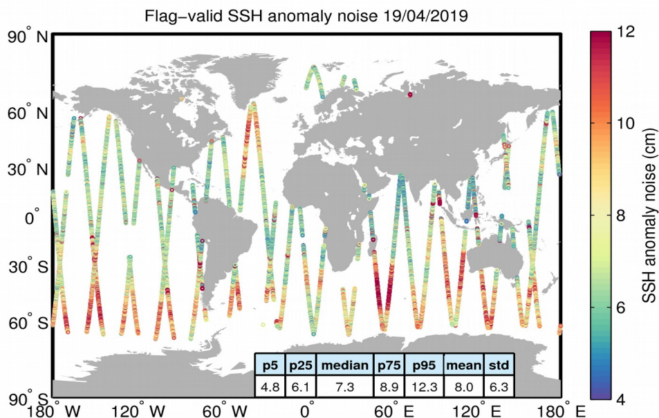
Figure 8. Geographical distribution of flag-valid 20-Hz SSH anomaly measurement noise over oceans and lakes for 19/04/2019. The statistical values shown in the table refer to the SSH anomaly noise and are calculated over all measurements shown in the figure.
