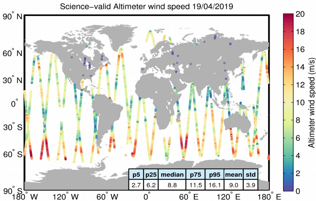
Figure 34. Geographical distribution of science-valid wind data over oceans and lakes for 19/04/2019. The statistical values shown in the table refer to the wind in m/s and are calculated over all measurements shown in the figure. Gray circles denote records that have been rejected based on the editing criteria described in Table 5.
