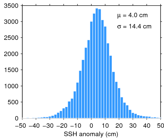
Figure 7. Histogram of flag-valid SSH anomaly over oceans and lakes for 19/04/2019. The mean ( \mu ) and standard deviation ( \sigma ) are also shown. Note that values outside [-50\ 50] cm are excluded from the histogram for the sake of readability but not from the computation of \mu and \sigma .
