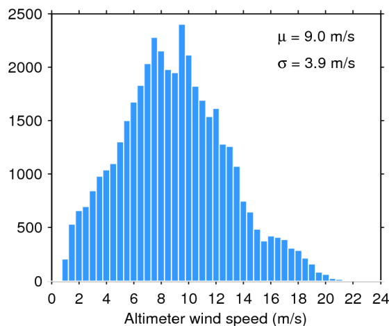
Figure 35. Histogram of science-valid wind over oceans and lakes for 19/04/2019. The mean ( \mu ) and standard deviation ( \sigma ) are also shown. Note that values larger than 24 m/s are excluded from the histogram for the sake of readability but not from the computation of \mu and \sigma .
