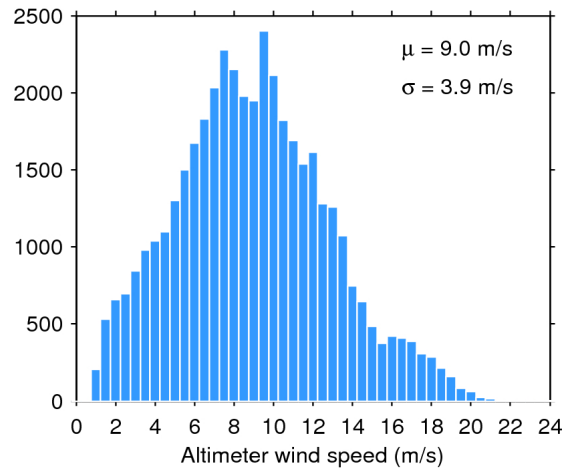
Figure 33. Histogram of flag-valid wind over oceans and lakes for 19/04/2019. The mean ( \mu ) and standard deviation ( \sigma ) are also shown. Note that values larger than 24 m/s are excluded from the histogram for the sake of readability but not from the computation of \mu and \sigma .
