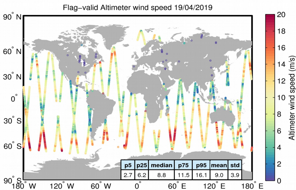
Figure 31. Geographical distribution of flag-valid wind data over oceans and lakes for 19/04/2019. The statistical values shown in the table refer to the wind in m/s and are calculated over all measurements shown in the figure.
