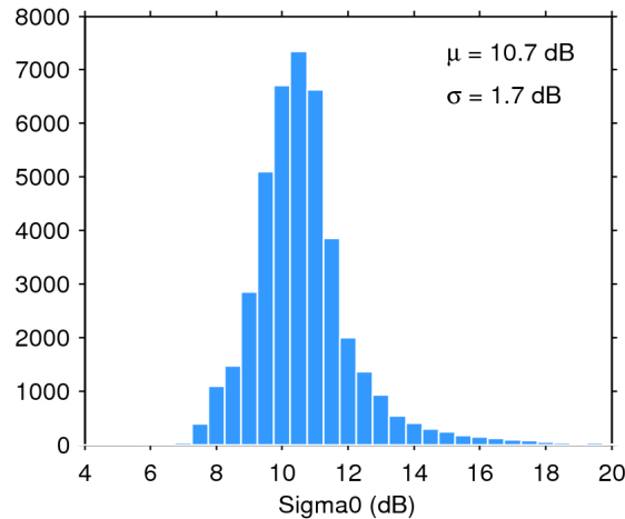
Figure 25. Histogram of flag-valid sigma0 over oceans and lakes for 19/04/2019. The mean ( \mu ) and standard deviation ( \sigma ) are also shown. Note that values outside [4 20] dB are excluded from the histogram for the sake of readability but not from the computation of \mu and \sigma .
