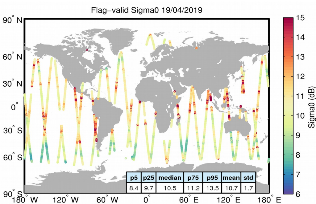
Figure 23. Geographical distribution of flag-valid sigma0 data over oceans and lakes for 19/04/2019. The statistical values shown in the table refer to the sigma0 in dB and are calculated over all measurements shown in the figure.
