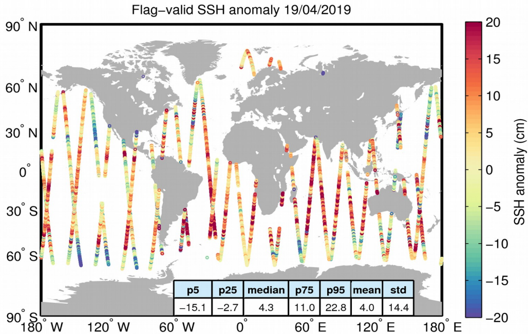
Figure 5. Geographical distribution of flag-valid 1-Hz SSH anomaly data over oceans and lakes for 19/04/2019. The statistical values shown in the table refer to the SSH anomaly in cm and are calculated over all measurements shown in the figure.
