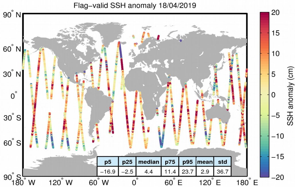
Figure 5. Geographical distribution of flag-valid 1-Hz SSH anomaly data over oceans and lakes for 18/04/2019. The statistical values shown in the table refer to the SSH anomaly in cm and are calculated over all measurements shown in the figure.
