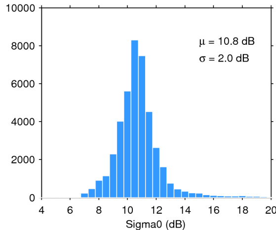
Figure 25. Histogram of flag-valid sigma0 over oceans and lakes for 18/04/2019. The mean ( \mu ) and standard deviation ( \sigma ) are also shown. Note that values outside [4 20] dB are excluded from the histogram for the sake of readability but not from the computation of \mu and \sigma .
