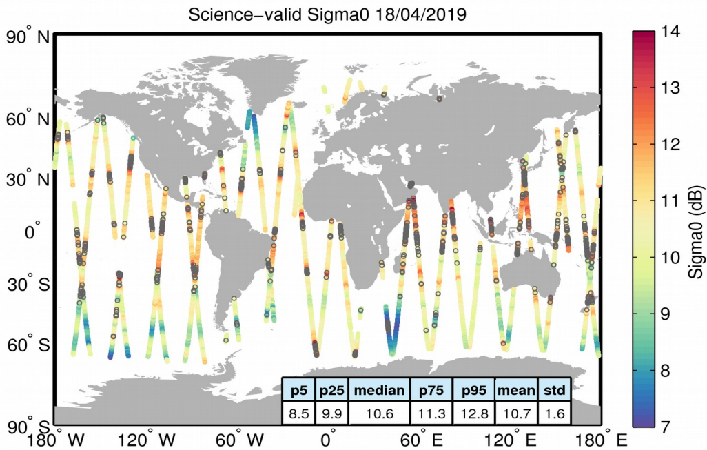
Figure 27. Geographical distribution of science-valid sigma0 data over oceans and lakes for 18/04/2019. The statistical values shown in the table refer to the sigma0 in dB and are calculated over all measurements shown in the figure. Gray circles denote records that have been rejected based on the editing criteria described in Table 4.
