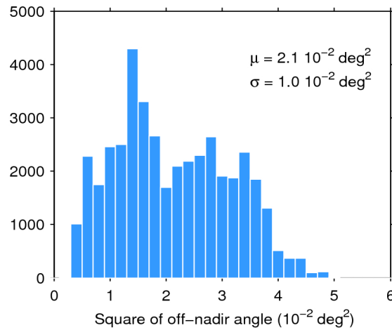
Figure 39. Histogram of flag-valid mispointing over oceans and lakes for 18/04/2019. The mean ( \mu ) and standard deviation ( \sigma ) are also shown. Note that values larger than 6 \cdot 10^{-2} \text{ deg}^2 are excluded from the histogram for the sake of readability but not from the computation of \mu and \sigma .
