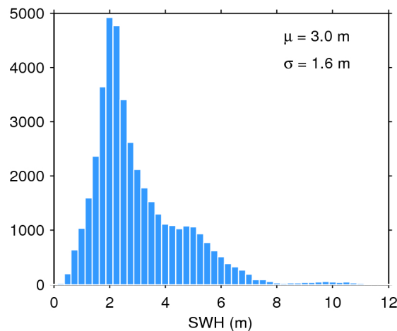
Figure 17. Histogram of flag-valid SWH over oceans and lakes for 18/04/2019. The mean ( \mu ) and standard deviation ( \sigma ) are also shown. Note that values larger than 12 m are excluded from the histogram for the sake of readability but not from the computation of \mu and \sigma .
