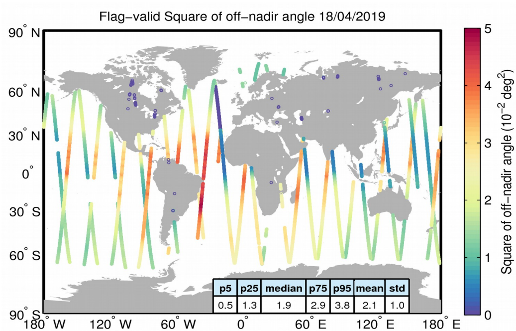
Figure 37. Geographical distribution of flag-valid mispointing data over oceans and lakes for 18/04/2019. The statistical values shown in the table refer to the mispointing in 10^{-2} deg 2 and are calculated over all measurements shown in the figure.
