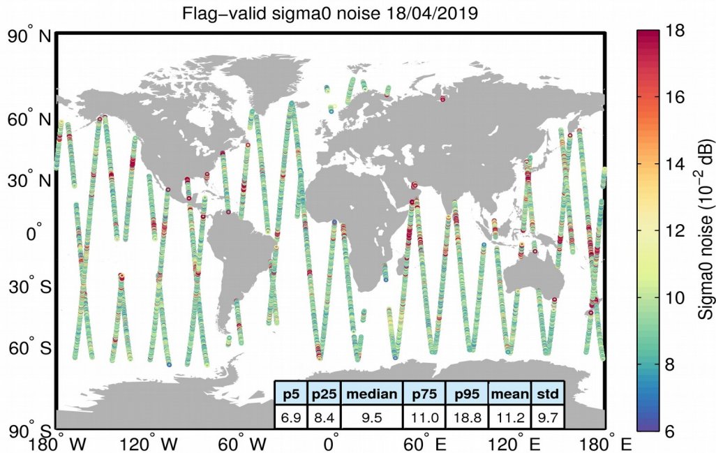
Figure 26. Geographical distribution of flag-valid 20-Hz sigma0 measurement noise over oceans and lakes for 18/04/2019. The statistical values shown in the table refer to the sigma0 noise and are calculated over all measurements shown in the figure.
