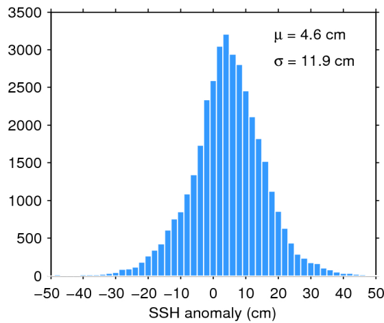
Figure 11. Histogram of science-valid SSH anomaly over oceans and lakes for 18/04/2019. The mean ( \mu ) and standard deviation ( \sigma ) are also shown. Note that values outside [-50 50] cm are excluded from the histogram for the sake of readability but not from the computation of \mu and \sigma .
