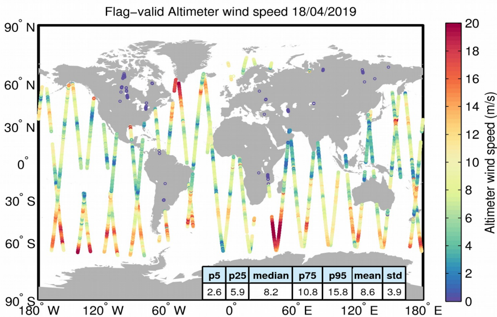
Figure 31. Geographical distribution of flag-valid wind data over oceans and lakes for 18/04/2019. The statistical values shown in the table refer to the wind in m/s and are calculated over all measurements shown in the figure.
