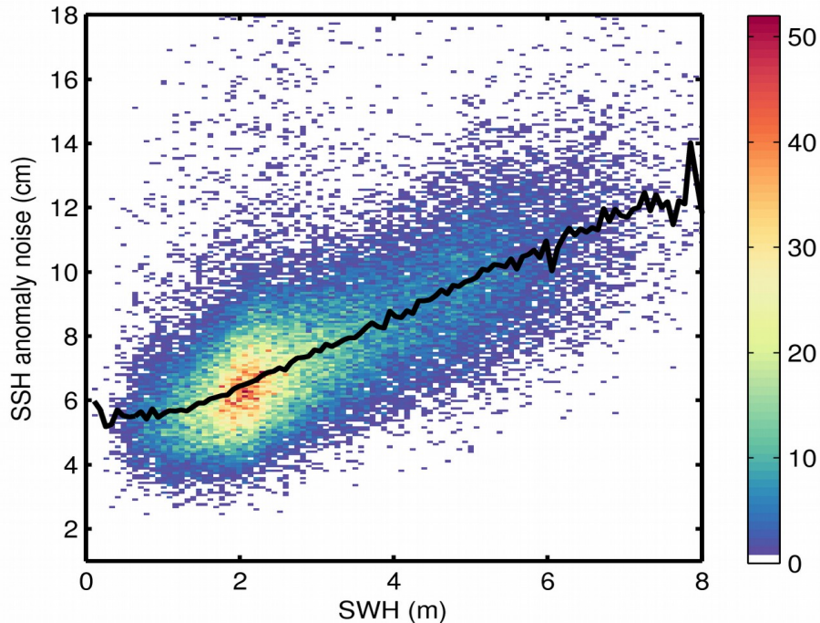
Figure 9. 2D histogram showing flag-valid SSH anomaly noise as a function of SWH for 18/04/2019. The black line denotes the median SSH anomaly noise as a function of SWH.
