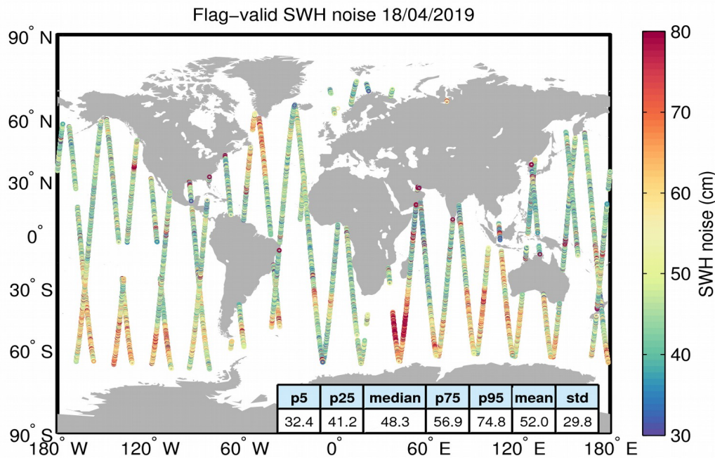
Figure 18. Geographical distribution of flag-valid 20-Hz SWH measurement noise over oceans and lakes for 18/04/2019. The statistical values shown in the figure refer to the SWH noise and are calculated over all measurements shown in the figure.
