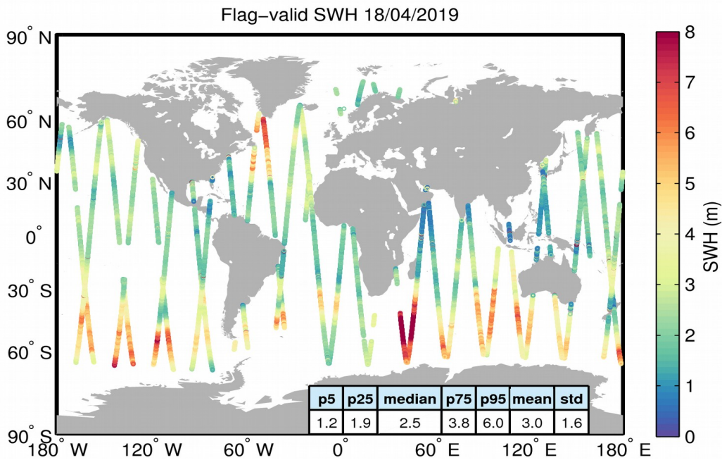
Figure 15. Geographical distribution of flag-valid SWH data over oceans and lakes for 18/04/2019. The statistical values shown in the table refer to the SWH in m and are calculated over all measurements shown in the figure.
