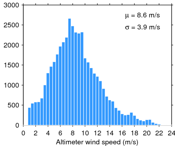
Figure 33. Histogram of flag-valid wind over oceans and lakes for 18/04/2019. The mean ( \mu ) and standard deviation ( \sigma ) are also shown. Note that values larger than 24 m/s are excluded from the histogram for the sake of readability but not from the computation of \mu and \sigma .
