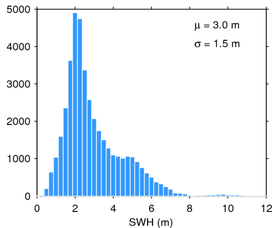
Figure 20. Histogram of science-valid SWH over oceans and lakes for 18/04/2019. The mean ( \mu ) and standard deviation ( \sigma ) are also shown. Note that values larger than 12 m are excluded from the histogram for the sake of readability but not from the computation of \mu and \sigma .
