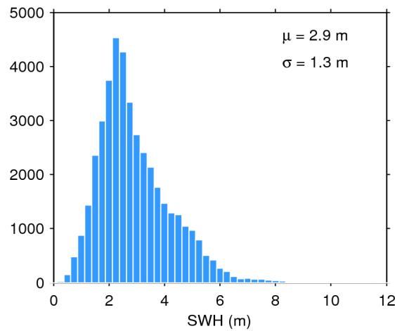
Figure 17. Histogram of flag-valid SWH over oceans and lakes for 16/04/2019. The mean ( \mu ) and standard deviation ( \sigma ) are also shown. Note that values larger than 12 m are excluded from the histogram for the sake of readability but not from the computation of \mu and \sigma .
