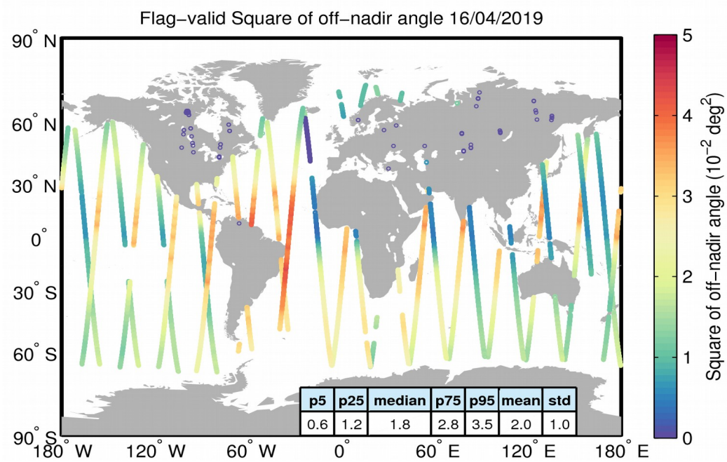
Figure 37. Geographical distribution of flag-valid mispointing data over oceans and lakes for 16/04/2019. The statistical values shown in the table refer to the mispointing in 10^{-2} \text{ deg}^2 and are calculated over all measurements shown in the figure.
