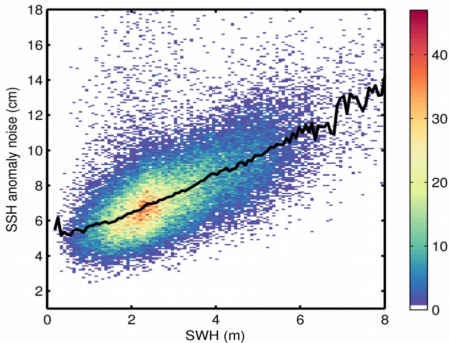
Figure 9. 2D histogram showing flag-valid SSH anomaly noise as a function of SWH for 16/04/2019. The black line denotes the median SSH anomaly noise as a function of SWH.
