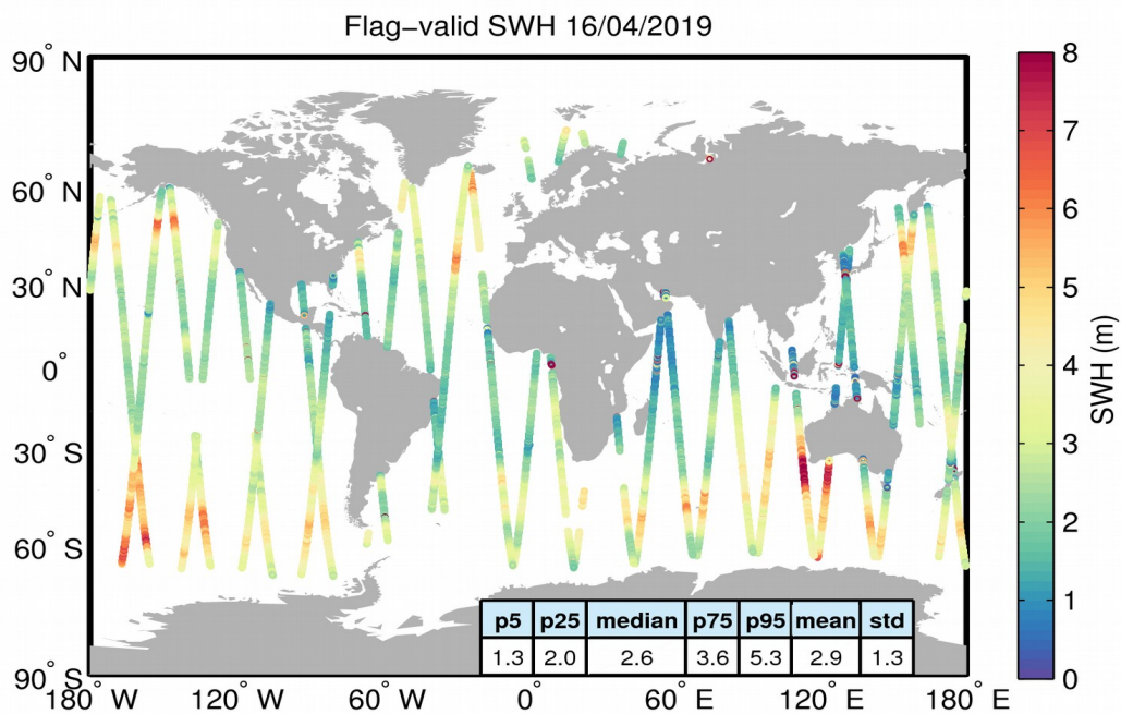
Figure 15. Geographical distribution of flag-valid SWH data over oceans and lakes for 16/04/2019. The statistical values shown in the table refer to the SWH in m and are calculated over all measurements shown in the figure.
