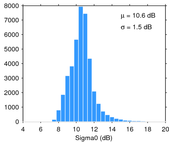
Figure 28. Histogram of science-valid sigma0 over oceans and lakes for 16/04/2019. The mean ( \mu ) and standard deviation ( \sigma ) are also shown. Note that values outside [4 20] dB are excluded from the histogram for the sake of readability but not from the computation of \mu and \sigma .
