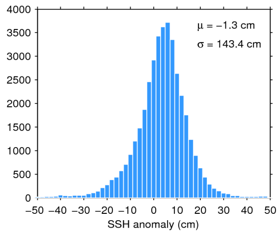
Figure 7. Histogram of flag-valid SSH anomaly over oceans and lakes for 16/04/2019. The mean ( \mu ) and standard deviation ( \sigma ) are also shown. Note that values outside [-50 50] cm are excluded from the histogram for the sake of readability but not from the computation of \mu and \sigma .
