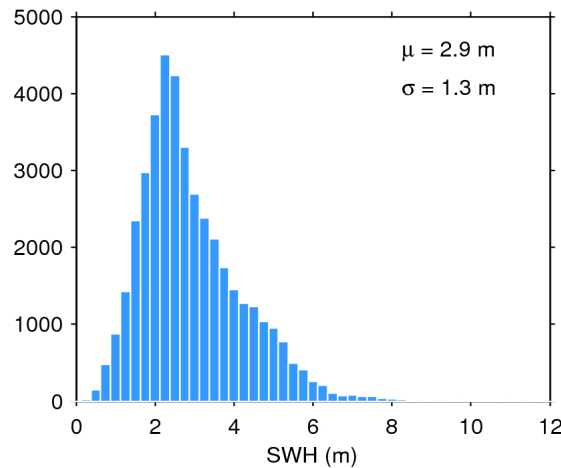
Figure 20. Histogram of science-valid SWH over oceans and lakes for 16/04/2019. The mean ( \mu ) and standard deviation ( \sigma ) are also shown. Note that values larger than 12 m are excluded from the histogram for the sake of readability but not from the computation of \mu and \sigma .
