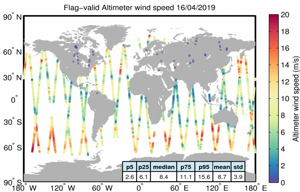
Figure 31. Geographical distribution of flag-valid wind data over oceans and lakes for 16/04/2019. The statistical values shown in the table refer to the wind in m/s and are calculated over all measurements shown in the figure.
