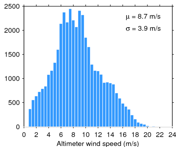
Figure 35. Histogram of science-valid wind over oceans and lakes for 16/04/2019. The mean ( \mu ) and standard deviation ( \sigma ) are also shown. Note that values larger than 24 m/s are excluded from the histogram for the sake of readability but not from the computation of \mu and \sigma .
