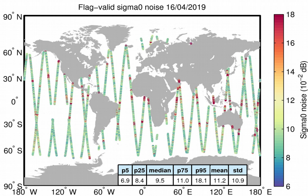
Figure 26. Geographical distribution of flag-valid 20-Hz sigma0 measurement noise over oceans and lakes for 16/04/2019. The statistical values shown in the table refer to the sigma0 noise and are calculated over all measurements shown in the figure.
