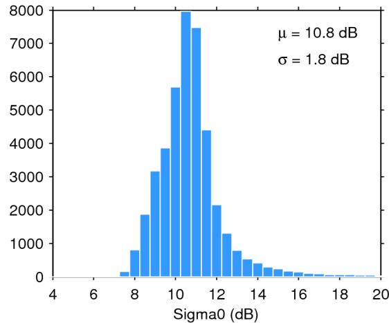
Figure 25. Histogram of flag-valid sigma0 over oceans and lakes for 16/04/2019. The mean ( \mu ) and standard deviation ( \sigma ) are also shown. Note that values outside [4 20] dB are excluded from the histogram for the sake of readability but not from the computation of \mu and \sigma .
