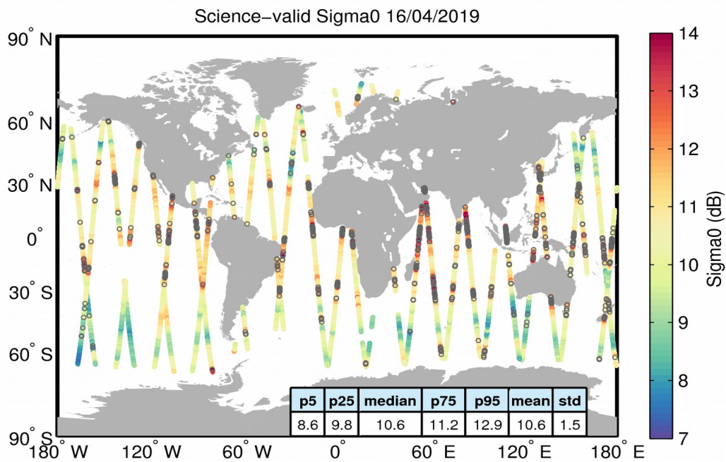
Figure 27. Geographical distribution of science-valid sigma0 data over oceans and lakes for 16/04/2019. The statistical values shown in the table refer to the sigma0 in dB and are calculated over all measurements shown in the figure. Gray circles denote records that have been rejected based on the editing criteria described in Table 4.
