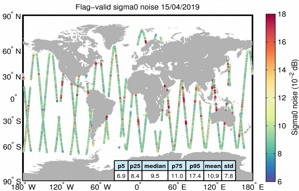
Figure 26. Geographical distribution of flag-valid 20-Hz sigma0 measurement noise over oceans and lakes for 15/04/2019. The statistical values shown in the table refer to the sigma0 noise and are calculated over all measurements shown in the figure.
