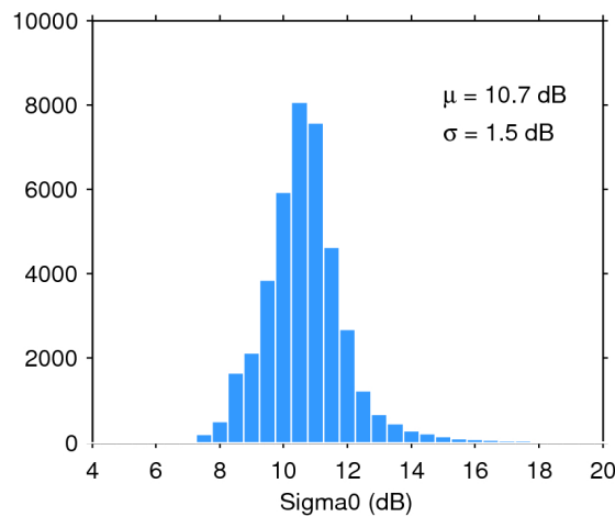
Figure 28. Histogram of science-valid sigma0 over oceans and lakes for 15/04/2019. The mean ( \mu ) and standard deviation ( \sigma ) are also shown. Note that values outside [4 20] dB are excluded from the histogram for the sake of readability but not from the computation of \mu and \sigma .
