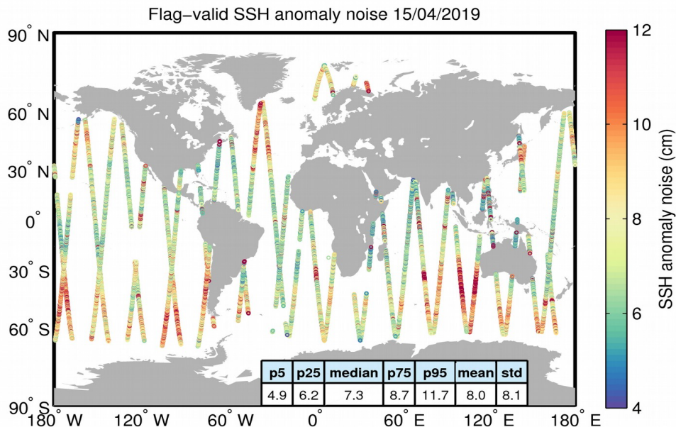
Figure 8. Geographical distribution of flag-valid 20-Hz SSH anomaly measurement noise over oceans and lakes for 15/04/2019. The statistical values shown in the table refer to the SSH anomaly noise and are calculated over all measurements shown in the figure.
