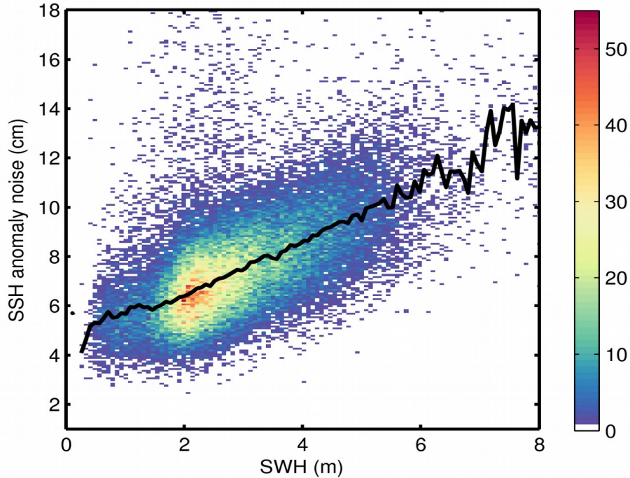
Figure 9. 2D histogram showing flag-valid SSH anomaly noise as a function of SWH for 15/04/2019. The black line denotes the median SSH anomaly noise as a function of SWH.
