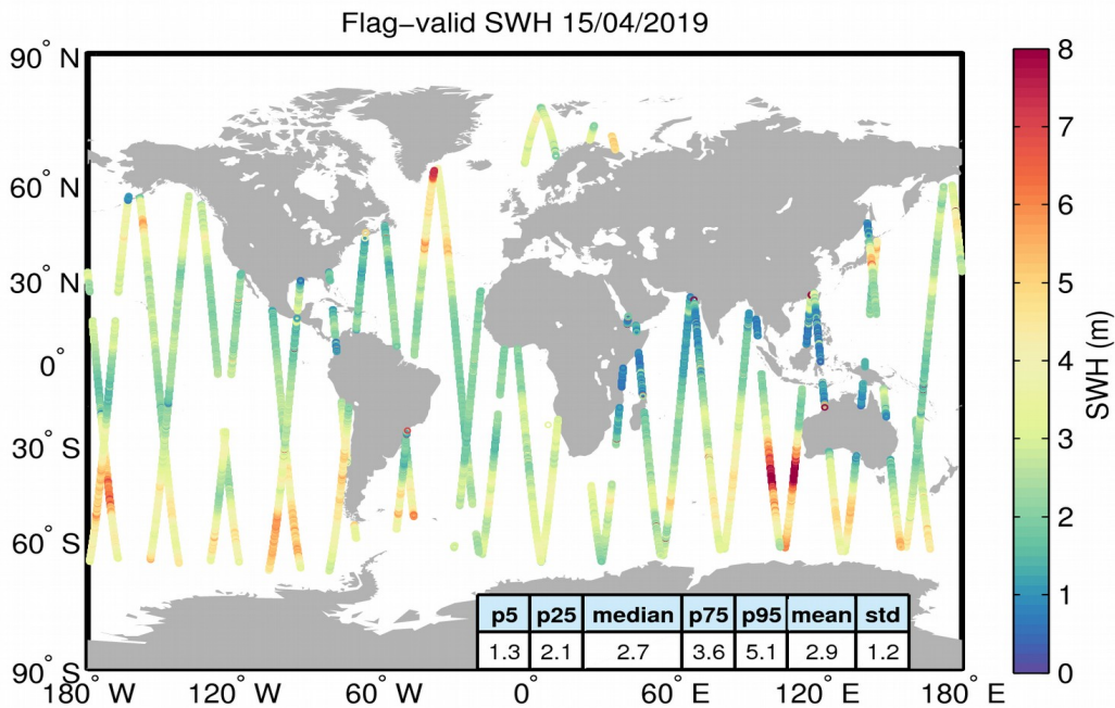
Figure 15. Geographical distribution of flag-valid SWH data over oceans and lakes for 15/04/2019. The statistical values shown in the table refer to the SWH in m and are calculated over all measurements shown in the figure.
