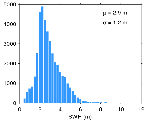
Figure 20. Histogram of science-valid SWH over oceans and lakes for 15/04/2019. The mean ( \mu ) and standard deviation ( \sigma ) are also shown. Note that values larger than 12 m are excluded from the histogram for the sake of readability but not from the computation of \mu and \sigma .
