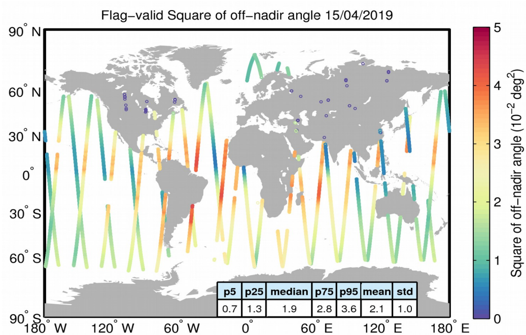
Figure 37. Geographical distribution of flag-valid mispointing data over oceans and lakes for 15/04/2019. The statistical values shown in the table refer to the mispointing in 10^{-2} deg 2 and are calculated over all measurements shown in the figure.
