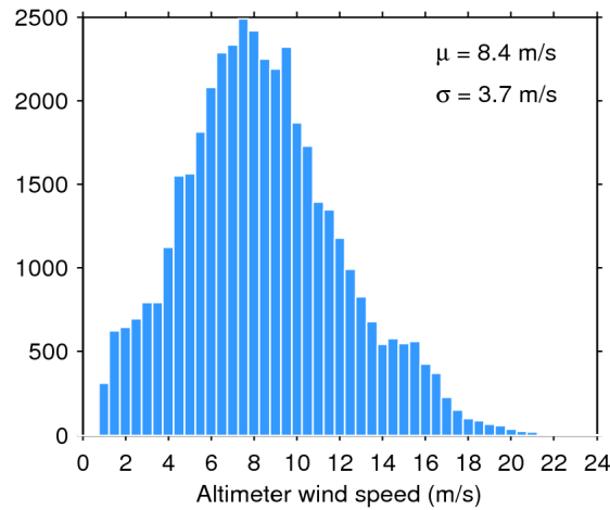
Figure 33. Histogram of flag-valid wind over oceans and lakes for 15/04/2019. The mean ( \mu ) and standard deviation ( \sigma ) are also shown. Note that values larger than 24 m/s are excluded from the histogram for the sake of readability but not from the computation of \mu and \sigma .
