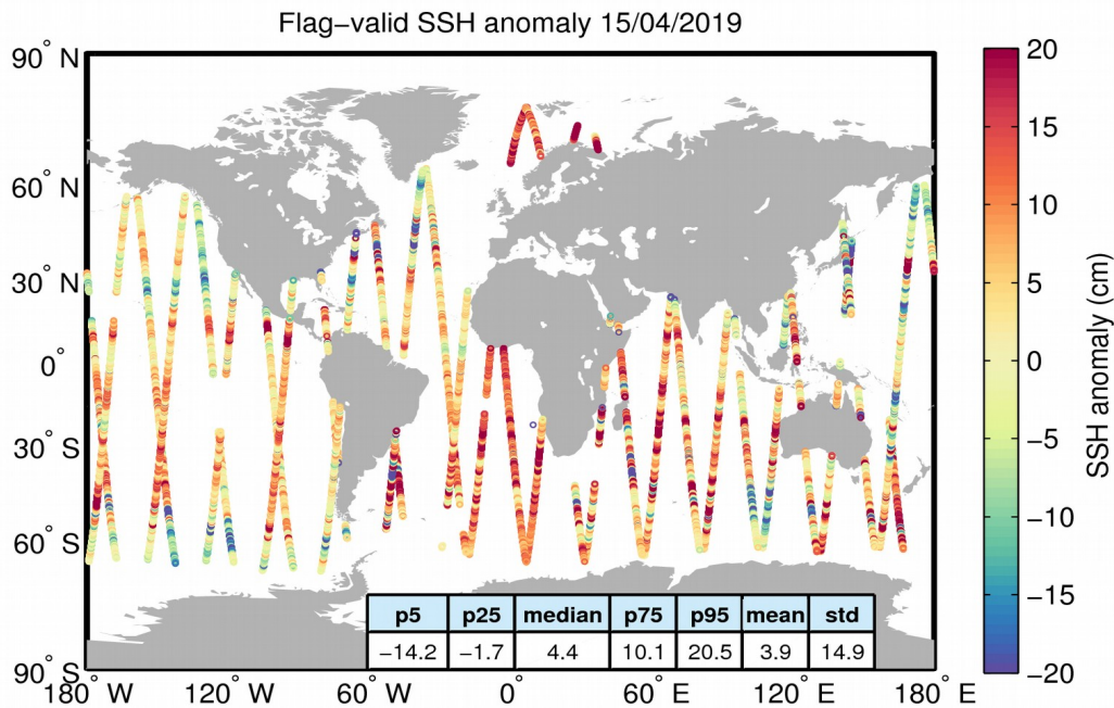
Figure 5. Geographical distribution of flag-valid 1-Hz SSH anomaly data over oceans and lakes for 15/04/2019. The statistical values shown in the table refer to the SSH anomaly in cm and are calculated over all measurements shown in the figure.
