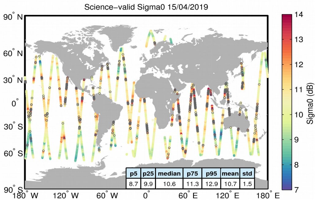
Figure 27. Geographical distribution of science-valid sigma0 data over oceans and lakes for 15/04/2019. The statistical values shown in the table refer to the sigma0 in dB and are calculated over all measurements shown in the figure. Gray circles denote records that have been rejected based on the editing criteria described in Table 4.
