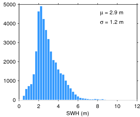
Figure 17. Histogram of flag-valid SWH over oceans and lakes for 15/04/2019. The mean ( \mu ) and standard deviation ( \sigma ) are also shown. Note that values larger than 12 m are excluded from the histogram for the sake of readability but not from the computation of \mu and \sigma .
