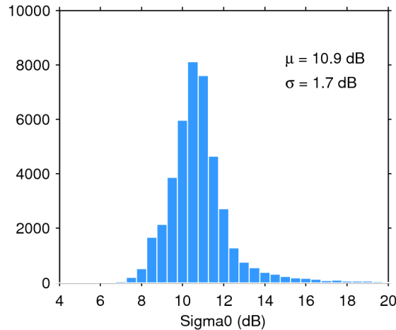
Figure 25. Histogram of flag-valid sigma0 over oceans and lakes for 15/04/2019. The mean ( \mu ) and standard deviation ( \sigma ) are also shown. Note that values outside [4 20] dB are excluded from the histogram for the sake of readability but not from the computation of \mu and \sigma .
