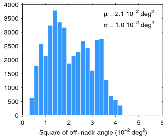
Figure 39. Histogram of flag-valid mispointing over oceans and lakes for 15/04/2019. The mean ( \mu ) and standard deviation ( \sigma ) are also shown. Note that values larger than 6 \cdot 10^{-2} \text{ deg}^2 are excluded from the histogram for the sake of readability but not from the computation of \mu and \sigma .
