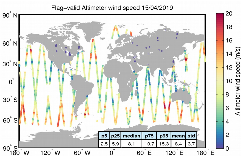
Figure 31. Geographical distribution of flag-valid wind data over oceans and lakes for 15/04/2019. The statistical values shown in the table refer to the wind in m/s and are calculated over all measurements shown in the figure.
