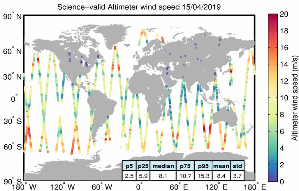
Figure 34. Geographical distribution of science-valid wind data over oceans and lakes for 15/04/2019. The statistical values shown in the table refer to the wind in m/s and are calculated over all measurements shown in the figure. Gray circles denote records that have been rejected based on the editing criteria described in Table 5.
