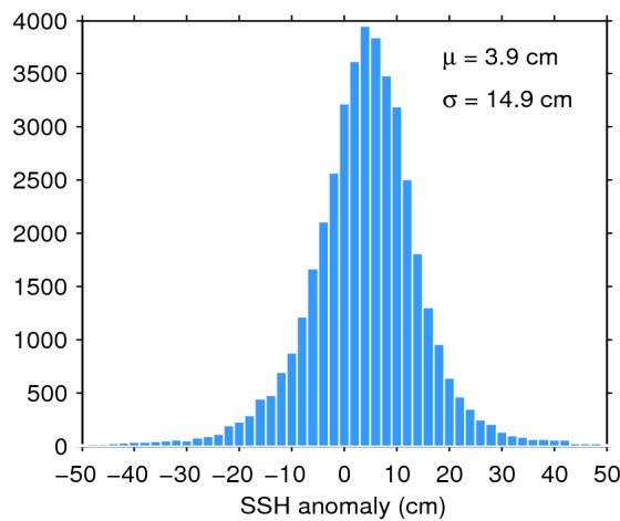
Figure 7. Histogram of flag-valid SSH anomaly over oceans and lakes for 15/04/2019. The mean ( \mu ) and standard deviation ( \sigma ) are also shown. Note that values outside [-50 50] cm are excluded from the histogram for the sake of readability but not from the computation of \mu and \sigma .
