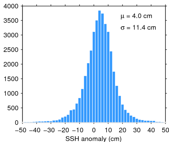
Figure 11. Histogram of science-valid SSH anomaly over oceans and lakes for 15/04/2019. The mean ( \mu ) and standard deviation ( \sigma ) are also shown. Note that values outside [-50 50] cm are excluded from the histogram for the sake of readability but not from the computation of \mu and \sigma .
