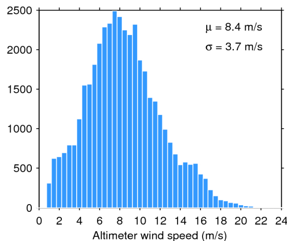
Figure 35. Histogram of science-valid wind over oceans and lakes for 15/04/2019. The mean ( \mu ) and standard deviation ( \sigma ) are also shown. Note that values larger than 24 m/s are excluded from the histogram for the sake of readability but not from the computation of \mu and \sigma .
