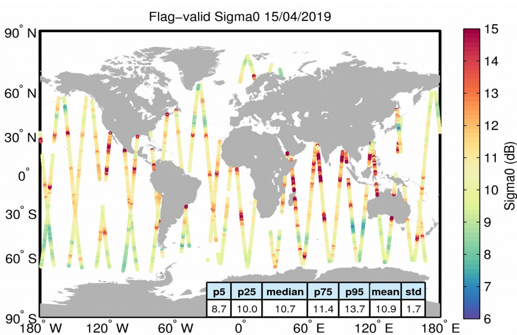
Figure 23. Geographical distribution of flag-valid sigma0 data over oceans and lakes for 15/04/2019. The statistical values shown in the table refer to the sigma0 in dB and are calculated over all measurements shown in the figure.
