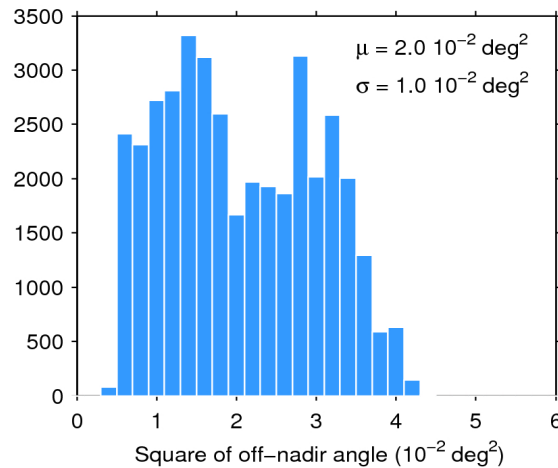
Figure 39. Histogram of flag-valid mispointing over oceans and lakes for 14/04/2019. The mean ( \mu ) and standard deviation ( \sigma ) are also shown. Note that values larger than 6 \cdot 10^{-2} \text{ deg}^2 are excluded from the histogram for the sake of readability but not from the computation of \mu and \sigma .
