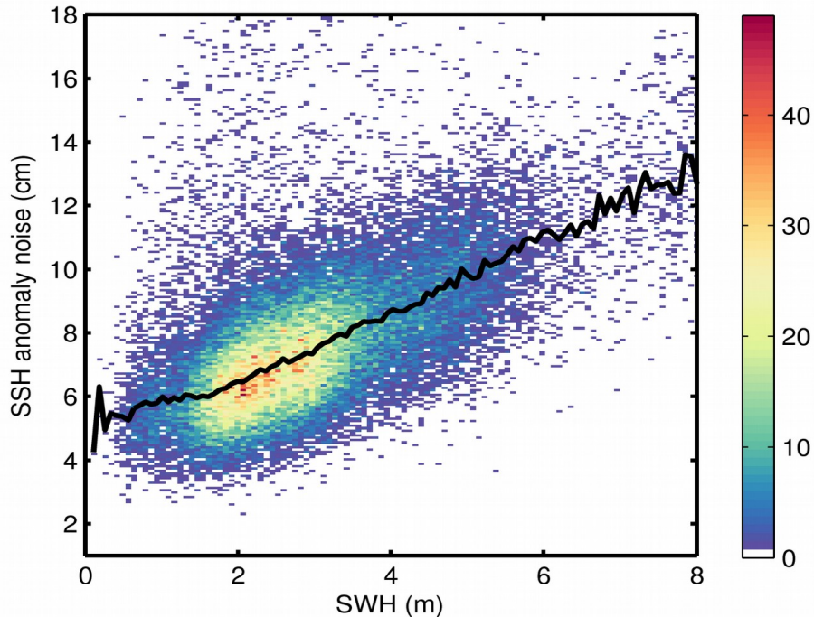
Figure 9. 2D histogram showing flag-valid SSH anomaly noise as a function of SWH for 14/04/2019. The black line denotes the median SSH anomaly noise as a function of SWH.
