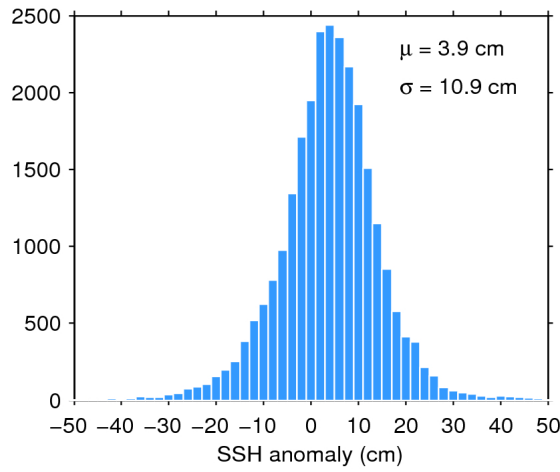
Figure 11. Histogram of science-valid SSH anomaly over oceans and lakes for 14/04/2019. The mean ( \mu ) and standard deviation ( \sigma ) are also shown. Note that values outside [-50 50] cm are excluded from the histogram for the sake of readability but not from the computation of \mu and \sigma .
