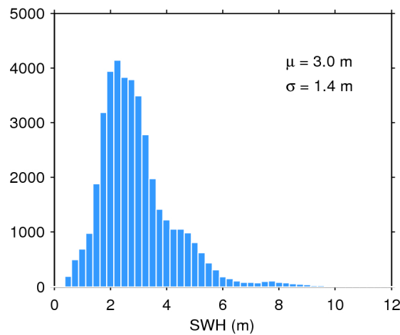
Figure 17. Histogram of flag-valid SWH over oceans and lakes for 14/04/2019. The mean ( \mu ) and standard deviation ( \sigma ) are also shown. Note that values larger than 12 m are excluded from the histogram for the sake of readability but not from the computation of \mu and \sigma .
