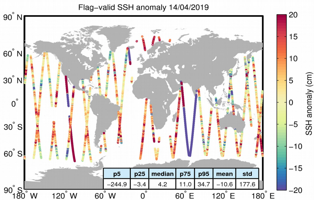
Figure 5. Geographical distribution of flag-valid 1-Hz SSH anomaly data over oceans and lakes for 14/04/2019. The statistical values shown in the table refer to the SSH anomaly in cm and are calculated over all measurements shown in the figure.
