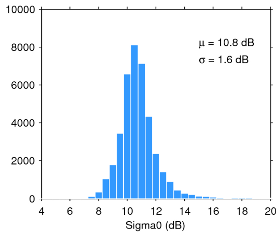
Figure 28. Histogram of science-valid sigma0 over oceans and lakes for 14/04/2019. The mean ( \mu ) and standard deviation ( \sigma ) are also shown. Note that values outside [4 20] dB are excluded from the histogram for the sake of readability but not from the computation of \mu and \sigma .
