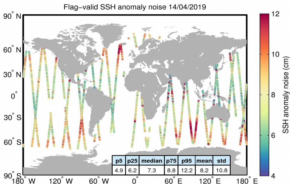
Figure 8. Geographical distribution of flag-valid 20-Hz SSH anomaly measurement noise over oceans and lakes for 14/04/2019. The statistical values shown in the table refer to the SSH anomaly noise and are calculated over all measurements shown in the figure.
