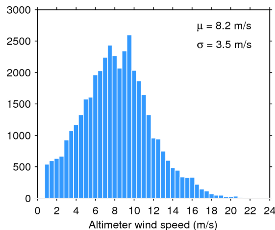
Figure 35. Histogram of science-valid wind over oceans and lakes for 14/04/2019. The mean ( \mu ) and standard deviation ( \sigma ) are also shown. Note that values larger than 24 m/s are excluded from the histogram for the sake of readability but not from the computation of \mu and \sigma .
