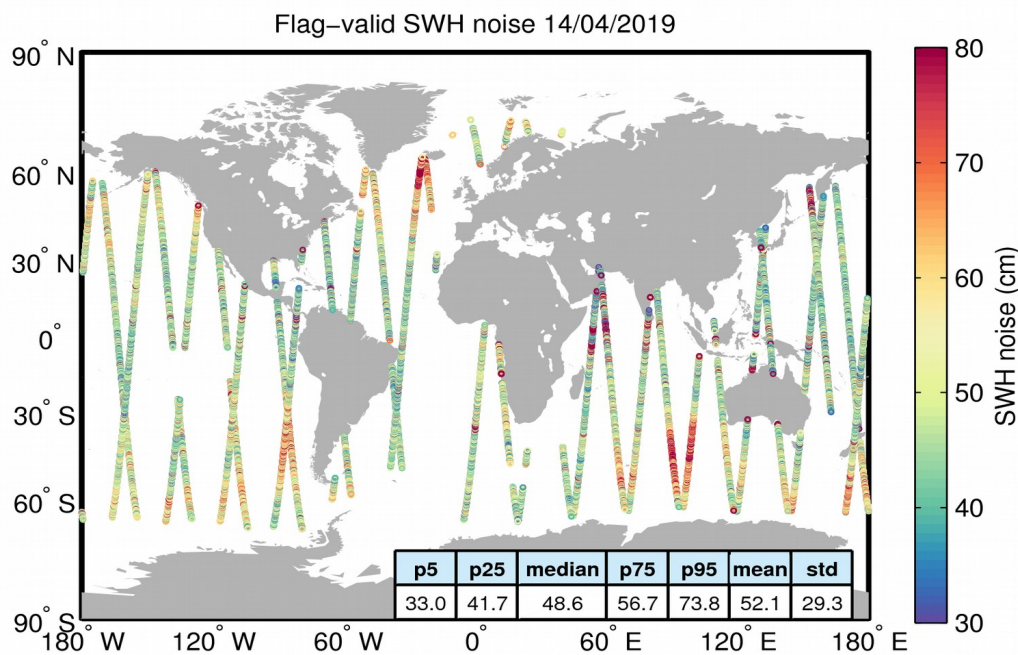
Figure 18. Geographical distribution of flag-valid 20-Hz SWH measurement noise over oceans and lakes for 14/04/2019. The statistical values shown in the table refer to the SWH noise and are calculated over all measurements shown in the figure.
