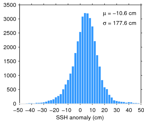
Figure 7. Histogram of flag-valid SSH anomaly over oceans and lakes for 14/04/2019. The mean ( \mu ) and standard deviation ( \sigma ) are also shown. Note that values outside [-50 50] cm are excluded from the histogram for the sake of readability but not from the computation of \mu and \sigma .
