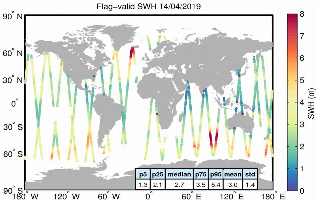
Figure 15. Geographical distribution of flag-valid SWH data over oceans and lakes for 14/04/2019. The statistical values shown in the table refer to the SWH in m and are calculated over all measurements shown in the figure.
