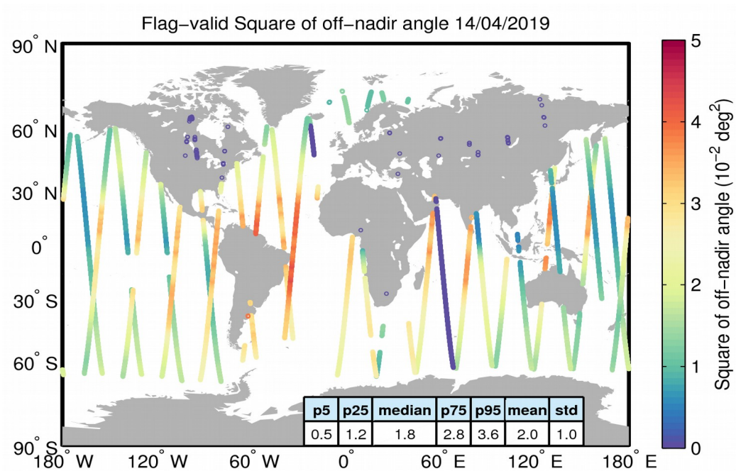
Figure 37. Geographical distribution of flag-valid mispointing data over oceans and lakes for 14/04/2019. The statistical values shown in the table refer to the mispointing in 10^{-2} deg 2 and are calculated over all measurements shown in the figure.
