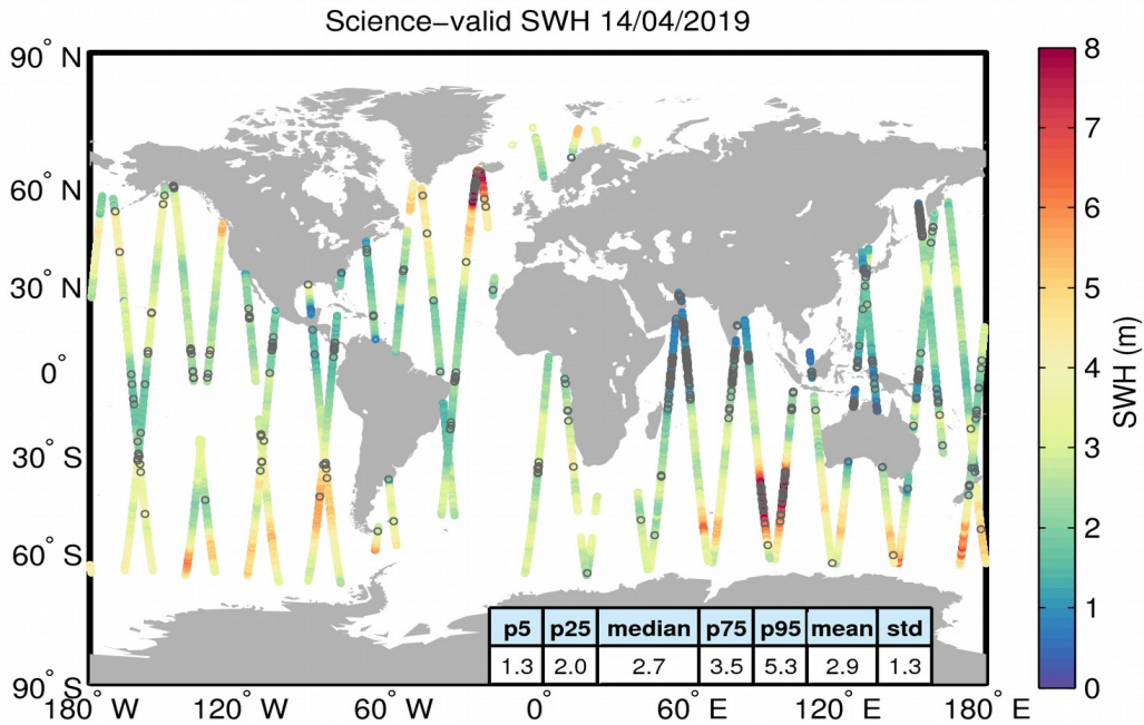
Figure 19. Geographical distribution of science-valid SWH data over oceans and lakes for 14/04/2019. The statistical values shown in the table refer to the SWH in m and are calculated over all measurements shown in the figure. Gray circles denote records that have been rejected based on the editing criteria described in Table 3.
