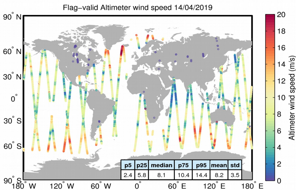
Figure 31. Geographical distribution of flag-valid wind data over oceans and lakes for 14/04/2019. The statistical values shown in the table refer to the wind in m/s and are calculated over all measurements shown in the figure.
