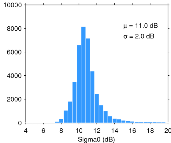
Figure 25. Histogram of flag-valid sigma0 over oceans and lakes for 14/04/2019. The mean ( \mu ) and standard deviation ( \sigma ) are also shown. Note that values outside [4 20] dB are excluded from the histogram for the sake of readability but not from the computation of \mu and \sigma .
