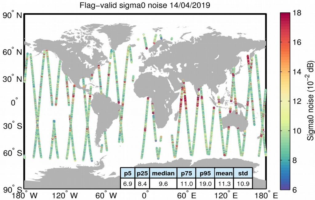
Figure 26. Geographical distribution of flag-valid 20-Hz sigma0 measurement noise over oceans and lakes for 14/04/2019. The statistical values shown in the table refer to the sigma0 noise and are calculated over all measurements shown in the figure.
