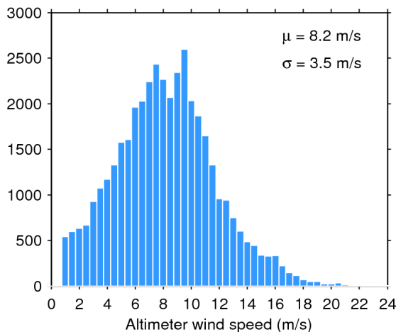
Figure 33. Histogram of flag-valid wind over oceans and lakes for 14/04/2019. The mean ( \mu ) and standard deviation ( \sigma ) are also shown. Note that values larger than 24 m/s are excluded from the histogram for the sake of readability but not from the computation of \mu and \sigma .
