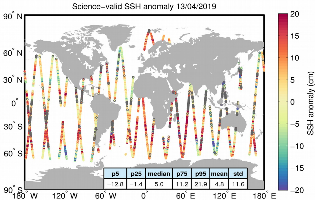
Figure 10. Geographical distribution of science-valid SSH anomaly data over oceans and lakes for 13/04/2019. The statistical values shown in the table refer to the SSH anomaly in cm and are calculated over all measurements shown in the figure. Gray circles denote records that have been rejected based on the editing criteria described in Table 2.
