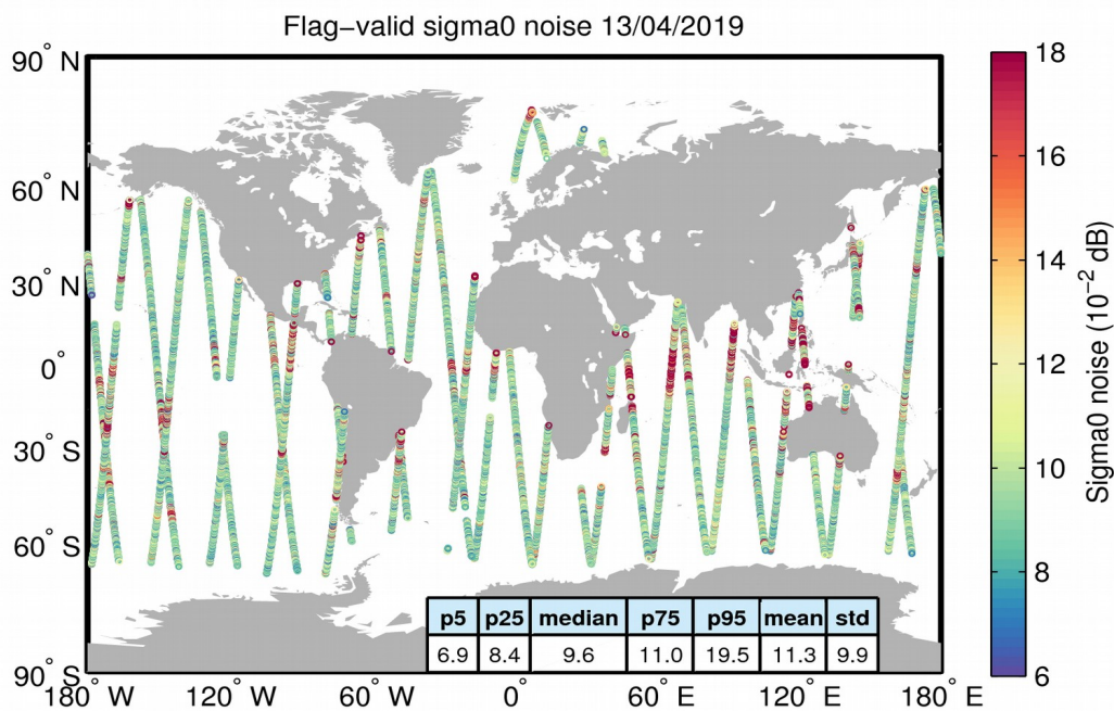
Figure 26. Geographical distribution of flag-valid 20-Hz sigma0 measurement noise over oceans and lakes for 13/04/2019. The statistical values shown in the table refer to the sigma0 noise and are calculated over all measurements shown in the figure.
