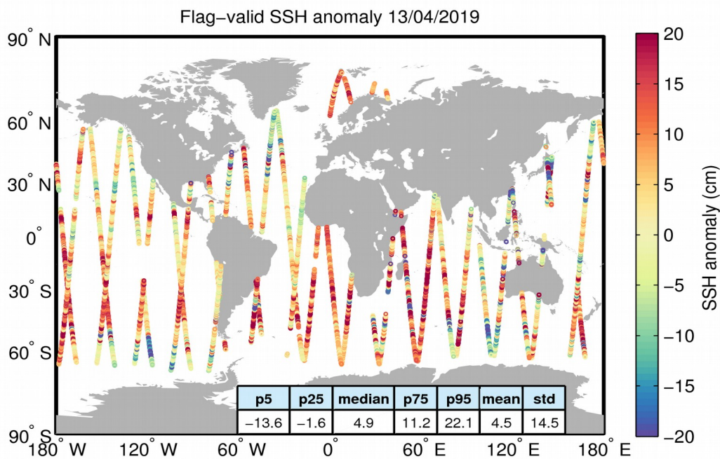
Figure 5. Geographical distribution of flag-valid 1-Hz SSH anomaly data over oceans and lakes for 13/04/2019. The statistical values shown in the table refer to the SSH anomaly in cm and are calculated over all measurements shown in the figure.
