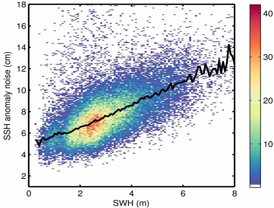
Figure 9. 2D histogram showing flag-valid SSH anomaly noise as a function of SWH for 13/04/2019. The black line denotes the median SSH anomaly noise as a function of SWH.
