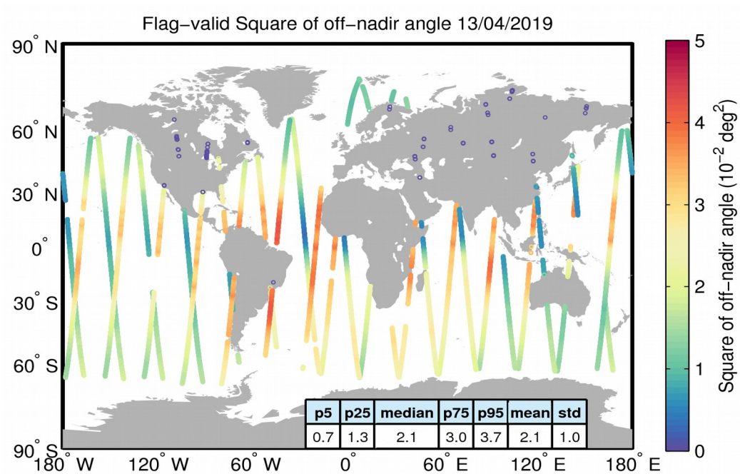
Figure 37. Geographical distribution of flag-valid mispointing data over oceans and lakes for 13/04/2019. The statistical values shown in the table refer to the mispointing in 10^{-2} deg 2 and are calculated over all measurements shown in the figure.
