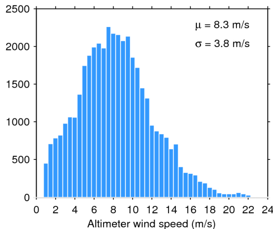
Figure 35. Histogram of science-valid wind over oceans and lakes for 13/04/2019. The mean ( \mu ) and standard deviation ( \sigma ) are also shown. Note that values larger than 24 m/s are excluded from the histogram for the sake of readability but not from the computation of \mu and \sigma .
