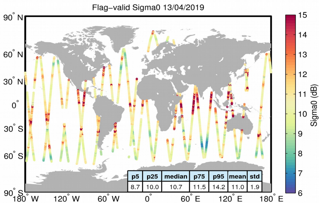
Figure 23. Geographical distribution of flag-valid sigma0 data over oceans and lakes for 13/04/2019. The statistical values shown in the table refer to the sigma0 in dB and are calculated over all measurements shown in the figure.
