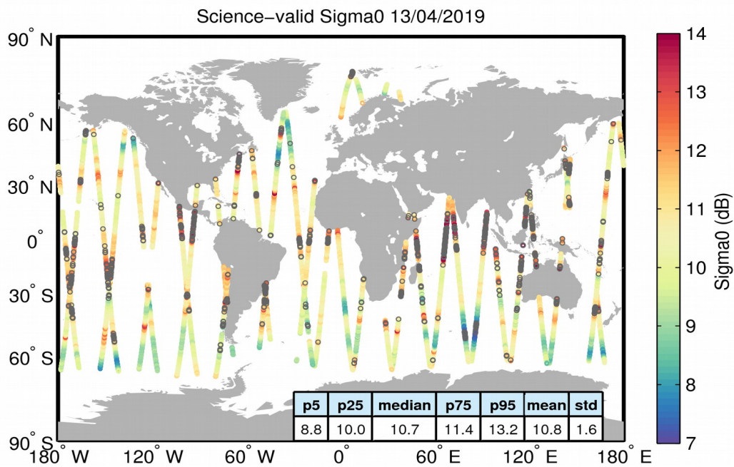
Figure 27. Geographical distribution of science-valid sigma0 data over oceans and lakes for 13/04/2019. The statistical values shown in the table refer to the sigma0 in dB and are calculated over all measurements shown in the figure. Gray circles denote records that have been rejected based on the editing criteria described in Table 4.
