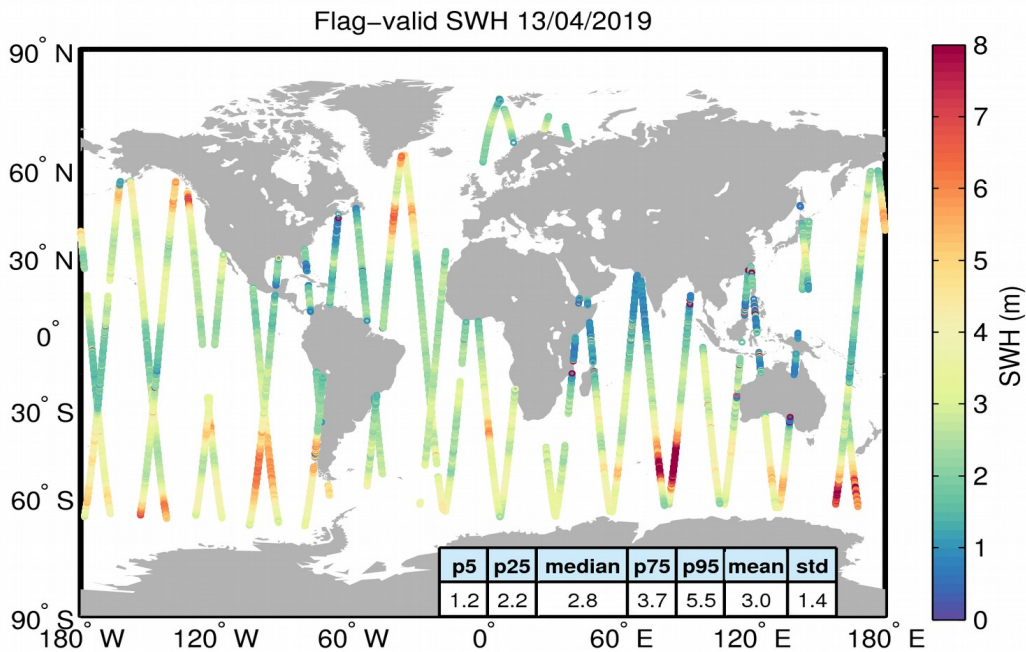
Figure 15. Geographical distribution of flag-valid SWH data over oceans and lakes for 13/04/2019. The statistical values shown in the table refer to the SWH in m and are calculated over all measurements shown in the figure.
