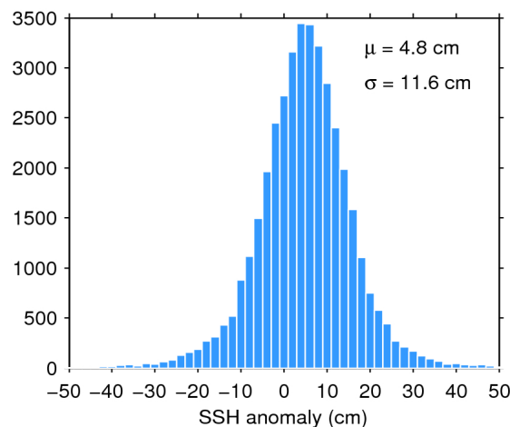
Figure 11. Histogram of science-valid SSH anomaly over oceans and lakes for 13/04/2019. The mean ( \mu ) and standard deviation ( \sigma ) are also shown. Note that values outside [-50 50] cm are excluded from the histogram for the sake of readability but not from the computation of \mu and \sigma .
