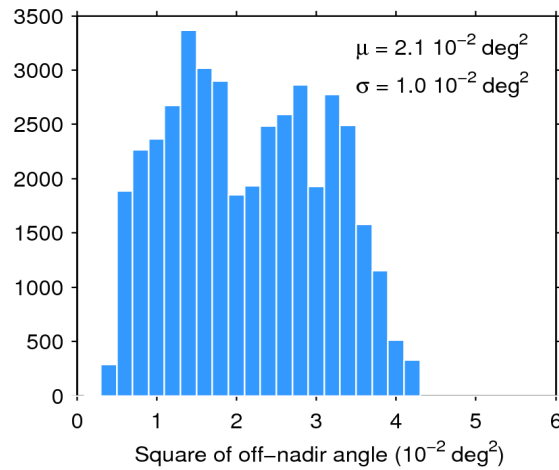
Figure 39. Histogram of flag-valid mispointing over oceans and lakes for 13/04/2019. The mean ( \mu ) and standard deviation ( \sigma ) are also shown. Note that values larger than 6 \cdot 10^{-2} \text{ deg}^2 are excluded from the histogram for the sake of readability but not from the computation of \mu and \sigma .
