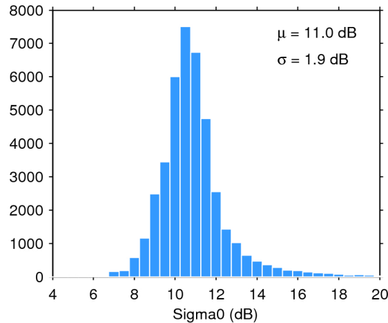
Figure 25. Histogram of flag-valid sigma0 over oceans and lakes for 13/04/2019. The mean ( \mu ) and standard deviation ( \sigma ) are also shown. Note that values outside [4 20] dB are excluded from the histogram for the sake of readability but not from the computation of \mu and \sigma .
