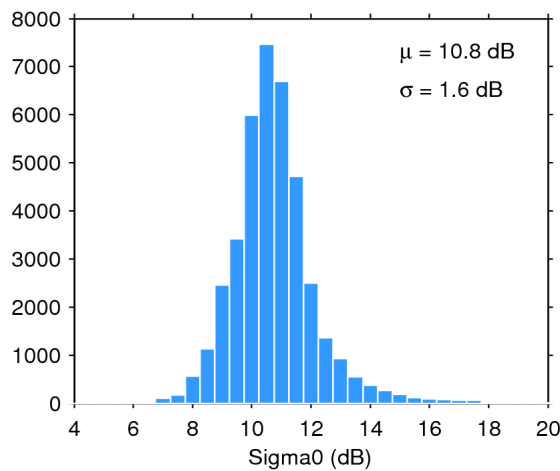
Figure 28. Histogram of science-valid sigma0 over oceans and lakes for 13/04/2019. The mean ( \mu ) and standard deviation ( \sigma ) are also shown. Note that values outside [4 20] dB are excluded from the histogram for the sake of readability but not from the computation of \mu and \sigma .
