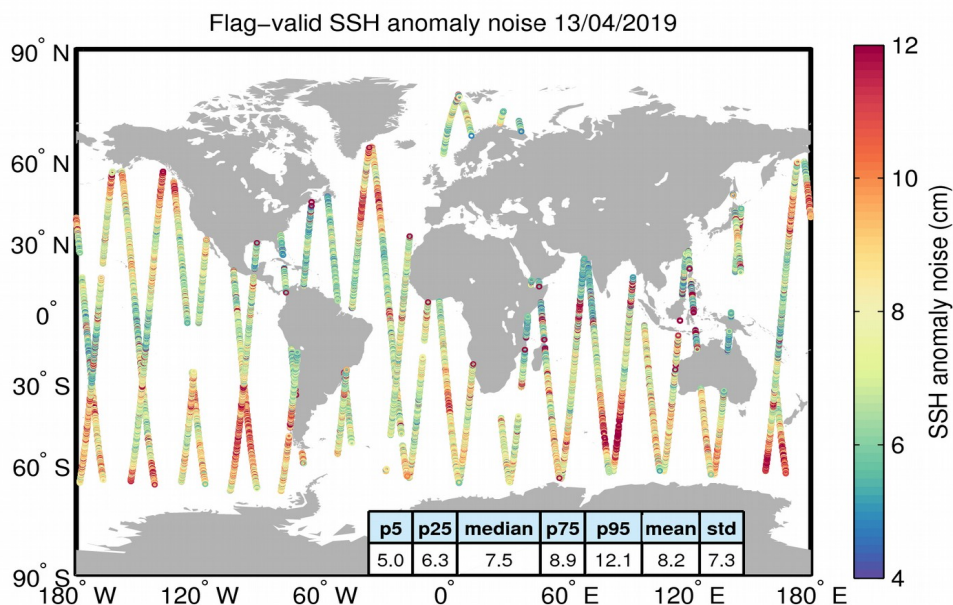
Figure 8. Geographical distribution of flag-valid 20-Hz SSH anomaly measurement noise over oceans and lakes for 13/04/2019. The statistical values shown in the table refer to the SSH anomaly noise and are calculated over all measurements shown in the figure.
