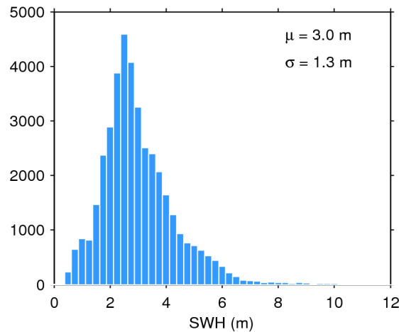
Figure 20. Histogram of science-valid SWH over oceans and lakes for 13/04/2019. The mean ( \mu ) and standard deviation ( \sigma ) are also shown. Note that values larger than 12 m are excluded from the histogram for the sake of readability but not from the computation of \mu and \sigma .
