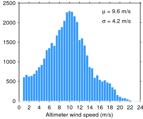
Figure 33. Histogram of flag-valid wind over oceans and lakes for 12/04/2019. The mean ( \mu ) and standard deviation ( \sigma ) are also shown. Note that values larger than 24 m/s are excluded from the histogram for the sake of readability but not from the computation of \mu and \sigma .
