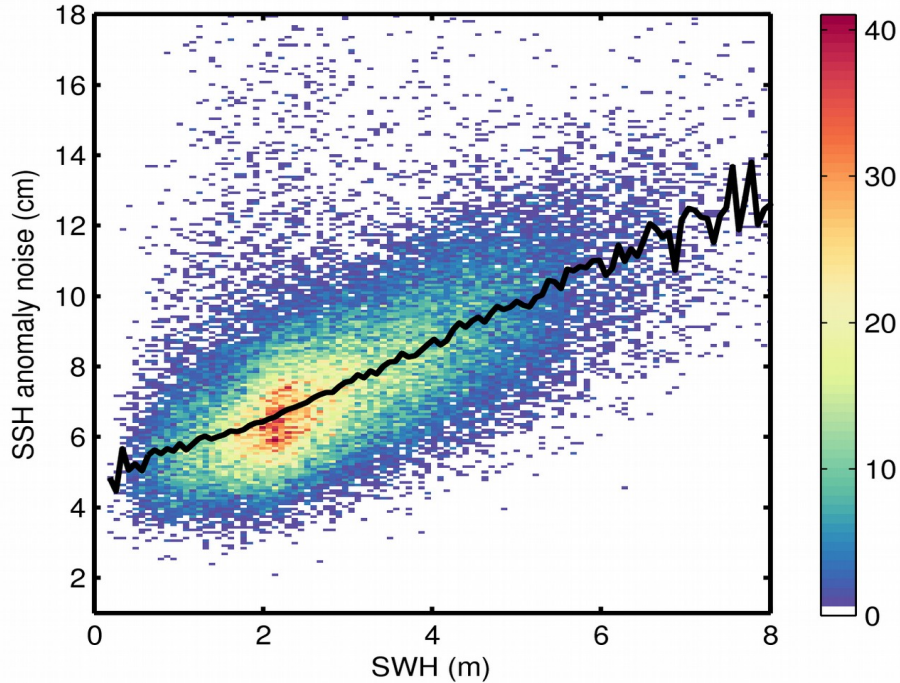
Figure 9. 2D histogram showing flag-valid SSH anomaly noise as a function of SWH for 12/04/2019. The black line denotes the median SSH anomaly noise as a function of SWH.
