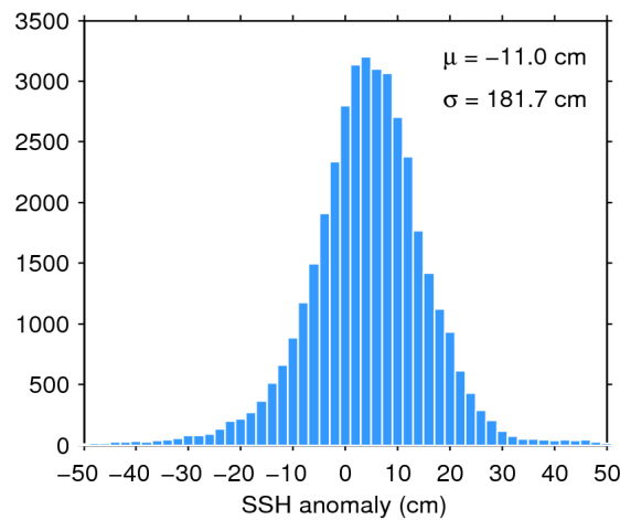
Figure 7. Histogram of flag-valid SSH anomaly over oceans and lakes for 12/04/2019. The mean ( \mu ) and standard deviation ( \sigma ) are also shown. Note that values outside [-50\ 50] cm are excluded from the histogram for the sake of readability but not from the computation of \mu and \sigma .
