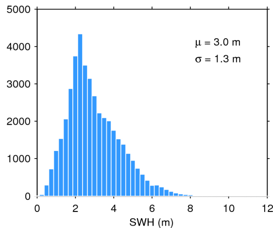
Figure 20. Histogram of science-valid SWH over oceans and lakes for 12/04/2019. The mean ( \mu ) and standard deviation ( \sigma ) are also shown. Note that values larger than 12 m are excluded from the histogram for the sake of readability but not from the computation of \mu and \sigma .
