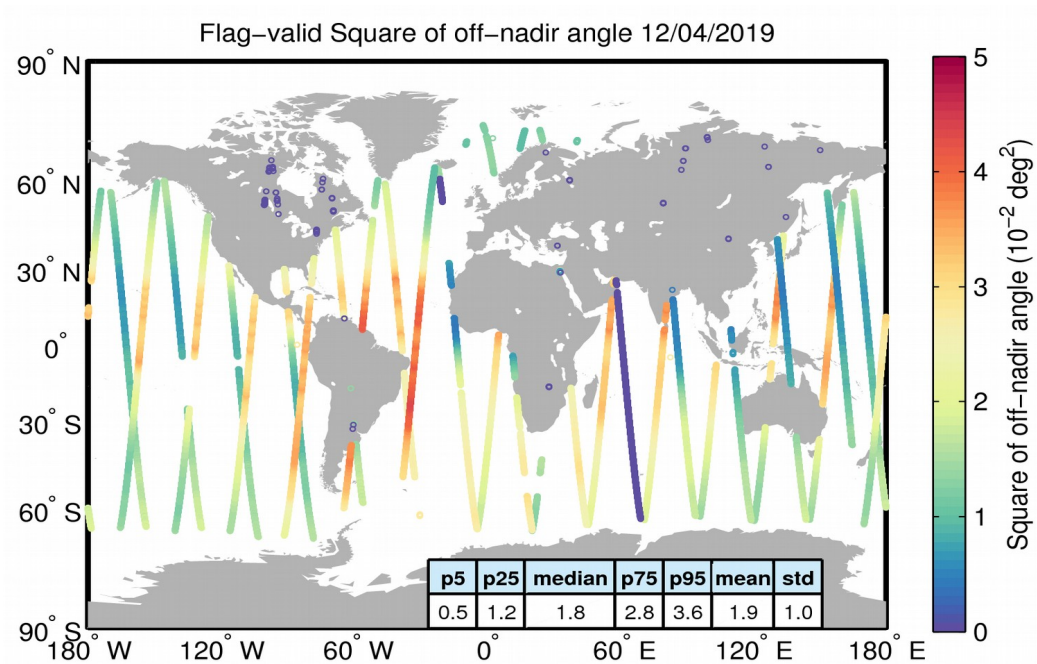
Figure 37. Geographical distribution of flag-valid mispointing data over oceans and lakes for 12/04/2019. The statistical values shown in the table refer to the mispointing in 10^{-2} \text{ deg}^2 and are calculated over all measurements shown in the figure.
