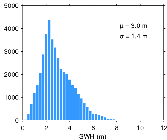
Figure 17. Histogram of flag-valid SWH over oceans and lakes for 12/04/2019. The mean ( \mu ) and standard deviation ( \sigma ) are also shown. Note that values larger than 12 m are excluded from the histogram for the sake of readability but not from the computation of \mu and \sigma .
