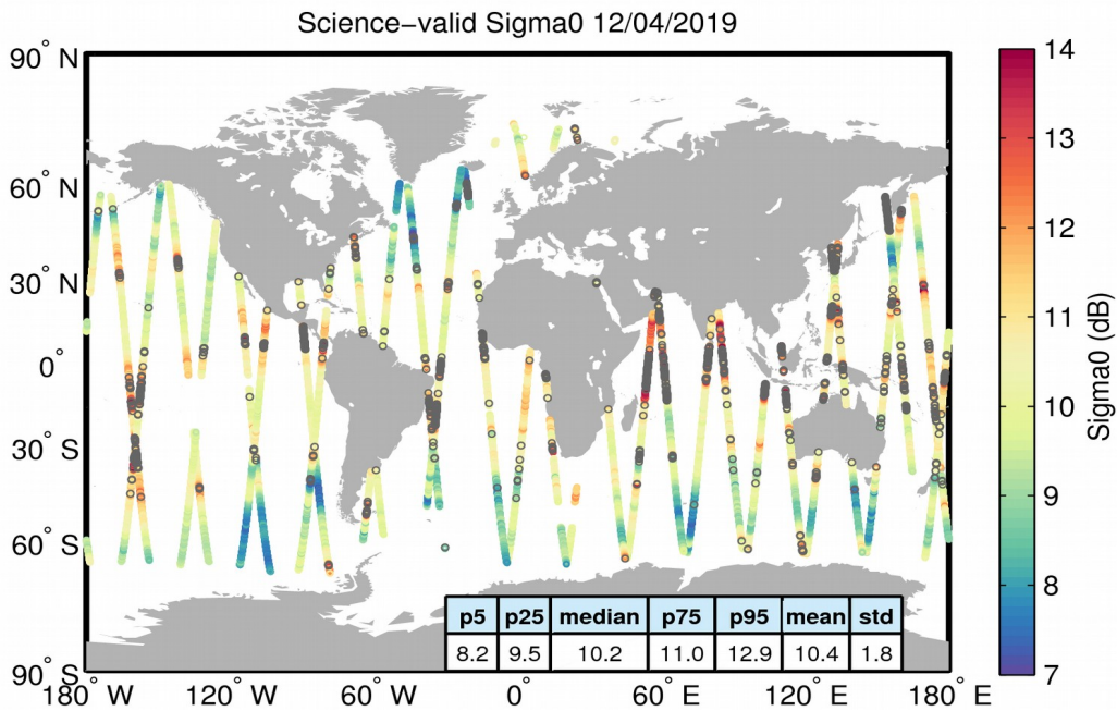
Figure 27. Geographical distribution of science-valid sigma0 data over oceans and lakes for 12/04/2019. The statistical values shown in the table refer to the sigma0 in dB and are calculated over all measurements shown in the figure. Gray circles denote records that have been rejected based on the editing criteria described in Table 4.
