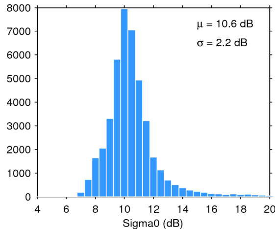
Figure 25. Histogram of flag-valid sigma0 over oceans and lakes for 12/04/2019. The mean ( \mu ) and standard deviation ( \sigma ) are also shown. Note that values outside [4 20] dB are excluded from the histogram for the sake of readability but not from the computation of \mu and \sigma .
