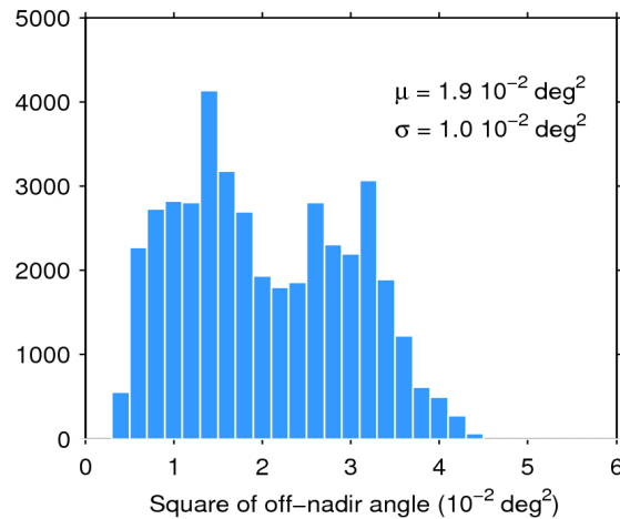
Figure 39. Histogram of flag-valid mispointing over oceans and lakes for 12/04/2019. The mean ( \mu ) and standard deviation ( \sigma ) are also shown. Note that values larger than 6 \cdot 10^{-2} \text{ deg}^2 are excluded from the histogram for the sake of readability but not from the computation of \mu and \sigma .
