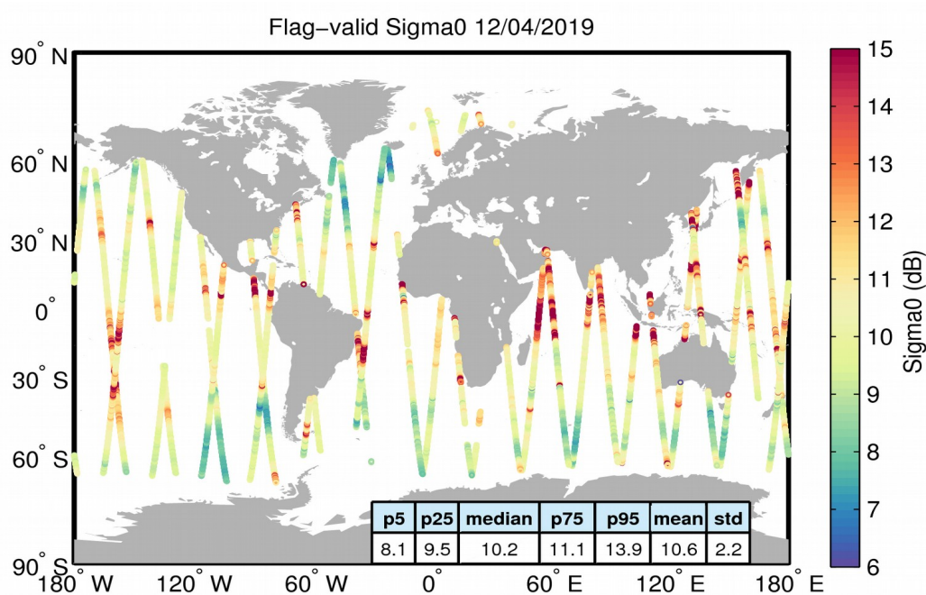
Figure 23. Geographical distribution of flag-valid sigma0 data over oceans and lakes for 12/04/2019. The statistical values shown in the table refer to the sigma0 in dB and are calculated over all measurements shown in the figure.
