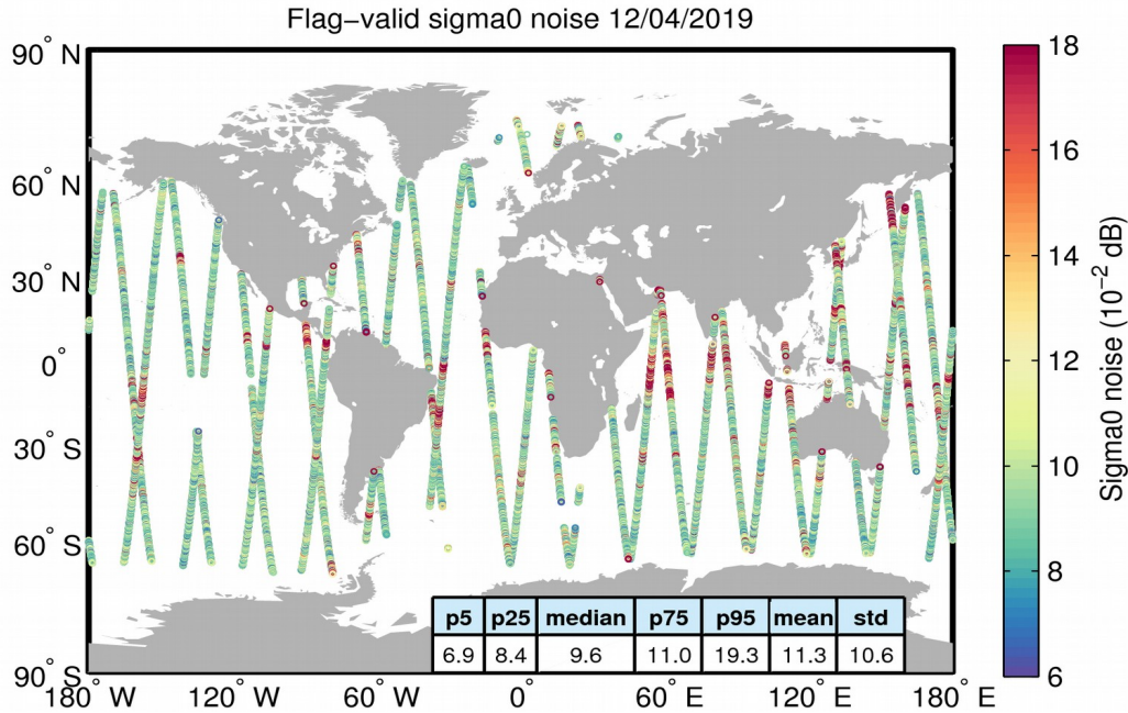
Figure 26. Geographical distribution of flag-valid 20-Hz sigma0 measurement noise over oceans and lakes for 12/04/2019. The statistical values shown in the table refer to the sigma0 noise and are calculated over all measurements shown in the figure.
