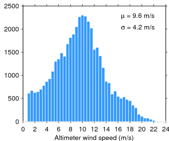
Figure 35. Histogram of science-valid wind over oceans and lakes for 12/04/2019. The mean ( \mu ) and standard deviation ( \sigma ) are also shown. Note that values larger than 24 m/s are excluded from the histogram for the sake of readability but not from the computation of \mu and \sigma .
