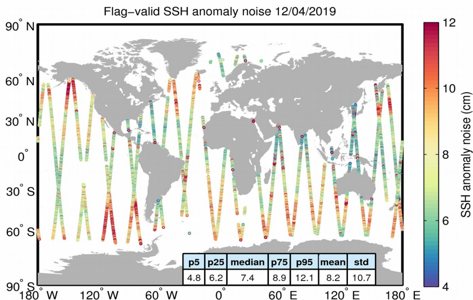
Figure 8. Geographical distribution of flag-valid 20-Hz SSH anomaly measurement noise over oceans and lakes for 12/04/2019. The statistical values shown in the table refer to the SSH anomaly noise and are calculated over all measurements shown in the figure.
