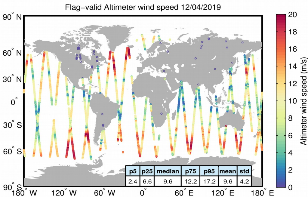
Figure 31. Geographical distribution of flag-valid wind data over oceans and lakes for 12/04/2019. The statistical values shown in the table refer to the wind in m/s and are calculated over all measurements shown in the figure.
