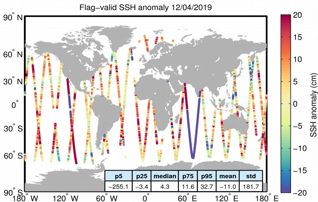
Figure 5. Geographical distribution of flag-valid 1-Hz SSH anomaly data over oceans and lakes for 12/04/2019. The statistical values shown in the table refer to the SSH anomaly in cm and are calculated over all measurements shown in the figure.
