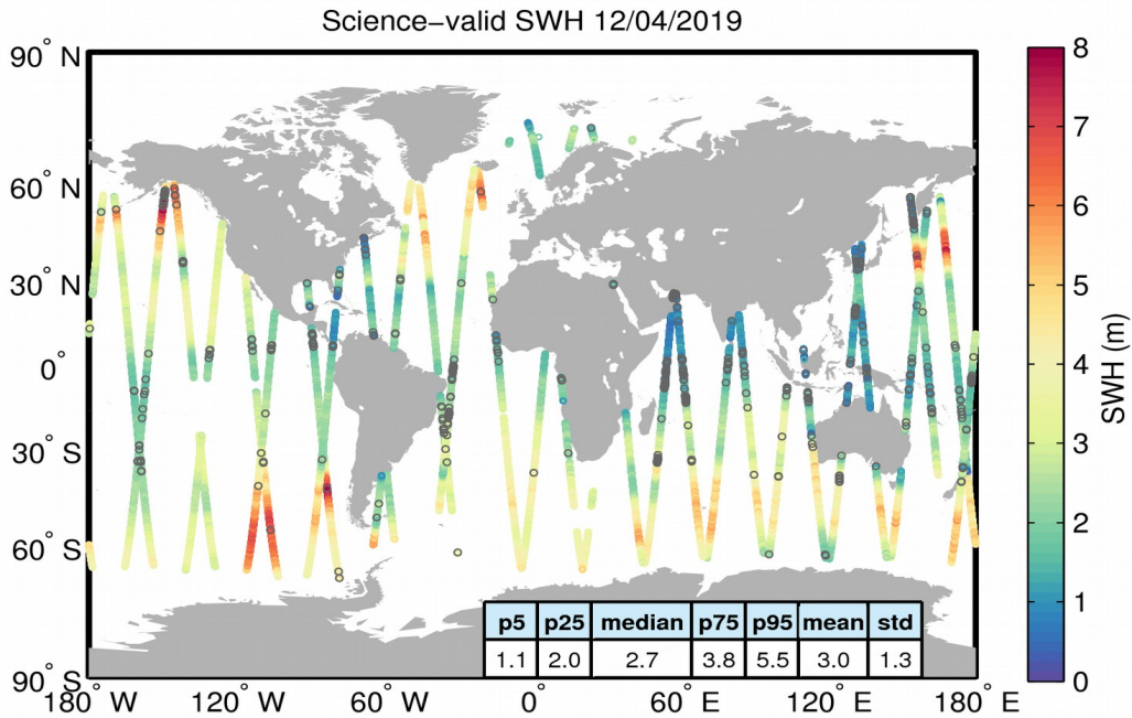
Figure 19. Geographical distribution of science-valid SWH data over oceans and lakes for 12/04/2019. The statistical values shown in the table refer to the SWH in m and are calculated over all measurements shown in the figure. Gray circles denote records that have been rejected based on the editing criteria described in Table 3.
