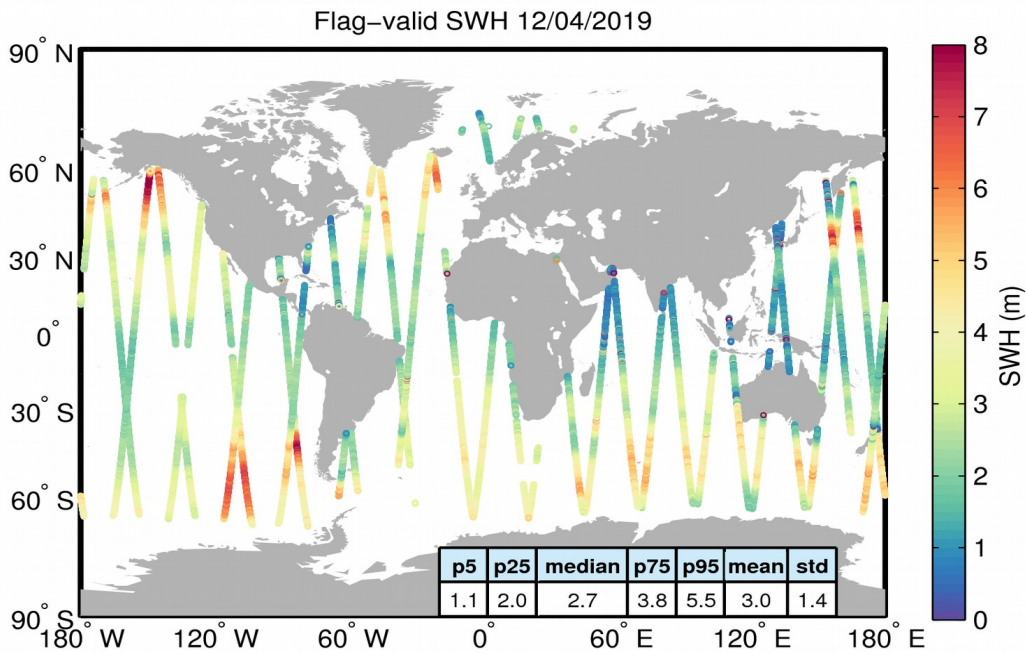
Figure 15. Geographical distribution of flag-valid SWH data over oceans and lakes for 12/04/2019. The statistical values shown in the table refer to the SWH in m and are calculated over all measurements shown in the figure.
