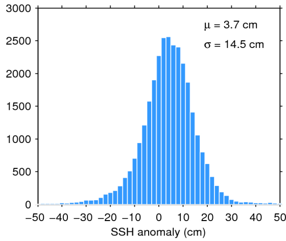
Figure 11. Histogram of science-valid SSH anomaly over oceans and lakes for 12/04/2019. The mean ( \mu ) and standard deviation ( \sigma ) are also shown. Note that values outside [-50 50] cm are excluded from the histogram for the sake of readability but not from the computation of \mu and \sigma .
