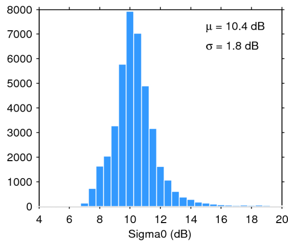
Figure 28. Histogram of science-valid sigma0 over oceans and lakes for 12/04/2019. The mean ( \mu ) and standard deviation ( \sigma ) are also shown. Note that values outside [4 20] dB are excluded from the histogram for the sake of readability but not from the computation of \mu and \sigma .
