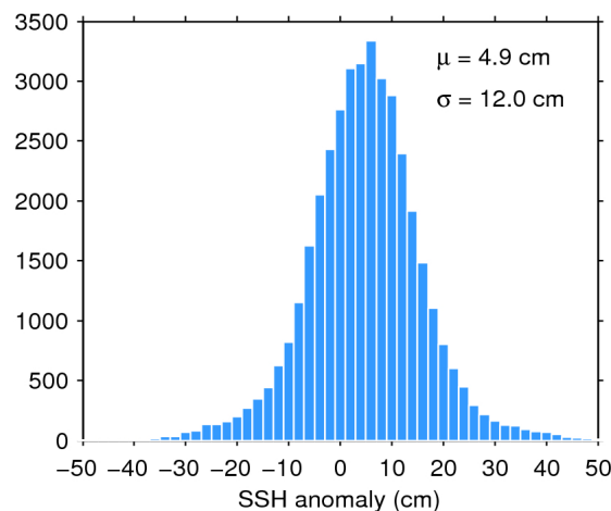
Figure 11. Histogram of science-valid SSH anomaly over oceans and lakes for 11/04/2019. The mean ( \mu ) and standard deviation ( \sigma ) are also shown. Note that values outside [-50 50] cm are excluded from the histogram for the sake of readability but not from the computation of \mu and \sigma .
