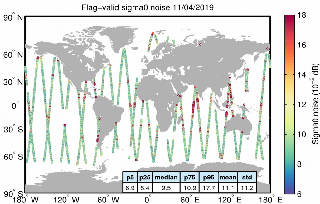
Figure 26. Geographical distribution of flag-valid 20-Hz sigma0 measurement noise over oceans and lakes for 11/04/2019. The statistical values shown in the table refer to the sigma0 noise and are calculated over all measurements shown in the figure.
