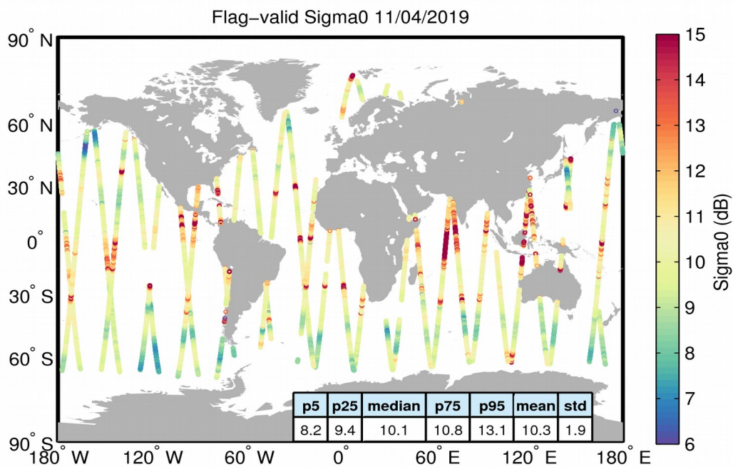
Figure 23. Geographical distribution of flag-valid sigma0 data over oceans and lakes for 11/04/2019. The statistical values shown in the table refer to the sigma0 in dB and are calculated over all measurements shown in the figure.
