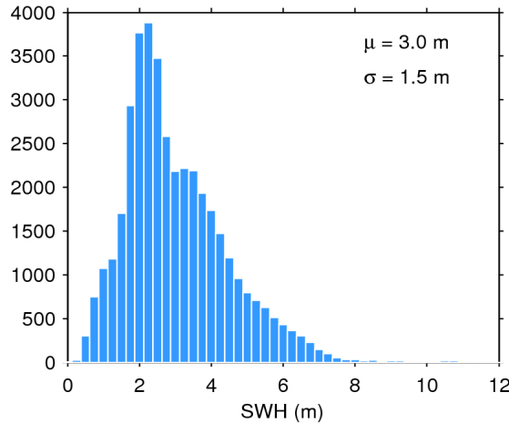
Figure 20. Histogram of science-valid SWH over oceans and lakes for 11/04/2019. The mean ( \mu ) and standard deviation ( \sigma ) are also shown. Note that values larger than 12 m are excluded from the histogram for the sake of readability but not from the computation of \mu and \sigma .
