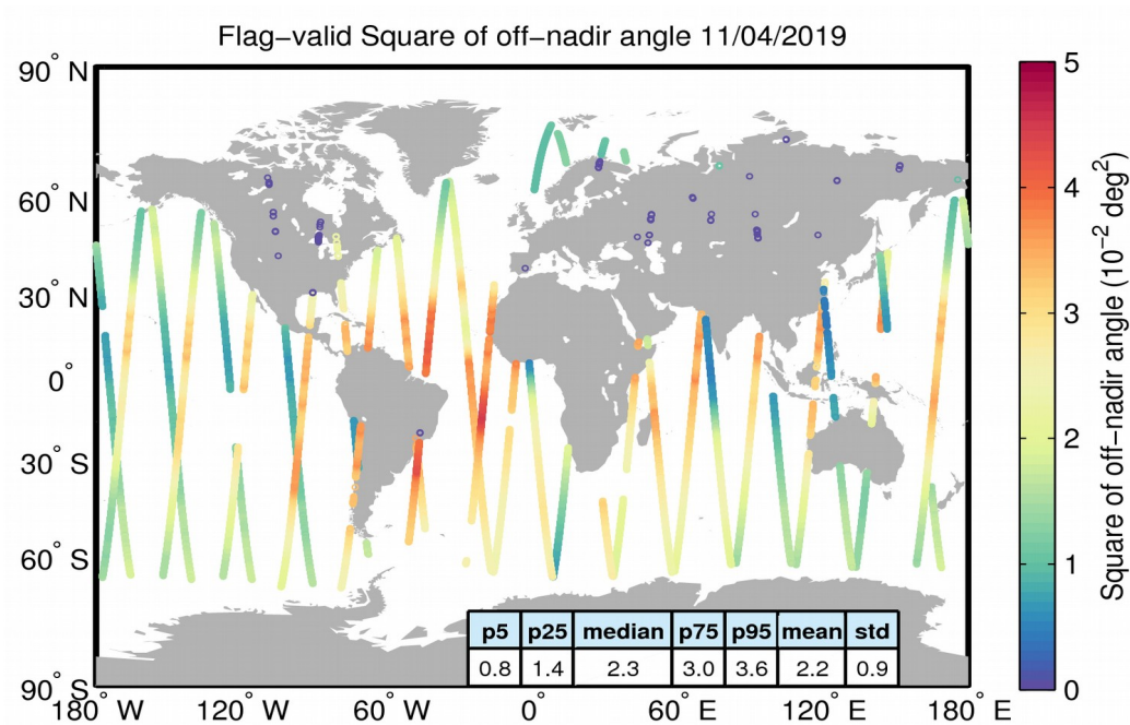
Figure 37. Geographical distribution of flag-valid mispointing data over oceans and lakes for 11/04/2019. The statistical values shown in the table refer to the mispointing in 10^{-2} \text{ deg}^2 and are calculated over all measurements shown in the figure.
