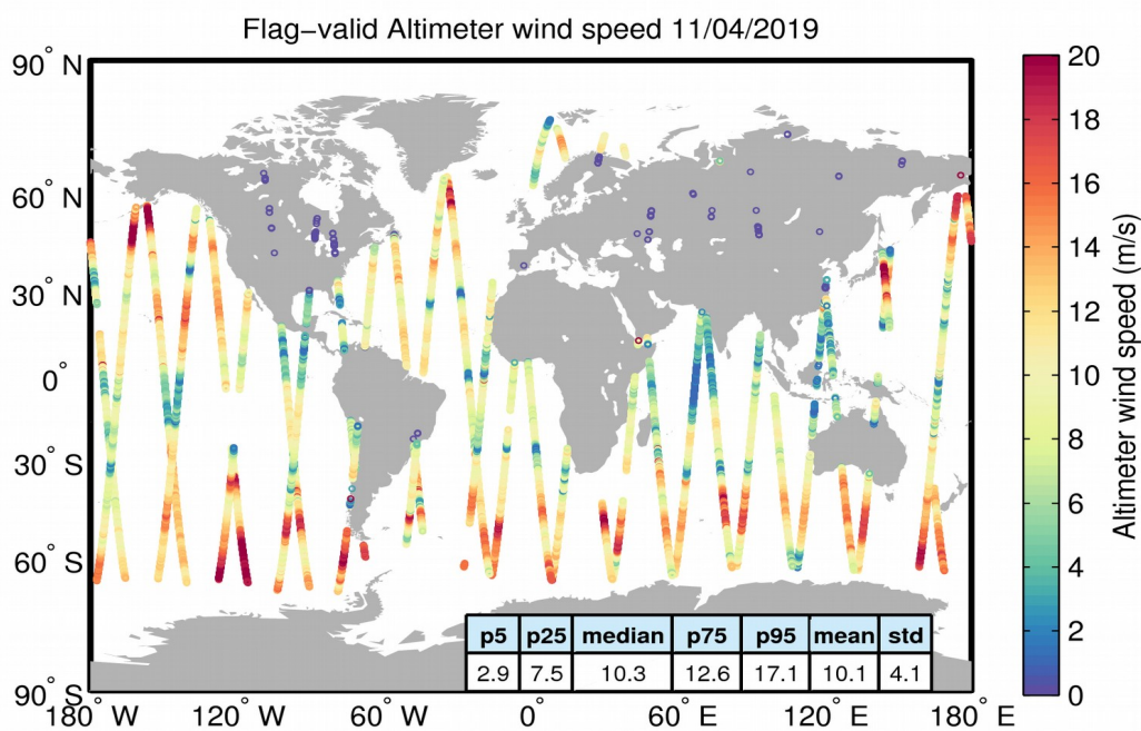
Figure 31. Geographical distribution of flag-valid wind data over oceans and lakes for 11/04/2019. The statistical values shown in the table refer to the wind in m/s and are calculated over all measurements shown in the figure.
