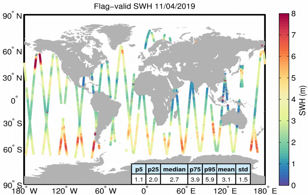
Figure 15. Geographical distribution of flag-valid SWH data over oceans and lakes for 11/04/2019. The statistical values shown in the table refer to the SWH in m and are calculated over all measurements shown in the figure.
