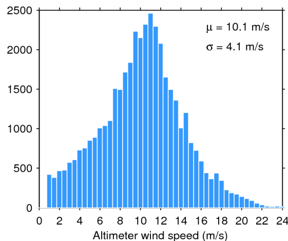
Figure 35. Histogram of science-valid wind over oceans and lakes for 11/04/2019. The mean ( \mu ) and standard deviation ( \sigma ) are also shown. Note that values larger than 24 m/s are excluded from the histogram for the sake of readability but not from the computation of \mu and \sigma .
