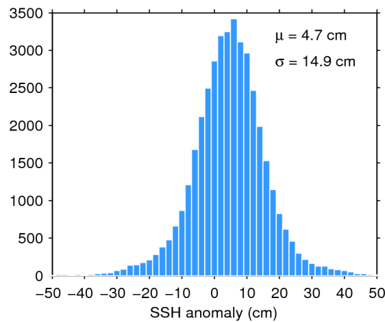
Figure 7. Histogram of flag-valid SSH anomaly over oceans and lakes for 11/04/2019. The mean ( \mu ) and standard deviation ( \sigma ) are also shown. Note that values outside [-50 50] cm are excluded from the histogram for the sake of readability but not from the computation of \mu and \sigma .
