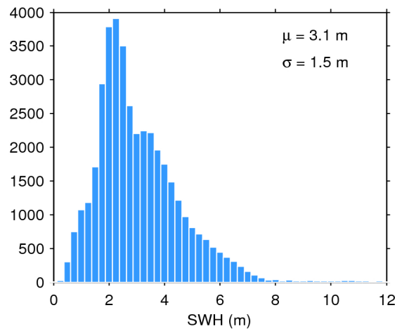
Figure 17. Histogram of flag-valid SWH over oceans and lakes for 11/04/2019. The mean ( \mu ) and standard deviation ( \sigma ) are also shown. Note that values larger than 12 m are excluded from the histogram for the sake of readability but not from the computation of \mu and \sigma .
