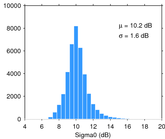
Figure 28. Histogram of science-valid sigma0 over oceans and lakes for 11/04/2019. The mean ( \mu ) and standard deviation ( \sigma ) are also shown. Note that values outside [4 20] dB are excluded from the histogram for the sake of readability but not from the computation of \mu and \sigma .
