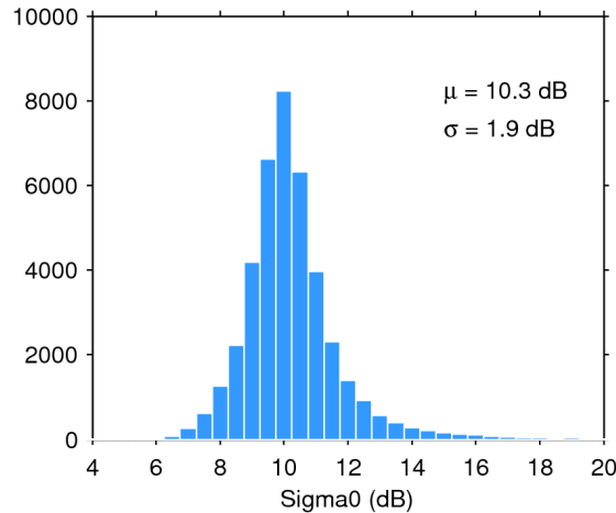
Figure 25. Histogram of flag-valid sigma0 over oceans and lakes for 11/04/2019. The mean ( \mu ) and standard deviation ( \sigma ) are also shown. Note that values outside [4 20] dB are excluded from the histogram for the sake of readability but not from the computation of \mu and \sigma .
