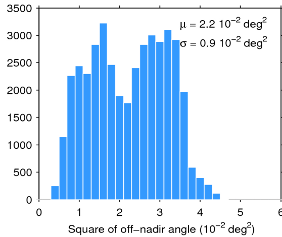
Figure 39. Histogram of flag-valid mispointing over oceans and lakes for 11/04/2019. The mean ( \mu ) and standard deviation ( \sigma ) are also shown. Note that values larger than 6 \cdot 10^{-2} \text{ deg}^2 are excluded from the histogram for the sake of readability but not from the computation of \mu and \sigma .
