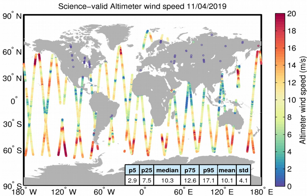
Figure 34. Geographical distribution of science-valid wind data over oceans and lakes for 11/04/2019. The statistical values shown in the table refer to the wind in m/s and are calculated over all measurements shown in the figure. Gray circles denote records that have been rejected based on the editing criteria described in Table 5.
