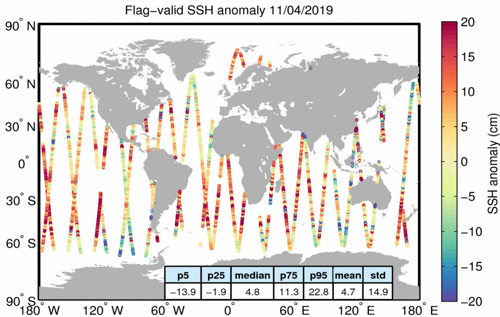
Figure 5. Geographical distribution of flag-valid 1-Hz SSH anomaly data over oceans and lakes for 11/04/2019. The statistical values shown in the table refer to the SSH anomaly in cm and are calculated over all measurements shown in the figure.
