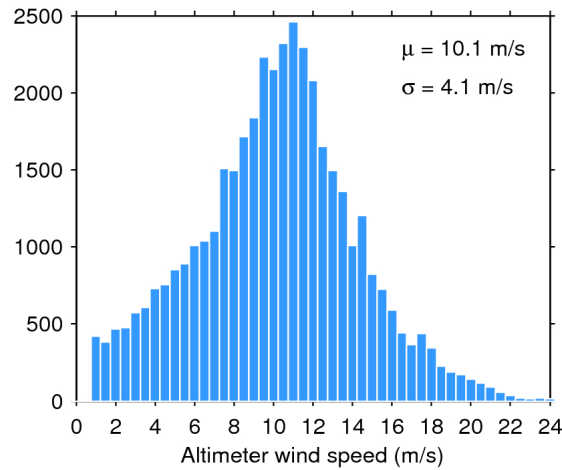
Figure 33. Histogram of flag-valid wind over oceans and lakes for 11/04/2019. The mean ( \mu ) and standard deviation ( \sigma ) are also shown. Note that values larger than 24 m/s are excluded from the histogram for the sake of readability but not from the computation of \mu and \sigma .
