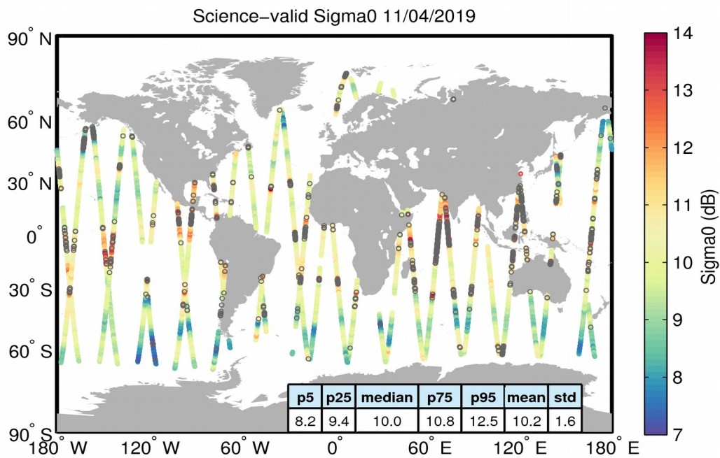
Figure 27. Geographical distribution of science-valid sigma0 data over oceans and lakes for 11/04/2019. The statistical values shown in the table refer to the sigma0 in dB and are calculated over all measurements shown in the figure. Gray circles denote records that have been rejected based on the editing criteria described in Table 4.
