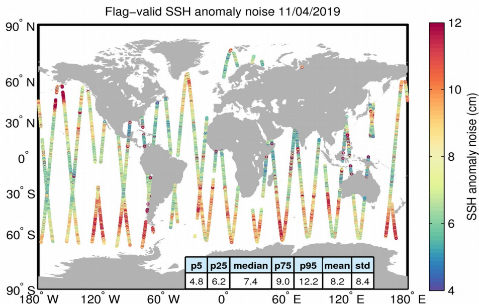
Figure 8. Geographical distribution of flag-valid 20-Hz SSH anomaly measurement noise over oceans and lakes for 11/04/2019. The statistical values shown in the table refer to the SSH anomaly noise and are calculated over all measurements shown in the figure.
