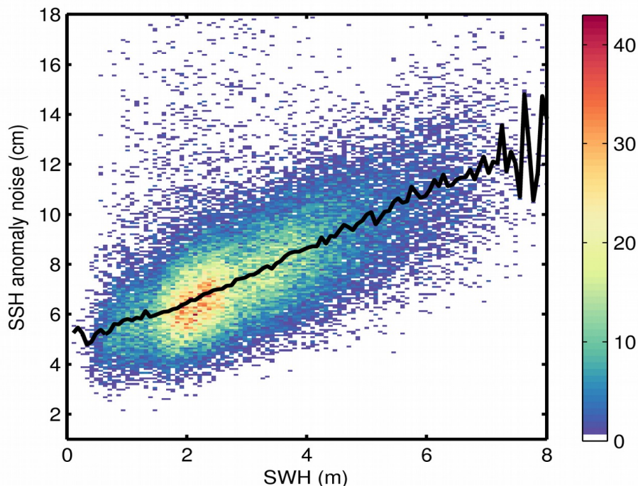
Figure 9. 2D histogram showing flag-valid SSH anomaly noise as a function of SWH for 11/04/2019. The black line denotes the median SSH anomaly noise as a function of SWH.
