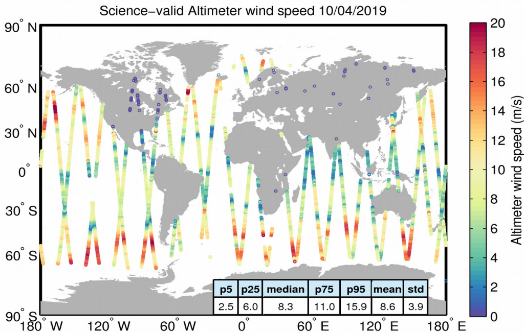
Figure 34. Geographical distribution of science-valid wind data over oceans and lakes for 10/04/2019. The statistical values shown in the table refer to the wind in m/s and are calculated over all measurements shown in the figure. Gray circles denote records that have been rejected based on the editing criteria described in Table 5.
