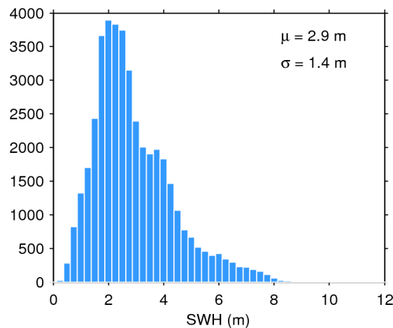
Figure 20. Histogram of science-valid SWH over oceans and lakes for 10/04/2019. The mean ( \mu ) and standard deviation ( \sigma ) are also shown. Note that values larger than 12 m are excluded from the histogram for the sake of readability but not from the computation of \mu and \sigma .
