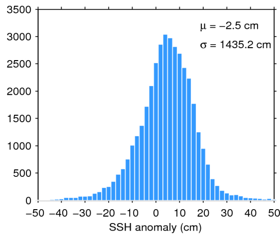
Figure 7. Histogram of flag-valid SSH anomaly over oceans and lakes for 10/04/2019. The mean ( \mu ) and standard deviation ( \sigma ) are also shown. Note that values outside [-50\ 50] cm are excluded from the histogram for the sake of readability but not from the computation of \mu and \sigma .
