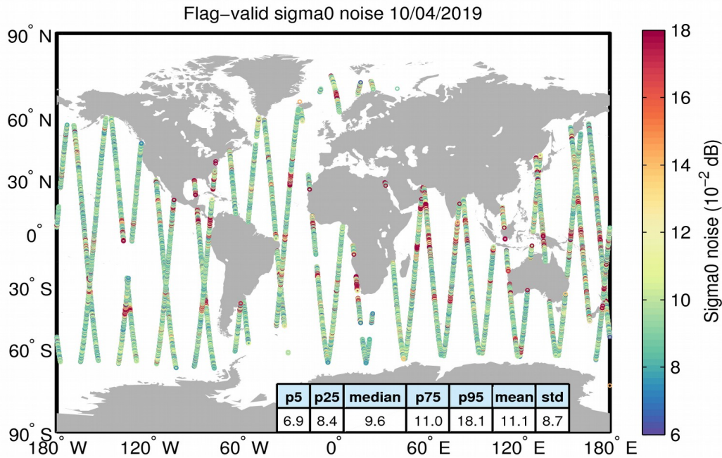
Figure 26. Geographical distribution of flag-valid 20-Hz sigma0 measurement noise over oceans and lakes for 10/04/2019. The statistical values shown in the table refer to the sigma0 noise and are calculated over all measurements shown in the figure.
