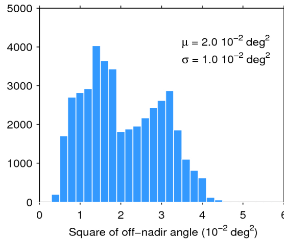
Figure 39. Histogram of flag-valid mispointing over oceans and lakes for 10/04/2019. The mean ( \mu ) and standard deviation ( \sigma ) are also shown. Note that values larger than 6 \cdot 10^{-2} \text{ deg}^2 are excluded from the histogram for the sake of readability but not from the computation of \mu and \sigma .
