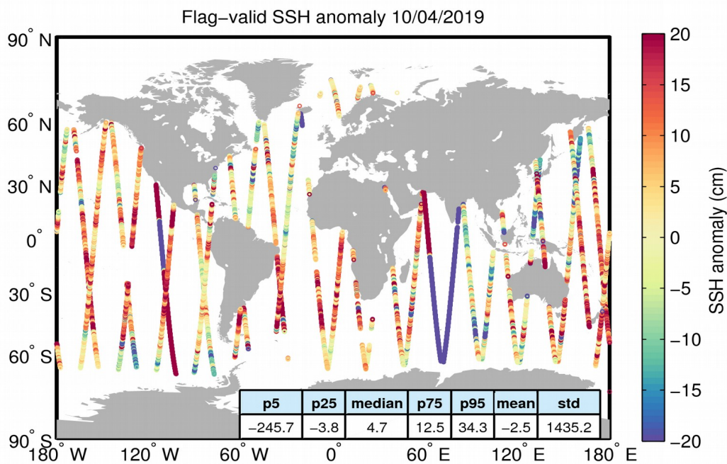
Figure 5. Geographical distribution of flag-valid 1-Hz SSH anomaly data over oceans and lakes for 10/04/2019. The statistical values shown in the table refer to the SSH anomaly in cm and are calculated over all measurements shown in the figure.
