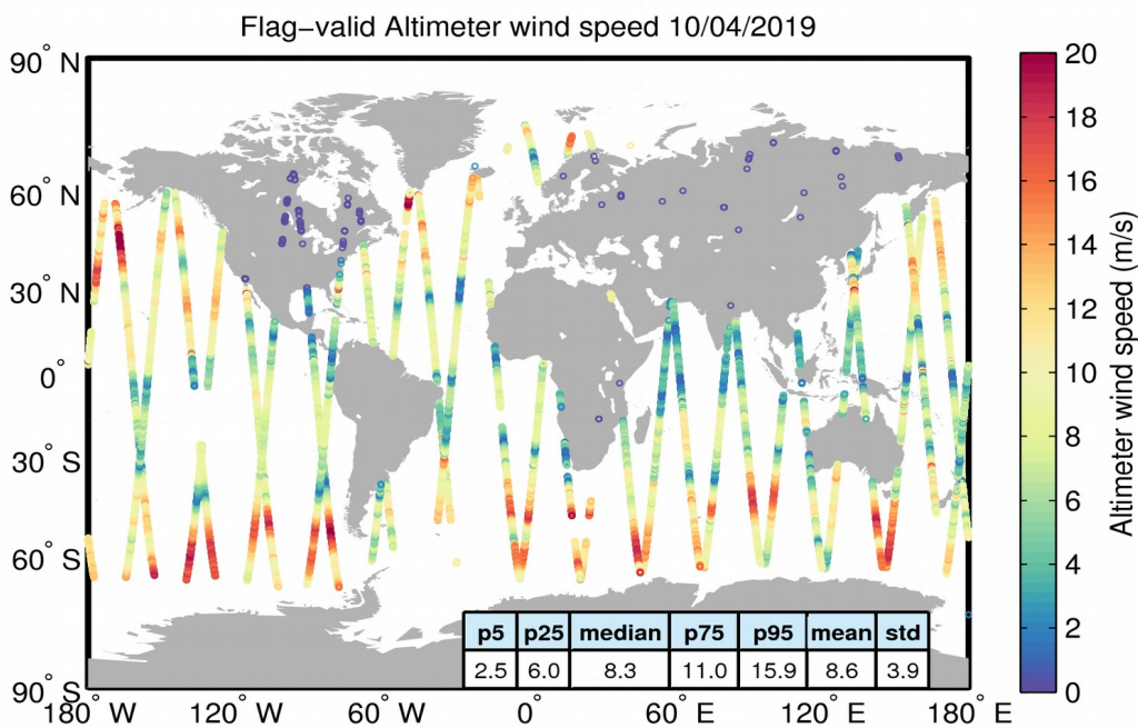
Figure 31. Geographical distribution of flag-valid wind data over oceans and lakes for 10/04/2019. The statistical values shown in the table refer to the wind in m/s and are calculated over all measurements shown in the figure.
