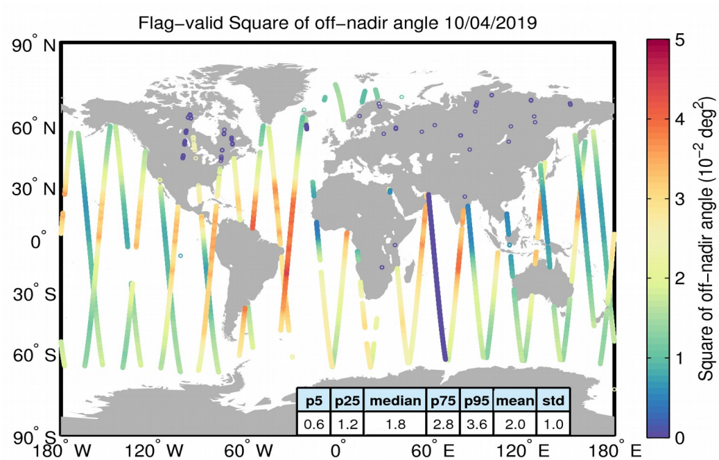
Figure 37. Geographical distribution of flag-valid mispointing data over oceans and lakes for 10/04/2019. The statistical values shown in the table refer to the mispointing in 10^{-2} deg 2 and are calculated over all measurements shown in the figure.
