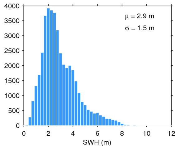
Figure 17. Histogram of flag-valid SWH over oceans and lakes for 10/04/2019. The mean ( \mu ) and standard deviation ( \sigma ) are also shown. Note that values larger than 12 m are excluded from the histogram for the sake of readability but not from the computation of \mu and \sigma .
