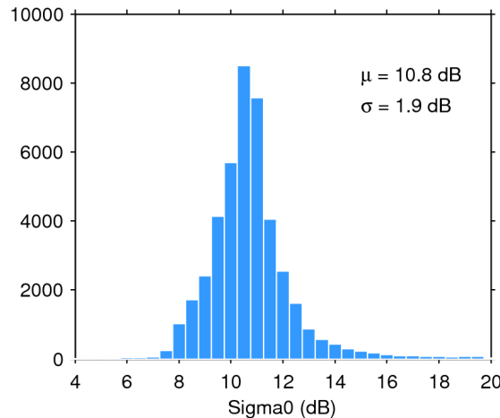
Figure 25. Histogram of flag-valid sigma0 over oceans and lakes for 10/04/2019. The mean ( \mu ) and standard deviation ( \sigma ) are also shown. Note that values outside [4 20] dB are excluded from the histogram for the sake of readability but not from the computation of \mu and \sigma .
