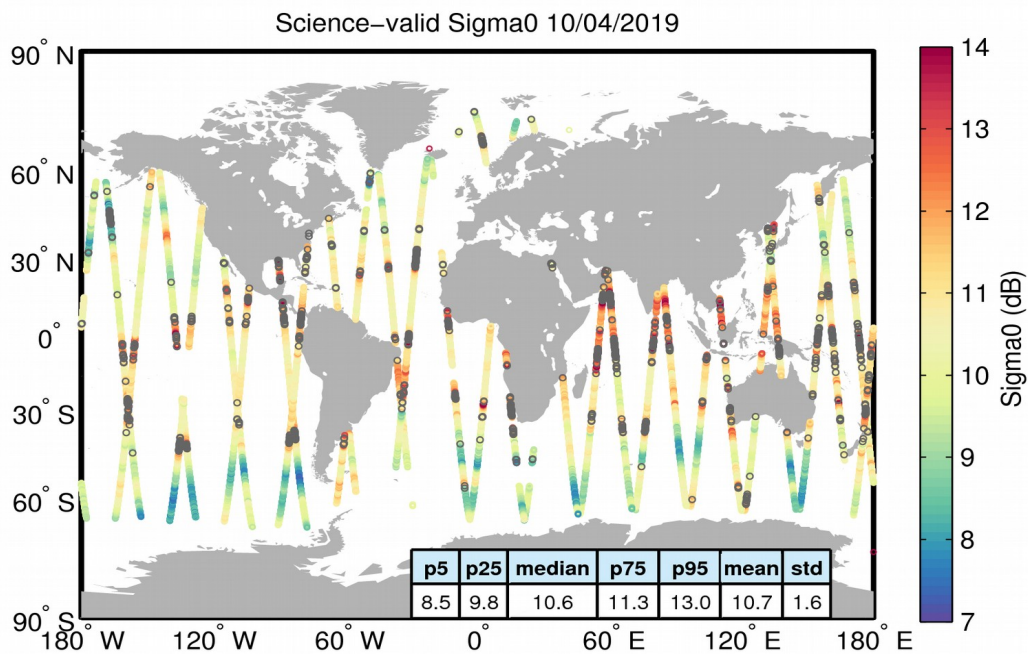
Figure 27. Geographical distribution of science-valid sigma0 data over oceans and lakes for 10/04/2019. The statistical values shown in the table refer to the sigma0 in dB and are calculated over all measurements shown in the figure. Gray circles denote records that have been rejected based on the editing criteria described in Table 4.
