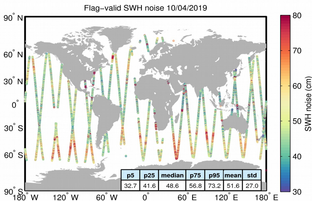
Figure 18. Geographical distribution of flag-valid 20-Hz SWH measurement noise over oceans and lakes for 10/04/2019. The statistical values shown in the table refer to the SWH noise and are calculated over all measurements shown in the figure.
