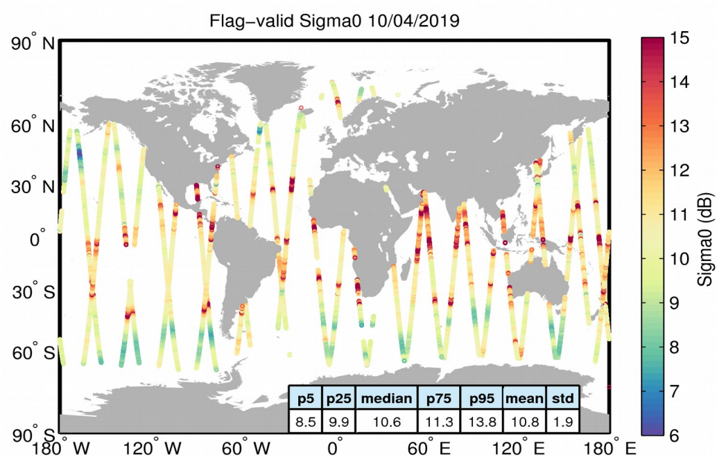
Figure 23. Geographical distribution of flag-valid sigma0 data over oceans and lakes for 10/04/2019. The statistical values shown in the table refer to the sigma0 in dB and are calculated over all measurements shown in the figure.
