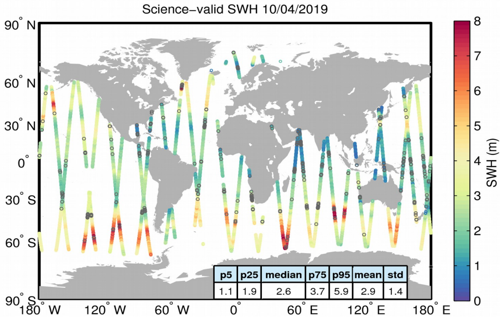
Figure 19. Geographical distribution of science-valid SWH data over oceans and lakes for 10/04/2019. The statistical values shown in the table refer to the SWH in m and are calculated over all measurements shown in the figure. Gray circles denote records that have been rejected based on the editing criteria described in Table 3.
