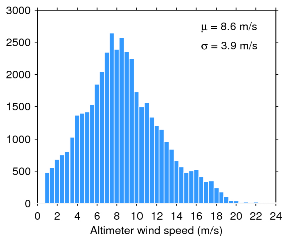
Figure 35. Histogram of science-valid wind over oceans and lakes for 10/04/2019. The mean ( \mu ) and standard deviation ( \sigma ) are also shown. Note that values larger than 24 m/s are excluded from the histogram for the sake of readability but not from the computation of \mu and \sigma .
