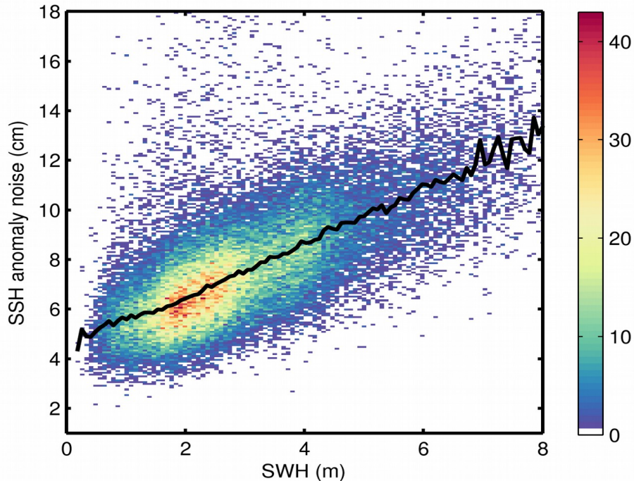
Figure 9. 2D histogram showing flag-valid SSH anomaly noise as a function of SWH for 10/04/2019. The black line denotes the median SSH anomaly noise as a function of SWH.
