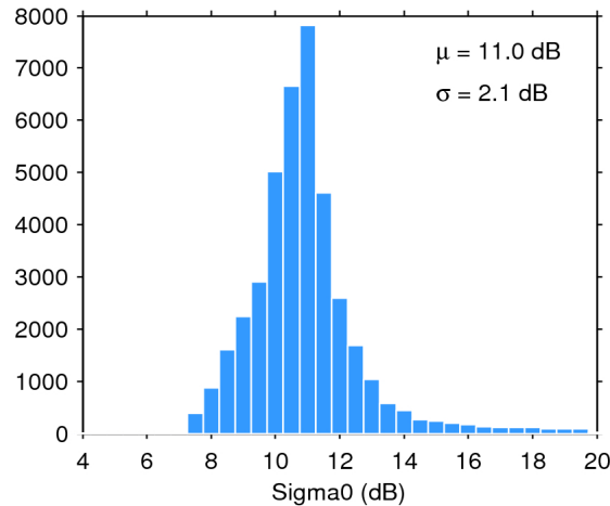
Figure 25. Histogram of flag-valid sigma0 over oceans and lakes for 09/04/2019. The mean ( \mu ) and standard deviation ( \sigma ) are also shown. Note that values outside [4 20] dB are excluded from the histogram for the sake of readability but not from the computation of \mu and \sigma .
