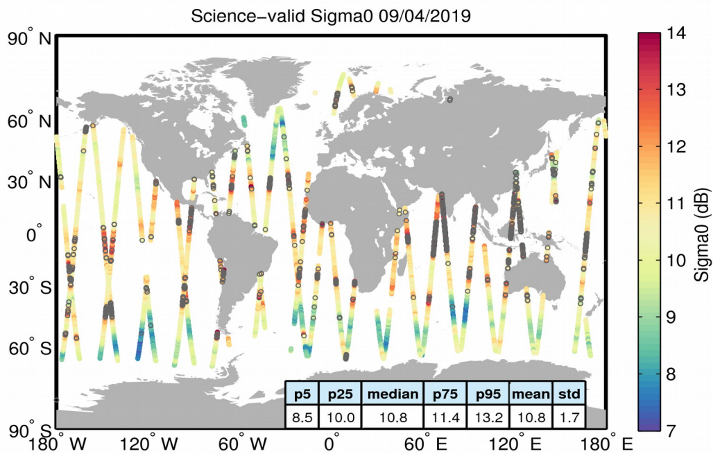
Figure 27. Geographical distribution of science-valid sigma0 data over oceans and lakes for 09/04/2019. The statistical values shown in the table refer to the sigma0 in dB and are calculated over all measurements shown in the figure. Gray circles denote records that have been rejected based on the editing criteria described in Table 4.
