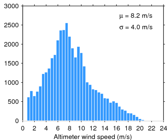
Figure 35. Histogram of science-valid wind over oceans and lakes for 09/04/2019. The mean ( \mu ) and standard deviation ( \sigma ) are also shown. Note that values larger than 24 m/s are excluded from the histogram for the sake of readability but not from the computation of \mu and \sigma .
