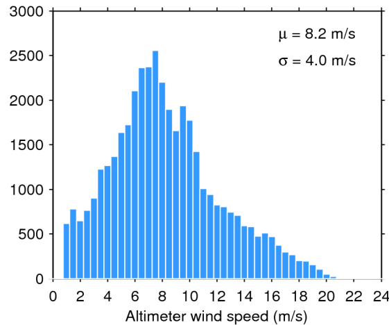
Figure 33. Histogram of flag-valid wind over oceans and lakes for 09/04/2019. The mean ( \mu ) and standard deviation ( \sigma ) are also shown. Note that values larger than 24 m/s are excluded from the histogram for the sake of readability but not from the computation of \mu and \sigma .
