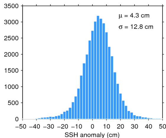
Figure 11. Histogram of science-valid SSH anomaly over oceans and lakes for 09/04/2019. The mean ( \mu ) and standard deviation ( \sigma ) are also shown. Note that values outside [-50 50] cm are excluded from the histogram for the sake of readability but not from the computation of \mu and \sigma .
