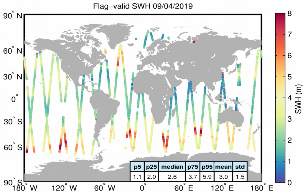
Figure 15. Geographical distribution of flag-valid SWH data over oceans and lakes for 09/04/2019. The statistical values shown in the table refer to the SWH in m and are calculated over all measurements shown in the figure.
