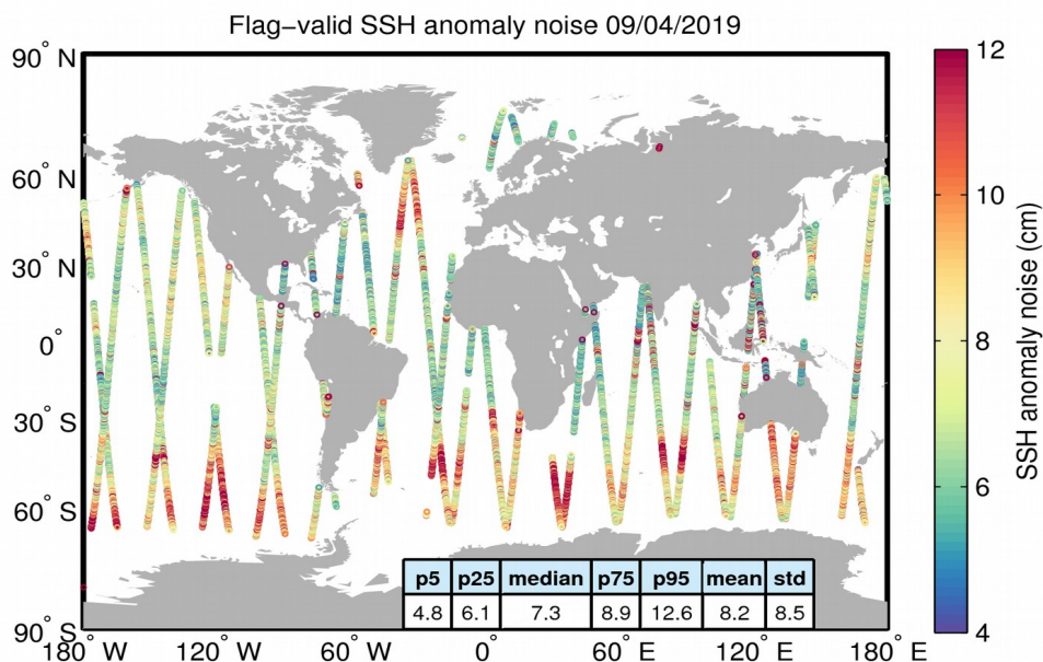
Figure 8. Geographical distribution of flag-valid 20-Hz SSH anomaly measurement noise over oceans and lakes for 09/04/2019. The statistical values shown in the table refer to the SSH anomaly noise and are calculated over all measurements shown in the figure.
