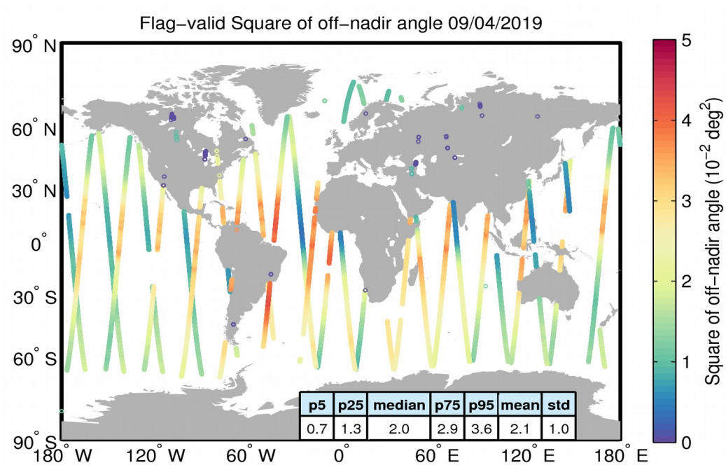
Figure 37. Geographical distribution of flag-valid mispointing data over oceans and lakes for 09/04/2019. The statistical values shown in the table refer to the mispointing in 10^{-2} \text{ deg}^2 and are calculated over all measurements shown in the figure.
