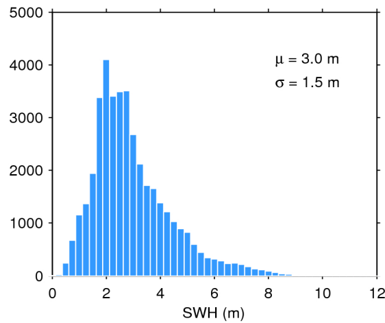
Figure 17. Histogram of flag-valid SWH over oceans and lakes for 09/04/2019. The mean ( \mu ) and standard deviation ( \sigma ) are also shown. Note that values larger than 12 m are excluded from the histogram for the sake of readability but not from the computation of \mu and \sigma .
