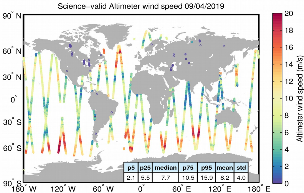
Figure 34. Geographical distribution of science-valid wind data over oceans and lakes for 09/04/2019. The statistical values shown in the table refer to the wind in m/s and are calculated over all measurements shown in the figure. Gray circles denote records that have been rejected based on the editing criteria described in Table 5.
