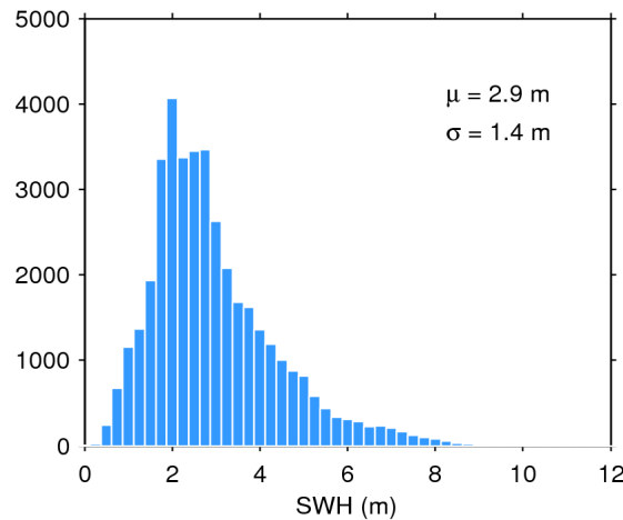
Figure 20. Histogram of science-valid SWH over oceans and lakes for 09/04/2019. The mean ( \mu ) and standard deviation ( \sigma ) are also shown. Note that values larger than 12 m are excluded from the histogram for the sake of readability but not from the computation of \mu and \sigma .
