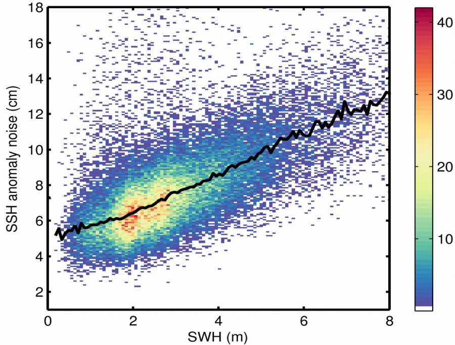
Figure 9. 2D histogram showing flag-valid SSH anomaly noise as a function of SWH for 09/04/2019. The black line denotes the median SSH anomaly noise as a function of SWH.
