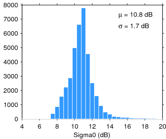
Figure 28. Histogram of science-valid sigma0 over oceans and lakes for 09/04/2019. The mean ( \mu ) and standard deviation ( \sigma ) are also shown. Note that values outside [4 20] dB are excluded from the histogram for the sake of readability but not from the computation of \mu and \sigma .
