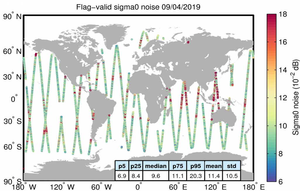
Figure 26. Geographical distribution of flag-valid 20-Hz sigma0 measurement noise over oceans and lakes for 09/04/2019. The statistical values shown in the table refer to the sigma0 noise and are calculated over all measurements shown in the figure.
