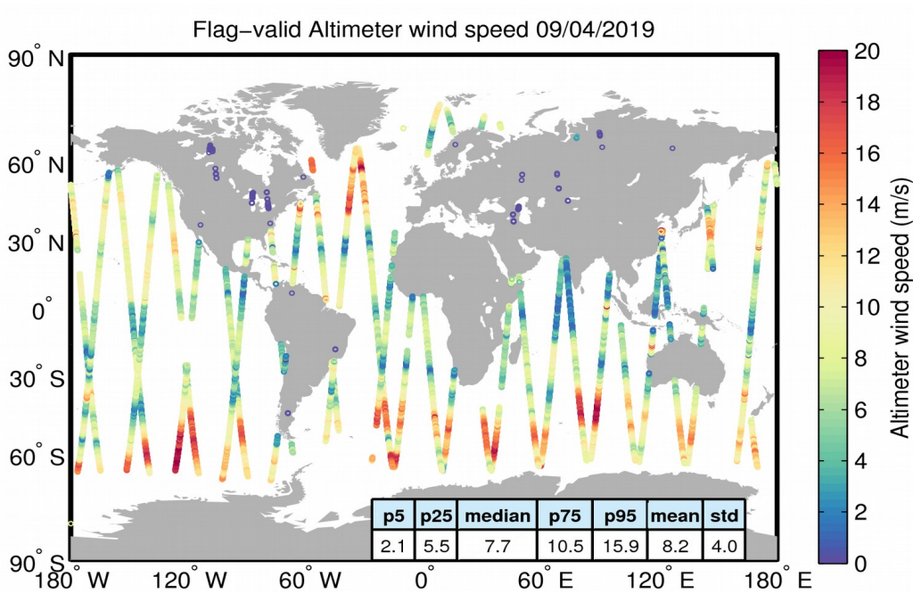
Figure 31. Geographical distribution of flag-valid wind data over oceans and lakes for 09/04/2019. The statistical values shown in the table refer to the wind in m/s and are calculated over all measurements shown in the figure.
