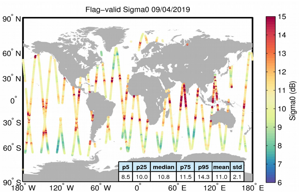
Figure 23. Geographical distribution of flag-valid sigma0 data over oceans and lakes for 09/04/2019. The statistical values shown in the table refer to the sigma0 in dB and are calculated over all measurements shown in the figure.
