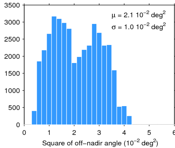
Figure 39. Histogram of flag-valid mispointing over oceans and lakes for 09/04/2019. The mean ( \mu ) and standard deviation ( \sigma ) are also shown. Note that values larger than 6 \cdot 10^{-2} \text{ deg}^2 are excluded from the histogram for the sake of readability but not from the computation of \mu and \sigma .
