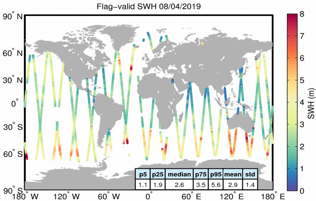
Figure 15. Geographical distribution of flag-valid SWH data over oceans and lakes for 08/04/2019. The statistical values shown in the table refer to the SWH in m and are calculated over all measurements shown in the figure.
