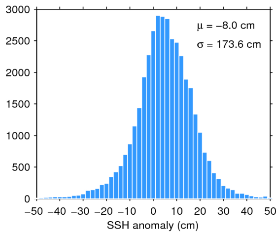
Figure 7. Histogram of flag-valid SSH anomaly over oceans and lakes for 08/04/2019. The mean ( \mu ) and standard deviation ( \sigma ) are also shown. Note that values outside [-50 50] cm are excluded from the histogram for the sake of readability but not from the computation of \mu and \sigma .
