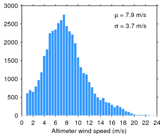
Figure 35. Histogram of science-valid wind over oceans and lakes for 08/04/2019. The mean ( \mu ) and standard deviation ( \sigma ) are also shown. Note that values larger than 24 m/s are excluded from the histogram for the sake of readability but not from the computation of \mu and \sigma .
