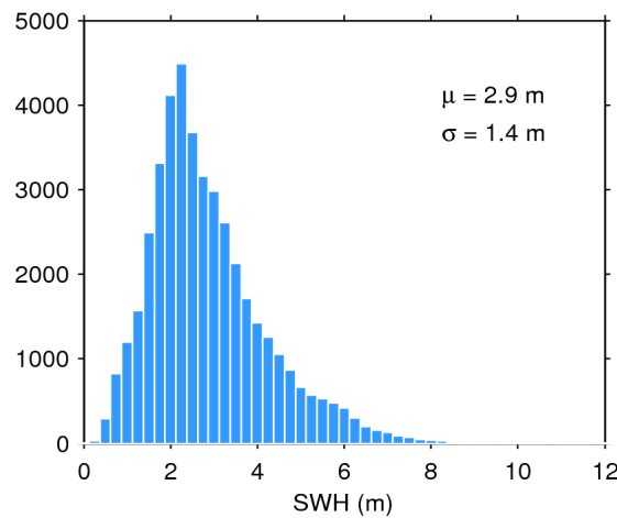
Figure 17. Histogram of flag-valid SWH over oceans and lakes for 08/04/2019. The mean ( \mu ) and standard deviation ( \sigma ) are also shown. Note that values larger than 12 m are excluded from the histogram for the sake of readability but not from the computation of \mu and \sigma .
