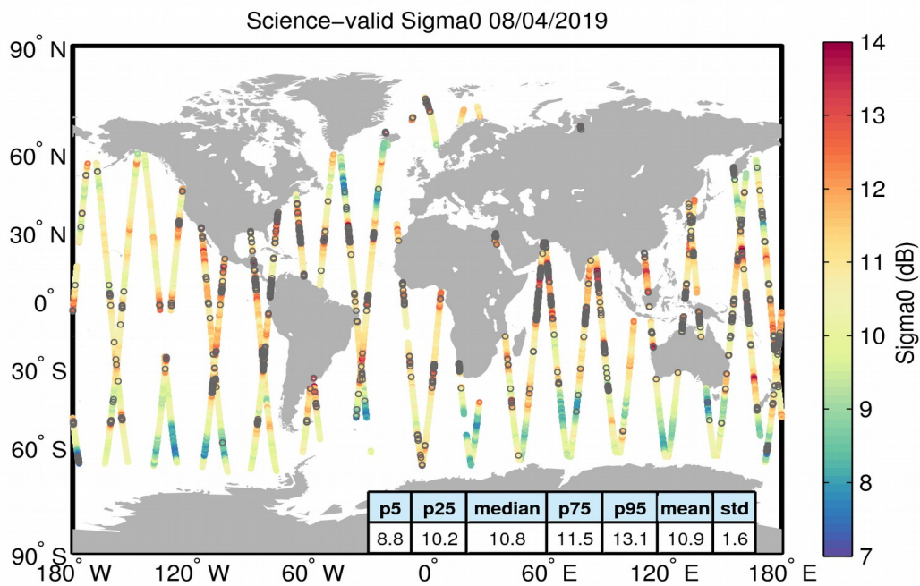
Figure 27. Geographical distribution of science-valid sigma0 data over oceans and lakes for 08/04/2019. The statistical values shown in the table refer to the sigma0 in dB and are calculated over all measurements shown in the figure. Gray circles denote records that have been rejected based on the editing criteria described in Table 4.
