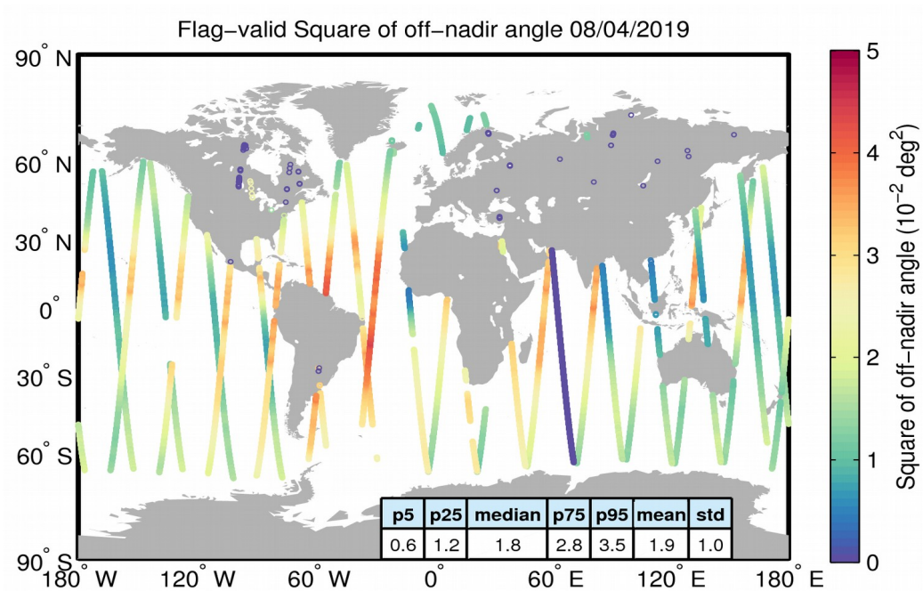
Figure 37. Geographical distribution of flag-valid mispointing data over oceans and lakes for 08/04/2019. The statistical values shown in the table refer to the mispointing in 10^{-2} \text{ deg}^2 and are calculated over all measurements shown in the figure.
