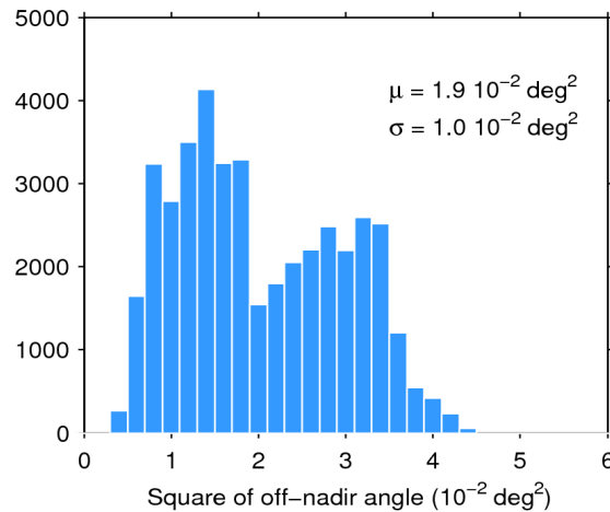
Figure 39. Histogram of flag-valid mispointing over oceans and lakes for 08/04/2019. The mean ( \mu ) and standard deviation ( \sigma ) are also shown. Note that values larger than 6 \cdot 10^{-2} \text{ deg}^2 are excluded from the histogram for the sake of readability but not from the computation of \mu and \sigma .
