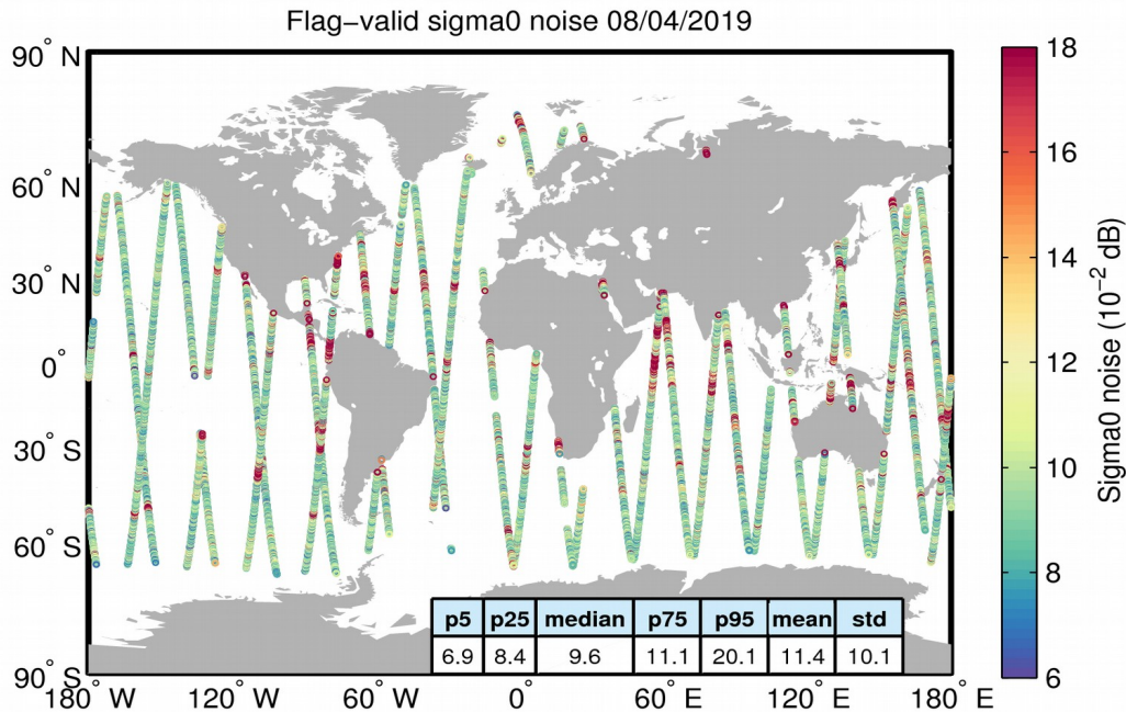
Figure 26. Geographical distribution of flag-valid 20-Hz sigma0 measurement noise over oceans and lakes for 08/04/2019. The statistical values shown in the table refer to the sigma0 noise and are calculated over all measurements shown in the figure.
