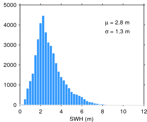
Figure 20. Histogram of science-valid SWH over oceans and lakes for 08/04/2019. The mean ( \mu ) and standard deviation ( \sigma ) are also shown. Note that values larger than 12 m are excluded from the histogram for the sake of readability but not from the computation of \mu and \sigma .
