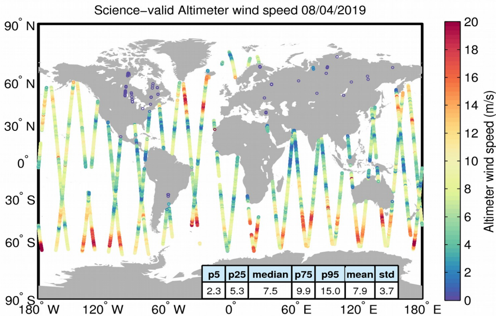
Figure 34. Geographical distribution of science-valid wind data over oceans and lakes for 08/04/2019. The statistical values shown in the table refer to the wind in m/s and are calculated over all measurements shown in the figure. Gray circles denote records that have been rejected based on the editing criteria described in Table 5.
