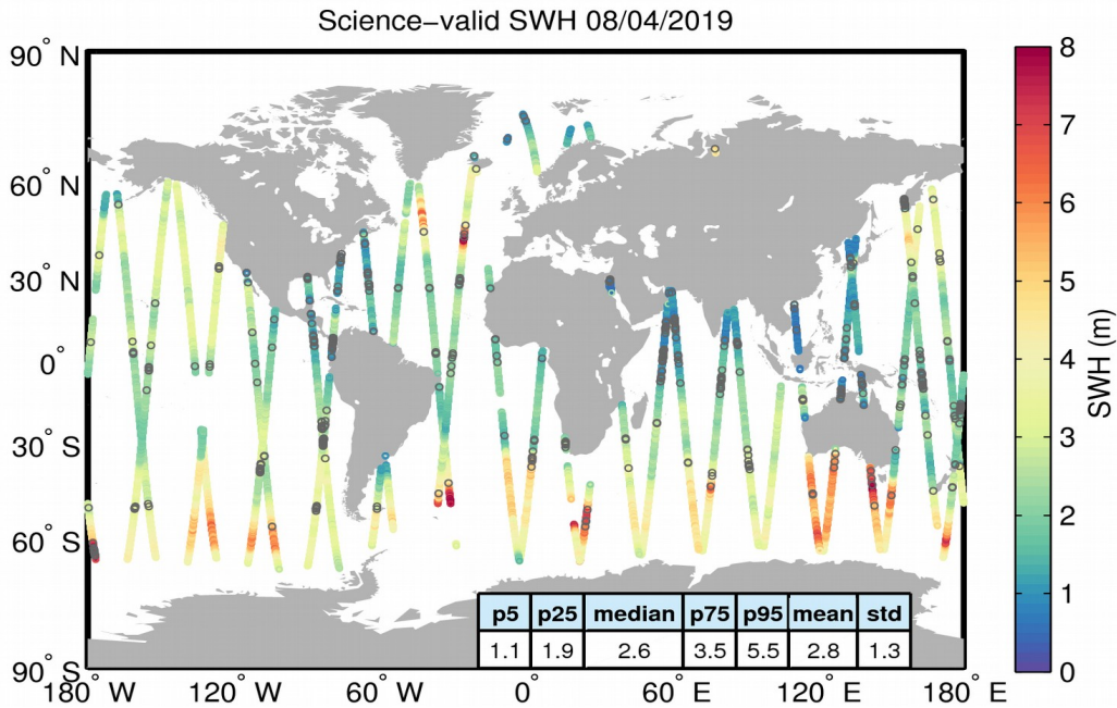
Figure 19. Geographical distribution of science-valid SWH data over oceans and lakes for 08/04/2019. The statistical values shown in the table refer to the SWH in m and are calculated over all measurements shown in the figure. Gray circles denote records that have been rejected based on the editing criteria described in Table 3.
