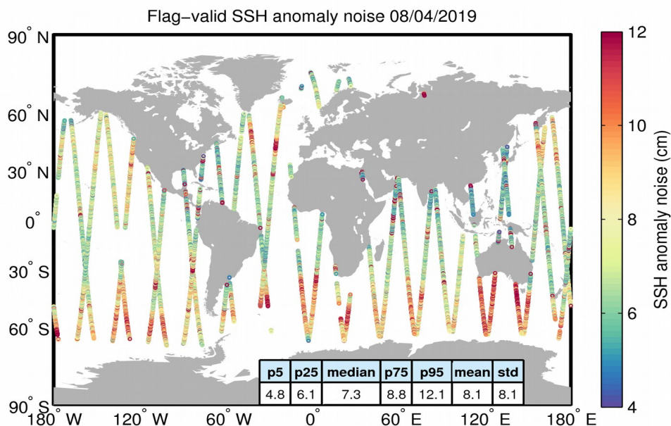
Figure 8. Geographical distribution of flag-valid 20-Hz SSH anomaly measurement noise over oceans and lakes for 08/04/2019. The statistical values shown in the table refer to the SSH anomaly noise and are calculated over all measurements shown in the figure.
