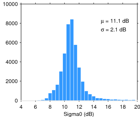
Figure 25. Histogram of flag-valid sigma0 over oceans and lakes for 08/04/2019. The mean ( \mu ) and standard deviation ( \sigma ) are also shown. Note that values outside [4 20] dB are excluded from the histogram for the sake of readability but not from the computation of \mu and \sigma .
