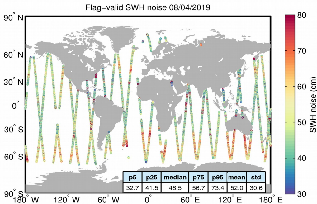
Figure 18. Geographical distribution of flag-valid 20-Hz SWH measurement noise over oceans and lakes for 08/04/2019. The statistical values shown in the table refer to the SWH noise and are calculated over all measurements shown in the figure.
