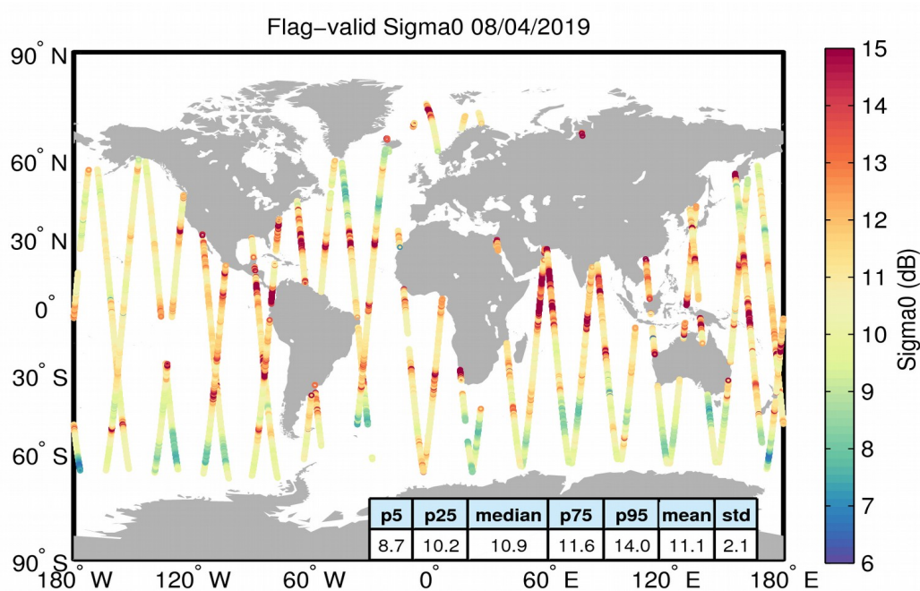
Figure 23. Geographical distribution of flag-valid sigma0 data over oceans and lakes for 08/04/2019. The statistical values shown in the table refer to the sigma0 in dB and are calculated over all measurements shown in the figure.
