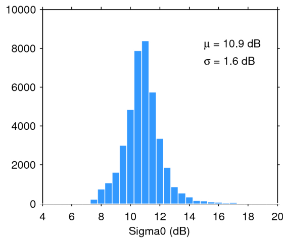
Figure 28. Histogram of science-valid sigma0 over oceans and lakes for 08/04/2019. The mean ( \mu ) and standard deviation ( \sigma ) are also shown. Note that values outside [4 20] dB are excluded from the histogram for the sake of readability but not from the computation of \mu and \sigma .
