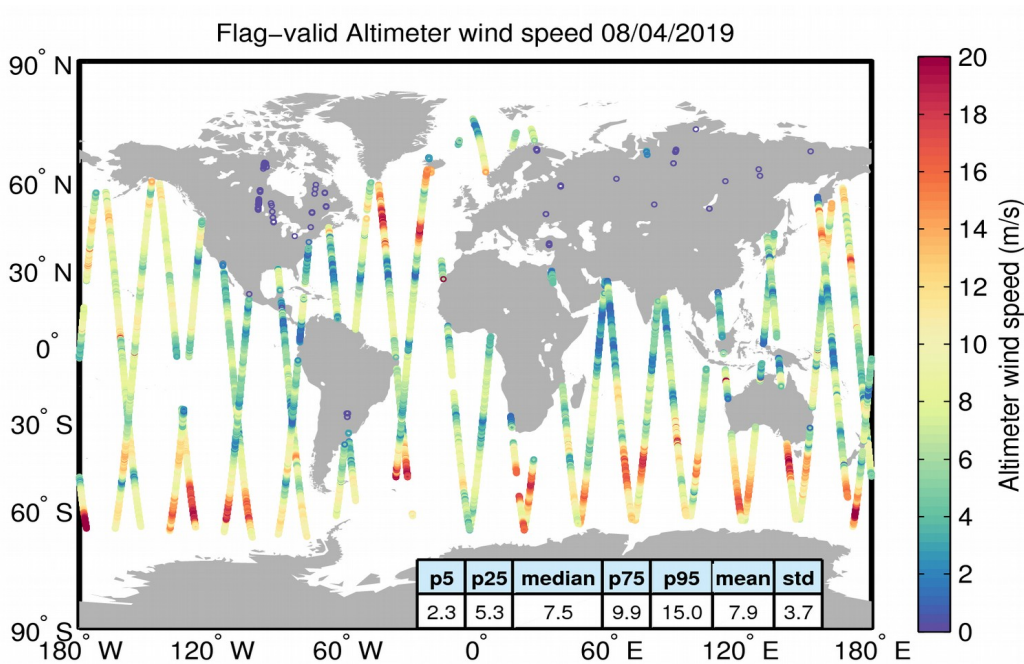
Figure 31. Geographical distribution of flag-valid wind data over oceans and lakes for 08/04/2019. The statistical values shown in the table refer to the wind in m/s and are calculated over all measurements shown in the figure.
