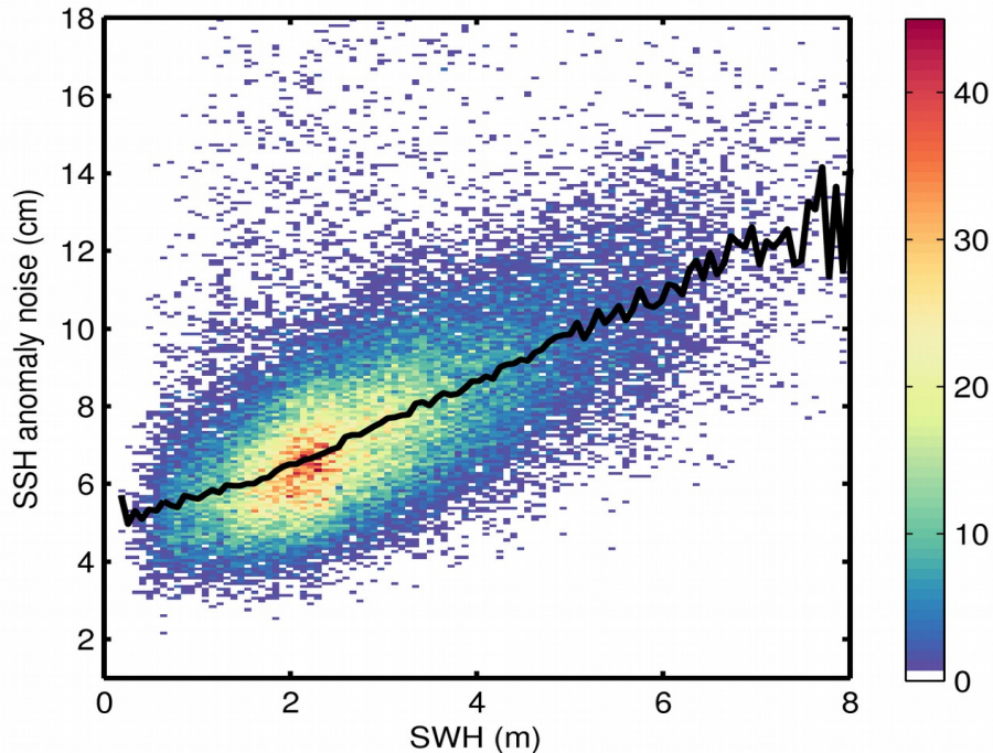
Figure 9. 2D histogram showing flag-valid SSH anomaly noise as a function of SWH for 08/04/2019. The black line denotes the median SSH anomaly noise as a function of SWH.
