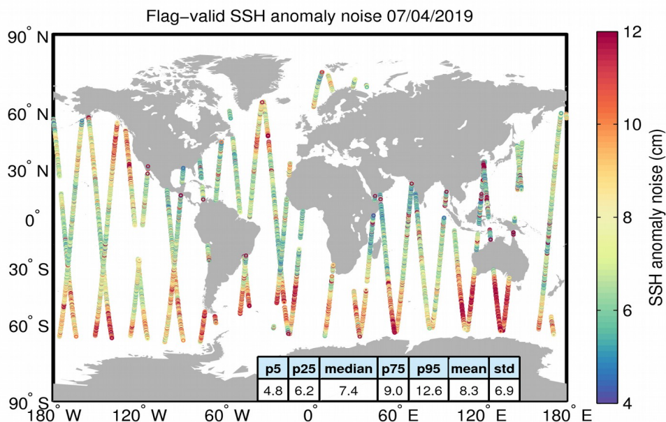
Figure 8. Geographical distribution of flag-valid 20-Hz SSH anomaly measurement noise over oceans and lakes for 07/04/2019. The statistical values shown in the table refer to the SSH anomaly noise and are calculated over all measurements shown in the figure.
