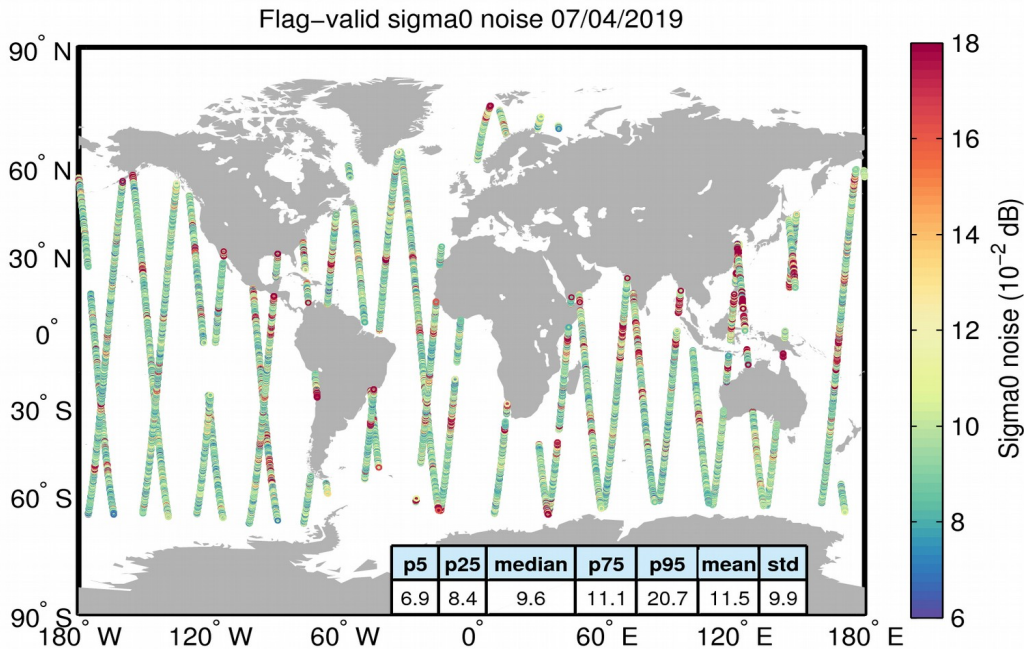
Figure 26. Geographical distribution of flag-valid 20-Hz sigma0 measurement noise over oceans and lakes for 07/04/2019. The statistical values shown in the table refer to the sigma0 noise and are calculated over all measurements shown in the figure.
