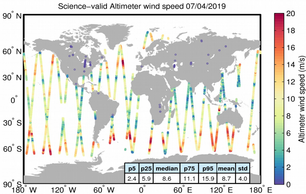
Figure 34. Geographical distribution of science-valid wind data over oceans and lakes for 07/04/2019. The statistical values shown in the table refer to the wind in m/s and are calculated over all measurements shown in the figure. Gray circles denote records that have been rejected based on the editing criteria described in Table 5.
