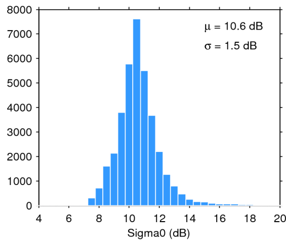
Figure 28. Histogram of science-valid sigma0 over oceans and lakes for 07/04/2019. The mean ( \mu ) and standard deviation ( \sigma ) are also shown. Note that values outside [4 20] dB are excluded from the histogram for the sake of readability but not from the computation of \mu and \sigma .
