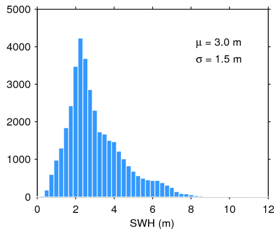
Figure 20. Histogram of science-valid SWH over oceans and lakes for 07/04/2019. The mean ( \mu ) and standard deviation ( \sigma ) are also shown. Note that values larger than 12 m are excluded from the histogram for the sake of readability but not from the computation of \mu and \sigma .
