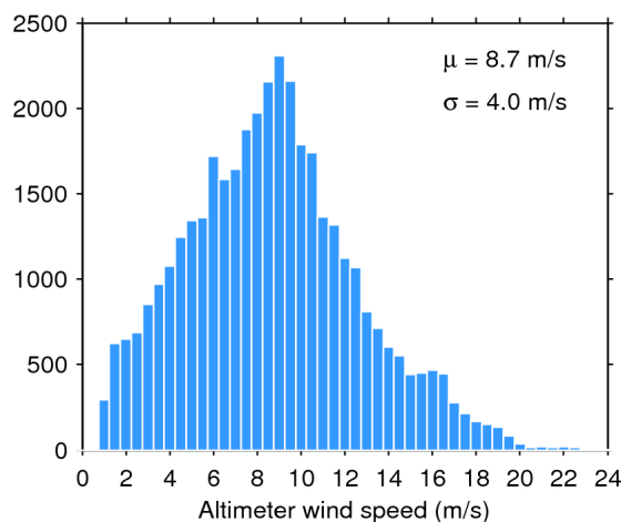
Figure 33. Histogram of flag-valid wind over oceans and lakes for 07/04/2019. The mean ( \mu ) and standard deviation ( \sigma ) are also shown. Note that values larger than 24 m/s are excluded from the histogram for the sake of readability but not from the computation of \mu and \sigma .
