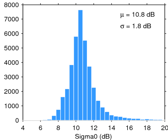
Figure 25. Histogram of flag-valid sigma0 over oceans and lakes for 07/04/2019. The mean ( \mu ) and standard deviation ( \sigma ) are also shown. Note that values outside [4 20] dB are excluded from the histogram for the sake of readability but not from the computation of \mu and \sigma .
