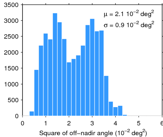
Figure 39. Histogram of flag-valid mispointing over oceans and lakes for 07/04/2019. The mean ( \mu ) and standard deviation ( \sigma ) are also shown. Note that values larger than 6 \cdot 10^{-2} \text{ deg}^2 are excluded from the histogram for the sake of readability but not from the computation of \mu and \sigma .
