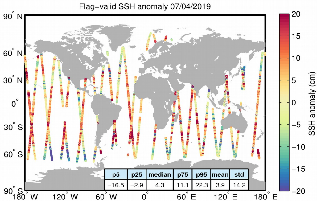
Figure 5. Geographical distribution of flag-valid 1-Hz SSH anomaly data over oceans and lakes for 07/04/2019. The statistical values shown in the table refer to the SSH anomaly in cm and are calculated over all measurements shown in the figure.
