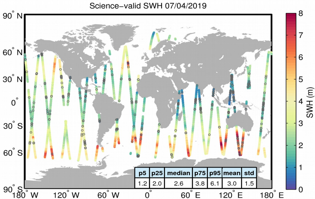
Figure 19. Geographical distribution of science-valid SWH data over oceans and lakes for 07/04/2019. The statistical values shown in the table refer to the SWH in m and are calculated over all measurements shown in the figure. Gray circles denote records that have been rejected based on the editing criteria described in Table 3.
