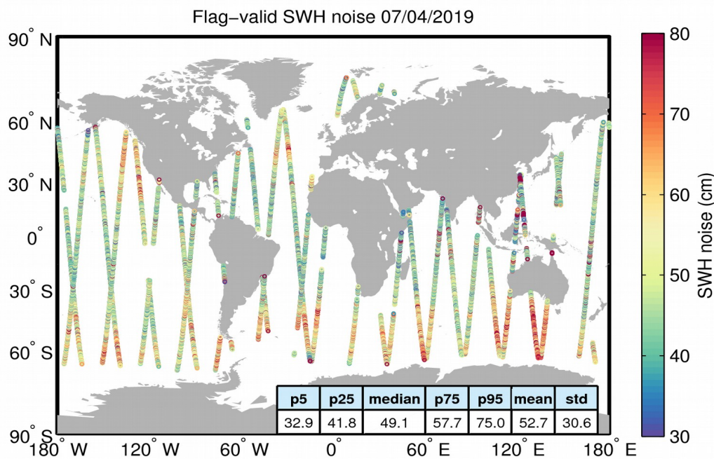
Figure 18. Geographical distribution of flag-valid 20-Hz SWH measurement noise over oceans and lakes for 07/04/2019. The statistical values shown in the figure refer to the SWH noise and are calculated over all measurements shown in the figure.
