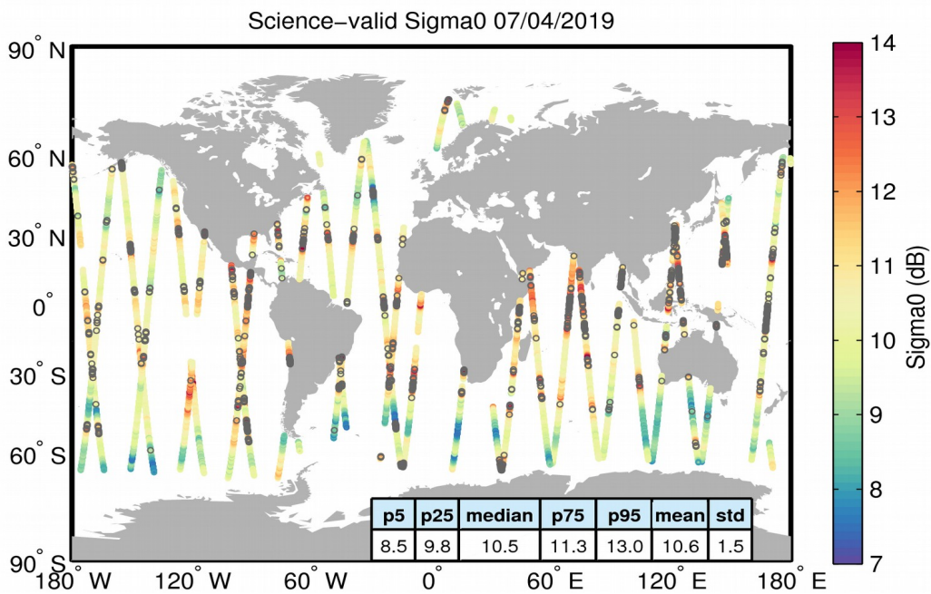
Figure 27. Geographical distribution of science-valid sigma0 data over oceans and lakes for 07/04/2019. The statistical values shown in the table refer to the sigma0 in dB and are calculated over all measurements shown in the figure. Gray circles denote records that have been rejected based on the editing criteria described in Table 4.
