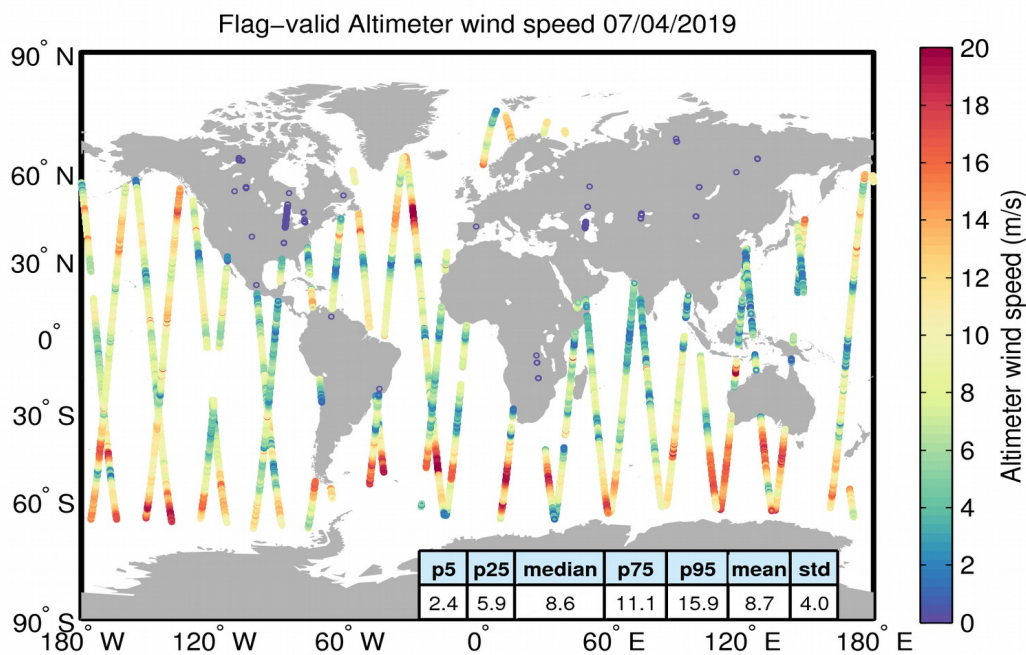
Figure 31. Geographical distribution of flag-valid wind data over oceans and lakes for 07/04/2019. The statistical values shown in the table refer to the wind in m/s and are calculated over all measurements shown in the figure.
