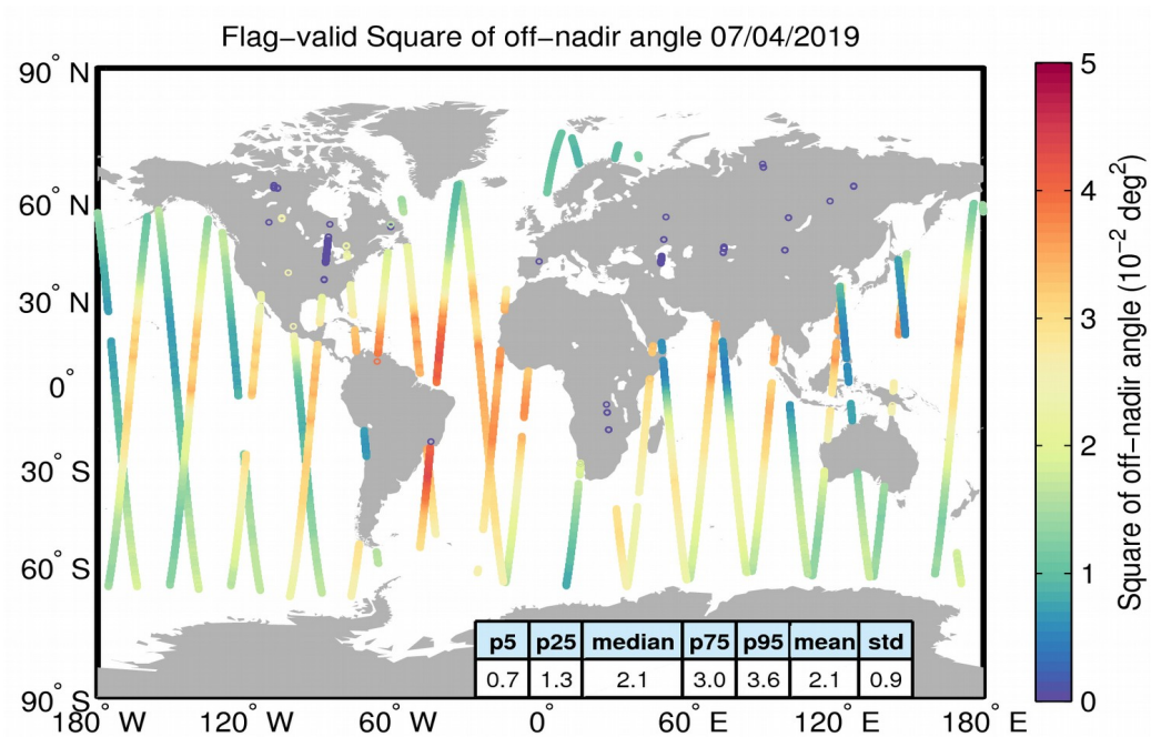
Figure 37. Geographical distribution of flag-valid mispointing data over oceans and lakes for 07/04/2019. The statistical values shown in the table refer to the mispointing in 10^{-2} deg 2 and are calculated over all measurements shown in the figure.
