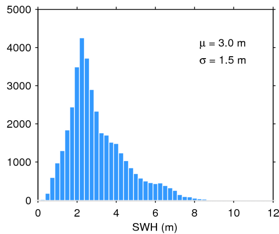
Figure 17. Histogram of flag-valid SWH over oceans and lakes for 07/04/2019. The mean ( \mu ) and standard deviation ( \sigma ) are also shown. Note that values larger than 12 m are excluded from the histogram for the sake of readability but not from the computation of \mu and \sigma .
