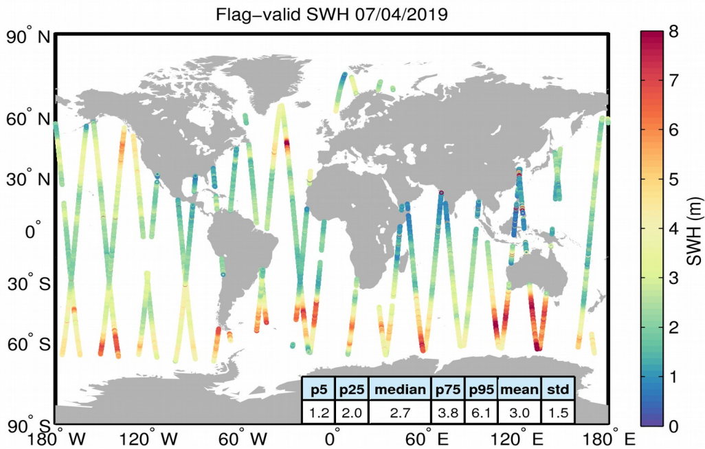
Figure 15. Geographical distribution of flag-valid SWH data over oceans and lakes for 07/04/2019. The statistical values shown in the table refer to the SWH in m and are calculated over all measurements shown in the figure.
