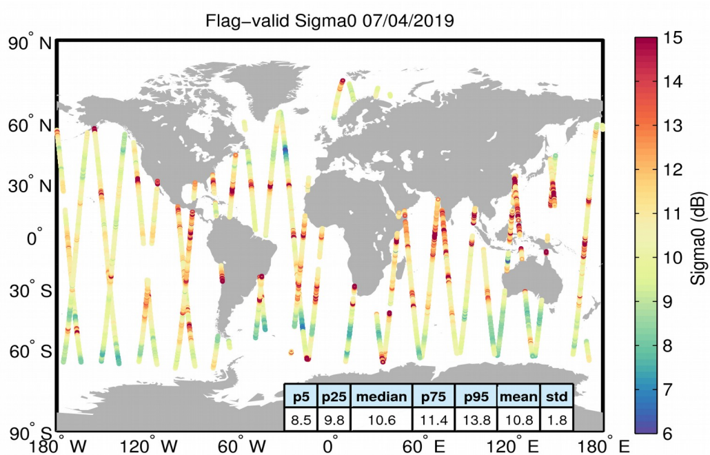
Figure 23. Geographical distribution of flag-valid sigma0 data over oceans and lakes for 07/04/2019. The statistical values shown in the table refer to the sigma0 in dB and are calculated over all measurements shown in the figure.
