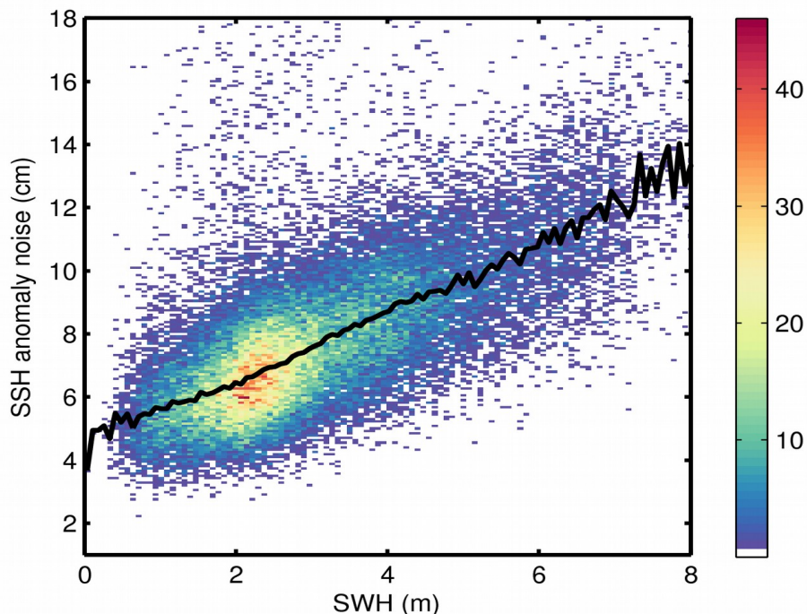
Figure 9. 2D histogram showing flag-valid SSH anomaly noise as a function of SWH for 07/04/2019. The black line denotes the median SSH anomaly noise as a function of SWH.
