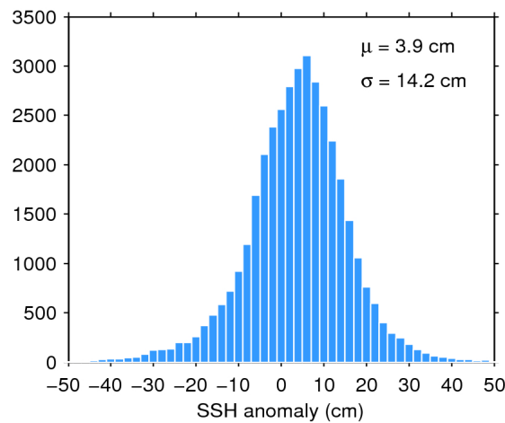
Figure 7. Histogram of flag-valid SSH anomaly over oceans and lakes for 07/04/2019. The mean ( \mu ) and standard deviation ( \sigma ) are also shown. Note that values outside [-50\ 50] cm are excluded from the histogram for the sake of readability but not from the computation of \mu and \sigma .
