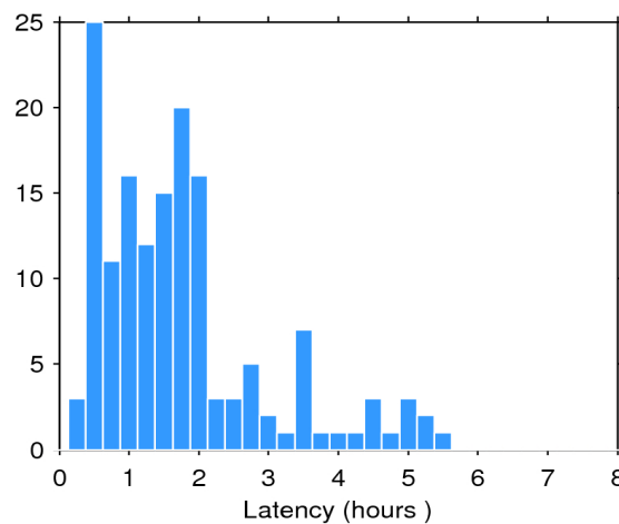
Figure 2. Histogram of the data latency for 07/04/2019. The y-axis denotes the number of files that are made available with a delay of x-hours with respect to the mean time of the records stored in the file.
