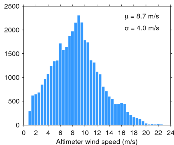
Figure 35. Histogram of science-valid wind over oceans and lakes for 07/04/2019. The mean ( \mu ) and standard deviation ( \sigma ) are also shown. Note that values larger than 24 m/s are excluded from the histogram for the sake of readability but not from the computation of \mu and \sigma .
