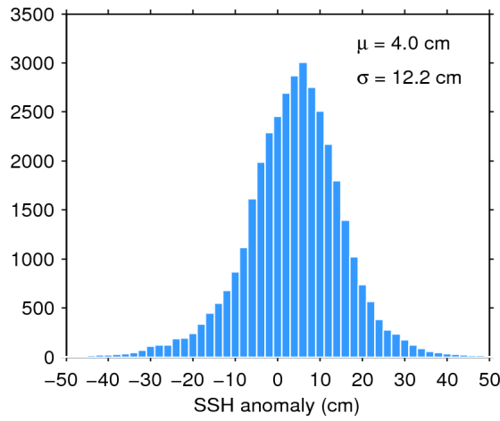
Figure 11. Histogram of science-valid SSH anomaly over oceans and lakes for 07/04/2019. The mean ( \mu ) and standard deviation ( \sigma ) are also shown. Note that values outside [-50 50] cm are excluded from the histogram for the sake of readability but not from the computation of \mu and \sigma .
