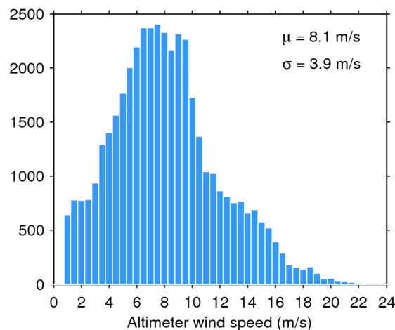
Figure 35. Histogram of science-valid wind over oceans and lakes for 06/04/2019. The mean ( \mu ) and standard deviation ( \sigma ) are also shown. Note that values larger than 24 m/s are excluded from the histogram for the sake of readability but not from the computation of \mu and \sigma .
