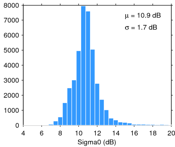
Figure 28. Histogram of science-valid sigma0 over oceans and lakes for 06/04/2019. The mean ( \mu ) and standard deviation ( \sigma ) are also shown. Note that values outside [4 20] dB are excluded from the histogram for the sake of readability but not from the computation of \mu and \sigma .
