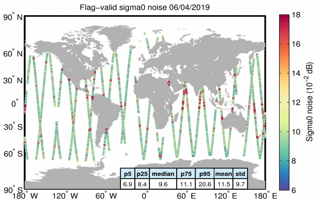
Figure 26. Geographical distribution of flag-valid 20-Hz sigma0 measurement noise over oceans and lakes for 06/04/2019. The statistical values shown in the table refer to the sigma0 noise and are calculated over all measurements shown in the figure.
