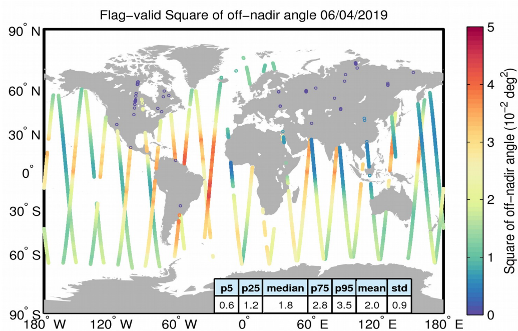
Figure 37. Geographical distribution of flag-valid mispointing data over oceans and lakes for 06/04/2019. The statistical values shown in the table refer to the mispointing in 10^{-2} deg 2 and are calculated over all measurements shown in the figure.
