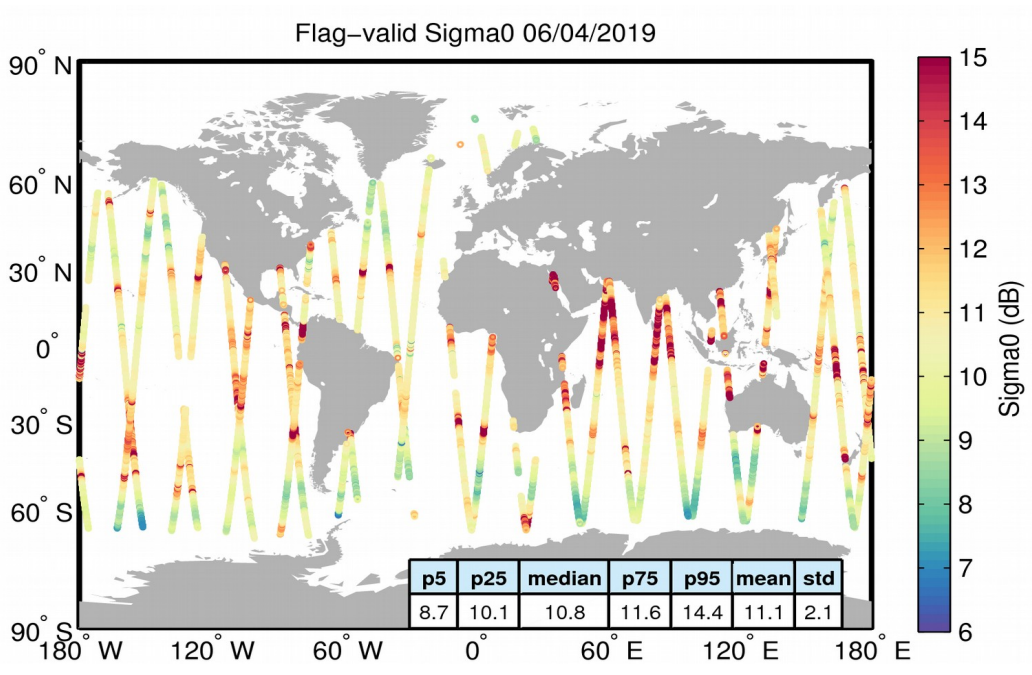
Figure 23. Geographical distribution of flag-valid sigma0 data over oceans and lakes for 06/04/2019. The statistical values shown in the table refer to the sigma0 in dB and are calculated over all measurements shown in the figure.
