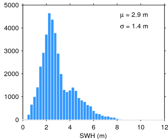
Figure 20. Histogram of science-valid SWH over oceans and lakes for 06/04/2019. The mean ( \mu ) and standard deviation ( \sigma ) are also shown. Note that values larger than 12 m are excluded from the histogram for the sake of readability but not from the computation of \mu and \sigma .
