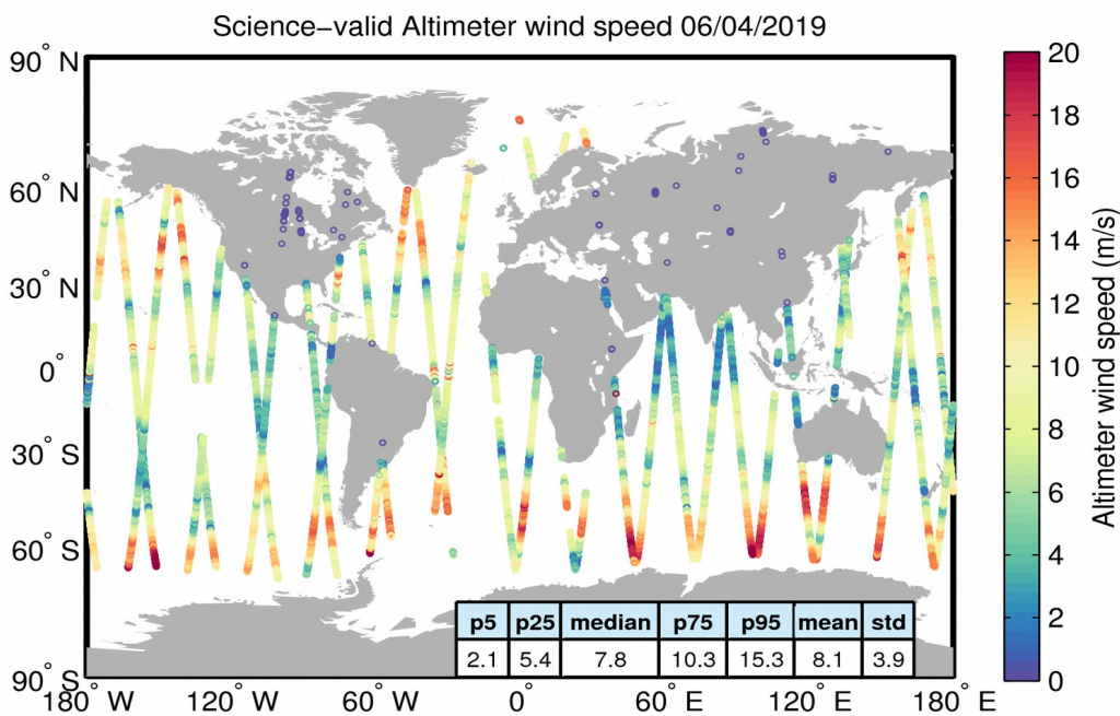
Figure 34. Geographical distribution of science-valid wind data over oceans and lakes for 06/04/2019. The statistical values shown in the table refer to the wind in m/s and are calculated over all measurements shown in the figure. Gray circles denote records that have been rejected based on the editing criteria described in Table 5.
