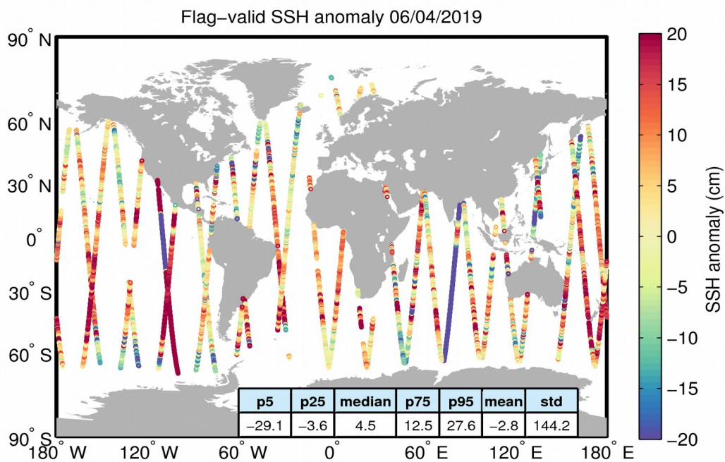
Figure 5. Geographical distribution of flag-valid 1-Hz SSH anomaly data over oceans and lakes for 06/04/2019. The statistical values shown in the table refer to the SSH anomaly in cm and are calculated over all measurements shown in the figure.
