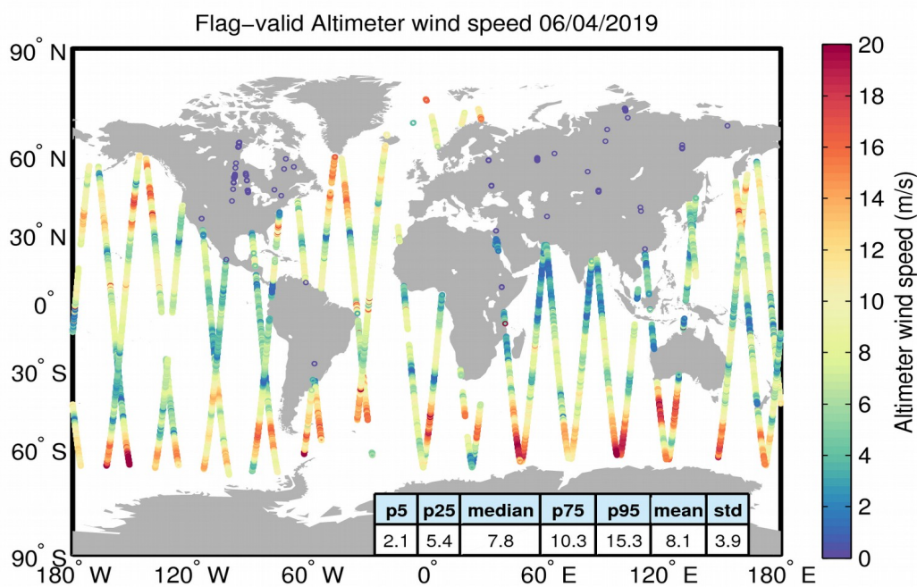
Figure 31. Geographical distribution of flag-valid wind data over oceans and lakes for 06/04/2019. The statistical values shown in the table refer to the wind in m/s and are calculated over all measurements shown in the figure.
