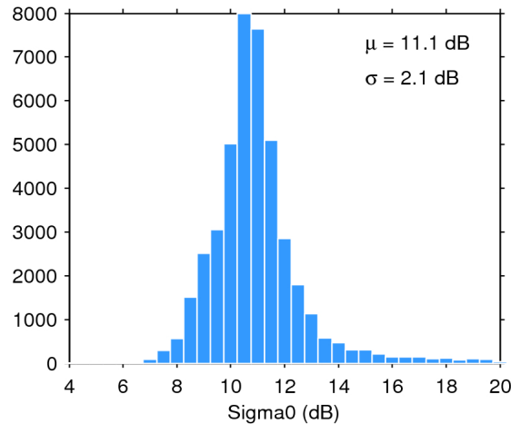
Figure 25. Histogram of flag-valid sigma0 over oceans and lakes for 06/04/2019. The mean ( \mu ) and standard deviation ( \sigma ) are also shown. Note that values outside [4 20] dB are excluded from the histogram for the sake of readability but not from the computation of \mu and \sigma .
