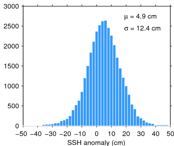
Figure 11. Histogram of science-valid SSH anomaly over oceans and lakes for 06/04/2019. The mean ( \mu ) and standard deviation ( \sigma ) are also shown. Note that values outside [-50 50] cm are excluded from the histogram for the sake of readability but not from the computation of \mu and \sigma .
