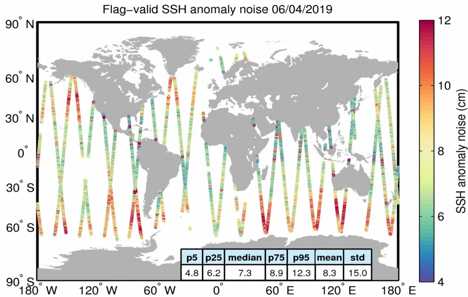
Figure 8. Geographical distribution of flag-valid 20-Hz SSH anomaly measurement noise over oceans and lakes for 06/04/2019. The statistical values shown in the table refer to the SSH anomaly noise and are calculated over all measurements shown in the figure.
