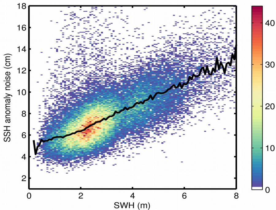
Figure 9. 2D histogram showing flag-valid SSH anomaly noise as a function of SWH for 06/04/2019. The black line denotes the median SSH anomaly noise as a function of SWH.
