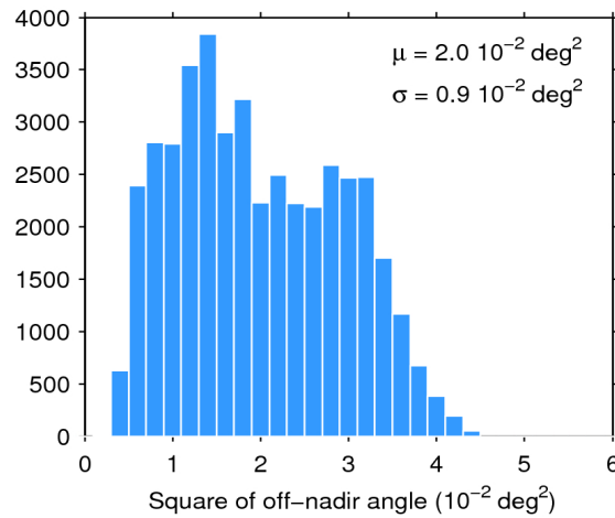
Figure 39. Histogram of flag-valid mispointing over oceans and lakes for 06/04/2019. The mean ( \mu ) and standard deviation ( \sigma ) are also shown. Note that values larger than 6 \cdot 10^{-2} \text{ deg}^2 are excluded from the histogram for the sake of readability but not from the computation of \mu and \sigma .
