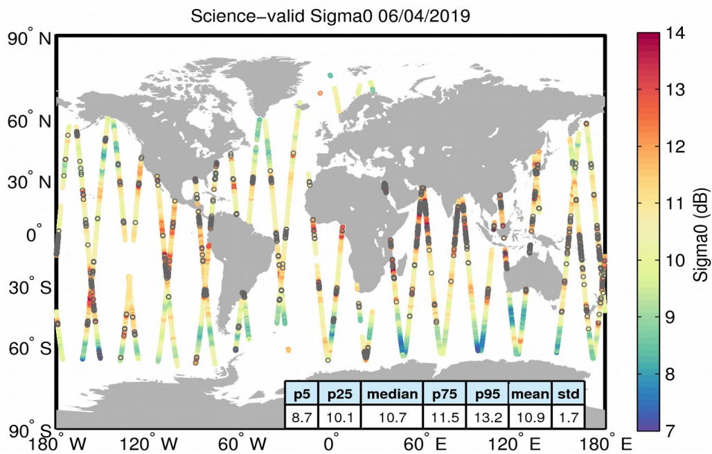
Figure 27. Geographical distribution of science-valid sigma0 data over oceans and lakes for 06/04/2019. The statistical values shown in the table refer to the sigma0 in dB and are calculated over all measurements shown in the figure. Gray circles denote records that have been rejected based on the editing criteria described in Table 4.
