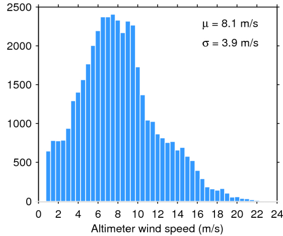
Figure 33. Histogram of flag-valid wind over oceans and lakes for 06/04/2019. The mean ( \mu ) and standard deviation ( \sigma ) are also shown. Note that values larger than 24 m/s are excluded from the histogram for the sake of readability but not from the computation of \mu and \sigma .
