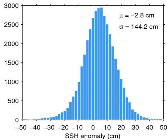
Figure 7. Histogram of flag-valid SSH anomaly over oceans and lakes for 06/04/2019. The mean ( \mu ) and standard deviation ( \sigma ) are also shown. Note that values outside [-50 50] cm are excluded from the histogram for the sake of readability but not from the computation of \mu and \sigma .
