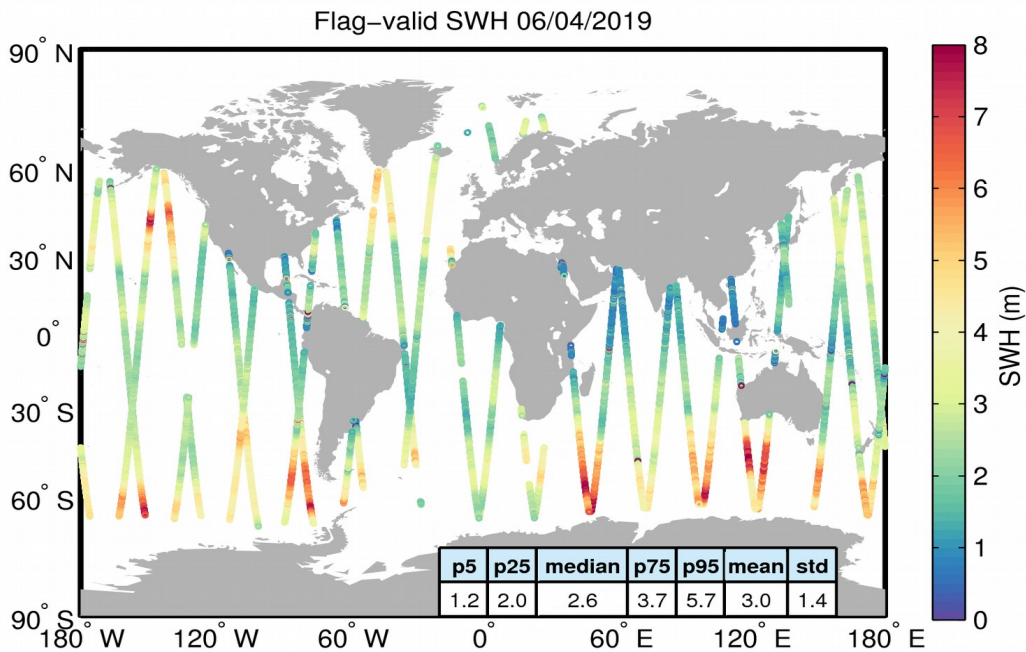
Figure 15. Geographical distribution of flag-valid SWH data over oceans and lakes for 06/04/2019. The statistical values shown in the table refer to the SWH in m and are calculated over all measurements shown in the figure.
