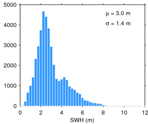
Figure 17. Histogram of flag-valid SWH over oceans and lakes for 06/04/2019. The mean ( \mu ) and standard deviation ( \sigma ) are also shown. Note that values larger than 12 m are excluded from the histogram for the sake of readability but not from the computation of \mu and \sigma .
