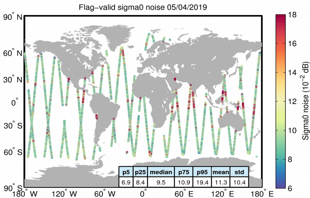
Figure 26. Geographical distribution of flag-valid 20-Hz sigma0 measurement noise over oceans and lakes for 05/04/2019. The statistical values shown in the table refer to the sigma0 noise and are calculated over all measurements shown in the figure.
