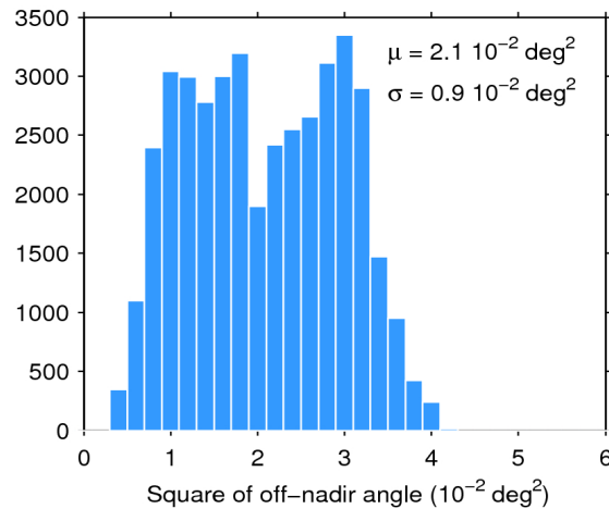
Figure 39. Histogram of flag-valid mispointing over oceans and lakes for 05/04/2019. The mean ( \mu ) and standard deviation ( \sigma ) are also shown. Note that values larger than 6 \cdot 10^{-2} \text{ deg}^2 are excluded from the histogram for the sake of readability but not from the computation of \mu and \sigma .
