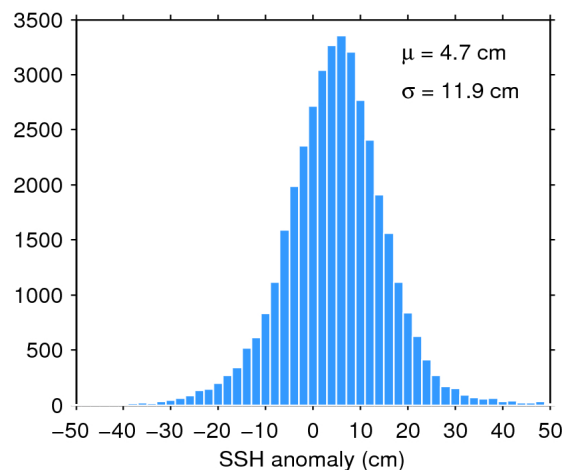
Figure 11. Histogram of science-valid SSH anomaly over oceans and lakes for 05/04/2019. The mean ( \mu ) and standard deviation ( \sigma ) are also shown. Note that values outside [-50 50] cm are excluded from the histogram for the sake of readability but not from the computation of \mu and \sigma .
