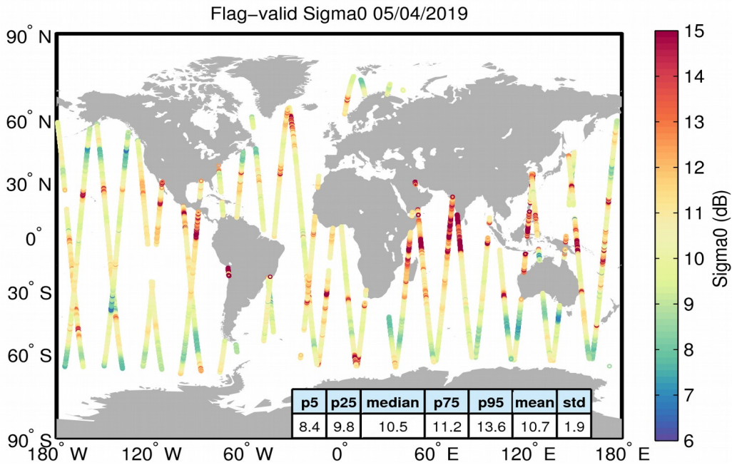
Figure 23. Geographical distribution of flag-valid sigma0 data over oceans and lakes for 05/04/2019. The statistical values shown in the table refer to the sigma0 in dB and are calculated over all measurements shown in the figure.
