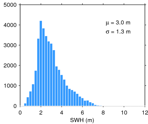
Figure 17. Histogram of flag-valid SWH over oceans and lakes for 05/04/2019. The mean ( \mu ) and standard deviation ( \sigma ) are also shown. Note that values larger than 12 m are excluded from the histogram for the sake of readability but not from the computation of \mu and \sigma .
