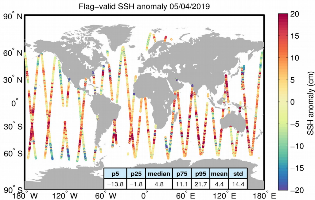
Figure 5. Geographical distribution of flag-valid 1-Hz SSH anomaly data over oceans and lakes for 05/04/2019. The statistical values shown in the table refer to the SSH anomaly in cm and are calculated over all measurements shown in the figure.
