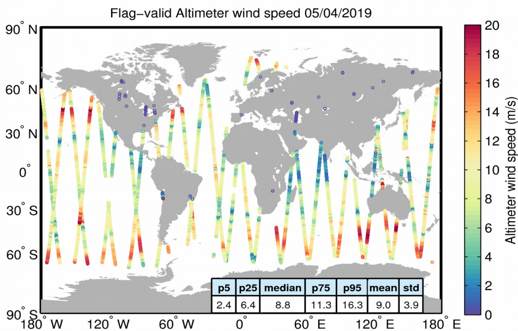
Figure 31. Geographical distribution of flag-valid wind data over oceans and lakes for 05/04/2019. The statistical values shown in the table refer to the wind in m/s and are calculated over all measurements shown in the figure.
