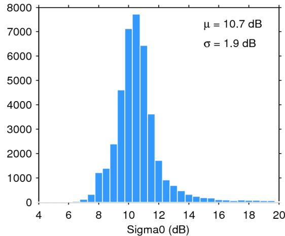
Figure 25. Histogram of flag-valid sigma0 over oceans and lakes for 05/04/2019. The mean ( \mu ) and standard deviation ( \sigma ) are also shown. Note that values outside [4 20] dB are excluded from the histogram for the sake of readability but not from the computation of \mu and \sigma .
