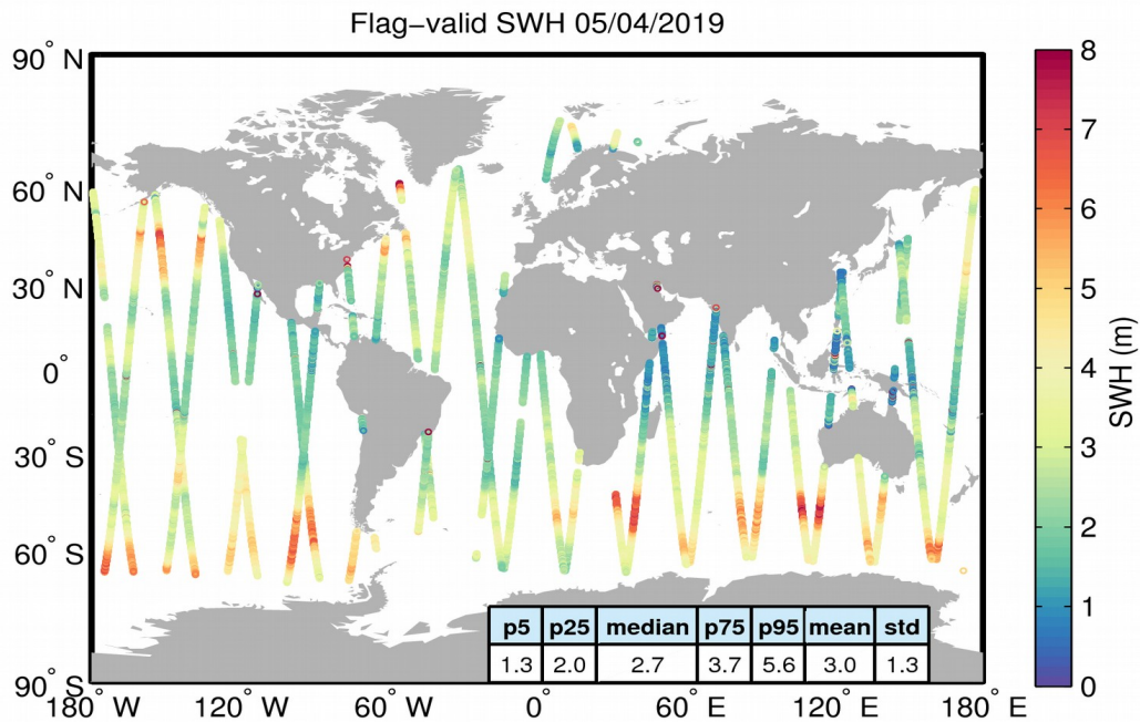
Figure 15. Geographical distribution of flag-valid SWH data over oceans and lakes for 05/04/2019. The statistical values shown in the table refer to the SWH in m and are calculated over all measurements shown in the figure.
