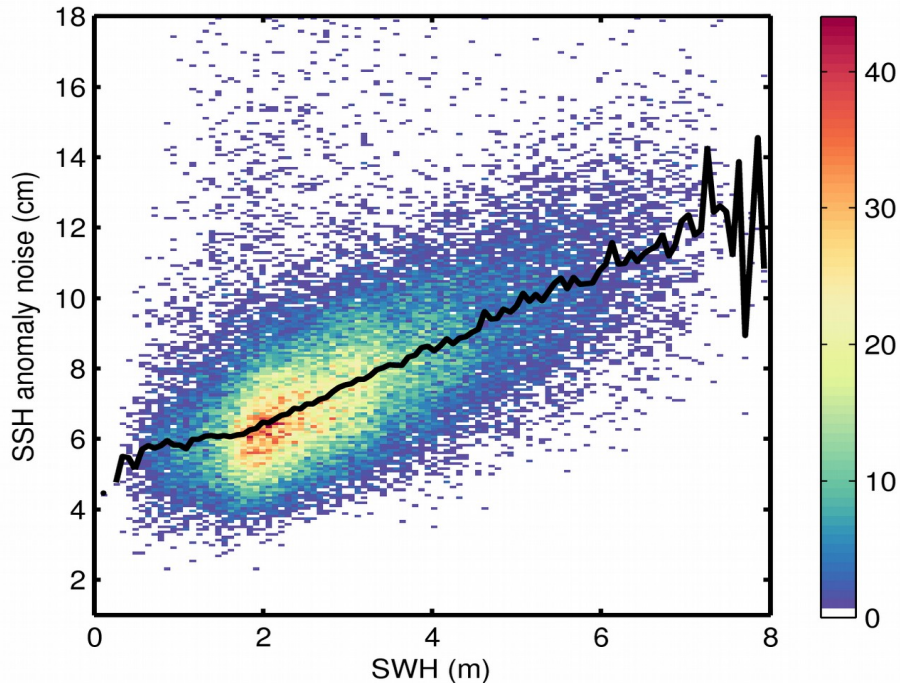
Figure 9. 2D histogram showing flag-valid SSH anomaly noise as a function of SWH for 05/04/2019. The black line denotes the median SSH anomaly noise as a function of SWH.
