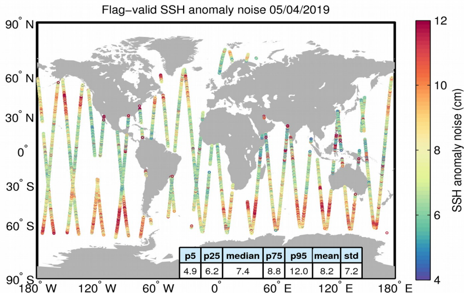
Figure 8. Geographical distribution of flag-valid 20-Hz SSH anomaly measurement noise over oceans and lakes for 05/04/2019. The statistical values shown in the table refer to the SSH anomaly noise and are calculated over all measurements shown in the figure.
