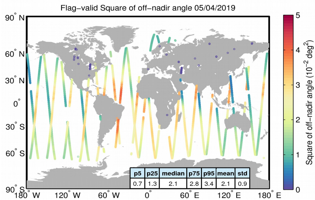
Figure 37. Geographical distribution of flag-valid mispointing data over oceans and lakes for 05/04/2019. The statistical values shown in the table refer to the mispointing in 10^{-2} \text{ deg}^2 and are calculated over all measurements shown in the figure.
