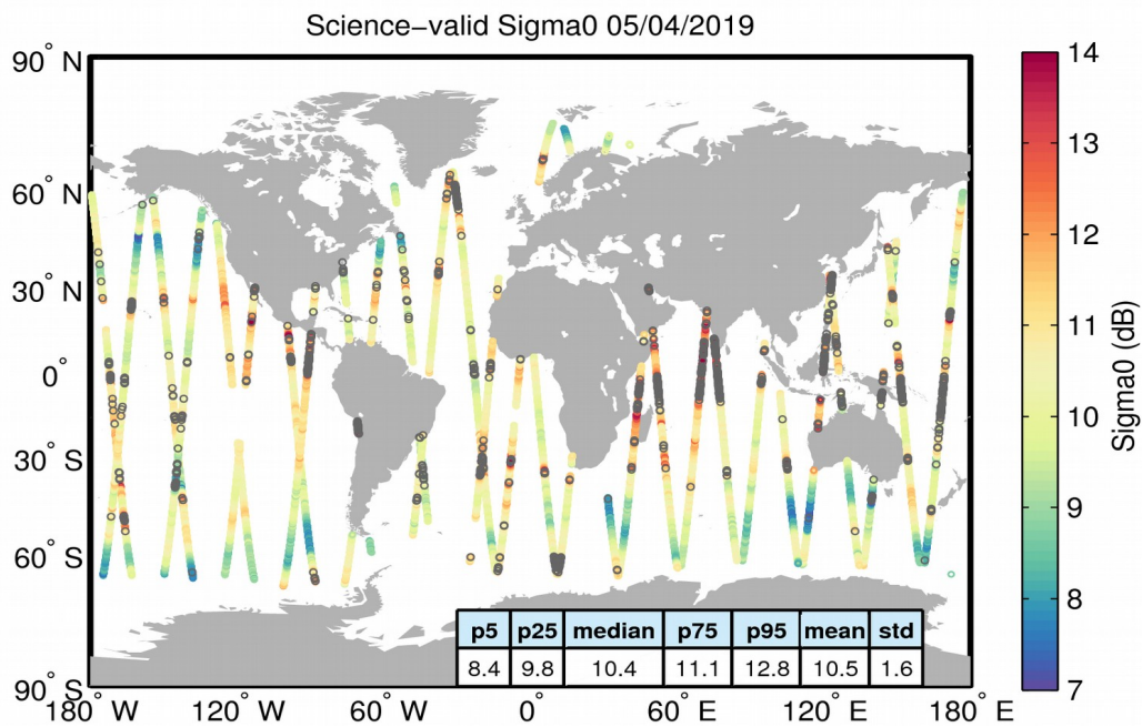
Figure 27. Geographical distribution of science-valid sigma0 data over oceans and lakes for 05/04/2019. The statistical values shown in the table refer to the sigma0 in dB and are calculated over all measurements shown in the figure. Gray circles denote records that have been rejected based on the editing criteria described in Table 4.
