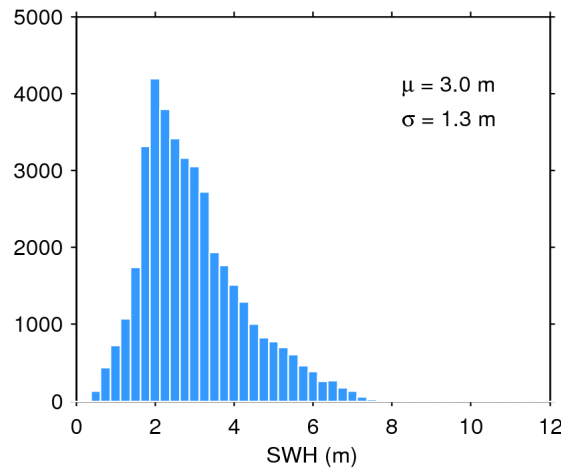
Figure 20. Histogram of science-valid SWH over oceans and lakes for 05/04/2019. The mean ( \mu ) and standard deviation ( \sigma ) are also shown. Note that values larger than 12 m are excluded from the histogram for the sake of readability but not from the computation of \mu and \sigma .
