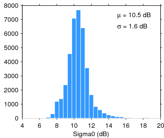
Figure 28. Histogram of science-valid sigma0 over oceans and lakes for 05/04/2019. The mean ( \mu ) and standard deviation ( \sigma ) are also shown. Note that values outside [4 20] dB are excluded from the histogram for the sake of readability but not from the computation of \mu and \sigma .
