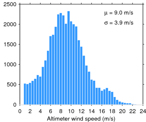
Figure 33. Histogram of flag-valid wind over oceans and lakes for 05/04/2019. The mean ( \mu ) and standard deviation ( \sigma ) are also shown. Note that values larger than 24 m/s are excluded from the histogram for the sake of readability but not from the computation of \mu and \sigma .
