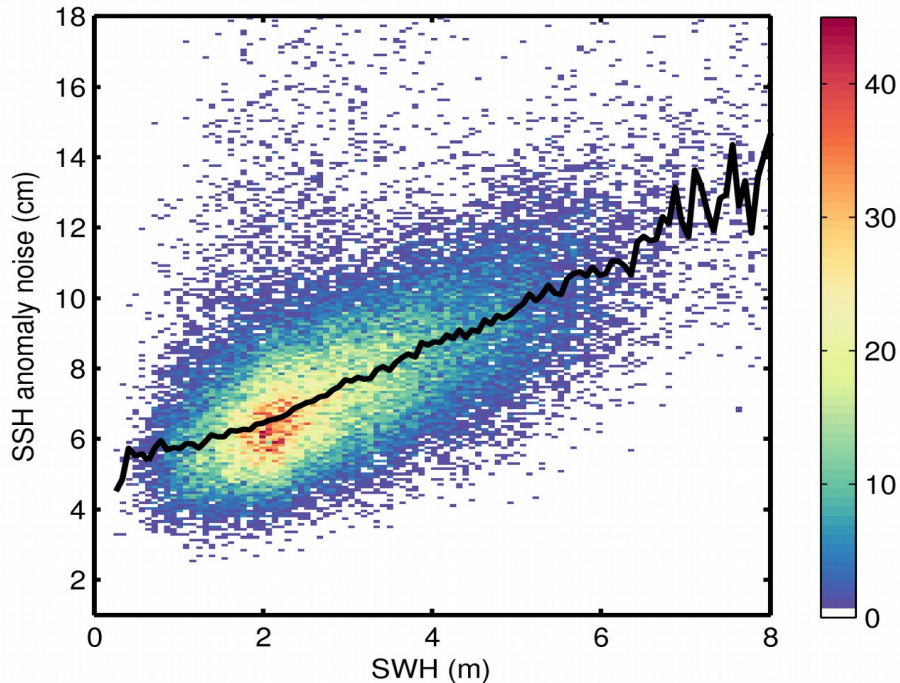
Figure 9. 2D histogram showing flag-valid SSH anomaly noise as a function of SWH for 04/04/2019. The black line denotes the median SSH anomaly noise as a function of SWH.
