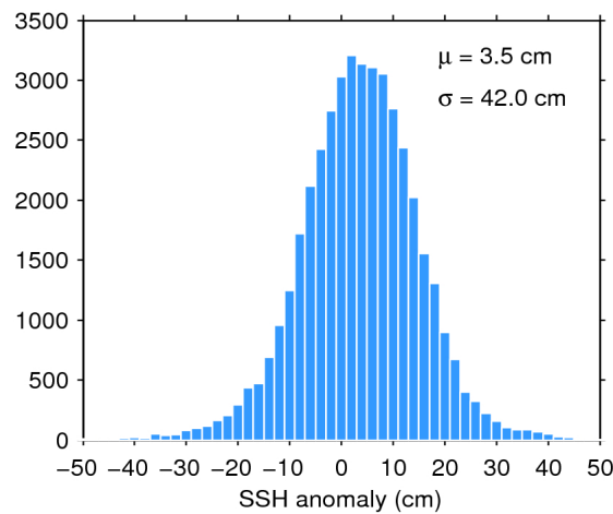
Figure 7. Histogram of flag-valid SSH anomaly over oceans and lakes for 04/04/2019. The mean ( \mu ) and standard deviation ( \sigma ) are also shown. Note that values outside [-50\ 50] cm are excluded from the histogram for the sake of readability but not from the computation of \mu and \sigma .
