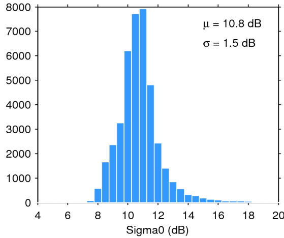
Figure 28. Histogram of science-valid sigma0 over oceans and lakes for 04/04/2019. The mean ( \mu ) and standard deviation ( \sigma ) are also shown. Note that values outside [4 20] dB are excluded from the histogram for the sake of readability but not from the computation of \mu and \sigma .
