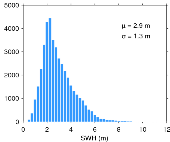
Figure 20. Histogram of science-valid SWH over oceans and lakes for 04/04/2019. The mean ( \mu ) and standard deviation ( \sigma ) are also shown. Note that values larger than 12 m are excluded from the histogram for the sake of readability but not from the computation of \mu and \sigma .
