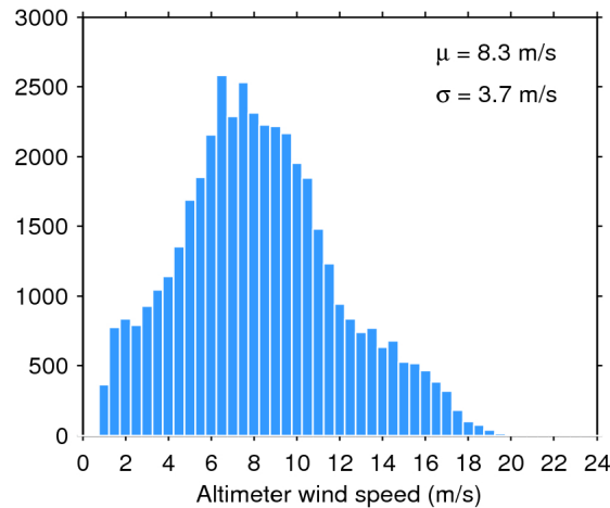
Figure 33. Histogram of flag-valid wind over oceans and lakes for 04/04/2019. The mean ( \mu ) and standard deviation ( \sigma ) are also shown. Note that values larger than 24 m/s are excluded from the histogram for the sake of readability but not from the computation of \mu and \sigma .
