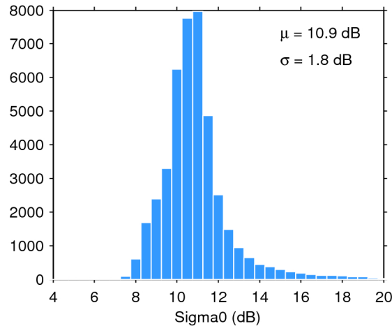
Figure 25. Histogram of flag-valid sigma0 over oceans and lakes for 04/04/2019. The mean ( \mu ) and standard deviation ( \sigma ) are also shown. Note that values outside [4 20] dB are excluded from the histogram for the sake of readability but not from the computation of \mu and \sigma .
