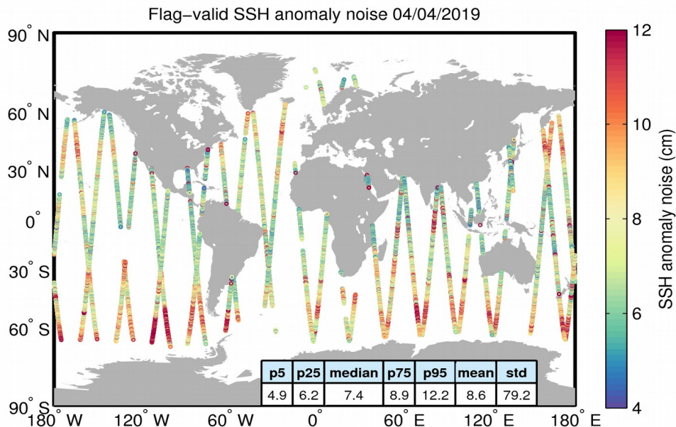
Figure 8. Geographical distribution of flag-valid 20-Hz SSH anomaly measurement noise over oceans and lakes for 04/04/2019. The statistical values shown in the table refer to the SSH anomaly noise and are calculated over all measurements shown in the figure.
