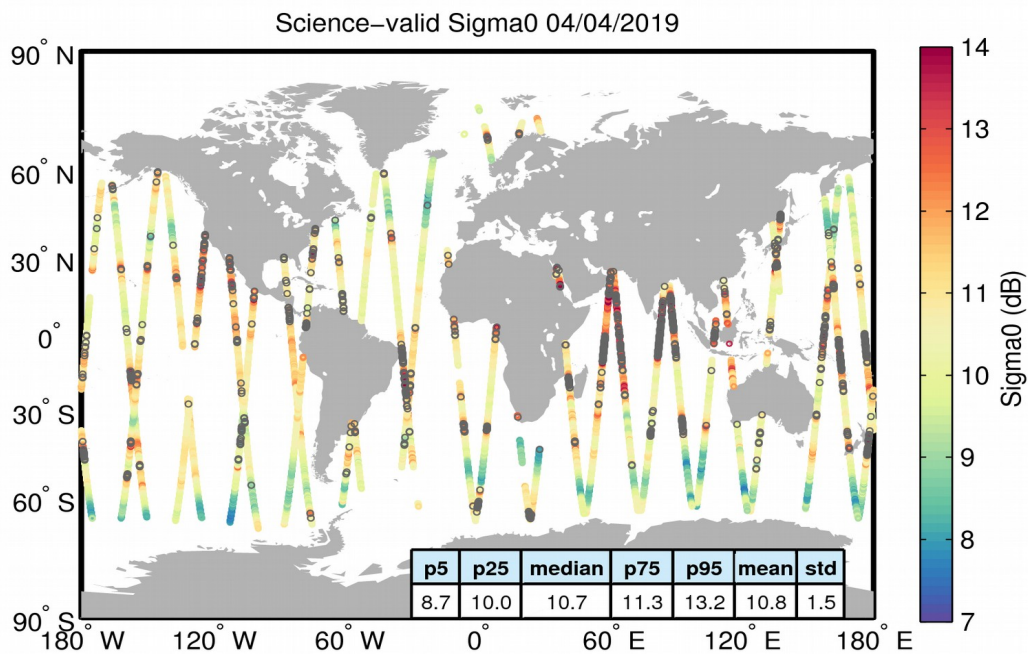
Figure 27. Geographical distribution of science-valid sigma0 data over oceans and lakes for 04/04/2019. The statistical values shown in the table refer to the sigma0 in dB and are calculated over all measurements shown in the figure. Gray circles denote records that have been rejected based on the editing criteria described in Table 4.
