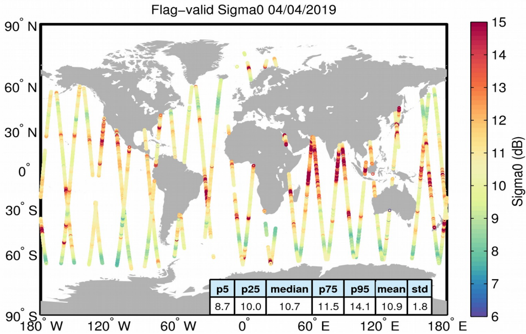
Figure 23. Geographical distribution of flag-valid sigma0 data over oceans and lakes for 04/04/2019. The statistical values shown in the table refer to the sigma0 in dB and are calculated over all measurements shown in the figure.
