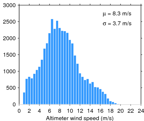
Figure 35. Histogram of science-valid wind over oceans and lakes for 04/04/2019. The mean ( \mu ) and standard deviation ( \sigma ) are also shown. Note that values larger than 24 m/s are excluded from the histogram for the sake of readability but not from the computation of \mu and \sigma .
