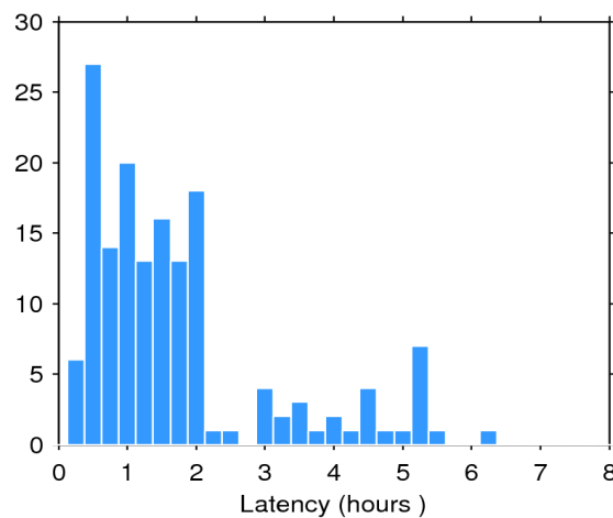
Figure 2. Histogram of the data latency for 04/04/2019. The y-axis denotes the number of files that are made available with a delay of x-hours with respect to the mean time of the records stored in the file.
