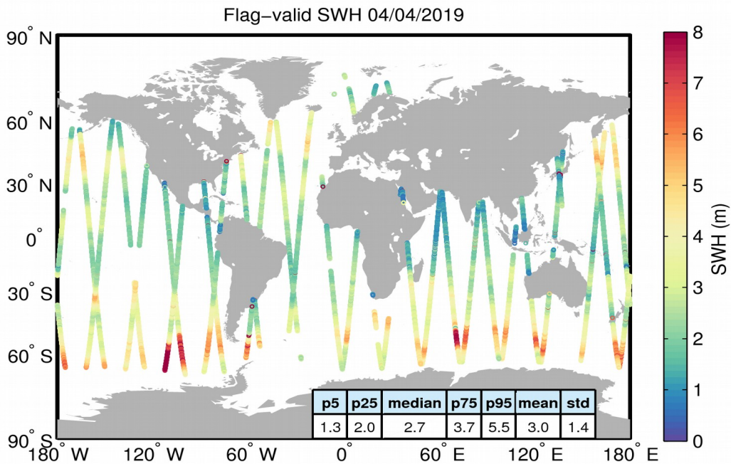
Figure 15. Geographical distribution of flag-valid SWH data over oceans and lakes for 04/04/2019. The statistical values shown in the table refer to the SWH in m and are calculated over all measurements shown in the figure.
