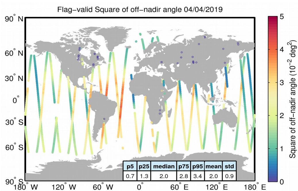
Figure 37. Geographical distribution of flag-valid mispointing data over oceans and lakes for 04/04/2019. The statistical values shown in the table refer to the mispointing in 10^{-2} \text{ deg}^2 and are calculated over all measurements shown in the figure.
