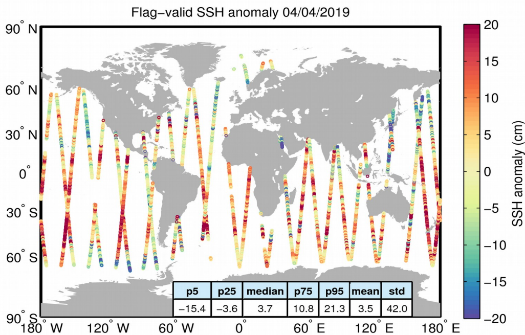
Figure 5. Geographical distribution of flag-valid 1-Hz SSH anomaly data over oceans and lakes for 04/04/2019. The statistical values shown in the table refer to the SSH anomaly in cm and are calculated over all measurements shown in the figure.
