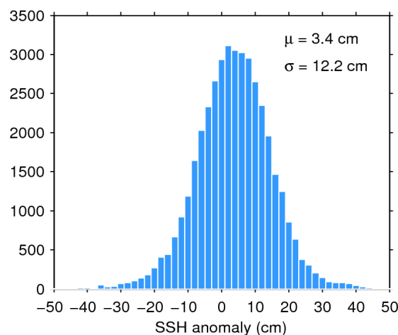
Figure 11. Histogram of science-valid SSH anomaly over oceans and lakes for 04/04/2019. The mean ( \mu ) and standard deviation ( \sigma ) are also shown. Note that values outside [-50 50] cm are excluded from the histogram for the sake of readability but not from the computation of \mu and \sigma .
