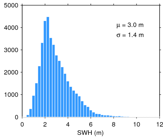
Figure 17. Histogram of flag-valid SWH over oceans and lakes for 04/04/2019. The mean ( \mu ) and standard deviation ( \sigma ) are also shown. Note that values larger than 12 m are excluded from the histogram for the sake of readability but not from the computation of \mu and \sigma .
