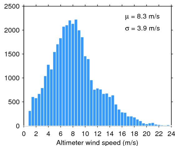
Figure 35. Histogram of science-valid wind over oceans and lakes for 03/04/2019. The mean ( \mu ) and standard deviation ( \sigma ) are also shown. Note that values larger than 24 m/s are excluded from the histogram for the sake of readability but not from the computation of \mu and \sigma .
