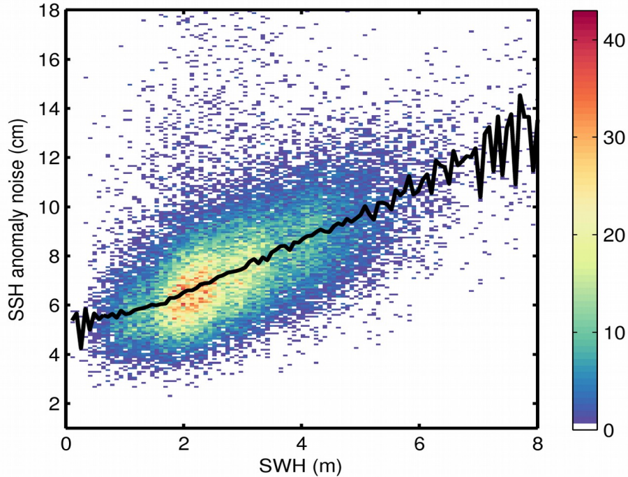
Figure 9. 2D histogram showing flag-valid SSH anomaly noise as a function of SWH for 03/04/2019. The black line denotes the median SSH anomaly noise as a function of SWH.
