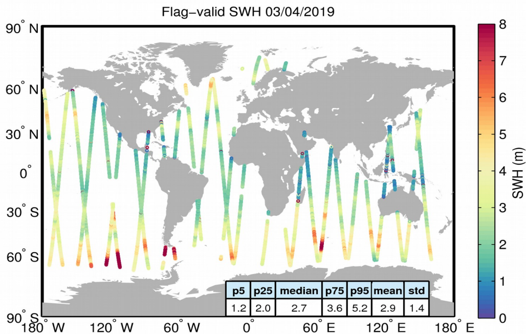
Figure 15. Geographical distribution of flag-valid SWH data over oceans and lakes for 03/04/2019. The statistical values shown in the table refer to the SWH in m and are calculated over all measurements shown in the figure.
