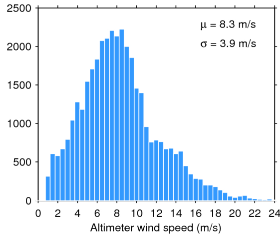
Figure 33. Histogram of flag-valid wind over oceans and lakes for 03/04/2019. The mean ( \mu ) and standard deviation ( \sigma ) are also shown. Note that values larger than 24 m/s are excluded from the histogram for the sake of readability but not from the computation of \mu and \sigma .
