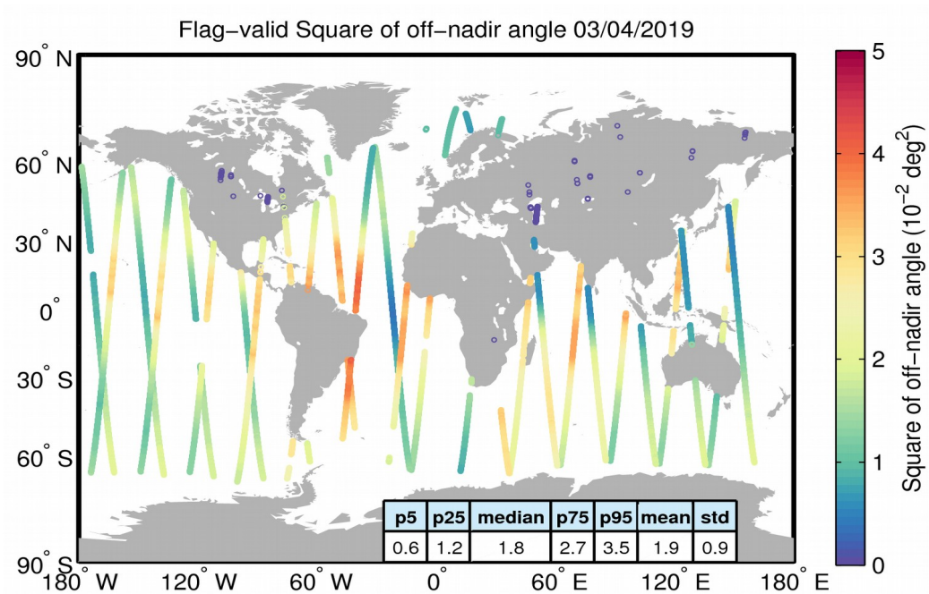
Figure 37. Geographical distribution of flag-valid mispointing data over oceans and lakes for 03/04/2019. The statistical values shown in the table refer to the mispointing in 10^{-2} \text{ deg}^2 and are calculated over all measurements shown in the figure.
