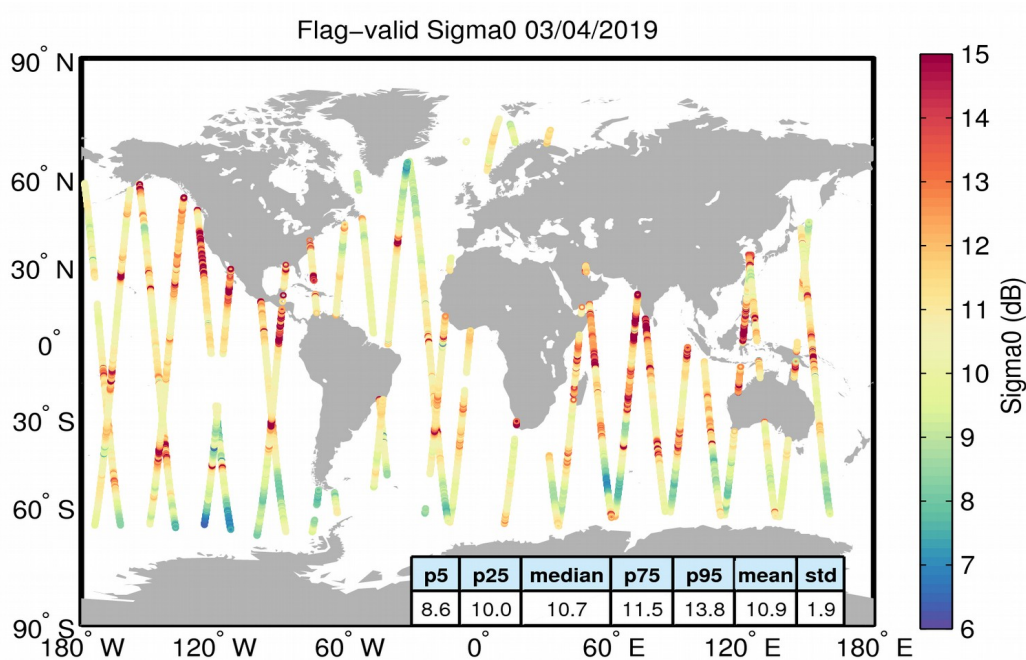
Figure 23. Geographical distribution of flag-valid sigma0 data over oceans and lakes for 03/04/2019. The statistical values shown in the table refer to the sigma0 in dB and are calculated over all measurements shown in the figure.
