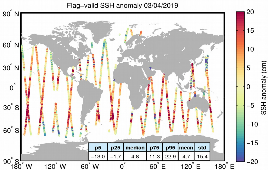
Figure 5. Geographical distribution of flag-valid 1-Hz SSH anomaly data over oceans and lakes for 03/04/2019. The statistical values shown in the table refer to the SSH anomaly in cm and are calculated over all measurements shown in the figure.
