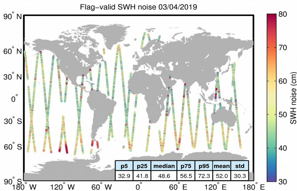
Figure 18. Geographical distribution of flag-valid 20-Hz SWH measurement noise over oceans and lakes for 03/04/2019. The statistical values shown in the figure refer to the SWH noise and are calculated over all measurements shown in the figure.
