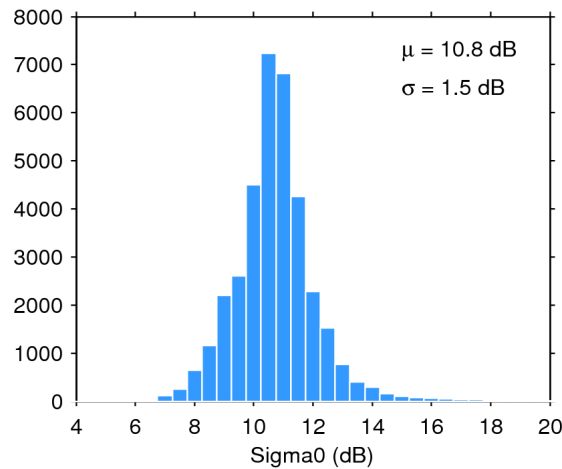
Figure 28. Histogram of science-valid sigma0 over oceans and lakes for 03/04/2019. The mean ( \mu ) and standard deviation ( \sigma ) are also shown. Note that values outside [4 20] dB are excluded from the histogram for the sake of readability but not from the computation of \mu and \sigma .
