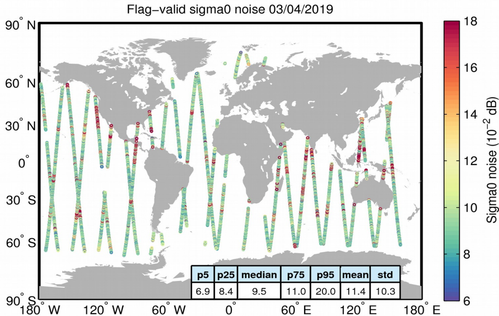
Figure 26. Geographical distribution of flag-valid 20-Hz sigma0 measurement noise over oceans and lakes for 03/04/2019. The statistical values shown in the table refer to the sigma0 noise and are calculated over all measurements shown in the figure.
