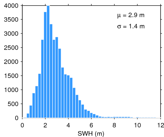
Figure 17. Histogram of flag-valid SWH over oceans and lakes for 03/04/2019. The mean ( \mu ) and standard deviation ( \sigma ) are also shown. Note that values larger than 12 m are excluded from the histogram for the sake of readability but not from the computation of \mu and \sigma .
