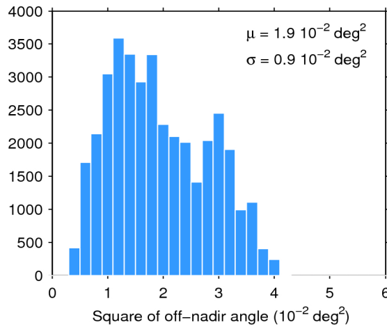
Figure 39. Histogram of flag-valid mispointing over oceans and lakes for 03/04/2019. The mean ( \mu ) and standard deviation ( \sigma ) are also shown. Note that values larger than 6 \cdot 10^{-2} \text{ deg}^2 are excluded from the histogram for the sake of readability but not from the computation of \mu and \sigma .
