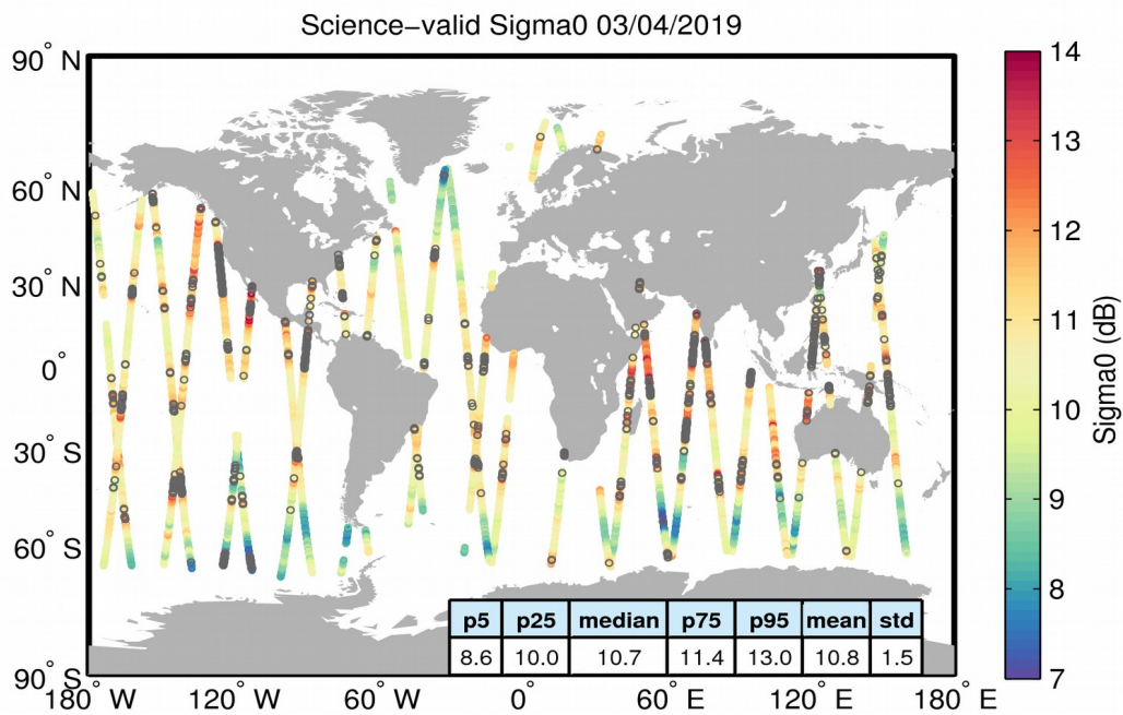
Figure 27. Geographical distribution of science-valid sigma0 data over oceans and lakes for 03/04/2019. The statistical values shown in the table refer to the sigma0 in dB and are calculated over all measurements shown in the figure. Gray circles denote records that have been rejected based on the editing criteria described in Table 4.
