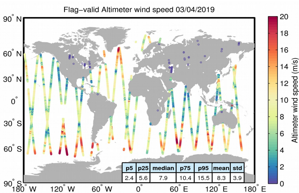
Figure 31. Geographical distribution of flag-valid wind data over oceans and lakes for 03/04/2019. The statistical values shown in the table refer to the wind in m/s and are calculated over all measurements shown in the figure.
