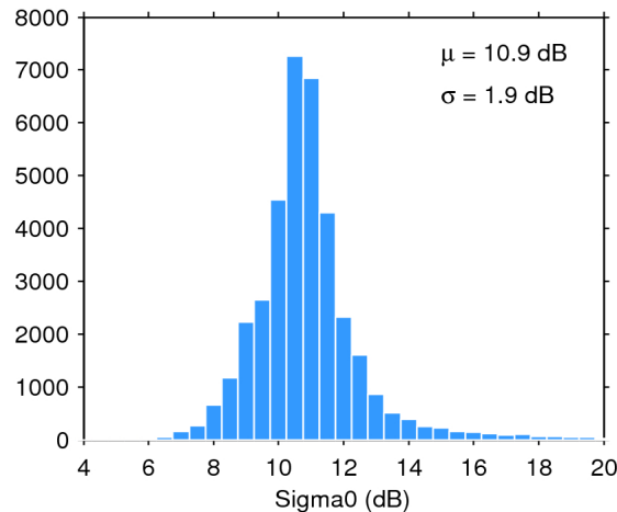
Figure 25. Histogram of flag-valid sigma0 over oceans and lakes for 03/04/2019. The mean ( \mu ) and standard deviation ( \sigma ) are also shown. Note that values outside [4 20] dB are excluded from the histogram for the sake of readability but not from the computation of \mu and \sigma .
