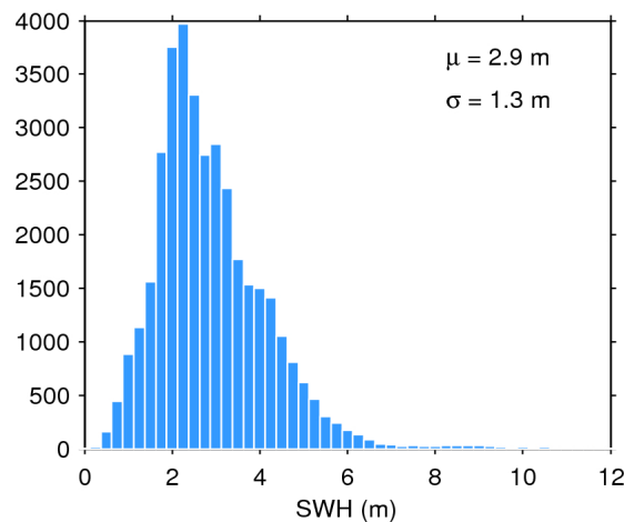
Figure 20. Histogram of science-valid SWH over oceans and lakes for 03/04/2019. The mean ( \mu ) and standard deviation ( \sigma ) are also shown. Note that values larger than 12 m are excluded from the histogram for the sake of readability but not from the computation of \mu and \sigma .
