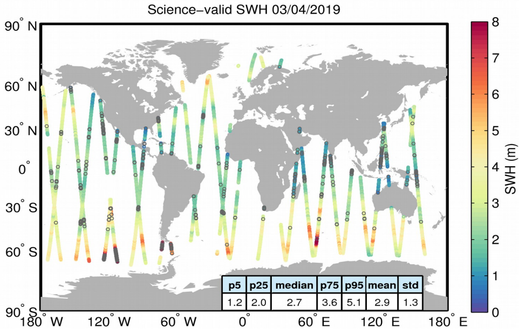
Figure 19. Geographical distribution of science-valid SWH data over oceans and lakes for 03/04/2019. The statistical values shown in the table refer to the SWH in m and are calculated over all measurements shown in the figure. Gray circles denote records that have been rejected based on the editing criteria described in Table 3.
