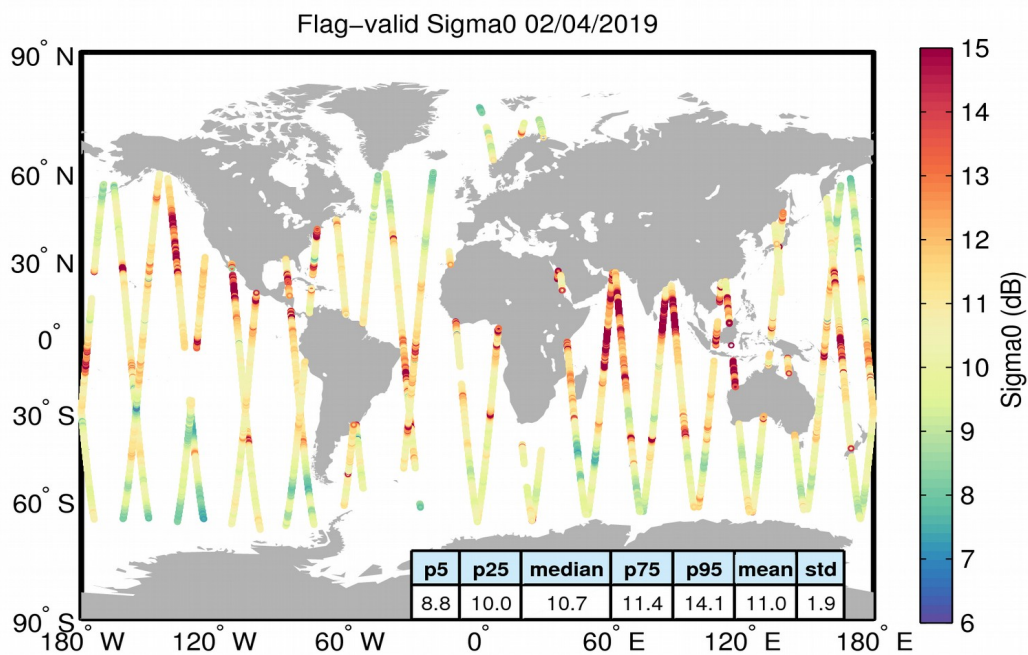
Figure 23. Geographical distribution of flag-valid sigma0 data over oceans and lakes for 02/04/2019. The statistical values shown in the table refer to the sigma0 in dB and are calculated over all measurements shown in the figure.
