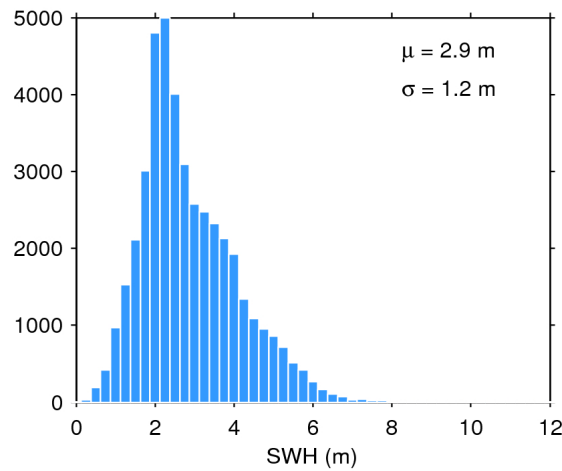
Figure 17. Histogram of flag-valid SWH over oceans and lakes for 02/04/2019. The mean ( \mu ) and standard deviation ( \sigma ) are also shown. Note that values larger than 12 m are excluded from the histogram for the sake of readability but not from the computation of \mu and \sigma .
