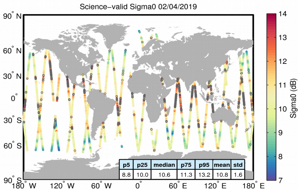
Figure 27. Geographical distribution of science-valid sigma0 data over oceans and lakes for 02/04/2019. The statistical values shown in the table refer to the sigma0 in dB and are calculated over all measurements shown in the figure. Gray circles denote records that have been rejected based on the editing criteria described in Table 4.
