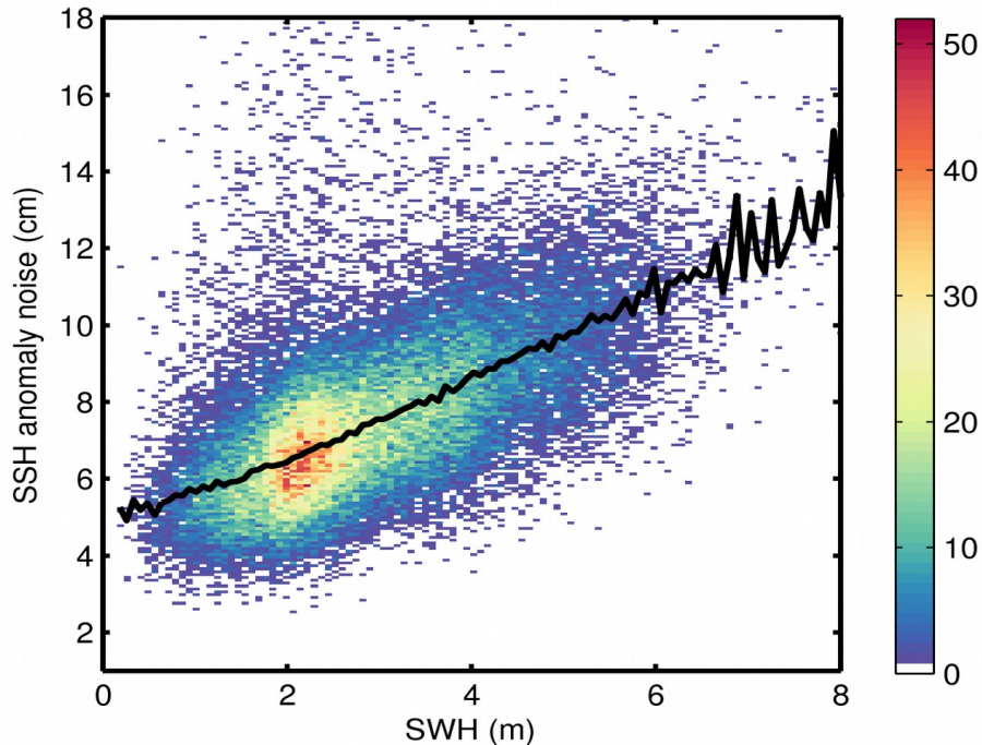
Figure 9. 2D histogram showing flag-valid SSH anomaly noise as a function of SWH for 02/04/2019. The black line denotes the median SSH anomaly noise as a function of SWH.
