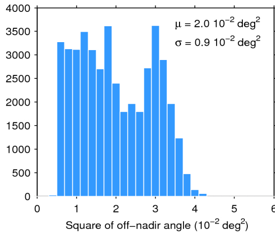
Figure 39. Histogram of flag-valid mispointing over oceans and lakes for 02/04/2019. The mean ( \mu ) and standard deviation ( \sigma ) are also shown. Note that values larger than 6 \cdot 10^{-2} \text{ deg}^2 are excluded from the histogram for the sake of readability but not from the computation of \mu and \sigma .
