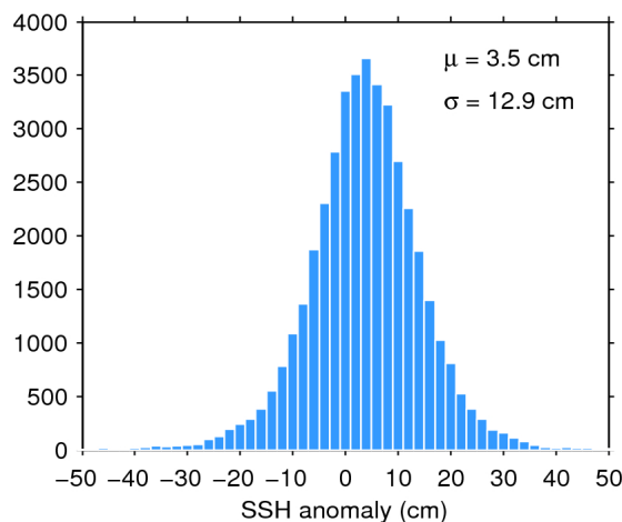
Figure 11. Histogram of science-valid SSH anomaly over oceans and lakes for 02/04/2019. The mean ( \mu ) and standard deviation ( \sigma ) are also shown. Note that values outside [-50 50] cm are excluded from the histogram for the sake of readability but not from the computation of \mu and \sigma .
