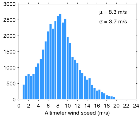
Figure 33. Histogram of flag-valid wind over oceans and lakes for 02/04/2019. The mean ( \mu ) and standard deviation ( \sigma ) are also shown. Note that values larger than 24 m/s are excluded from the histogram for the sake of readability but not from the computation of \mu and \sigma .
