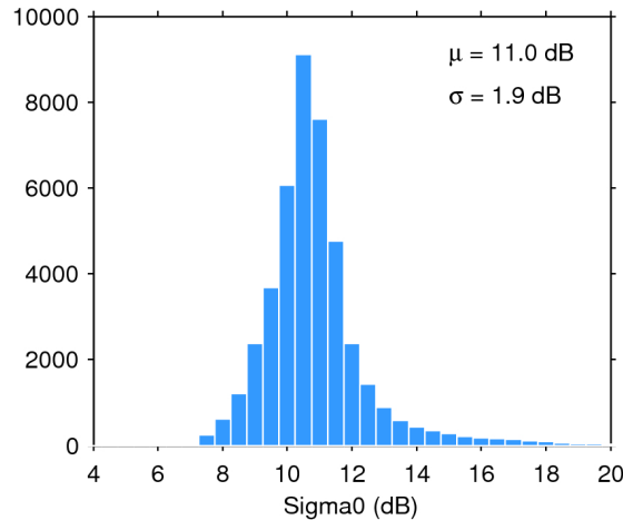
Figure 25. Histogram of flag-valid sigma0 over oceans and lakes for 02/04/2019. The mean ( \mu ) and standard deviation ( \sigma ) are also shown. Note that values outside [4 20] dB are excluded from the histogram for the sake of readability but not from the computation of \mu and \sigma .
