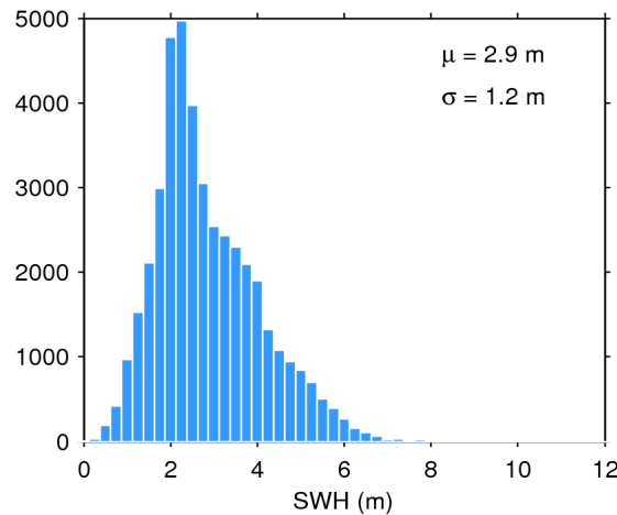
Figure 20. Histogram of science-valid SWH over oceans and lakes for 02/04/2019. The mean ( \mu ) and standard deviation ( \sigma ) are also shown. Note that values larger than 12 m are excluded from the histogram for the sake of readability but not from the computation of \mu and \sigma .
