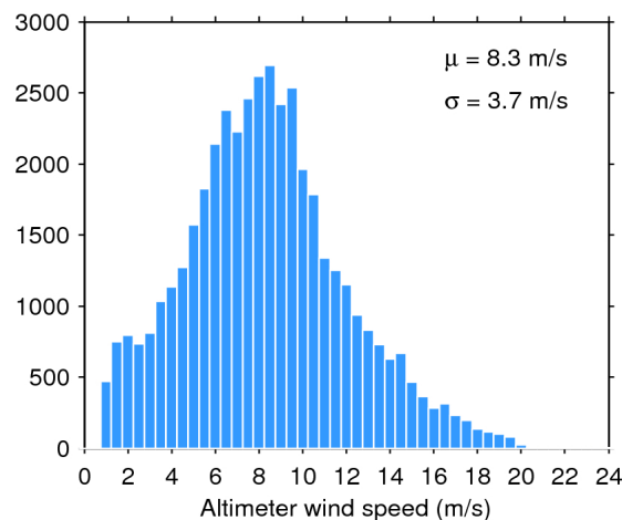
Figure 35. Histogram of science-valid wind over oceans and lakes for 02/04/2019. The mean ( \mu ) and standard deviation ( \sigma ) are also shown. Note that values larger than 24 m/s are excluded from the histogram for the sake of readability but not from the computation of \mu and \sigma .
