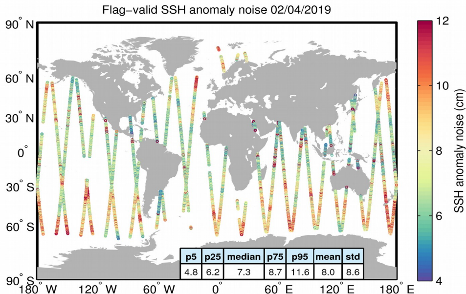
Figure 8. Geographical distribution of flag-valid 20-Hz SSH anomaly measurement noise over oceans and lakes for 02/04/2019. The statistical values shown in the table refer to the SSH anomaly noise and are calculated over all measurements shown in the figure.
