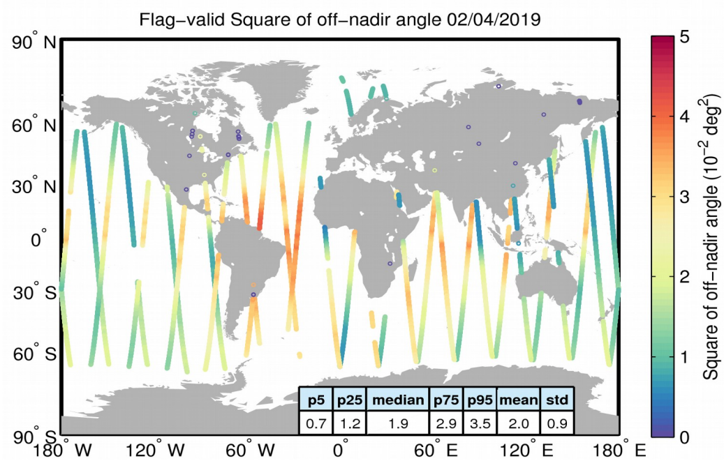
Figure 37. Geographical distribution of flag-valid mispointing data over oceans and lakes for 02/04/2019. The statistical values shown in the table refer to the mispointing in 10^{-2} deg 2 and are calculated over all measurements shown in the figure.
