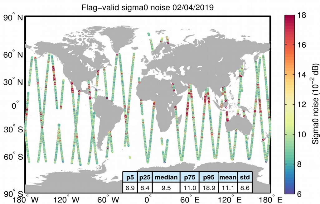
Figure 26. Geographical distribution of flag-valid 20-Hz sigma0 measurement noise over oceans and lakes for 02/04/2019. The statistical values shown in the table refer to the sigma0 noise and are calculated over all measurements shown in the figure.
