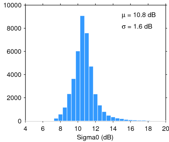
Figure 28. Histogram of science-valid sigma0 over oceans and lakes for 02/04/2019. The mean ( \mu ) and standard deviation ( \sigma ) are also shown. Note that values outside [4 20] dB are excluded from the histogram for the sake of readability but not from the computation of \mu and \sigma .
