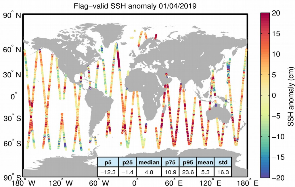
Figure 5. Geographical distribution of flag-valid 1-Hz SSH anomaly data over oceans and lakes for 01/04/2019. The statistical values shown in the table refer to the SSH anomaly in cm and are calculated over all measurements shown in the figure.
