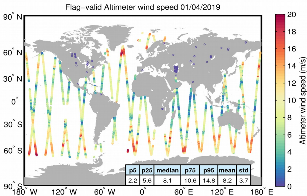
Figure 31. Geographical distribution of flag-valid wind data over oceans and lakes for 01/04/2019. The statistical values shown in the table refer to the wind in m/s and are calculated over all measurements shown in the figure.
