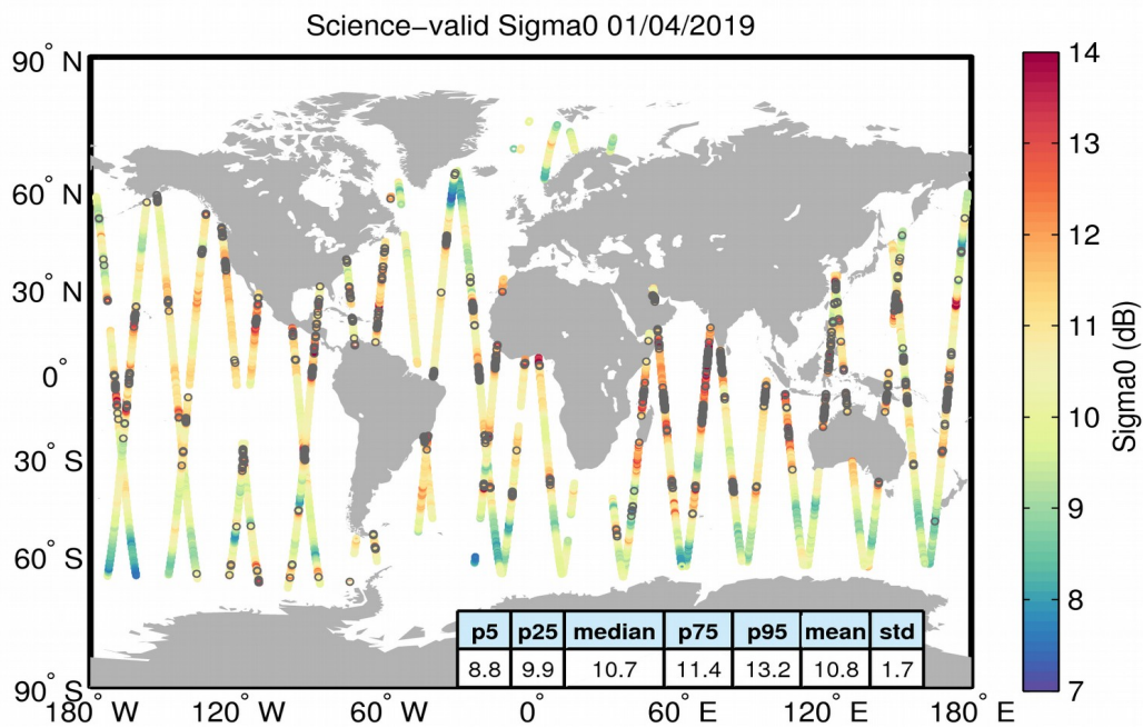
Figure 27. Geographical distribution of science-valid sigma0 data over oceans and lakes for 01/04/2019. The statistical values shown in the table refer to the sigma0 in dB and are calculated over all measurements shown in the figure. Gray circles denote records that have been rejected based on the editing criteria described in Table 4.
