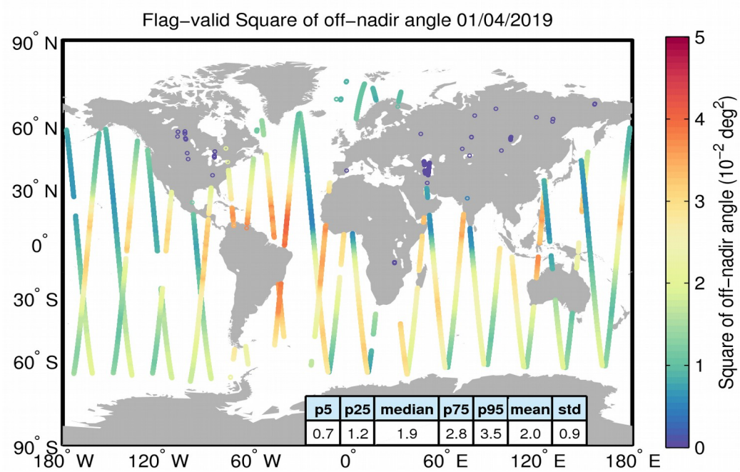
Figure 37. Geographical distribution of flag-valid mispointing data over oceans and lakes for 01/04/2019. The statistical values shown in the table refer to the mispointing in 10^{-2} \text{ deg}^2 and are calculated over all measurements shown in the figure.
