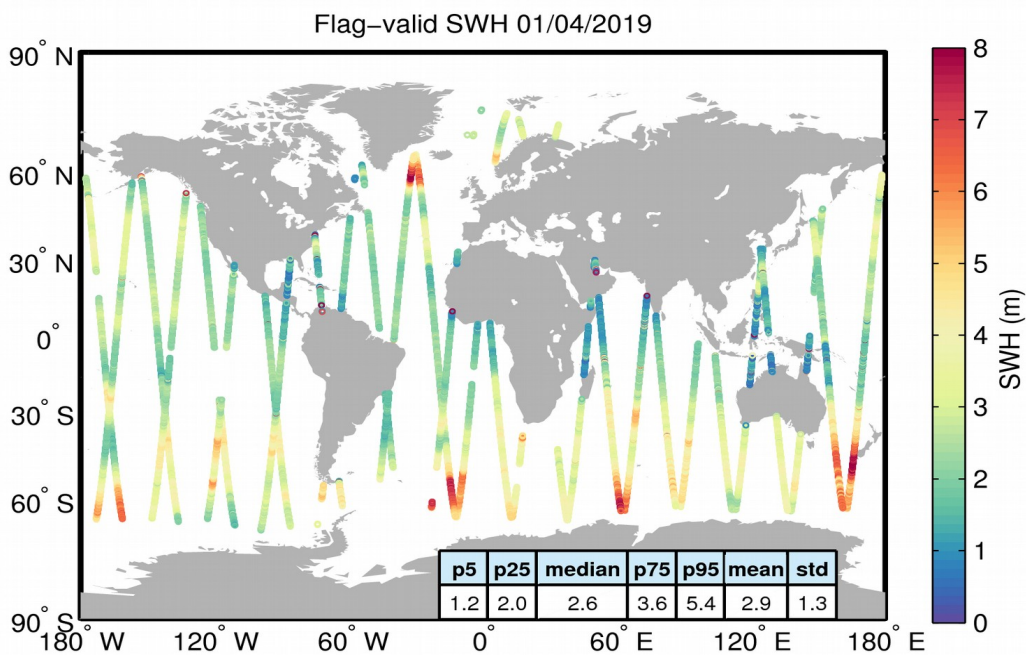
Figure 15. Geographical distribution of flag-valid SWH data over oceans and lakes for 01/04/2019. The statistical values shown in the table refer to the SWH in m and are calculated over all measurements shown in the figure.
