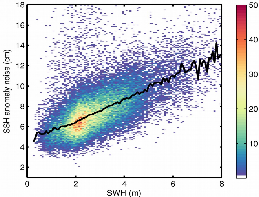
Figure 9. 2D histogram showing flag-valid SSH anomaly noise as a function of SWH for 01/04/2019. The black line denotes the median SSH anomaly noise as a function of SWH.
