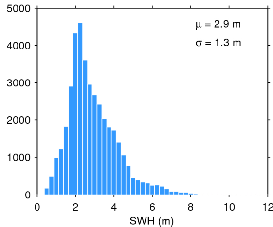
Figure 20. Histogram of science-valid SWH over oceans and lakes for 01/04/2019. The mean ( \mu ) and standard deviation ( \sigma ) are also shown. Note that values larger than 12 m are excluded from the histogram for the sake of readability but not from the computation of \mu and \sigma .
