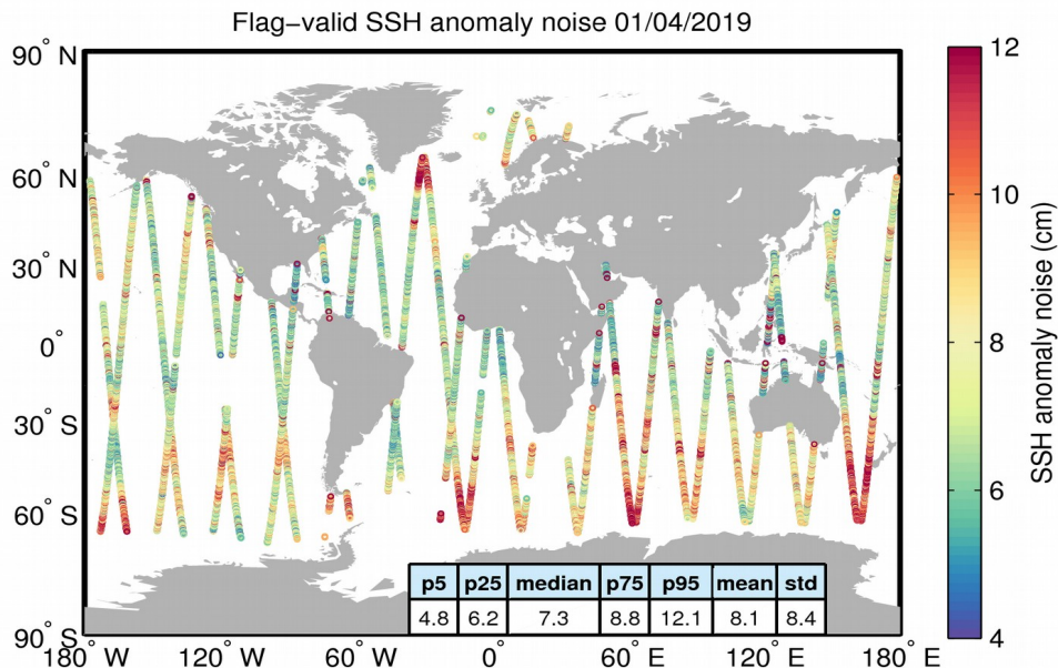
Figure 8. Geographical distribution of flag-valid 20-Hz SSH anomaly measurement noise over oceans and lakes for 01/04/2019. The statistical values shown in the table refer to the SSH anomaly noise and are calculated over all measurements shown in the figure.
