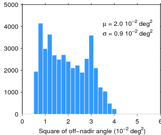
Figure 39. Histogram of flag-valid mispointing over oceans and lakes for 01/04/2019. The mean ( \mu ) and standard deviation ( \sigma ) are also shown. Note that values larger than 6 \cdot 10^{-2} \text{ deg}^2 are excluded from the histogram for the sake of readability but not from the computation of \mu and \sigma .
