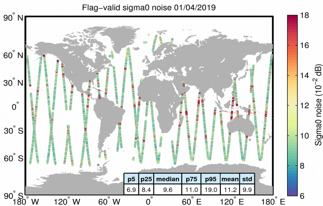
Figure 26. Geographical distribution of flag-valid 20-Hz sigma0 measurement noise over oceans and lakes for 01/04/2019. The statistical values shown in the figure refer to the sigma0 noise and are calculated over all measurements shown in the figure.
