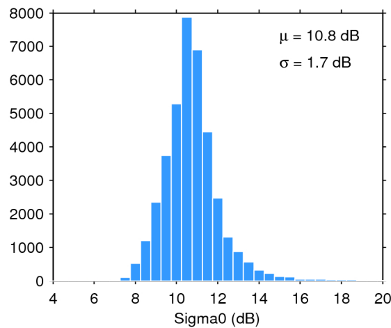
Figure 28. Histogram of science-valid sigma0 over oceans and lakes for 01/04/2019. The mean ( \mu ) and standard deviation ( \sigma ) are also shown. Note that values outside [4 20] dB are excluded from the histogram for the sake of readability but not from the computation of \mu and \sigma .
