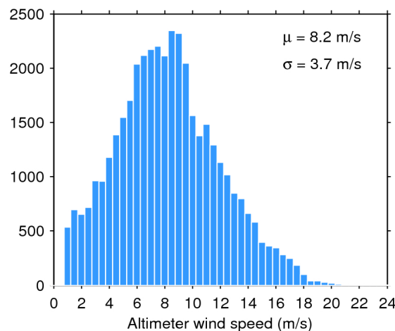
Figure 35. Histogram of science-valid wind over oceans and lakes for 01/04/2019. The mean ( \mu ) and standard deviation ( \sigma ) are also shown. Note that values larger than 24 m/s are excluded from the histogram for the sake of readability but not from the computation of \mu and \sigma .
