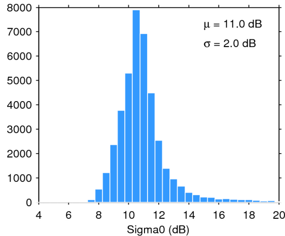
Figure 25. Histogram of flag-valid sigma0 over oceans and lakes for 01/04/2019. The mean ( \mu ) and standard deviation ( \sigma ) are also shown. Note that values outside [4 20] dB are excluded from the histogram for the sake of readability but not from the computation of \mu and \sigma .
