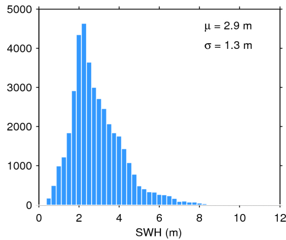
Figure 17. Histogram of flag-valid SWH over oceans and lakes for 01/04/2019. The mean ( \mu ) and standard deviation ( \sigma ) are also shown. Note that values larger than 12 m are excluded from the histogram for the sake of readability but not from the computation of \mu and \sigma .
