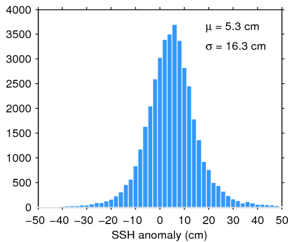
Figure 7. Histogram of flag-valid SSH anomaly over oceans and lakes for 01/04/2019. The mean ( \mu ) and standard deviation ( \sigma ) are also shown. Note that values outside [-50\ 50] cm are excluded from the histogram for the sake of readability but not from the computation of \mu and \sigma .
