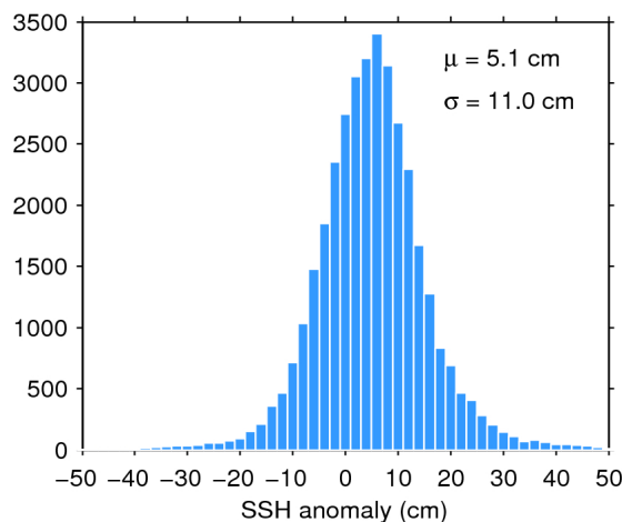
Figure 11. Histogram of science-valid SSH anomaly over oceans and lakes for 01/04/2019. The mean ( \mu ) and standard deviation ( \sigma ) are also shown. Note that values outside [-50 50] cm are excluded from the histogram for the sake of readability but not from the computation of \mu and \sigma .
