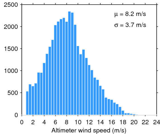
Figure 33. Histogram of flag-valid wind over oceans and lakes for 01/04/2019. The mean ( \mu ) and standard deviation ( \sigma ) are also shown. Note that values larger than 24 m/s are excluded from the histogram for the sake of readability but not from the computation of \mu and \sigma .
