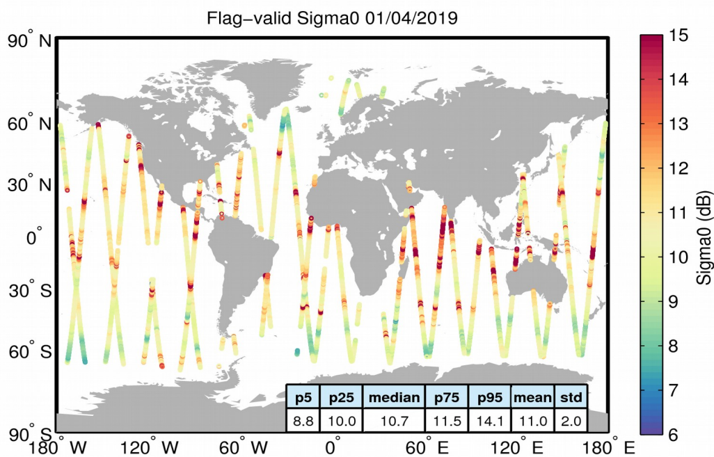
Figure 23. Geographical distribution of flag-valid sigma0 data over oceans and lakes for 01/04/2019. The statistical values shown in the table refer to the sigma0 in dB and are calculated over all measurements shown in the figure.
