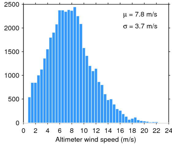
Figure 33. Histogram of flag-valid wind over oceans and lakes for 31/03/2019. The mean ( \mu ) and standard deviation ( \sigma ) are also shown. Note that values larger than 24 m/s are excluded from the histogram for the sake of readability but not from the computation of \mu and \sigma .
