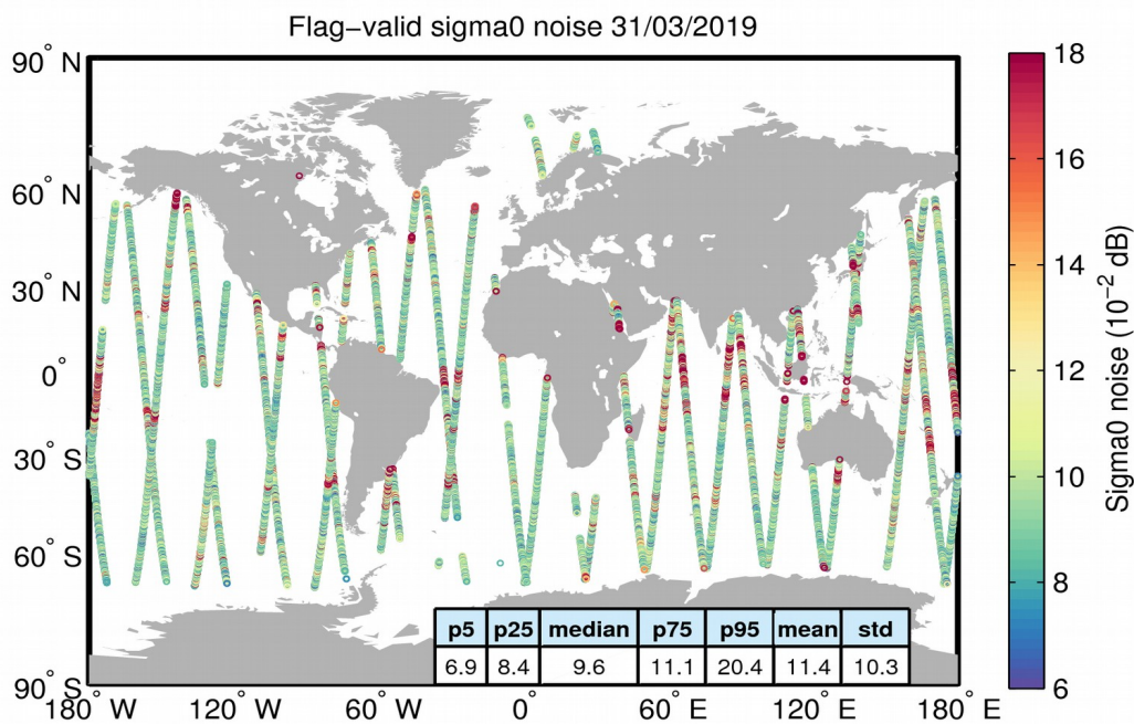
Figure 26. Geographical distribution of flag-valid 20-Hz sigma0 measurement noise over oceans and lakes for 31/03/2019. The statistical values shown in the table refer to the sigma0 noise and are calculated over all measurements shown in the figure.
