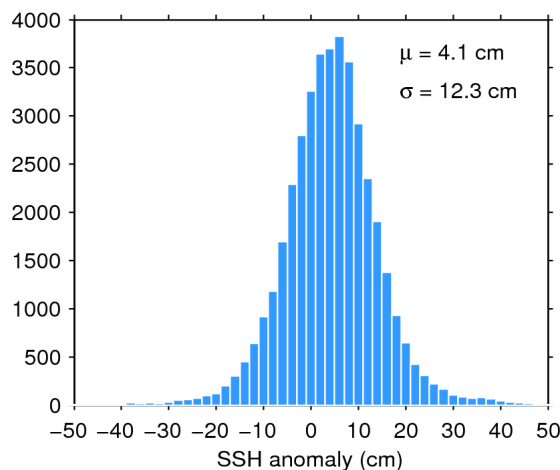
Figure 11. Histogram of science-valid SSH anomaly over oceans and lakes for 31/03/2019. The mean ( \mu ) and standard deviation ( \sigma ) are also shown. Note that values outside [-50 50] cm are excluded from the histogram for the sake of readability but not from the computation of \mu and \sigma .
