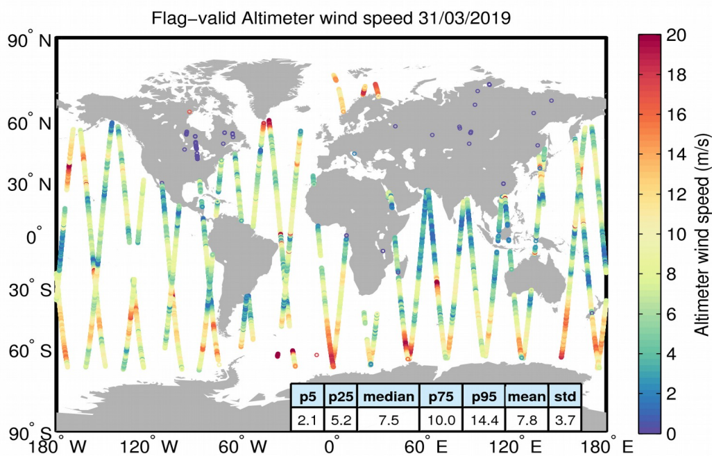
Figure 31. Geographical distribution of flag-valid wind data over oceans and lakes for 31/03/2019. The statistical values shown in the table refer to the wind in m/s and are calculated over all measurements shown in the figure.
