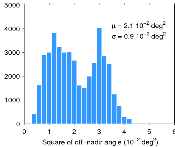
Figure 39. Histogram of flag-valid mispointing over oceans and lakes for 31/03/2019. The mean ( \mu ) and standard deviation ( \sigma ) are also shown. Note that values larger than 6 \cdot 10^{-2} \text{ deg}^2 are excluded from the histogram for the sake of readability but not from the computation of \mu and \sigma .
