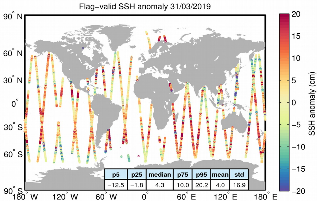
Figure 5. Geographical distribution of flag-valid 1-Hz SSH anomaly data over oceans and lakes for 31/03/2019. The statistical values shown in the table refer to the SSH anomaly in cm and are calculated over all measurements shown in the figure.
