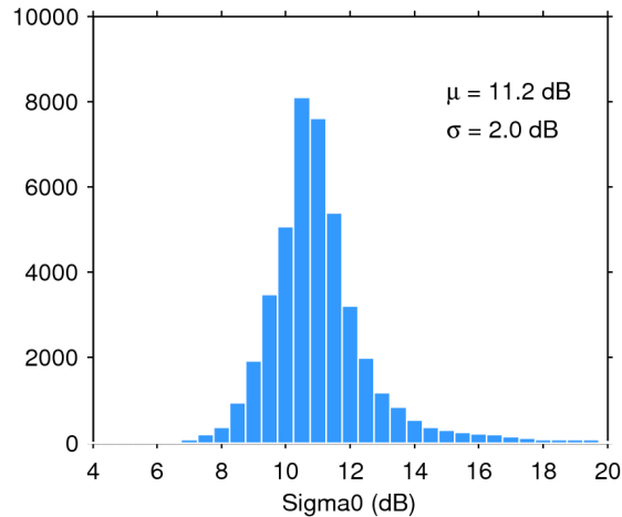
Figure 25. Histogram of flag-valid sigma0 over oceans and lakes for 31/03/2019. The mean ( \mu ) and standard deviation ( \sigma ) are also shown. Note that values outside [4 20] dB are excluded from the histogram for the sake of readability but not from the computation of \mu and \sigma .
