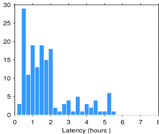
Figure 2. Histogram of the data latency for 31/03/2019. The y-axis denotes the number of files that are made available with a delay of x-hours with respect to the mean time of the records stored in the file.
