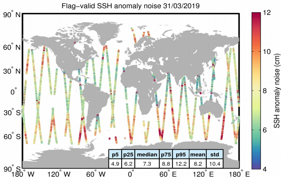
Figure 8. Geographical distribution of flag-valid 20-Hz SSH anomaly measurement noise over oceans and lakes for 31/03/2019. The statistical values shown in the table refer to the SSH anomaly noise and are calculated over all measurements shown in the figure.
