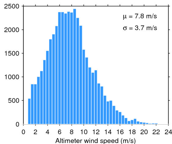
Figure 35. Histogram of science-valid wind over oceans and lakes for 31/03/2019. The mean ( \mu ) and standard deviation ( \sigma ) are also shown. Note that values larger than 24 m/s are excluded from the histogram for the sake of readability but not from the computation of \mu and \sigma .
