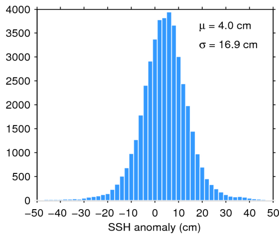
Figure 7. Histogram of flag-valid SSH anomaly over oceans and lakes for 31/03/2019. The mean ( \mu ) and standard deviation ( \sigma ) are also shown. Note that values outside [-50 50] cm are excluded from the histogram for the sake of readability but not from the computation of \mu and \sigma .
