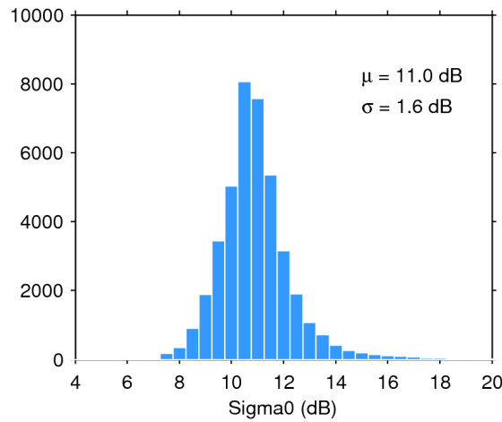
Figure 28. Histogram of science-valid sigma0 over oceans and lakes for 31/03/2019. The mean ( \mu ) and standard deviation ( \sigma ) are also shown. Note that values outside [4 20] dB are excluded from the histogram for the sake of readability but not from the computation of \mu and \sigma .
