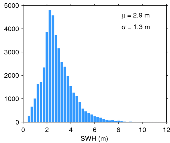
Figure 17. Histogram of flag-valid SWH over oceans and lakes for 31/03/2019. The mean ( \mu ) and standard deviation ( \sigma ) are also shown. Note that values larger than 12 m are excluded from the histogram for the sake of readability but not from the computation of \mu and \sigma .
