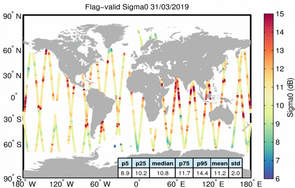
Figure 23. Geographical distribution of flag-valid sigma0 data over oceans and lakes for 31/03/2019. The statistical values shown in the table refer to the sigma0 in dB and are calculated over all measurements shown in the figure.
