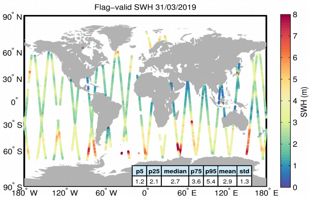
Figure 15. Geographical distribution of flag-valid SWH data over oceans and lakes for 31/03/2019. The statistical values shown in the table refer to the SWH in m and are calculated over all measurements shown in the figure.
