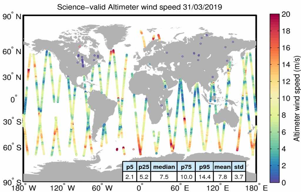
Figure 34. Geographical distribution of science-valid wind data over oceans and lakes for 31/03/2019. The statistical values shown in the table refer to the wind in m/s and are calculated over all measurements shown in the figure. Gray circles denote records that have been rejected based on the editing criteria described in Table 5.
