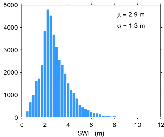
Figure 20. Histogram of science-valid SWH over oceans and lakes for 31/03/2019. The mean ( \mu ) and standard deviation ( \sigma ) are also shown. Note that values larger than 12 m are excluded from the histogram for the sake of readability but not from the computation of \mu and \sigma .
