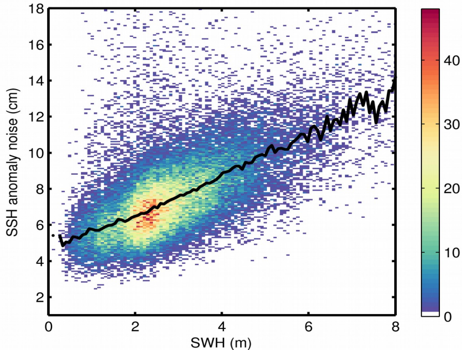
Figure 9. 2D histogram showing flag-valid SSH anomaly noise as a function of SWH for 31/03/2019. The black line denotes the median SSH anomaly noise as a function of SWH.
