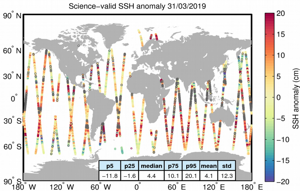
Figure 10. Geographical distribution of science-valid SSH anomaly data over oceans and lakes for 31/03/2019. The statistical values shown in the table refer to the SSH anomaly in cm and are calculated over all measurements shown in the figure. Gray circles denote records that have been rejected based on the editing criteria described in Table 2.
