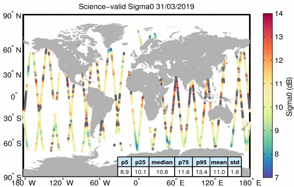
Figure 27. Geographical distribution of science-valid sigma0 data over oceans and lakes for 31/03/2019. The statistical values shown in the table refer to the sigma0 in dB and are calculated over all measurements shown in the figure. Gray circles denote records that have been rejected based on the editing criteria described in Table 4.
